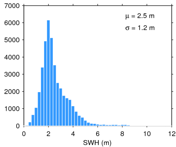
Figure 17. Histogram of flag-valid SWH over oceans and lakes for 03/01/2017. The mean ( \mu ) and standard deviation ( \sigma ) are also shown. Note that values larger than 12 m are excluded from the histogram for the sake of readability but not from the computation of \mu and \sigma .
