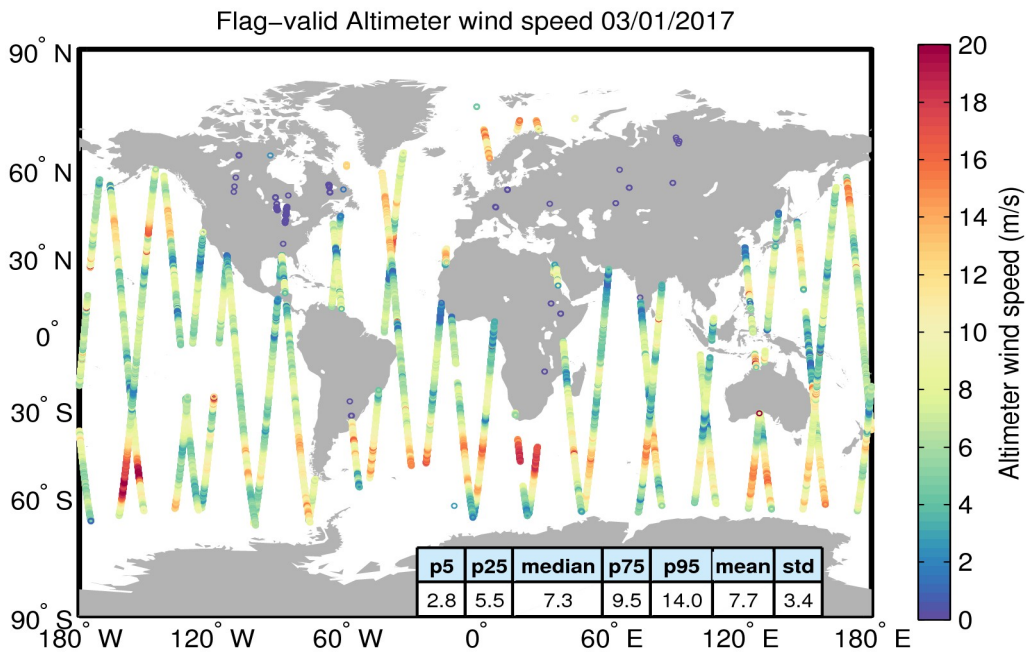
Figure 31. Geographical distribution of flag-valid wind data over oceans and lakes for 03/01/2017. The statistical values shown in the table refer to the wind in m/s and are calculated over all measurements shown in the figure.
