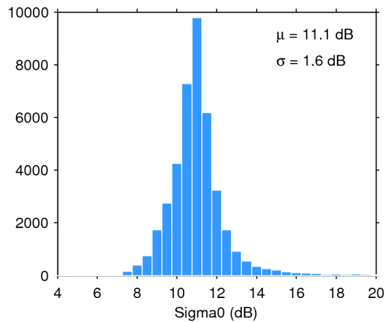
Figure 25. Histogram of flag-valid sigma0 over oceans and lakes for 03/01/2017. The mean ( \mu ) and standard deviation ( \sigma ) are also shown. Note that values outside [4 20] dB are excluded from the histogram for the sake of readability but not from the computation of \mu and \sigma .
