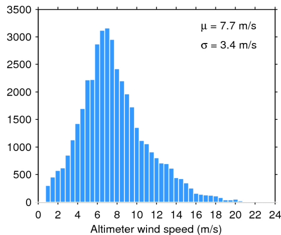
Figure 35. Histogram of science-valid wind over oceans and lakes for 03/01/2017. The mean ( \mu ) and standard deviation ( \sigma ) are also shown. Note that values larger than 24 m/s are excluded from the histogram for the sake of readability but not from the computation of \mu and \sigma .
