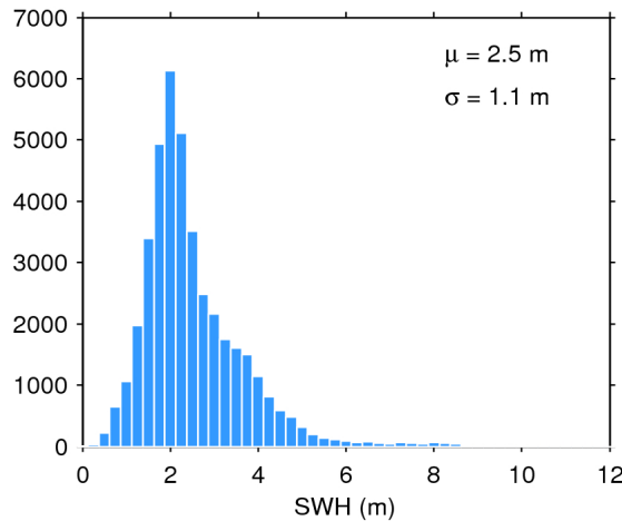
Figure 20. Histogram of science-valid SWH over oceans and lakes for 03/01/2017. The mean ( \mu ) and standard deviation ( \sigma ) are also shown. Note that values larger than 12 m are excluded from the histogram for the sake of readability but not from the computation of \mu and \sigma .
