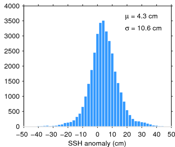
Figure 11. Histogram of science-valid SSH anomaly over oceans and lakes for 03/01/2017. The mean ( \mu ) and standard deviation ( \sigma ) are also shown. Note that values outside [-50 50] cm are excluded from the histogram for the sake of readability but not from the computation of \mu and \sigma .
