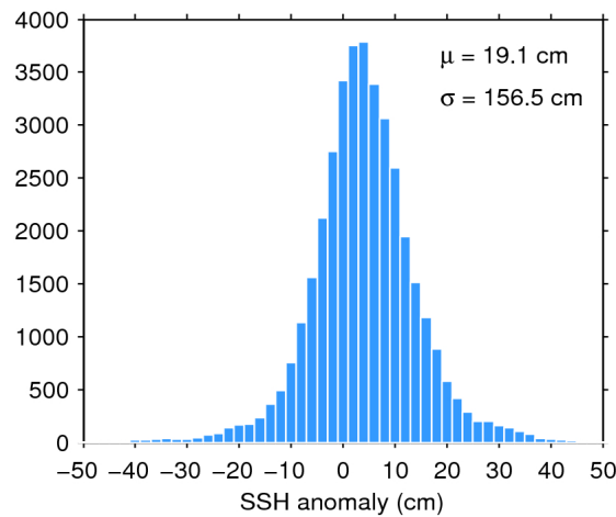
Figure 7. Histogram of flag-valid SSH anomaly over oceans and lakes for 03/01/2017. The mean ( \mu ) and standard deviation ( \sigma ) are also shown. Note that values outside [-50 50] cm are excluded from the histogram for the sake of readability but not from the computation of \mu and \sigma .
