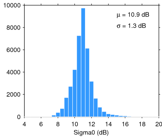
Figure 28. Histogram of science-valid sigma0 over oceans and lakes for 03/01/2017. The mean ( \mu ) and standard deviation ( \sigma ) are also shown. Note that values outside [4 20] dB are excluded from the histogram for the sake of readability but not from the computation of \mu and \sigma .
