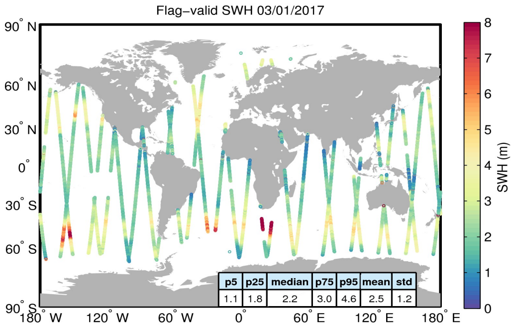
Figure 15. Geographical distribution of flag-valid SWH data over oceans and lakes for 03/01/2017. The statistical values shown in the table refer to the SWH in m and are calculated over all measurements shown in the figure.
