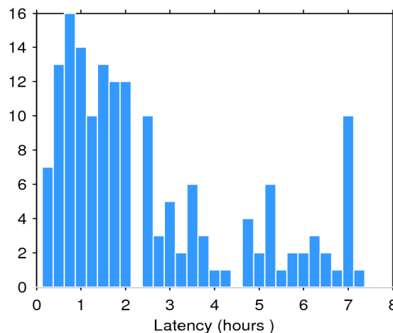
Figure 2. Histogram of the data latency for 03/01/2017. The y-axis denotes the number of files that are made available with a delay of x-hours with respect to the mean time of the records stored in the file.
