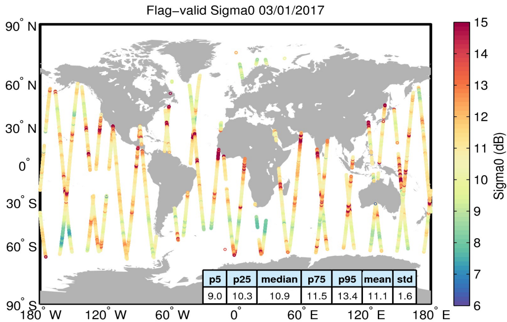
Figure 23. Geographical distribution of flag-valid sigma0 data over oceans and lakes for 03/01/2017. The statistical values shown in the table refer to the sigma0 in dB and are calculated over all measurements shown in the figure.
