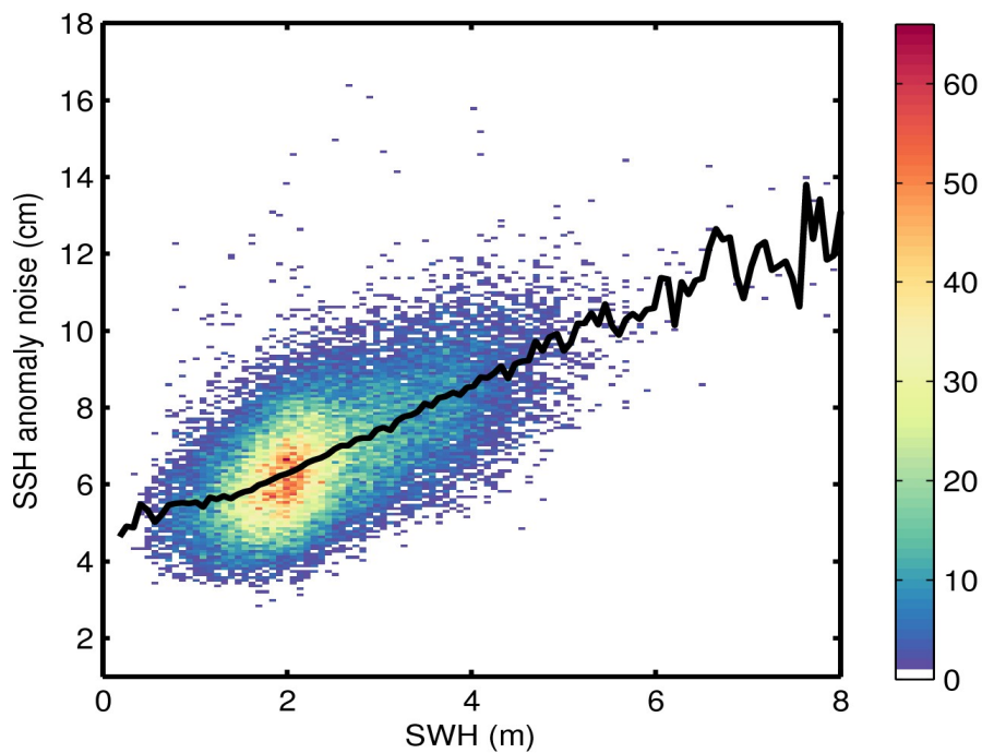
Figure 9. 2D histogram showing flag-valid SSH anomaly noise as a function of SWH for 03/01/2017. The black line denotes the median SSH anomaly noise as a function of SWH.
