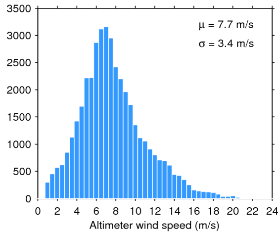
Figure 33. Histogram of flag-valid wind over oceans and lakes for 03/01/2017. The mean ( \mu ) and standard deviation ( \sigma ) are also shown. Note that values larger than 24 m/s are excluded from the histogram for the sake of readability but not from the computation of \mu and \sigma .
