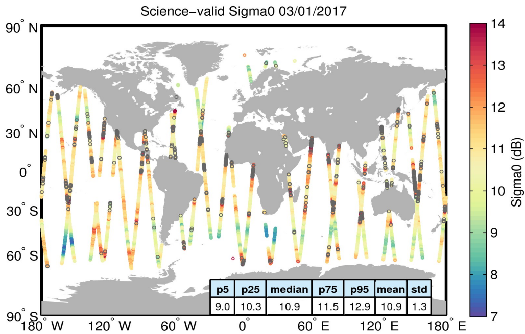
Figure 27. Geographical distribution of science-valid sigma0 data over oceans and lakes for 03/01/2017. The statistical values shown in the table refer to the sigma0 in dB and are calculated over all measurements shown in the figure. Gray circles denote records that have been rejected based on the editing criteria described in Table 4.
