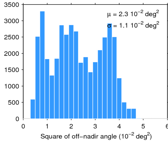
Figure 39. Histogram of flag-valid mispointing over oceans and lakes for 03/01/2017. The mean ( \mu ) and standard deviation ( \sigma ) are also shown. Note that values larger than 6 \cdot 10^{-2} \text{ deg}^2 are excluded from the histogram for the sake of readability but not from the computation of \mu and \sigma .
