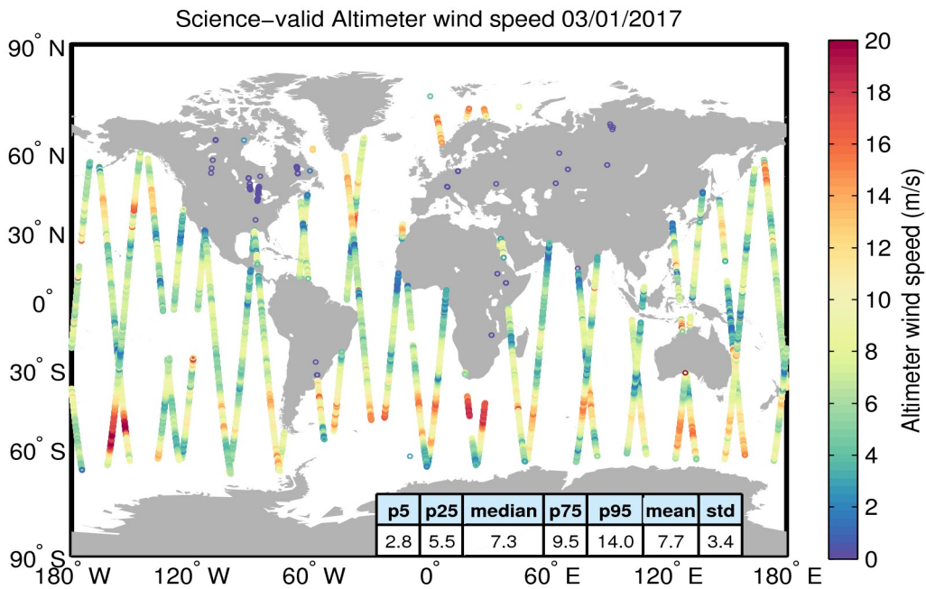
Figure 34. Geographical distribution of science-valid wind data over oceans and lakes for 03/01/2017. The statistical values shown in the table refer to the wind in m/s and are calculated over all measurements shown in the figure. Gray circles denote records that have been rejected based on the editing criteria described in Table 5.
