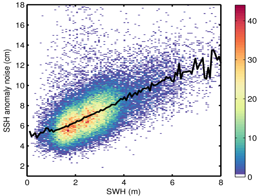
Figure 9. 2D histogram showing flag-valid SSH anomaly noise as a function of SWH for 31/12/2016. The black line denotes the median SSH anomaly noise as a function of SWH.
