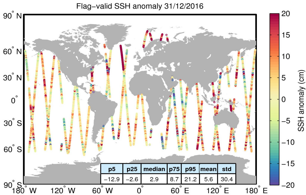
Figure 5. Geographical distribution of flag-valid 1-Hz SSH anomaly data over oceans and lakes for 31/12/2016. The statistical values shown in the table refer to the SSH anomaly in cm and are calculated over all measurements shown in the figure.
