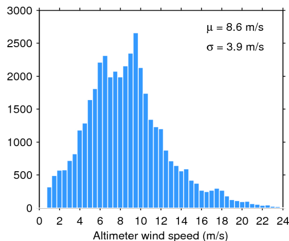
Figure 35. Histogram of science-valid wind over oceans and lakes for 31/12/2016. The mean ( \mu ) and standard deviation ( \sigma ) are also shown. Note that values larger than 24 m/s are excluded from the histogram for the sake of readability but not from the computation of \mu and \sigma .
