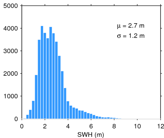
Figure 20. Histogram of science-valid SWH over oceans and lakes for 31/12/2016. The mean ( \mu ) and standard deviation ( \sigma ) are also shown. Note that values larger than 12 m are excluded from the histogram for the sake of readability but not from the computation of \mu and \sigma .
