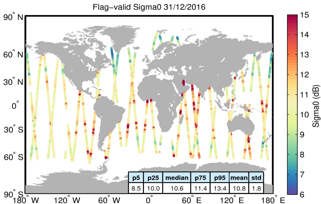
Figure 23. Geographical distribution of flag-valid sigma0 data over oceans and lakes for 31/12/2016. The statistical values shown in the table refer to the sigma0 in dB and are calculated over all measurements shown in the figure.
