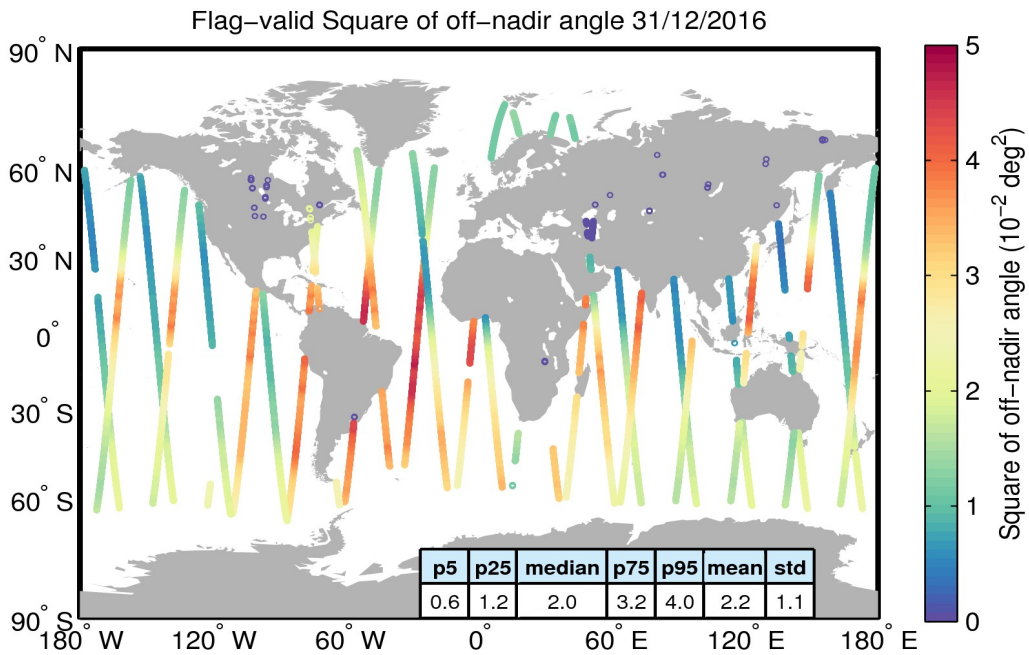
Figure 37. Geographical distribution of flag-valid mispointing data over oceans and lakes for 31/12/2016. The statistical values shown in the table refer to the mispointing in 10^{-2} \text{deg}^2 and are calculated over all measurements shown in the figure.
