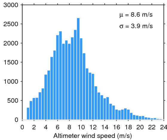
Figure 33. Histogram of flag-valid wind over oceans and lakes for 31/12/2016. The mean ( \mu ) and standard deviation ( \sigma ) are also shown. Note that values larger than 24 m/s are excluded from the histogram for the sake of readability but not from the computation of \mu and \sigma .
