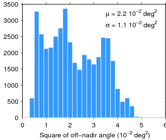
Figure 39. Histogram of flag-valid mispointing over oceans and lakes for 31/12/2016. The mean ( \mu ) and standard deviation ( \sigma ) are also shown. Note that values larger than 6 \cdot 10^{-2} \text{ deg}^2 are excluded from the histogram for the sake of readability but not from the computation of \mu and \sigma .
