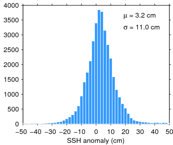
Figure 11. Histogram of science-valid SSH anomaly over oceans and lakes for 31/12/2016. The mean ( \mu ) and standard deviation ( \sigma ) are also shown. Note that values outside [-50 50] cm are excluded from the histogram for the sake of readability but not from the computation of \mu and \sigma .
