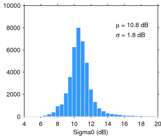
Figure 25. Histogram of flag-valid sigma0 over oceans and lakes for 31/12/2016. The mean ( \mu ) and standard deviation ( \sigma ) are also shown. Note that values outside [4 20] dB are excluded from the histogram for the sake of readability but not from the computation of \mu and \sigma .
