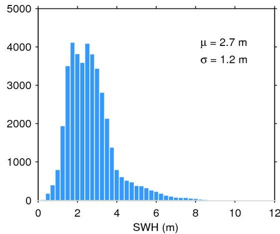
Figure 17. Histogram of flag-valid SWH over oceans and lakes for 31/12/2016. The mean ( \mu ) and standard deviation ( \sigma ) are also shown. Note that values larger than 12 m are excluded from the histogram for the sake of readability but not from the computation of \mu and \sigma .
