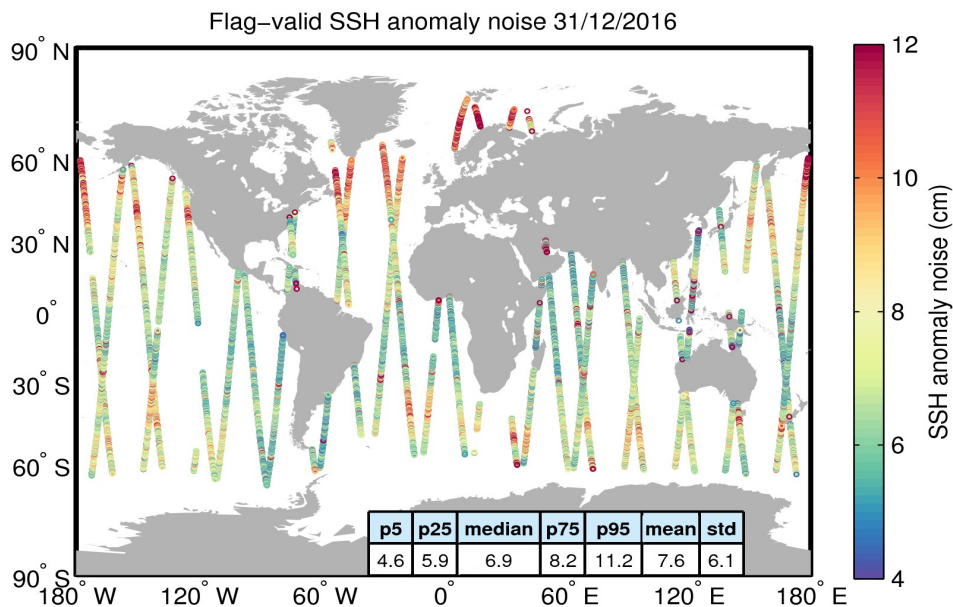
Figure 8. Geographical distribution of flag-valid 20-Hz SSH anomaly measurement noise over oceans and lakes for 31/12/2016. The statistical values shown in the table refer to the SSH anomaly noise and are calculated over all measurements shown in the figure.
