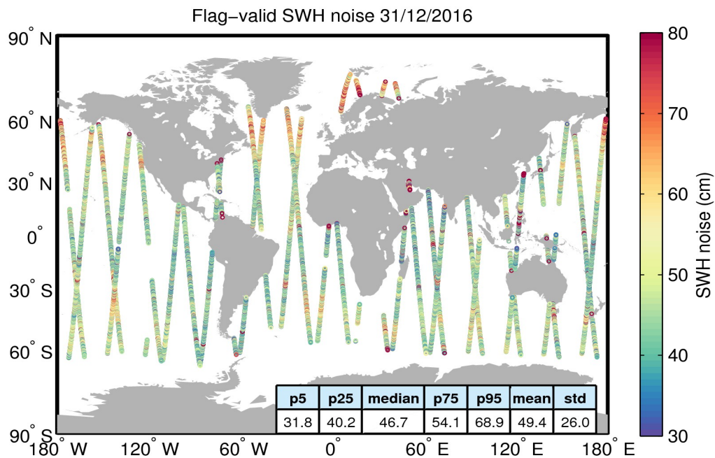
Figure 18. Geographical distribution of flag-valid 20-Hz SWH measurement noise over oceans and lakes for 31/12/2016. The statistical values shown in the table refer to the SWH noise and are calculated over all measurements shown in the figure.
