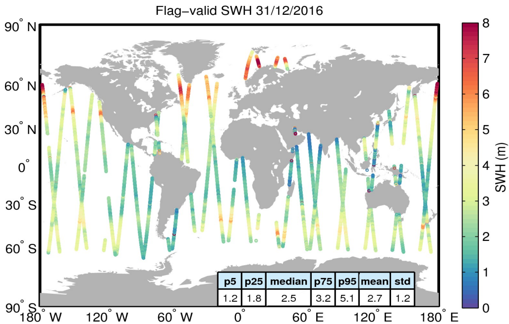
Figure 15. Geographical distribution of flag-valid SWH data over oceans and lakes for 31/12/2016. The statistical values shown in the table refer to the SWH in m and are calculated over all measurements shown in the figure.
