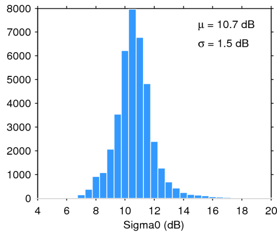
Figure 28. Histogram of science-valid sigma0 over oceans and lakes for 31/12/2016. The mean ( \mu ) and standard deviation ( \sigma ) are also shown. Note that values outside [4 20] dB are excluded from the histogram for the sake of readability but not from the computation of \mu and \sigma .
