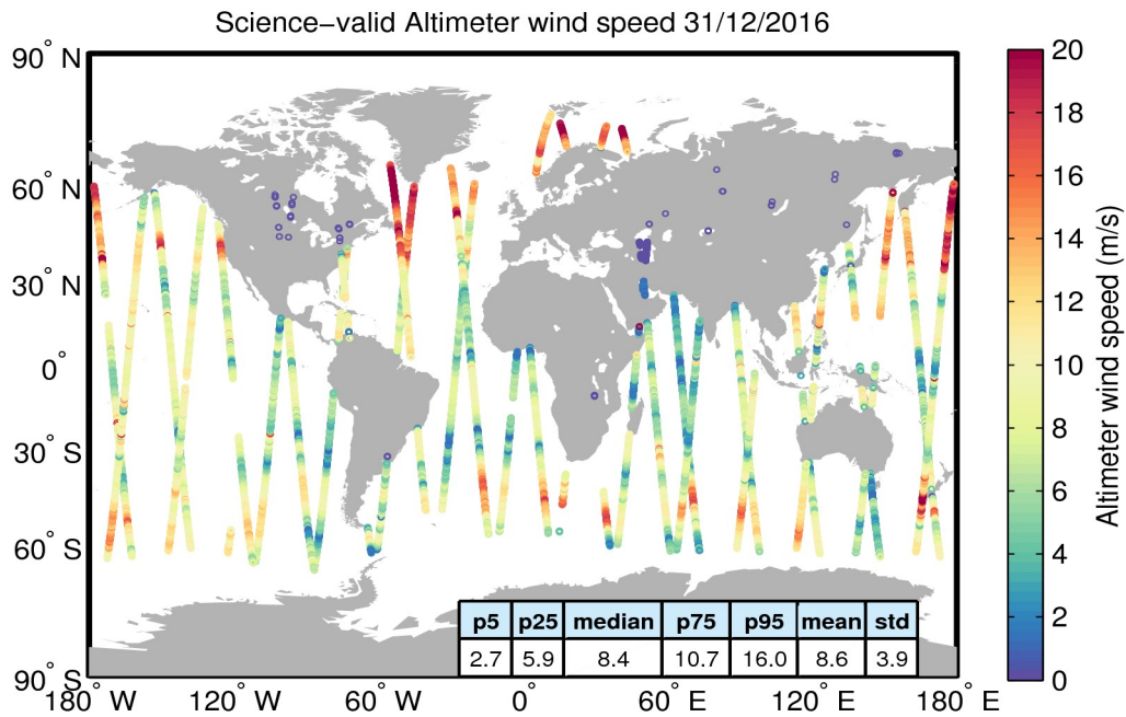
Figure 34. Geographical distribution of science-valid wind data over oceans and lakes for 31/12/2016. The statistical values shown in the table refer to the wind in m/s and are calculated over all measurements shown in the figure. Gray circles denote records that have been rejected based on the editing criteria described in Table 5.
