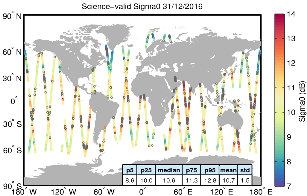
Figure 27. Geographical distribution of science-valid sigma0 data over oceans and lakes for 31/12/2016. The statistical values shown in the table refer to the sigma0 in dB and are calculated over all measurements shown in the figure. Gray circles denote records that have been rejected based on the editing criteria described in Table 4.
