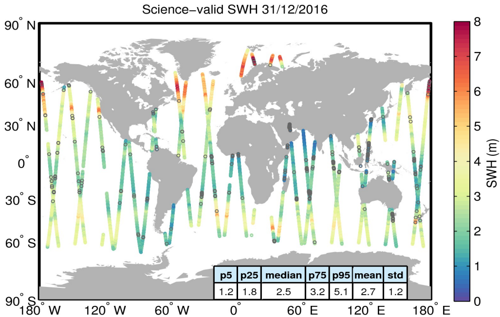
Figure 19. Geographical distribution of science-valid SWH data over oceans and lakes for 31/12/2016. The statistical values shown in the table refer to the SWH in m and are calculated over all measurements shown in the figure. Gray circles denote records that have been rejected based on the editing criteria described in Table 3.
