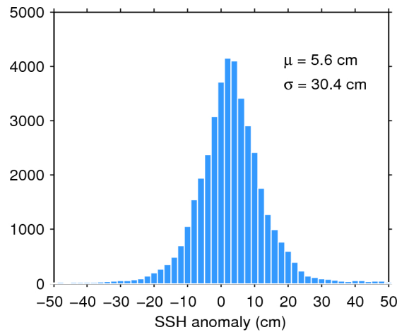
Figure 7. Histogram of flag-valid SSH anomaly over oceans and lakes for 31/12/2016. The mean ( \mu ) and standard deviation ( \sigma ) are also shown. Note that values outside [-50\ 50] cm are excluded from the histogram for the sake of readability but not from the computation of \mu and \sigma .
