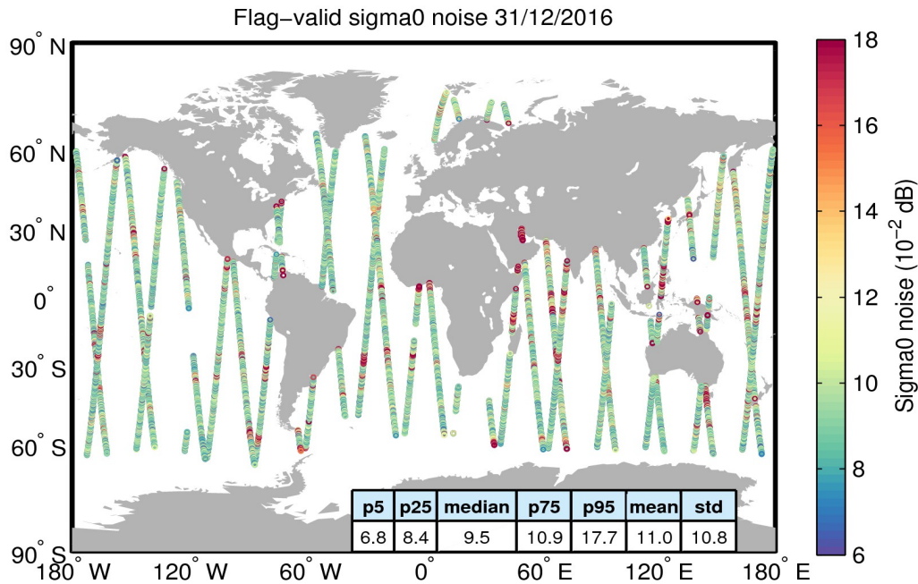
Figure 26. Geographical distribution of flag-valid 20-Hz sigma0 measurement noise over oceans and lakes for 31/12/2016. The statistical values shown in the table refer to the sigma0 noise and are calculated over all measurements shown in the figure.
