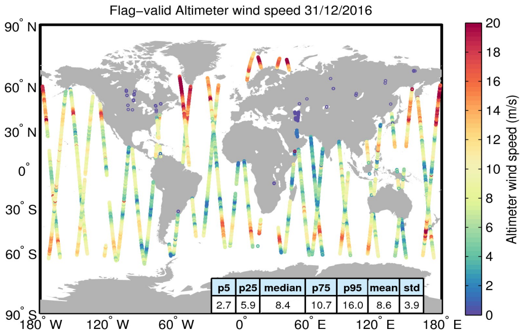
Figure 31. Geographical distribution of flag-valid wind data over oceans and lakes for 31/12/2016. The statistical values shown in the table refer to the wind in m/s and are calculated over all measurements shown in the figure.
