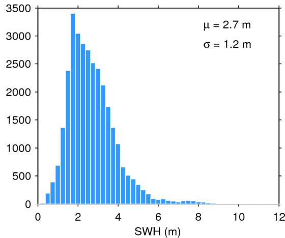
Figure 20. Histogram of science-valid SWH over oceans and lakes for 30/12/2016. The mean ( \mu ) and standard deviation ( \sigma ) are also shown. Note that values larger than 12 m are excluded from the histogram for the sake of readability but not from the computation of \mu and \sigma .
