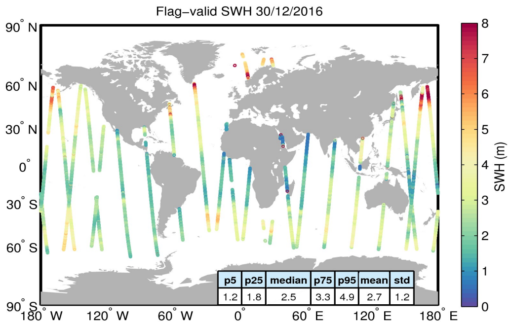
Figure 15. Geographical distribution of flag-valid SWH data over oceans and lakes for 30/12/2016. The statistical values shown in the table refer to the SWH in m and are calculated over all measurements shown in the figure.
