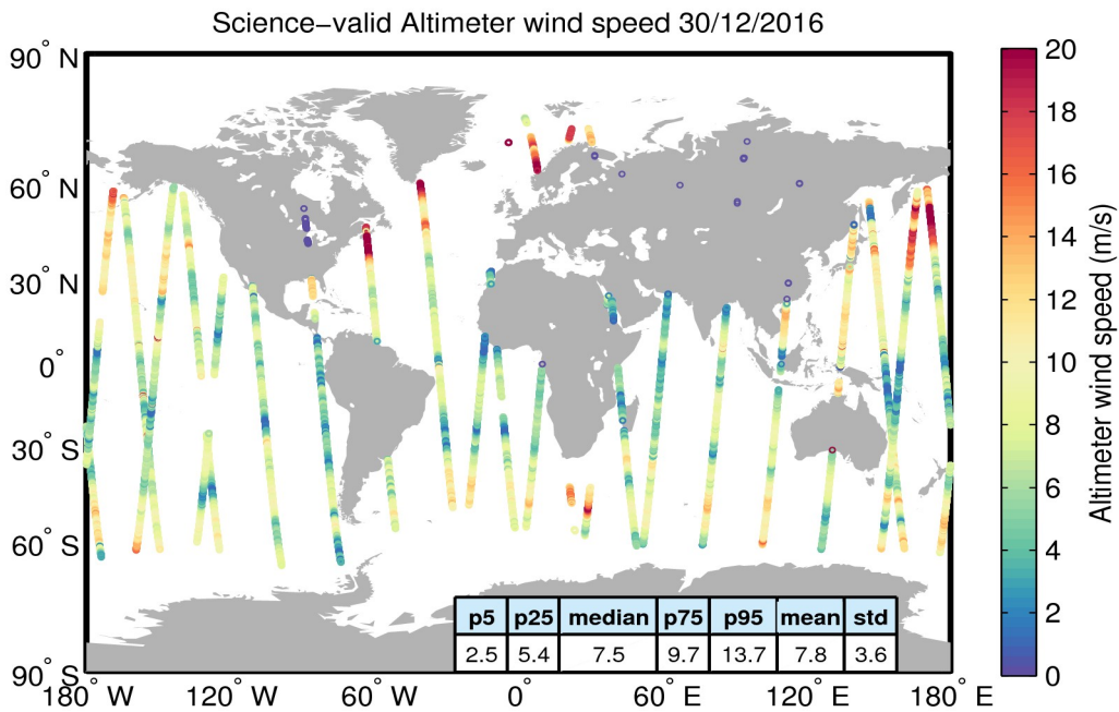
Figure 34. Geographical distribution of science-valid wind data over oceans and lakes for 30/12/2016. The statistical values shown in the table refer to the wind in m/s and are calculated over all measurements shown in the figure. Gray circles denote records that have been rejected based on the editing criteria described in Table 5.
