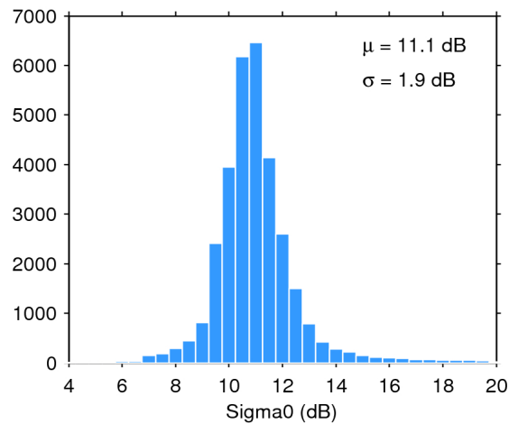
Figure 25. Histogram of flag-valid sigma0 over oceans and lakes for 30/12/2016. The mean ( \mu ) and standard deviation ( \sigma ) are also shown. Note that values outside [4 20] dB are excluded from the histogram for the sake of readability but not from the computation of \mu and \sigma .
