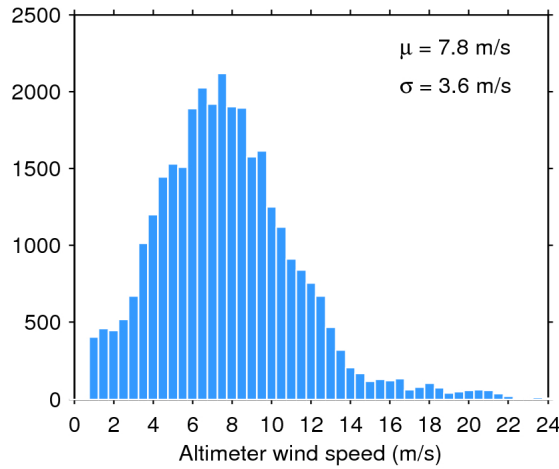
Figure 33. Histogram of flag-valid wind over oceans and lakes for 30/12/2016. The mean ( \mu ) and standard deviation ( \sigma ) are also shown. Note that values larger than 24 m/s are excluded from the histogram for the sake of readability but not from the computation of \mu and \sigma .
