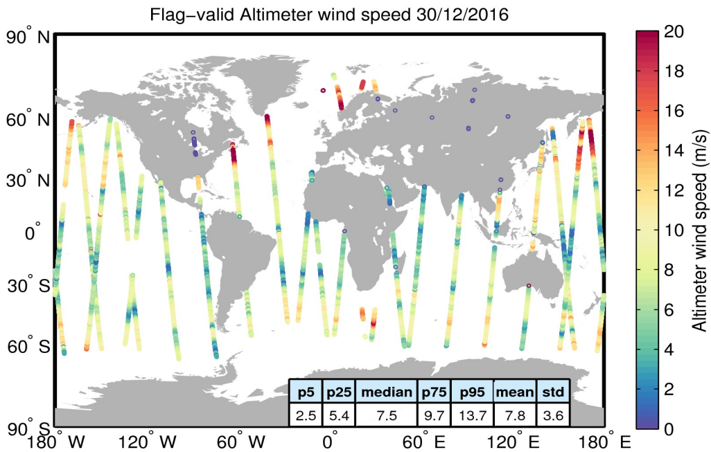
Figure 31. Geographical distribution of flag-valid wind data over oceans and lakes for 30/12/2016. The statistical values shown in the table refer to the wind in m/s and are calculated over all measurements shown in the figure.
