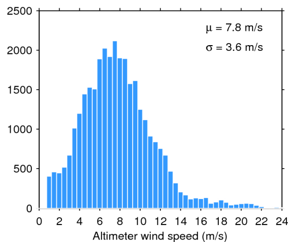
Figure 35. Histogram of science-valid wind over oceans and lakes for 30/12/2016. The mean ( \mu ) and standard deviation ( \sigma ) are also shown. Note that values larger than 24 m/s are excluded from the histogram for the sake of readability but not from the computation of \mu and \sigma .
