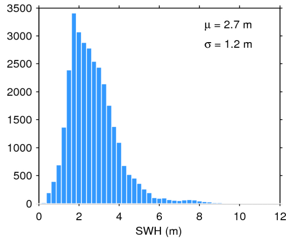
Figure 17. Histogram of flag-valid SWH over oceans and lakes for 30/12/2016. The mean ( \mu ) and standard deviation ( \sigma ) are also shown. Note that values larger than 12 m are excluded from the histogram for the sake of readability but not from the computation of \mu and \sigma .
