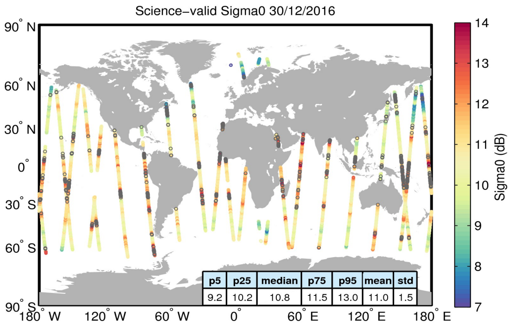
Figure 27. Geographical distribution of science-valid sigma0 data over oceans and lakes for 30/12/2016. The statistical values shown in the table refer to the sigma0 in dB and are calculated over all measurements shown in the figure. Gray circles denote records that have been rejected based on the editing criteria described in Table 4.
