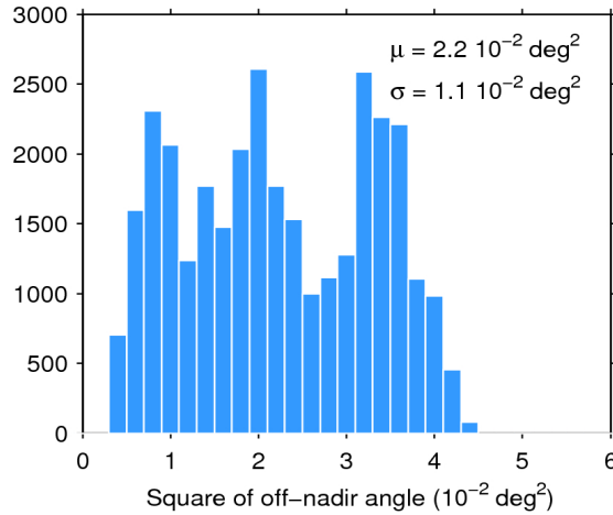
Figure 39. Histogram of flag-valid mispointing over oceans and lakes for 30/12/2016. The mean ( \mu ) and standard deviation ( \sigma ) are also shown. Note that values larger than 6 \cdot 10^{-2} \text{ deg}^2 are excluded from the histogram for the sake of readability but not from the computation of \mu and \sigma .
