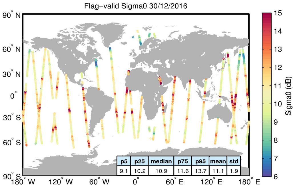
Figure 23. Geographical distribution of flag-valid sigma0 data over oceans and lakes for 30/12/2016. The statistical values shown in the table refer to the sigma0 in dB and are calculated over all measurements shown in the figure.
