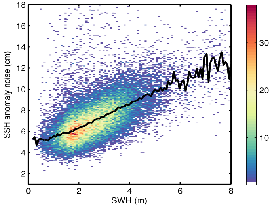
Figure 9. 2D histogram showing flag-valid SSH anomaly noise as a function of SWH for 30/12/2016. The black line denotes the median SSH anomaly noise as a function of SWH.
