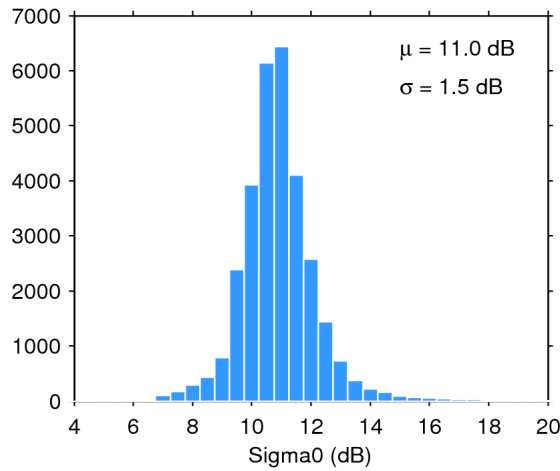
Figure 28. Histogram of science-valid sigma0 over oceans and lakes for 30/12/2016. The mean ( \mu ) and standard deviation ( \sigma ) are also shown. Note that values outside [4 20] dB are excluded from the histogram for the sake of readability but not from the computation of \mu and \sigma .
