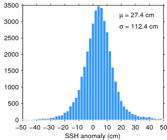
Figure 7. Histogram of flag-valid SSH anomaly over oceans and lakes for 29/12/2016. The mean ( \mu ) and standard deviation ( \sigma ) are also shown. Note that values outside [-50\ 50] cm are excluded from the histogram for the sake of readability but not from the computation of \mu and \sigma .
