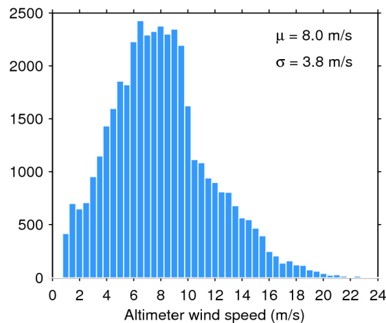
Figure 35. Histogram of science-valid wind over oceans and lakes for 29/12/2016. The mean ( \mu ) and standard deviation ( \sigma ) are also shown. Note that values larger than 24 m/s are excluded from the histogram for the sake of readability but not from the computation of \mu and \sigma .
