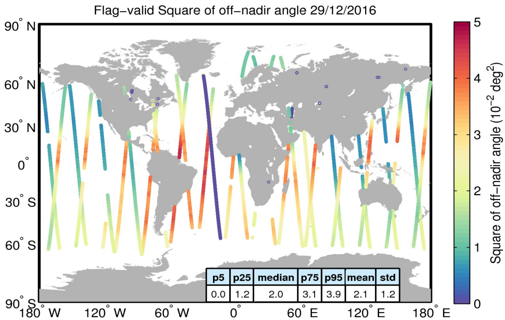
Figure 37. Geographical distribution of flag-valid mispointing data over oceans and lakes for 29/12/2016. The statistical values shown in the table refer to the mispointing in 10^{-2} deg 2 and are calculated over all measurements shown in the figure.
