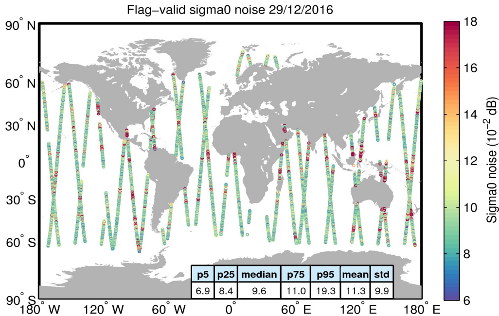
Figure 26. Geographical distribution of flag-valid 20-Hz sigma0 measurement noise over oceans and lakes for 29/12/2016. The statistical values shown in the table refer to the sigma0 noise and are calculated over all measurements shown in the figure.
