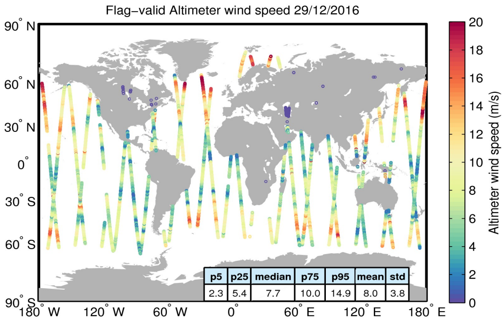
Figure 31. Geographical distribution of flag-valid wind data over oceans and lakes for 29/12/2016. The statistical values shown in the table refer to the wind in m/s and are calculated over all measurements shown in the figure.
