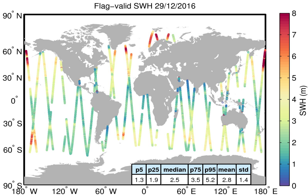
Figure 15. Geographical distribution of flag-valid SWH data over oceans and lakes for 29/12/2016. The statistical values shown in the table refer to the SWH in m and are calculated over all measurements shown in the figure.
