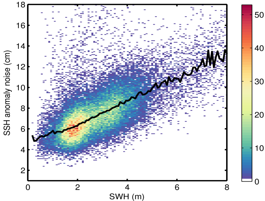
Figure 9. 2D histogram showing flag-valid SSH anomaly noise as a function of SWH for 29/12/2016. The black line denotes the median SSH anomaly noise as a function of SWH.
