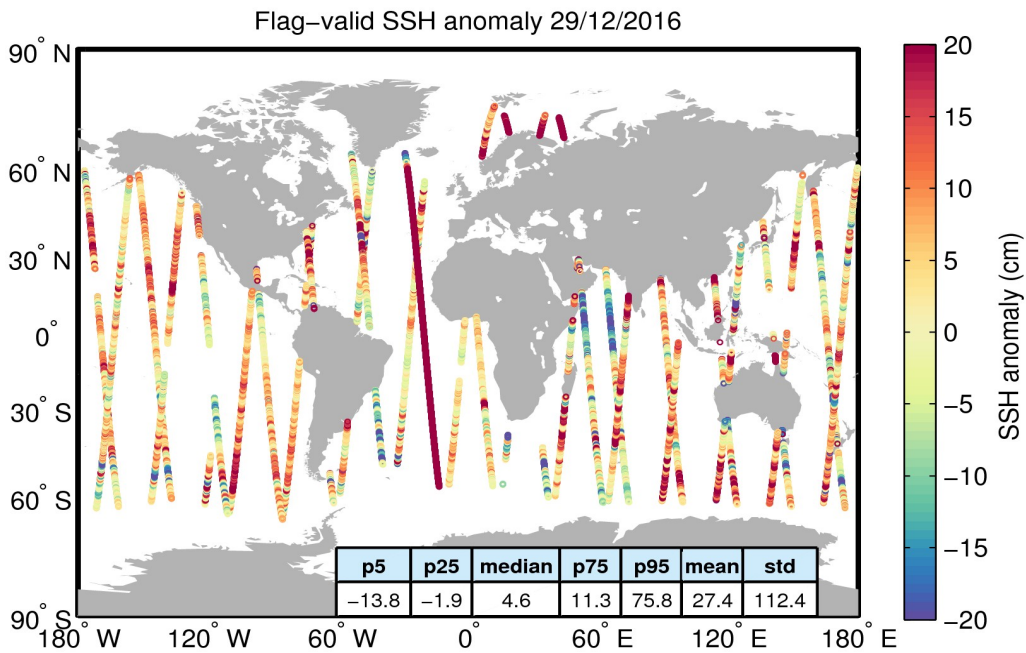
Figure 5. Geographical distribution of flag-valid 1-Hz SSH anomaly data over oceans and lakes for 29/12/2016. The statistical values shown in the table refer to the SSH anomaly in cm and are calculated over all measurements shown in the figure.
