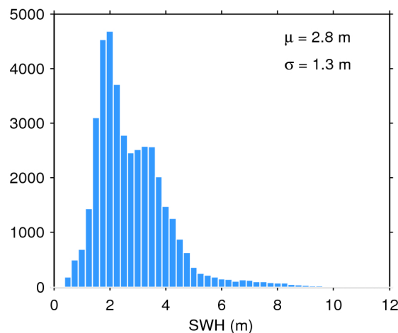
Figure 20. Histogram of science-valid SWH over oceans and lakes for 29/12/2016. The mean ( \mu ) and standard deviation ( \sigma ) are also shown. Note that values larger than 12 m are excluded from the histogram for the sake of readability but not from the computation of \mu and \sigma .
