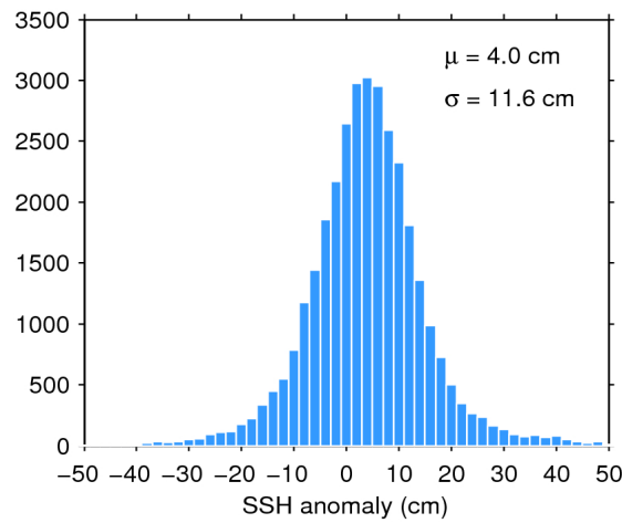
Figure 11. Histogram of science-valid SSH anomaly over oceans and lakes for 29/12/2016. The mean ( \mu ) and standard deviation ( \sigma ) are also shown. Note that values outside [-50 50] cm are excluded from the histogram for the sake of readability but not from the computation of \mu and \sigma .
