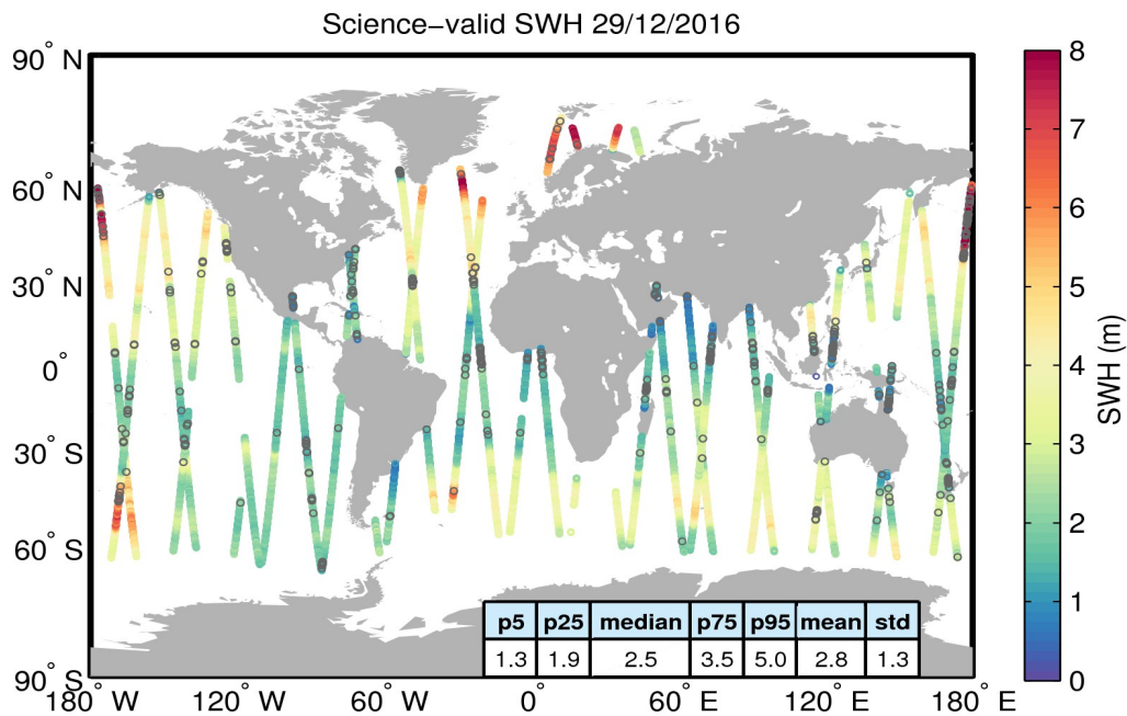
Figure 19. Geographical distribution of science-valid SWH data over oceans and lakes for 29/12/2016. The statistical values shown in the table refer to the SWH in m and are calculated over all measurements shown in the figure. Gray circles denote records that have been rejected based on the editing criteria described in Table 3.
