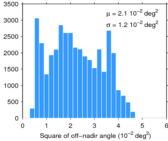
Figure 39. Histogram of flag-valid mispointing over oceans and lakes for 29/12/2016. The mean ( \mu ) and standard deviation ( \sigma ) are also shown. Note that values larger than 6 \cdot 10^{-2} \text{ deg}^2 are excluded from the histogram for the sake of readability but not from the computation of \mu and \sigma .
