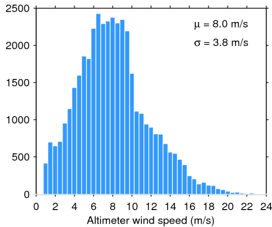
Figure 33. Histogram of flag-valid wind over oceans and lakes for 29/12/2016. The mean ( \mu ) and standard deviation ( \sigma ) are also shown. Note that values larger than 24 m/s are excluded from the histogram for the sake of readability but not from the computation of \mu and \sigma .
