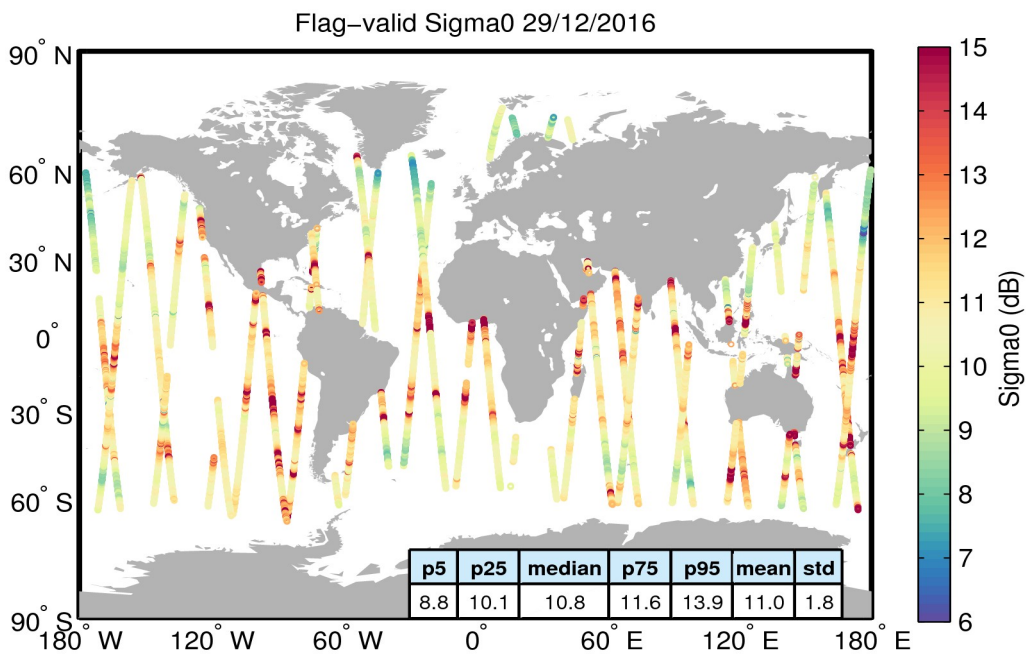
Figure 23. Geographical distribution of flag-valid sigma0 data over oceans and lakes for 29/12/2016. The statistical values shown in the table refer to the sigma0 in dB and are calculated over all measurements shown in the figure.
