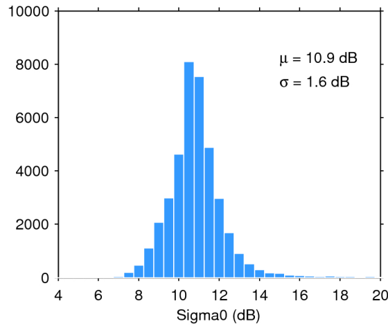
Figure 28. Histogram of science-valid sigma0 over oceans and lakes for 29/12/2016. The mean ( \mu ) and standard deviation ( \sigma ) are also shown. Note that values outside [4 20] dB are excluded from the histogram for the sake of readability but not from the computation of \mu and \sigma .
