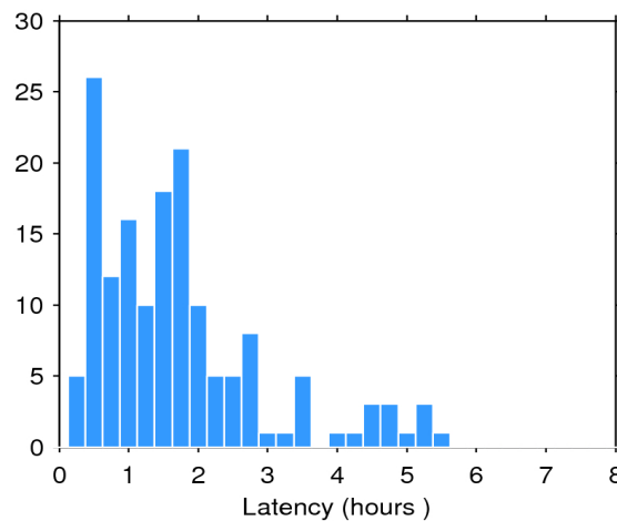
Figure 2. Histogram of the data latency for 29/12/2016. The y-axis denotes the number of files that are made available with a delay of x-hours with respect to the mean time of the records stored in the file.
