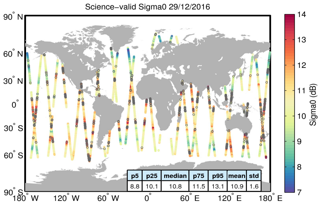
Figure 27. Geographical distribution of science-valid sigma0 data over oceans and lakes for 29/12/2016. The statistical values shown in the table refer to the sigma0 in dB and are calculated over all measurements shown in the figure. Gray circles denote records that have been rejected based on the editing criteria described in Table 4.
