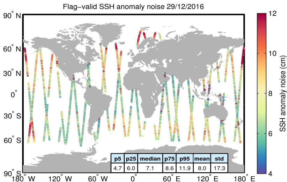
Figure 8. Geographical distribution of flag-valid 20-Hz SSH anomaly measurement noise over oceans and lakes for 29/12/2016. The statistical values shown in the table refer to the SSH anomaly noise and are calculated over all measurements shown in the figure.
