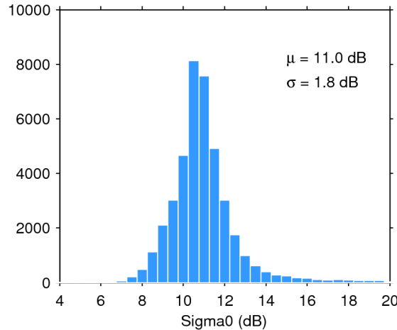
Figure 25. Histogram of flag-valid sigma0 over oceans and lakes for 29/12/2016. The mean ( \mu ) and standard deviation ( \sigma ) are also shown. Note that values outside [4 20] dB are excluded from the histogram for the sake of readability but not from the computation of \mu and \sigma .
