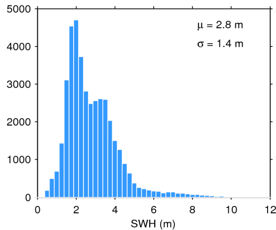
Figure 17. Histogram of flag-valid SWH over oceans and lakes for 29/12/2016. The mean ( \mu ) and standard deviation ( \sigma ) are also shown. Note that values larger than 12 m are excluded from the histogram for the sake of readability but not from the computation of \mu and \sigma .
