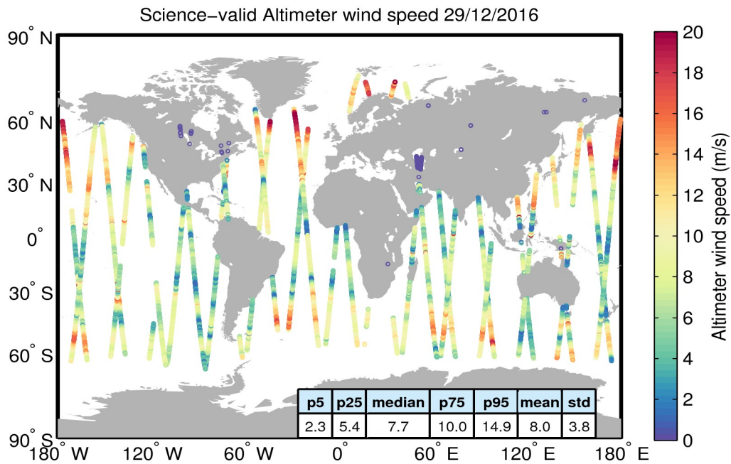
Figure 34. Geographical distribution of science-valid wind data over oceans and lakes for 29/12/2016. The statistical values shown in the table refer to the wind in m/s and are calculated over all measurements shown in the figure. Gray circles denote records that have been rejected based on the editing criteria described in Table 5.
