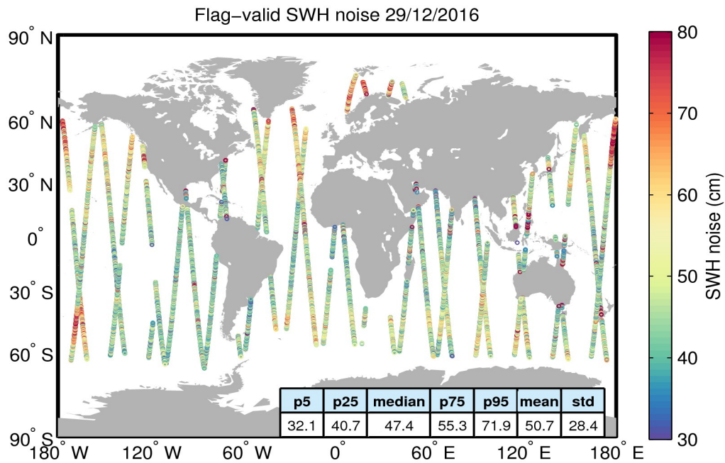
Figure 18. Geographical distribution of flag-valid 20-Hz SWH measurement noise over oceans and lakes for 29/12/2016. The statistical values shown in the table refer to the SWH noise and are calculated over all measurements shown in the figure.
