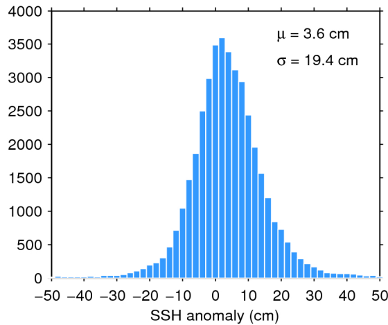
Figure 7. Histogram of flag-valid SSH anomaly over oceans and lakes for 28/12/2016. The mean ( \mu ) and standard deviation ( \sigma ) are also shown. Note that values outside [-50 50] cm are excluded from the histogram for the sake of readability but not from the computation of \mu and \sigma .
