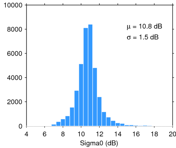
Figure 28. Histogram of science-valid sigma0 over oceans and lakes for 28/12/2016. The mean ( \mu ) and standard deviation ( \sigma ) are also shown. Note that values outside [4 20] dB are excluded from the histogram for the sake of readability but not from the computation of \mu and \sigma .
