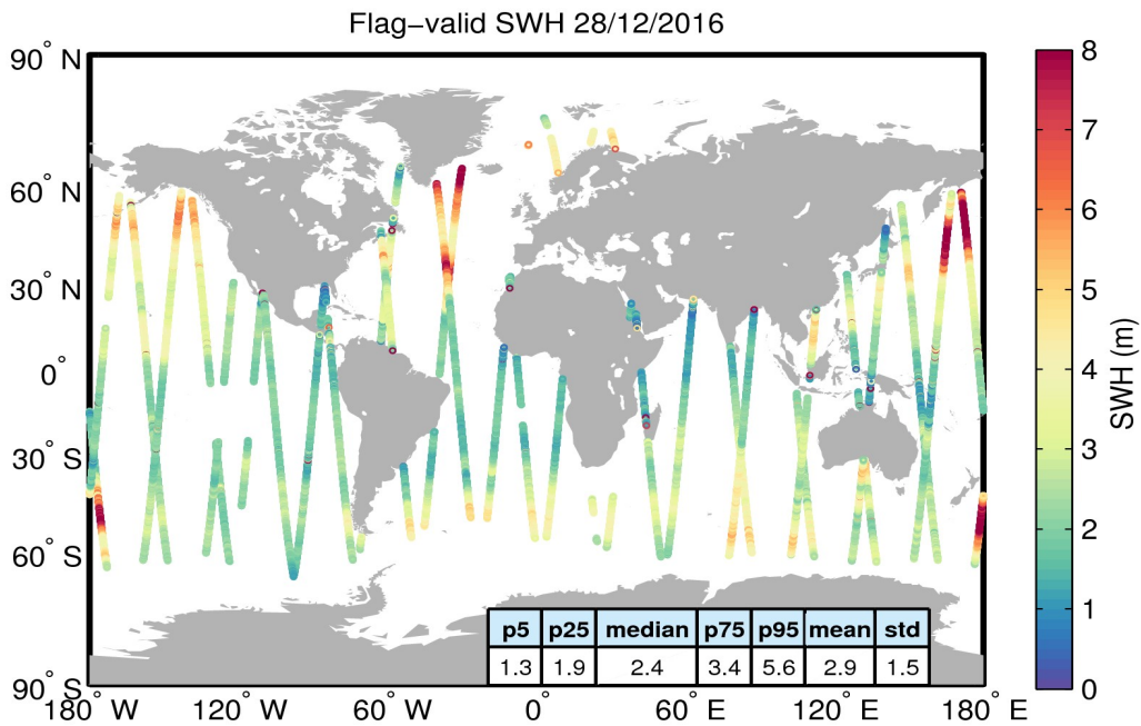
Figure 15. Geographical distribution of flag-valid SWH data over oceans and lakes for 28/12/2016. The statistical values shown in the table refer to the SWH in m and are calculated over all measurements shown in the figure.
