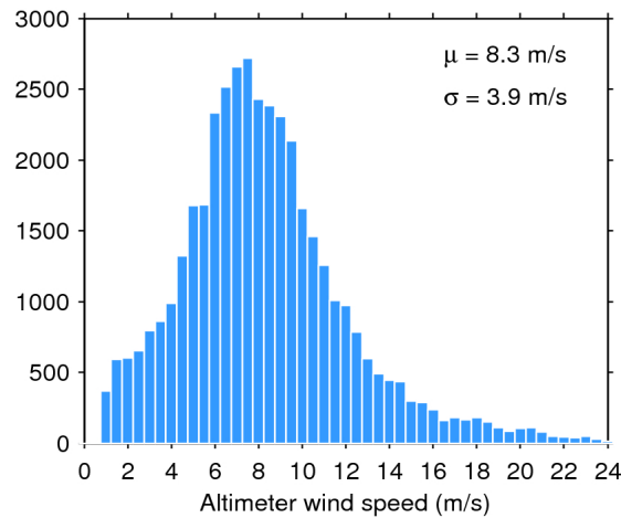
Figure 33. Histogram of flag-valid wind over oceans and lakes for 28/12/2016. The mean ( \mu ) and standard deviation ( \sigma ) are also shown. Note that values larger than 24 m/s are excluded from the histogram for the sake of readability but not from the computation of \mu and \sigma .
