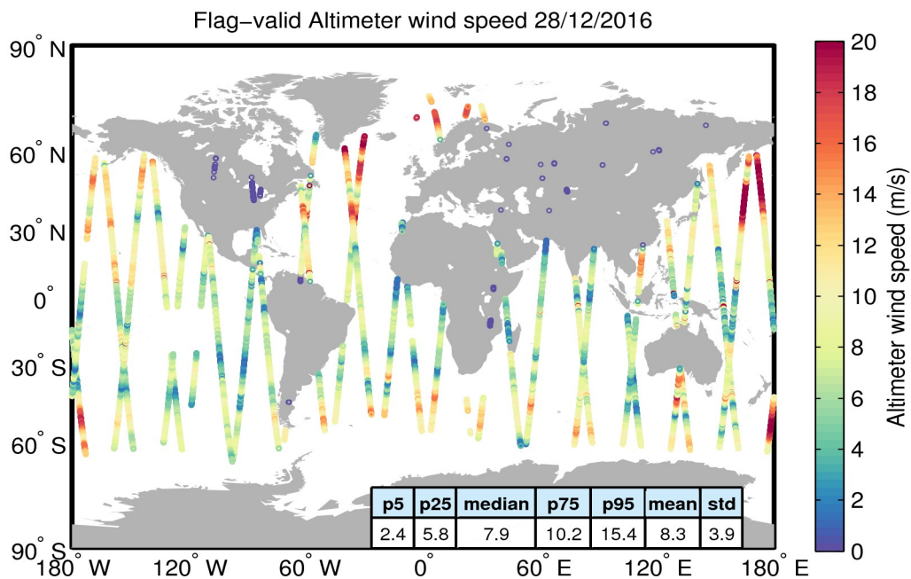
Figure 31. Geographical distribution of flag-valid wind data over oceans and lakes for 28/12/2016. The statistical values shown in the table refer to the wind in m/s and are calculated over all measurements shown in the figure.
