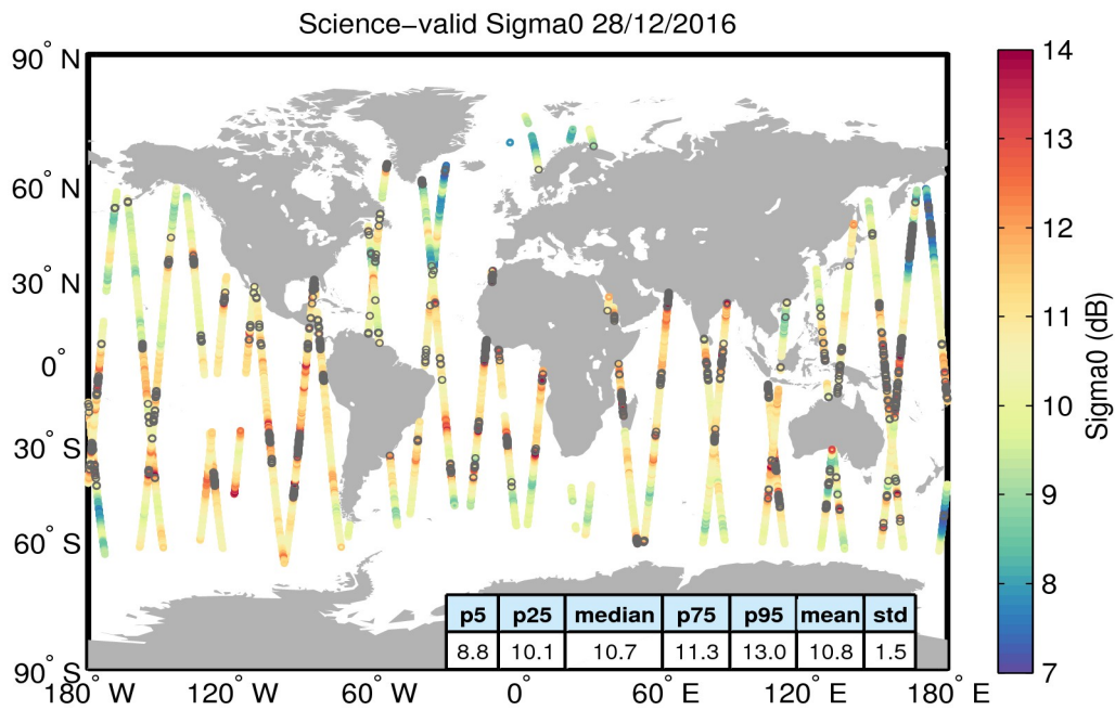
Figure 27. Geographical distribution of science-valid sigma0 data over oceans and lakes for 28/12/2016. The statistical values shown in the table refer to the sigma0 in dB and are calculated over all measurements shown in the figure. Gray circles denote records that have been rejected based on the editing criteria described in Table 4.
