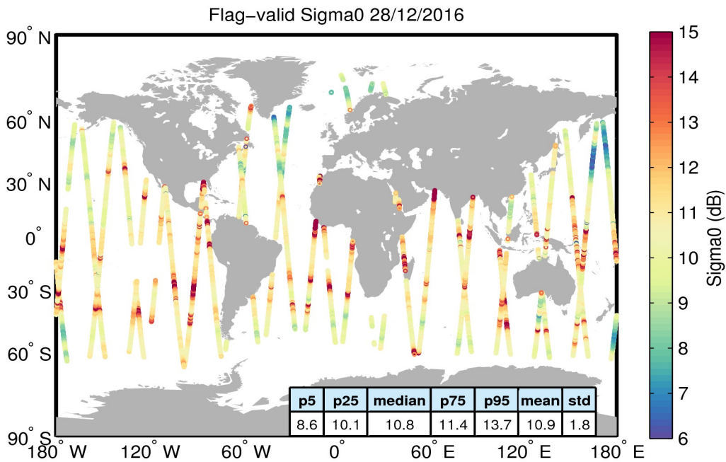
Figure 23. Geographical distribution of flag-valid sigma0 data over oceans and lakes for 28/12/2016. The statistical values shown in the table refer to the sigma0 in dB and are calculated over all measurements shown in the figure.
