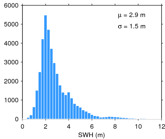
Figure 17. Histogram of flag-valid SWH over oceans and lakes for 28/12/2016. The mean ( \mu ) and standard deviation ( \sigma ) are also shown. Note that values larger than 12 m are excluded from the histogram for the sake of readability but not from the computation of \mu and \sigma .
