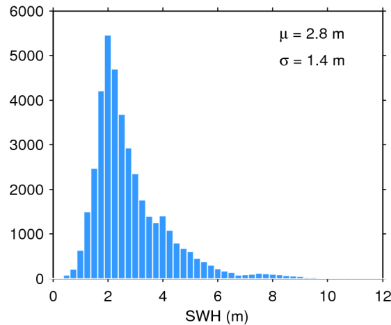
Figure 20. Histogram of science-valid SWH over oceans and lakes for 28/12/2016. The mean ( \mu ) and standard deviation ( \sigma ) are also shown. Note that values larger than 12 m are excluded from the histogram for the sake of readability but not from the computation of \mu and \sigma .
