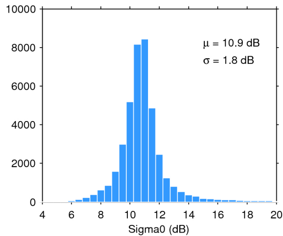
Figure 25. Histogram of flag-valid sigma0 over oceans and lakes for 28/12/2016. The mean ( \mu ) and standard deviation ( \sigma ) are also shown. Note that values outside [4 20] dB are excluded from the histogram for the sake of readability but not from the computation of \mu and \sigma .
