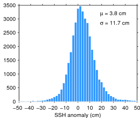
Figure 11. Histogram of science-valid SSH anomaly over oceans and lakes for 28/12/2016. The mean ( \mu ) and standard deviation ( \sigma ) are also shown. Note that values outside [-50 50] cm are excluded from the histogram for the sake of readability but not from the computation of \mu and \sigma .
