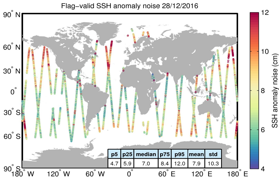
Figure 8. Geographical distribution of flag-valid 20-Hz SSH anomaly measurement noise over oceans and lakes for 28/12/2016. The statistical values shown in the table refer to the SSH anomaly noise and are calculated over all measurements shown in the figure.
