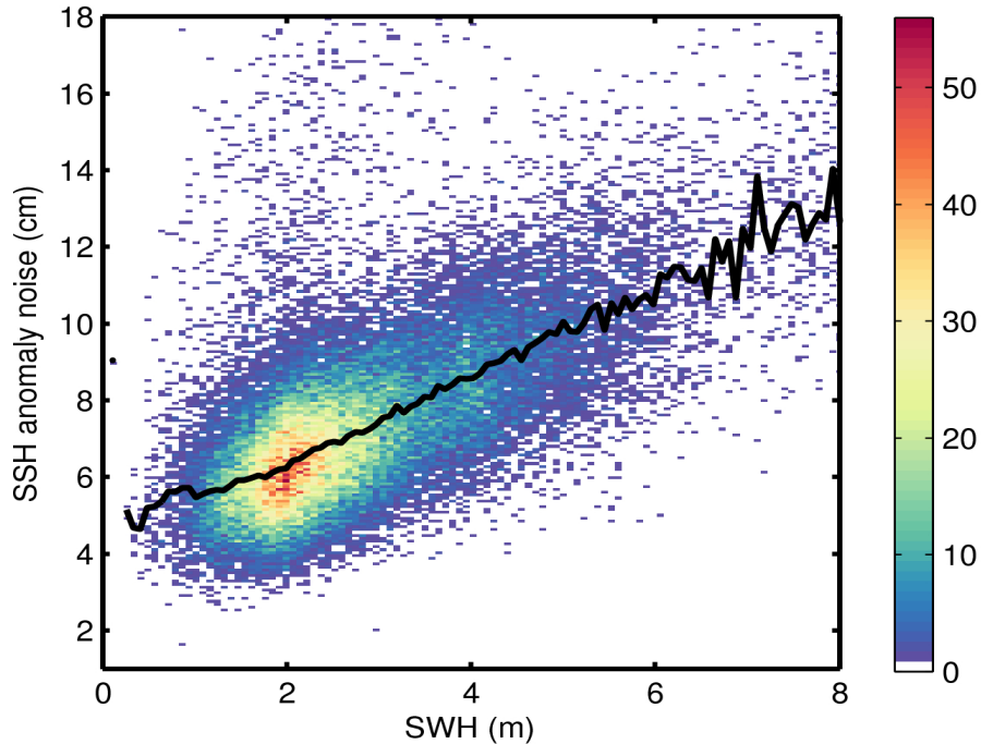
Figure 9. 2D histogram showing flag-valid SSH anomaly noise as a function of SWH for 28/12/2016. The black line denotes the median SSH anomaly noise as a function of SWH.
