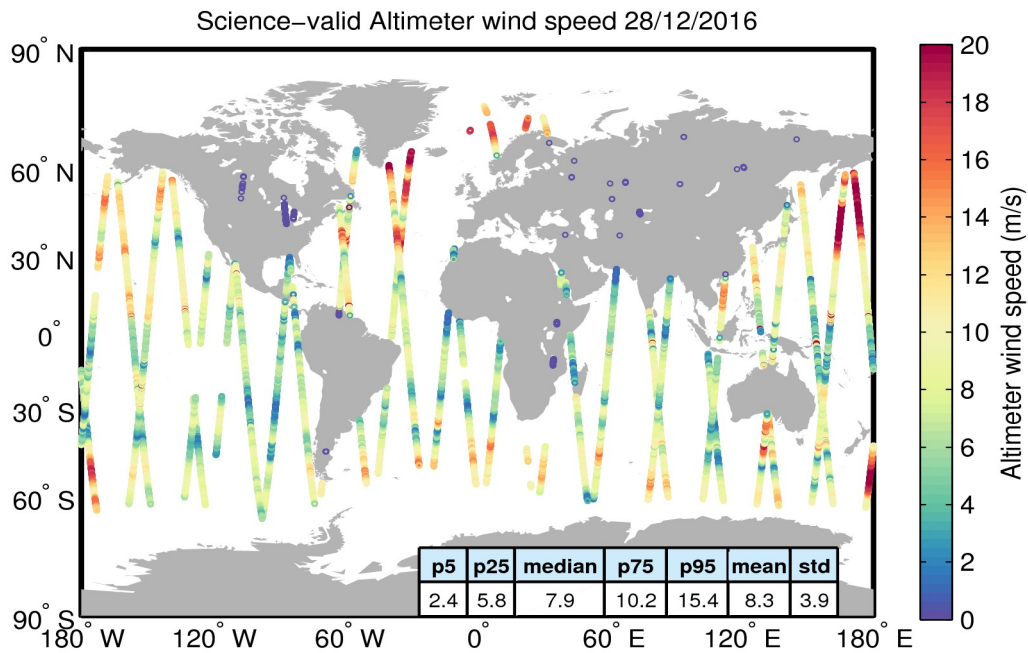
Figure 34. Geographical distribution of science-valid wind data over oceans and lakes for 28/12/2016. The statistical values shown in the table refer to the wind in m/s and are calculated over all measurements shown in the figure. Gray circles denote records that have been rejected based on the editing criteria described in Table 5.
