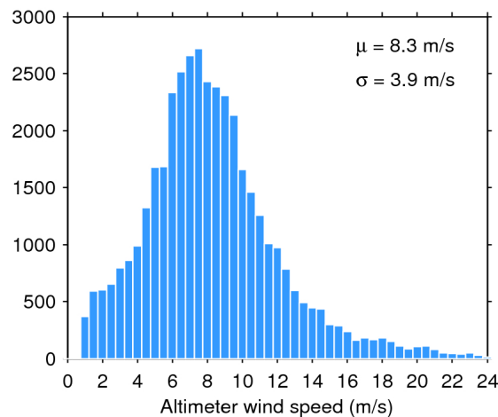
Figure 35. Histogram of science-valid wind over oceans and lakes for 28/12/2016. The mean ( \mu ) and standard deviation ( \sigma ) are also shown. Note that values larger than 24 m/s are excluded from the histogram for the sake of readability but not from the computation of \mu and \sigma .
