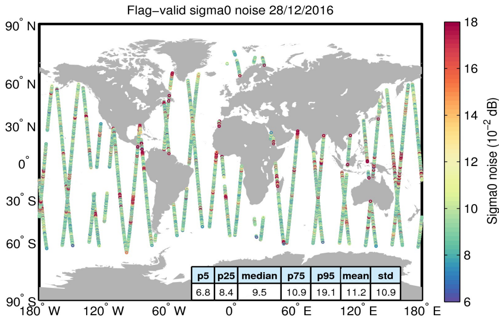
Figure 26. Geographical distribution of flag-valid 20-Hz sigma0 measurement noise over oceans and lakes for 28/12/2016. The statistical values shown in the table refer to the sigma0 noise and are calculated over all measurements shown in the figure.
