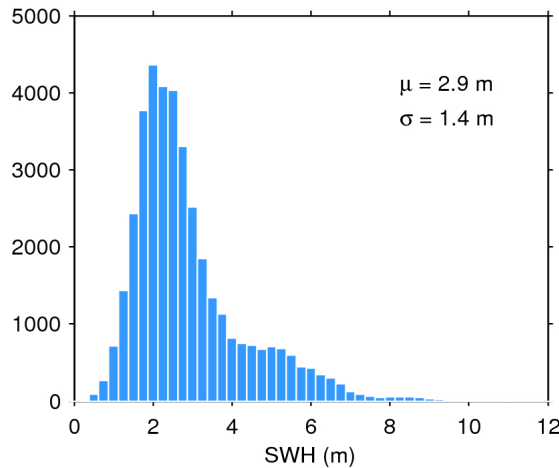
Figure 20. Histogram of science-valid SWH over oceans and lakes for 27/12/2016. The mean ( \mu ) and standard deviation ( \sigma ) are also shown. Note that values larger than 12 m are excluded from the histogram for the sake of readability but not from the computation of \mu and \sigma .
