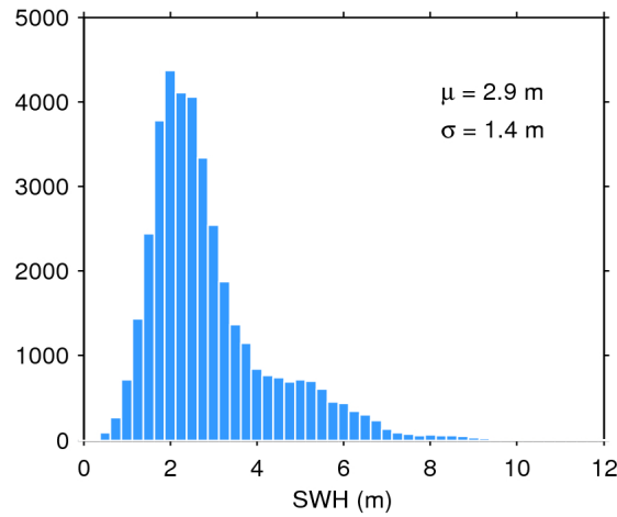
Figure 17. Histogram of flag-valid SWH over oceans and lakes for 27/12/2016. The mean ( \mu ) and standard deviation ( \sigma ) are also shown. Note that values larger than 12 m are excluded from the histogram for the sake of readability but not from the computation of \mu and \sigma .
