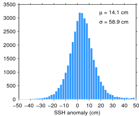
Figure 7. Histogram of flag-valid SSH anomaly over oceans and lakes for 27/12/2016. The mean ( \mu ) and standard deviation ( \sigma ) are also shown. Note that values outside [-50 50] cm are excluded from the histogram for the sake of readability but not from the computation of \mu and \sigma .
