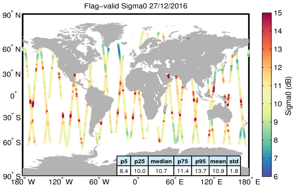
Figure 23. Geographical distribution of flag-valid sigma0 data over oceans and lakes for 27/12/2016. The statistical values shown in the table refer to the sigma0 in dB and are calculated over all measurements shown in the figure.
