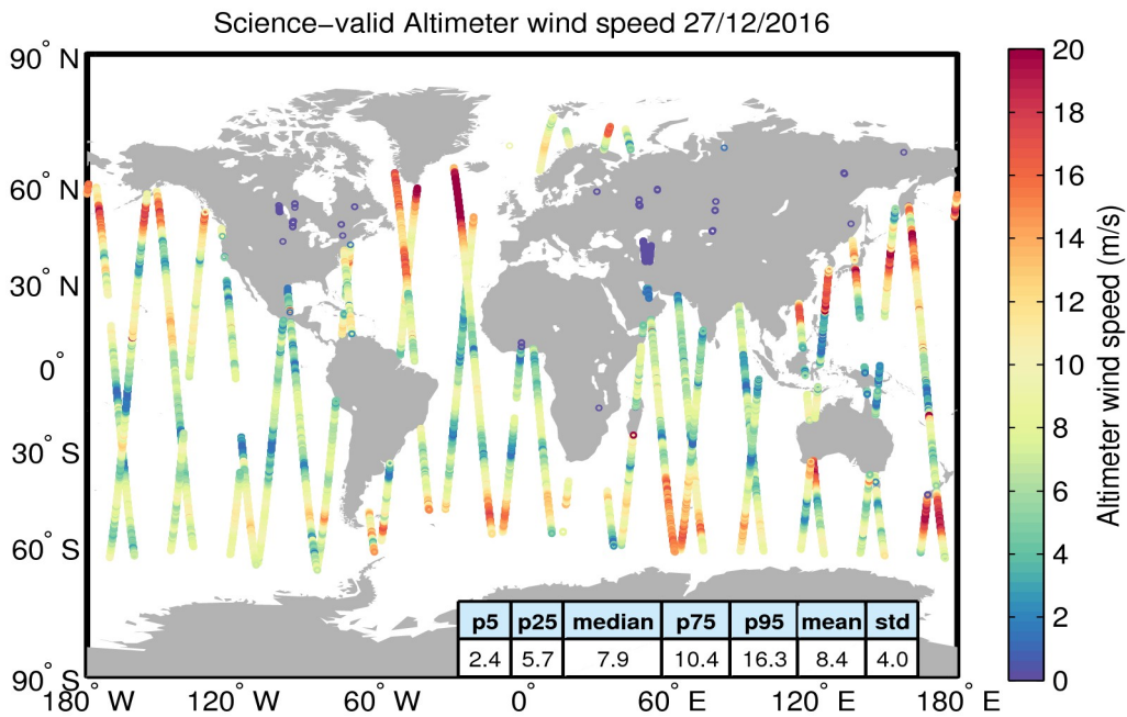
Figure 34. Geographical distribution of science-valid wind data over oceans and lakes for 27/12/2016. The statistical values shown in the table refer to the wind in m/s and are calculated over all measurements shown in the figure. Gray circles denote records that have been rejected based on the editing criteria described in Table 5.
