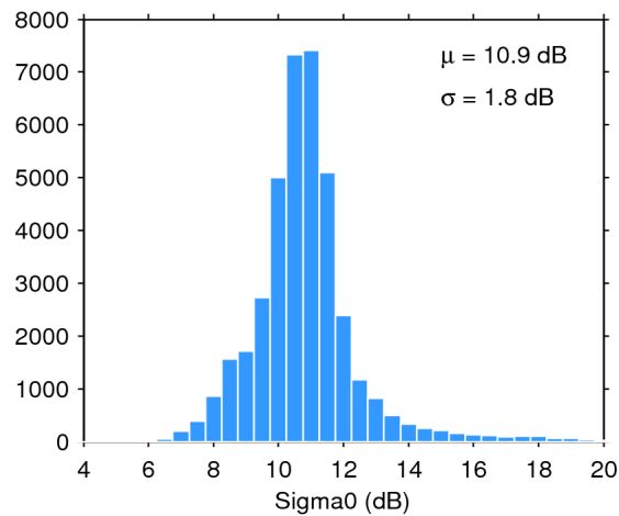
Figure 25. Histogram of flag-valid sigma0 over oceans and lakes for 27/12/2016. The mean ( \mu ) and standard deviation ( \sigma ) are also shown. Note that values outside [4 20] dB are excluded from the histogram for the sake of readability but not from the computation of \mu and \sigma .
