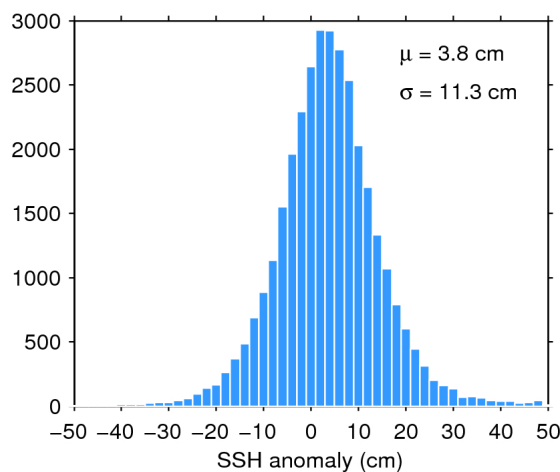
Figure 11. Histogram of science-valid SSH anomaly over oceans and lakes for 27/12/2016. The mean ( \mu ) and standard deviation ( \sigma ) are also shown. Note that values outside [-50 50] cm are excluded from the histogram for the sake of readability but not from the computation of \mu and \sigma .
