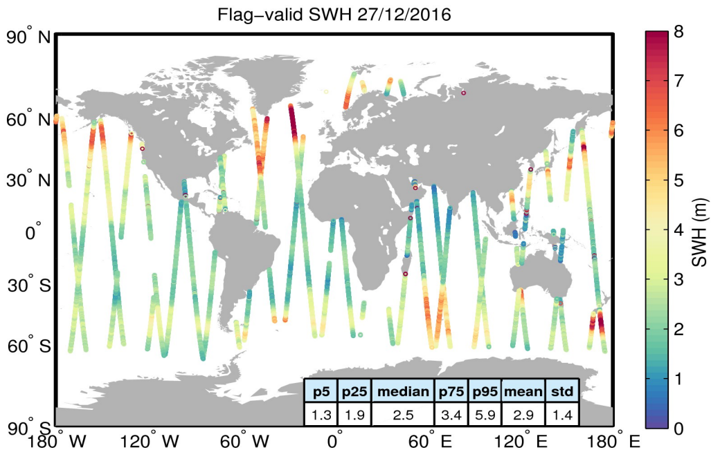
Figure 15. Geographical distribution of flag-valid SWH data over oceans and lakes for 27/12/2016. The statistical values shown in the table refer to the SWH in m and are calculated over all measurements shown in the figure.
