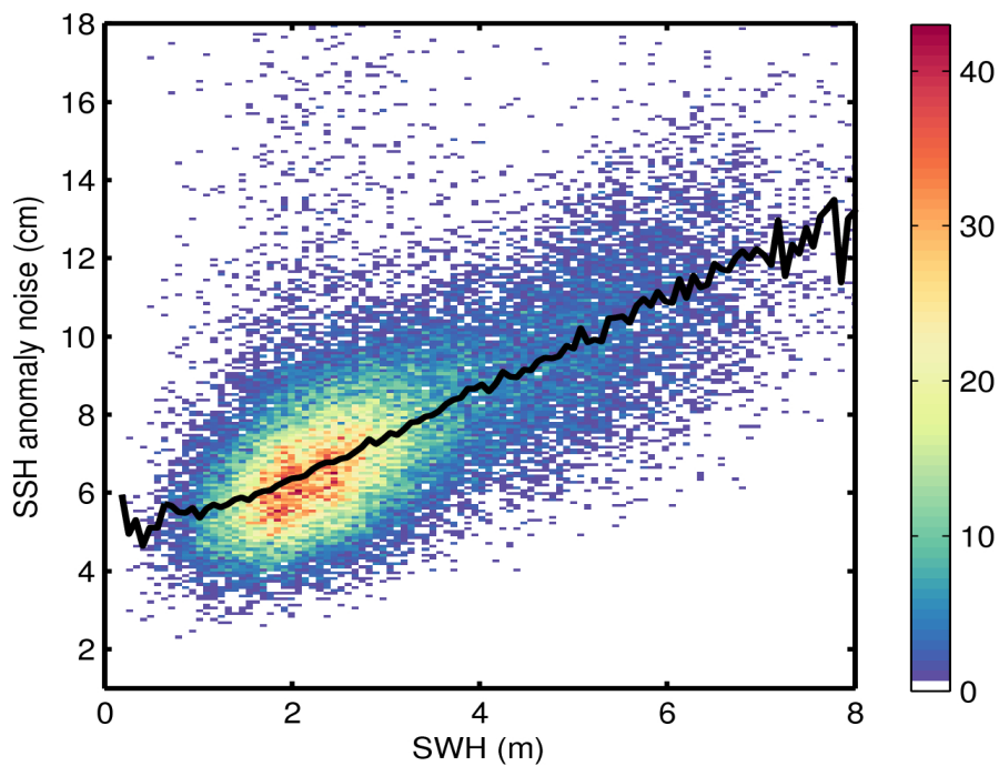
Figure 9. 2D histogram showing flag-valid SSH anomaly noise as a function of SWH for 27/12/2016. The black line denotes the median SSH anomaly noise as a function of SWH.
