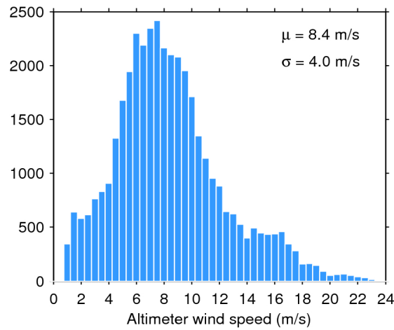
Figure 33. Histogram of flag-valid wind over oceans and lakes for 27/12/2016. The mean ( \mu ) and standard deviation ( \sigma ) are also shown. Note that values larger than 24 m/s are excluded from the histogram for the sake of readability but not from the computation of \mu and \sigma .
