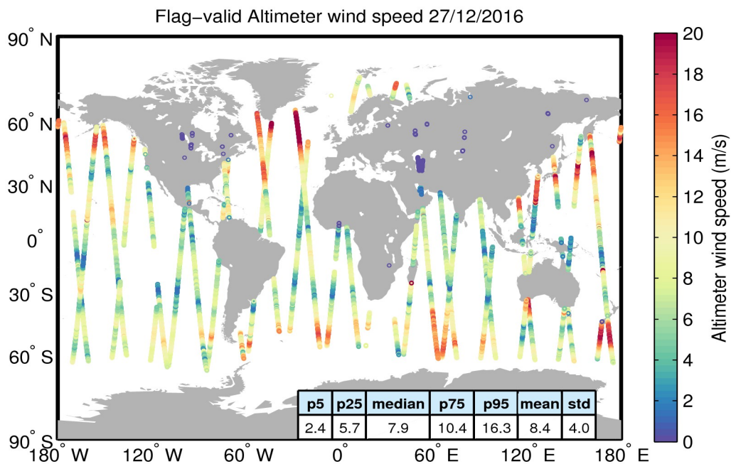
Figure 31. Geographical distribution of flag-valid wind data over oceans and lakes for 27/12/2016. The statistical values shown in the table refer to the wind in m/s and are calculated over all measurements shown in the figure.
