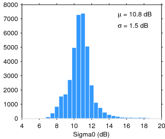
Figure 28. Histogram of science-valid sigma0 over oceans and lakes for 27/12/2016. The mean ( \mu ) and standard deviation ( \sigma ) are also shown. Note that values outside [4 20] dB are excluded from the histogram for the sake of readability but not from the computation of \mu and \sigma .
