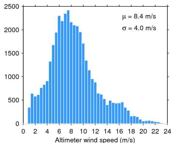
Figure 35. Histogram of science-valid wind over oceans and lakes for 27/12/2016. The mean ( \mu ) and standard deviation ( \sigma ) are also shown. Note that values larger than 24 m/s are excluded from the histogram for the sake of readability but not from the computation of \mu and \sigma .
