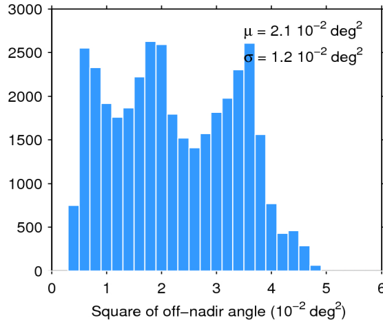
Figure 39. Histogram of flag-valid mispointing over oceans and lakes for 27/12/2016. The mean ( \mu ) and standard deviation ( \sigma ) are also shown. Note that values larger than 6 \cdot 10^{-2} \text{ deg}^2 are excluded from the histogram for the sake of readability but not from the computation of \mu and \sigma .
