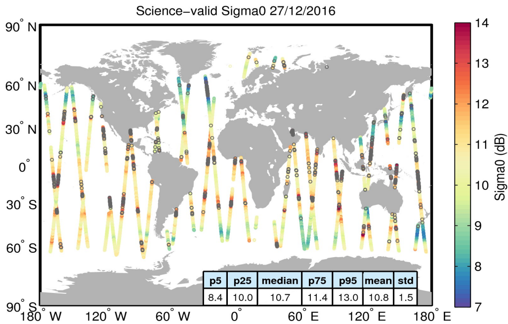
Figure 27. Geographical distribution of science-valid sigma0 data over oceans and lakes for 27/12/2016. The statistical values shown in the table refer to the sigma0 in dB and are calculated over all measurements shown in the figure. Gray circles denote records that have been rejected based on the editing criteria described in Table 4.
