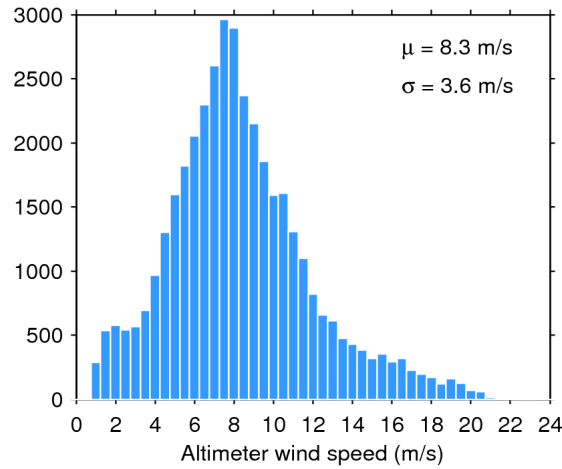
Figure 33. Histogram of flag-valid wind over oceans and lakes for 26/12/2016. The mean ( \mu ) and standard deviation ( \sigma ) are also shown. Note that values larger than 24 m/s are excluded from the histogram for the sake of readability but not from the computation of \mu and \sigma .
