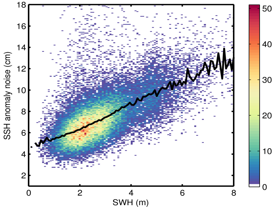
Figure 9. 2D histogram showing flag-valid SSH anomaly noise as a function of SWH for 26/12/2016. The black line denotes the median SSH anomaly noise as a function of SWH.
