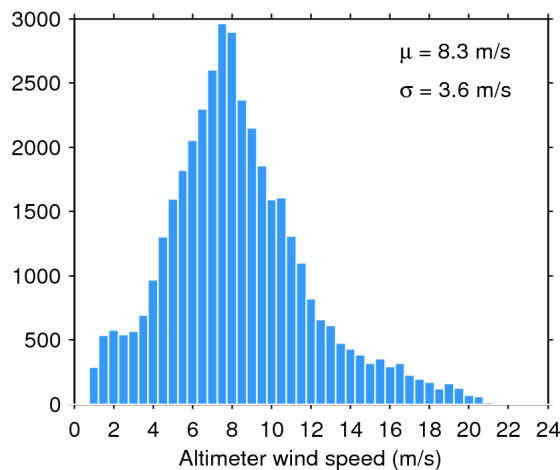
Figure 35. Histogram of science-valid wind over oceans and lakes for 26/12/2016. The mean ( \mu ) and standard deviation ( \sigma ) are also shown. Note that values larger than 24 m/s are excluded from the histogram for the sake of readability but not from the computation of \mu and \sigma .
