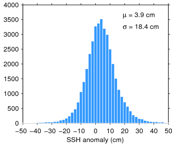
Figure 7. Histogram of flag-valid SSH anomaly over oceans and lakes for 26/12/2016. The mean ( \mu ) and standard deviation ( \sigma ) are also shown. Note that values outside [-50 50] cm are excluded from the histogram for the sake of readability but not from the computation of \mu and \sigma .
