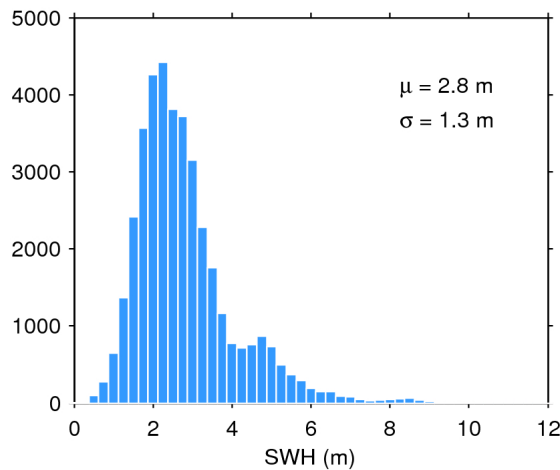
Figure 20. Histogram of science-valid SWH over oceans and lakes for 26/12/2016. The mean ( \mu ) and standard deviation ( \sigma ) are also shown. Note that values larger than 12 m are excluded from the histogram for the sake of readability but not from the computation of \mu and \sigma .
