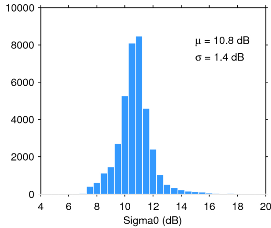
Figure 28. Histogram of science-valid sigma0 over oceans and lakes for 26/12/2016. The mean ( \mu ) and standard deviation ( \sigma ) are also shown. Note that values outside [4 20] dB are excluded from the histogram for the sake of readability but not from the computation of \mu and \sigma .
