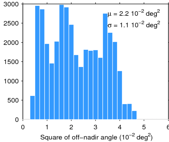
Figure 39. Histogram of flag-valid mispointing over oceans and lakes for 26/12/2016. The mean ( \mu ) and standard deviation ( \sigma ) are also shown. Note that values larger than 6 \cdot 10^{-2} \text{ deg}^2 are excluded from the histogram for the sake of readability but not from the computation of \mu and \sigma .
