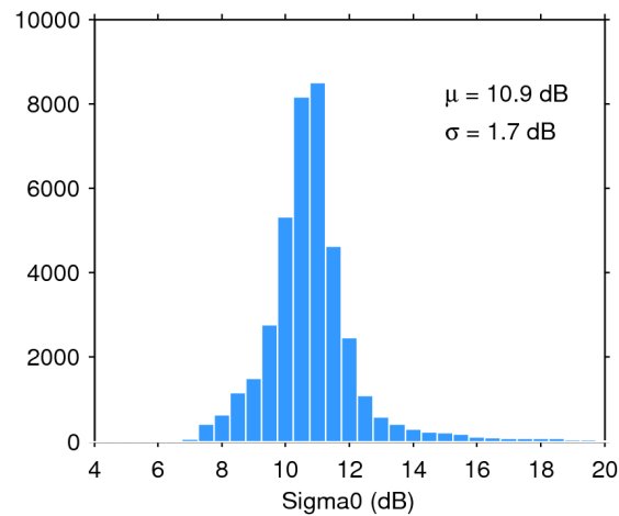
Figure 25. Histogram of flag-valid sigma0 over oceans and lakes for 26/12/2016. The mean ( \mu ) and standard deviation ( \sigma ) are also shown. Note that values outside [4 20] dB are excluded from the histogram for the sake of readability but not from the computation of \mu and \sigma .
