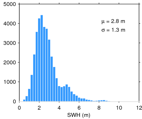
Figure 17. Histogram of flag-valid SWH over oceans and lakes for 26/12/2016. The mean ( \mu ) and standard deviation ( \sigma ) are also shown. Note that values larger than 12 m are excluded from the histogram for the sake of readability but not from the computation of \mu and \sigma .
