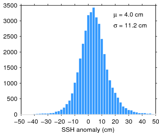
Figure 11. Histogram of science-valid SSH anomaly over oceans and lakes for 26/12/2016. The mean ( \mu ) and standard deviation ( \sigma ) are also shown. Note that values outside [-50 50] cm are excluded from the histogram for the sake of readability but not from the computation of \mu and \sigma .
