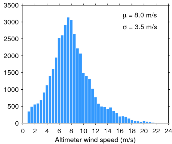
Figure 33. Histogram of flag-valid wind over oceans and lakes for 25/12/2016. The mean ( \mu ) and standard deviation ( \sigma ) are also shown. Note that values larger than 24 m/s are excluded from the histogram for the sake of readability but not from the computation of \mu and \sigma .
