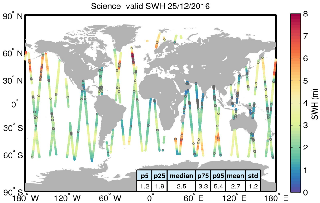
Figure 19. Geographical distribution of science-valid SWH data over oceans and lakes for 25/12/2016. The statistical values shown in the table refer to the SWH in m and are calculated over all measurements shown in the figure. Gray circles denote records that have been rejected based on the editing criteria described in Table 3.
