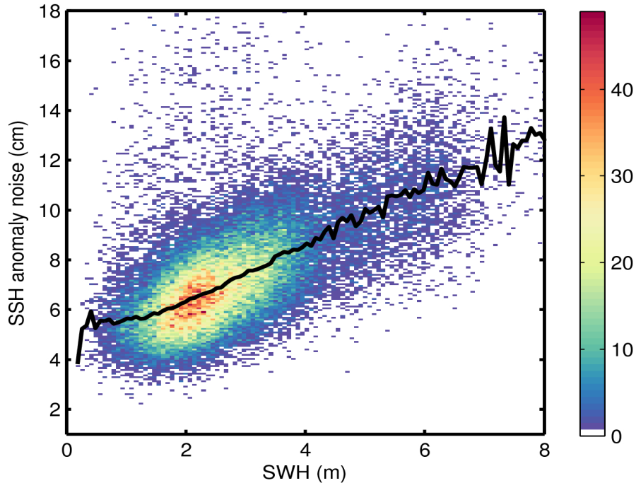
Figure 9. 2D histogram showing flag-valid SSH anomaly noise as a function of SWH for 25/12/2016. The black line denotes the median SSH anomaly noise as a function of SWH.
