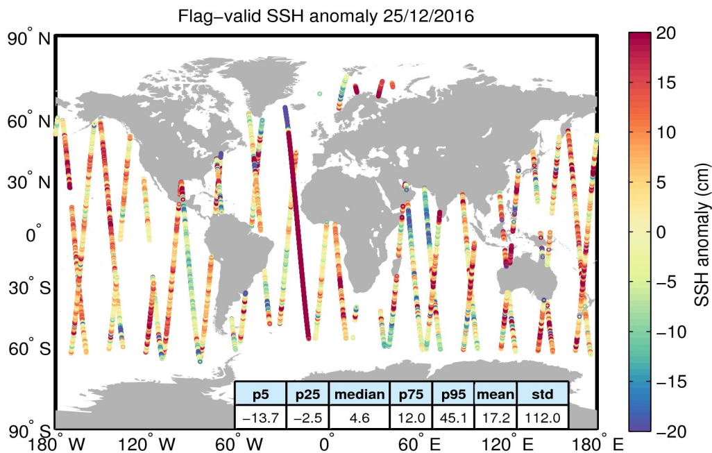
Figure 5. Geographical distribution of flag-valid 1-Hz SSH anomaly data over oceans and lakes for 25/12/2016. The statistical values shown in the table refer to the SSH anomaly in cm and are calculated over all measurements shown in the figure.
