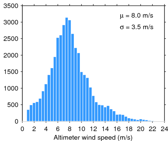
Figure 35. Histogram of science-valid wind over oceans and lakes for 25/12/2016. The mean ( \mu ) and standard deviation ( \sigma ) are also shown. Note that values larger than 24 m/s are excluded from the histogram for the sake of readability but not from the computation of \mu and \sigma .
