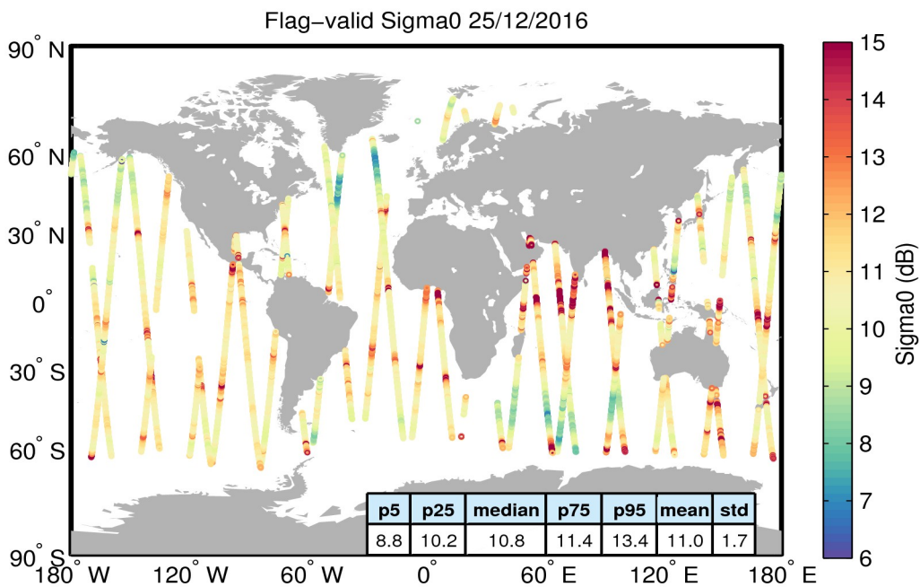
Figure 23. Geographical distribution of flag-valid sigma0 data over oceans and lakes for 25/12/2016. The statistical values shown in the table refer to the sigma0 in dB and are calculated over all measurements shown in the figure.
