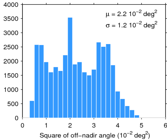
Figure 39. Histogram of flag-valid mispointing over oceans and lakes for 25/12/2016. The mean ( \mu ) and standard deviation ( \sigma ) are also shown. Note that values larger than 6 \cdot 10^{-2} \text{ deg}^2 are excluded from the histogram for the sake of readability but not from the computation of \mu and \sigma .
