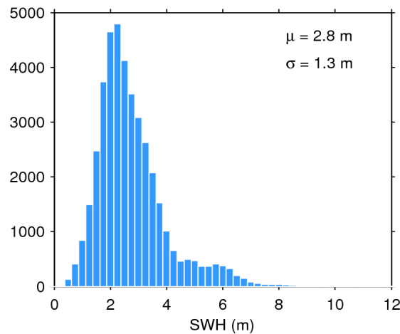
Figure 17. Histogram of flag-valid SWH over oceans and lakes for 25/12/2016. The mean ( \mu ) and standard deviation ( \sigma ) are also shown. Note that values larger than 12 m are excluded from the histogram for the sake of readability but not from the computation of \mu and \sigma .
