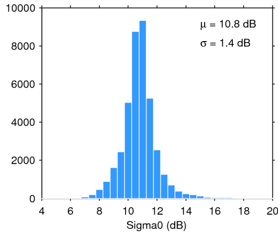
Figure 28. Histogram of science-valid sigma0 over oceans and lakes for 25/12/2016. The mean ( \mu ) and standard deviation ( \sigma ) are also shown. Note that values outside [4 20] dB are excluded from the histogram for the sake of readability but not from the computation of \mu and \sigma .
