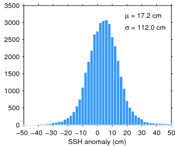
Figure 7. Histogram of flag-valid SSH anomaly over oceans and lakes for 25/12/2016. The mean ( \mu ) and standard deviation ( \sigma ) are also shown. Note that values outside [-50 50] cm are excluded from the histogram for the sake of readability but not from the computation of \mu and \sigma .
