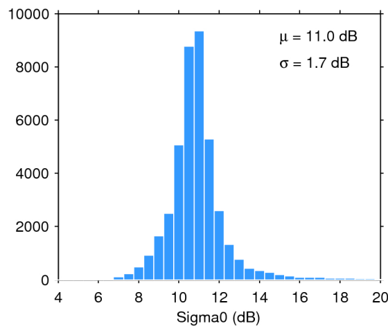
Figure 25. Histogram of flag-valid sigma0 over oceans and lakes for 25/12/2016. The mean ( \mu ) and standard deviation ( \sigma ) are also shown. Note that values outside [4 20] dB are excluded from the histogram for the sake of readability but not from the computation of \mu and \sigma .
