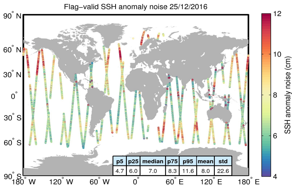
Figure 8. Geographical distribution of flag-valid 20-Hz SSH anomaly measurement noise over oceans and lakes for 25/12/2016. The statistical values shown in the table refer to the SSH anomaly noise and are calculated over all measurements shown in the figure.
