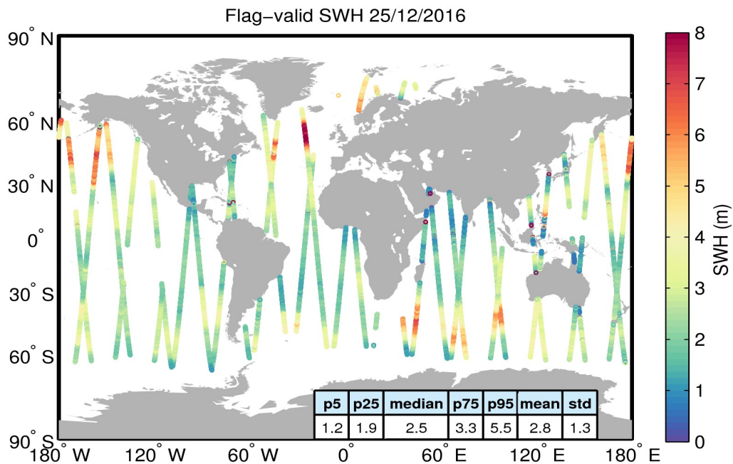
Figure 15. Geographical distribution of flag-valid SWH data over oceans and lakes for 25/12/2016. The statistical values shown in the table refer to the SWH in m and are calculated over all measurements shown in the figure.
