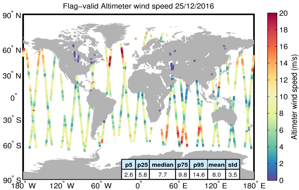
Figure 31. Geographical distribution of flag-valid wind data over oceans and lakes for 25/12/2016. The statistical values shown in the table refer to the wind in m/s and are calculated over all measurements shown in the figure.
