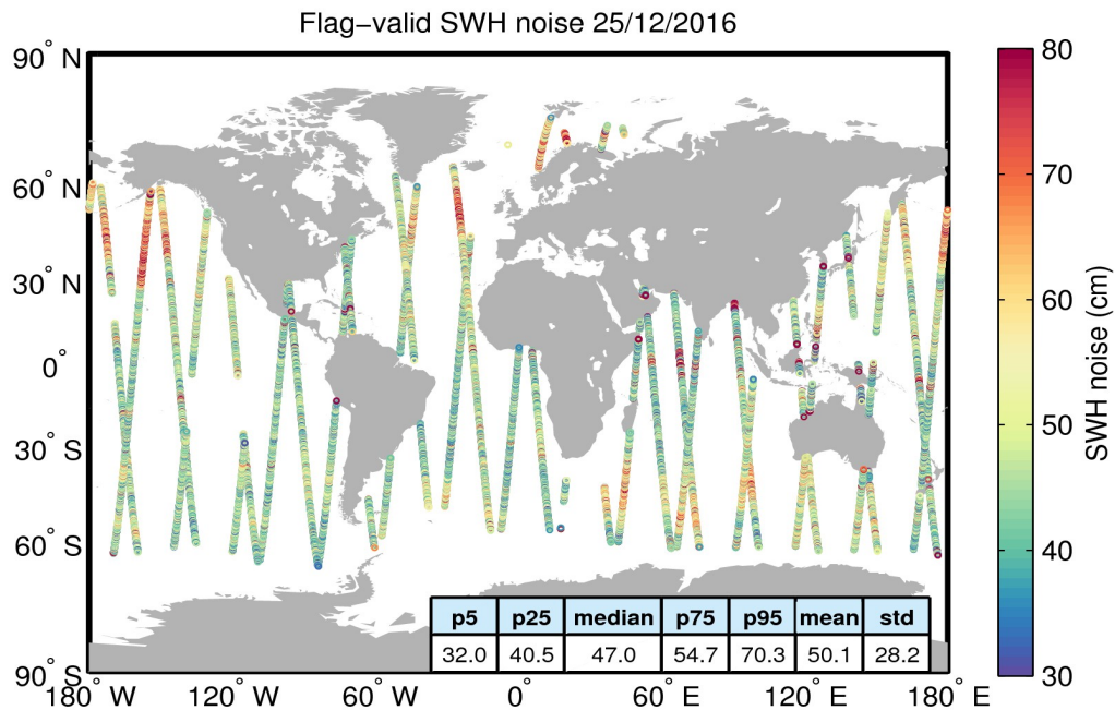
Figure 18. Geographical distribution of flag-valid 20-Hz SWH measurement noise over oceans and lakes for 25/12/2016. The statistical values shown in the table refer to the SWH noise and are calculated over all measurements shown in the figure.
