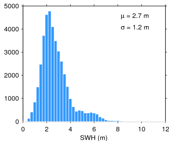
Figure 20. Histogram of science-valid SWH over oceans and lakes for 25/12/2016. The mean ( \mu ) and standard deviation ( \sigma ) are also shown. Note that values larger than 12 m are excluded from the histogram for the sake of readability but not from the computation of \mu and \sigma .
