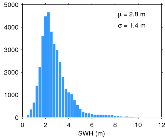
Figure 17. Histogram of flag-valid SWH over oceans and lakes for 24/12/2016. The mean ( \mu ) and standard deviation ( \sigma ) are also shown. Note that values larger than 12 m are excluded from the histogram for the sake of readability but not from the computation of \mu and \sigma .
