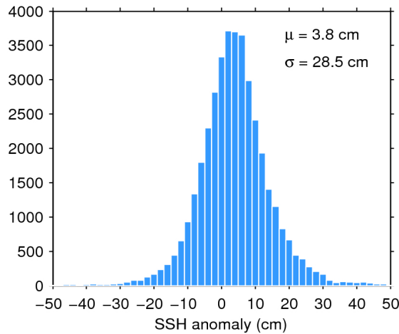
Figure 7. Histogram of flag-valid SSH anomaly over oceans and lakes for 24/12/2016. The mean ( \mu ) and standard deviation ( \sigma ) are also shown. Note that values outside [-50 50] cm are excluded from the histogram for the sake of readability but not from the computation of \mu and \sigma .
