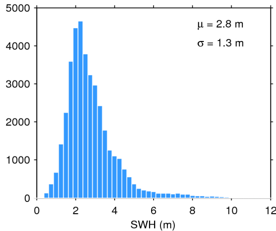
Figure 20. Histogram of science-valid SWH over oceans and lakes for 24/12/2016. The mean ( \mu ) and standard deviation ( \sigma ) are also shown. Note that values larger than 12 m are excluded from the histogram for the sake of readability but not from the computation of \mu and \sigma .
