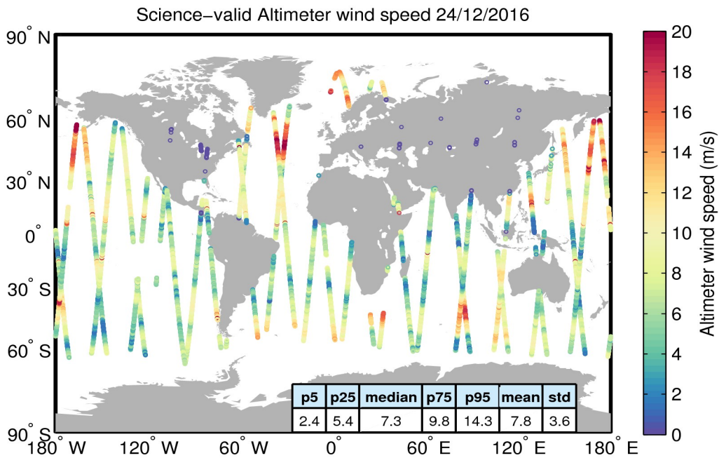
Figure 34. Geographical distribution of science-valid wind data over oceans and lakes for 24/12/2016. The statistical values shown in the table refer to the wind in m/s and are calculated over all measurements shown in the figure. Gray circles denote records that have been rejected based on the editing criteria described in Table 5.
