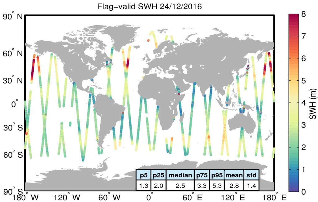
Figure 15. Geographical distribution of flag-valid SWH data over oceans and lakes for 24/12/2016. The statistical values shown in the table refer to the SWH in m and are calculated over all measurements shown in the figure.
