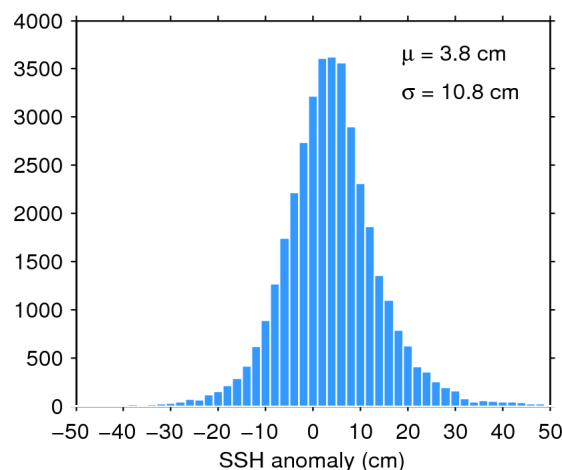
Figure 11. Histogram of science-valid SSH anomaly over oceans and lakes for 24/12/2016. The mean ( \mu ) and standard deviation ( \sigma ) are also shown. Note that values outside [-50 50] cm are excluded from the histogram for the sake of readability but not from the computation of \mu and \sigma .
