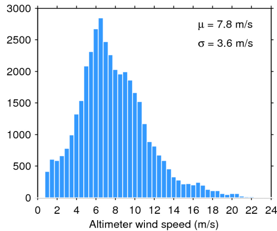
Figure 33. Histogram of flag-valid wind over oceans and lakes for 24/12/2016. The mean ( \mu ) and standard deviation ( \sigma ) are also shown. Note that values larger than 24 m/s are excluded from the histogram for the sake of readability but not from the computation of \mu and \sigma .
