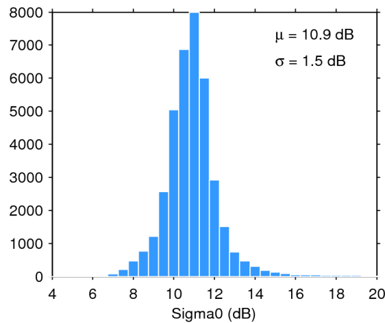
Figure 28. Histogram of science-valid sigma0 over oceans and lakes for 24/12/2016. The mean ( \mu ) and standard deviation ( \sigma ) are also shown. Note that values outside [4 20] dB are excluded from the histogram for the sake of readability but not from the computation of \mu and \sigma .
