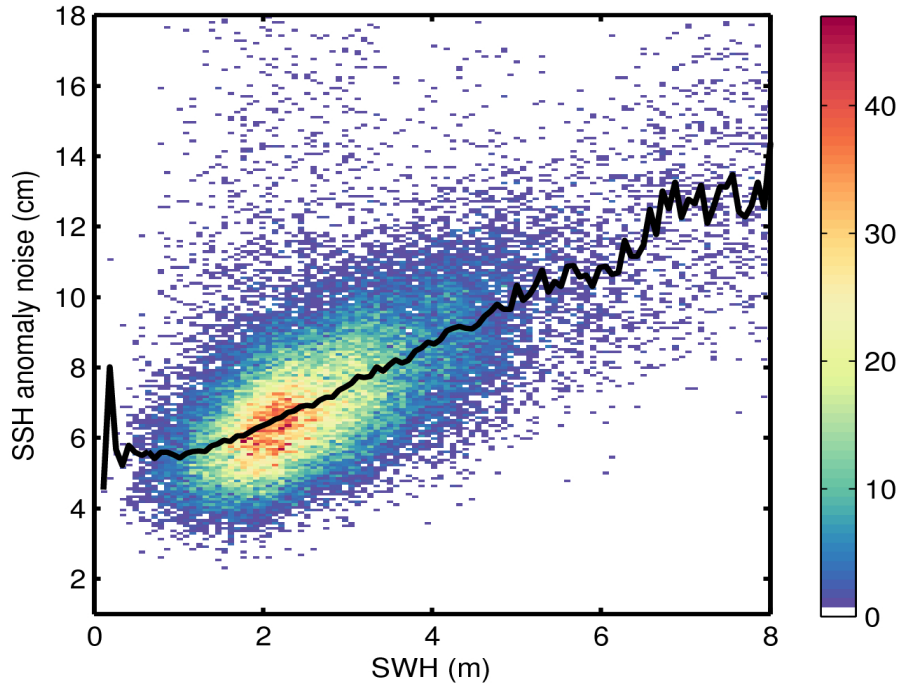
Figure 9. 2D histogram showing flag-valid SSH anomaly noise as a function of SWH for 24/12/2016. The black line denotes the median SSH anomaly noise as a function of SWH.
