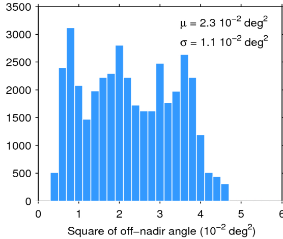
Figure 39. Histogram of flag-valid mispointing over oceans and lakes for 24/12/2016. The mean ( \mu ) and standard deviation ( \sigma ) are also shown. Note that values larger than 6 \cdot 10^{-2} \text{ deg}^2 are excluded from the histogram for the sake of readability but not from the computation of \mu and \sigma .
