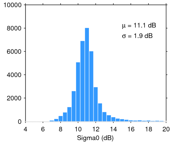
Figure 25. Histogram of flag-valid sigma0 over oceans and lakes for 24/12/2016. The mean ( \mu ) and standard deviation ( \sigma ) are also shown. Note that values outside [4 20] dB are excluded from the histogram for the sake of readability but not from the computation of \mu and \sigma .
