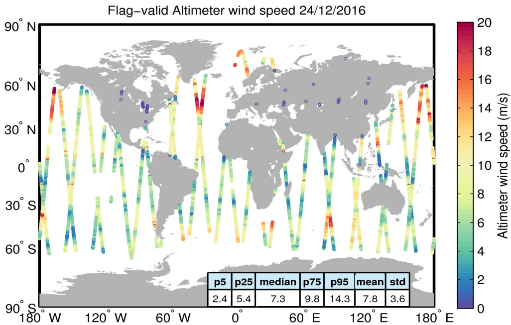
Figure 31. Geographical distribution of flag-valid wind data over oceans and lakes for 24/12/2016. The statistical values shown in the table refer to the wind in m/s and are calculated over all measurements shown in the figure.
