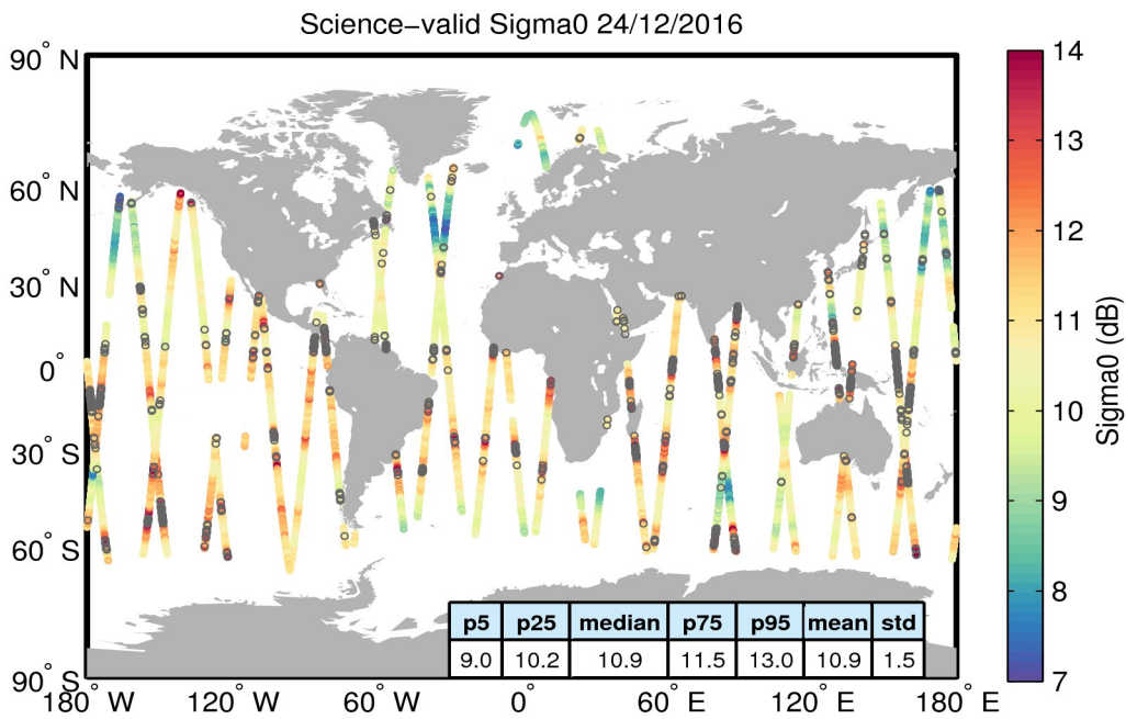
Figure 27. Geographical distribution of science-valid sigma0 data over oceans and lakes for 24/12/2016. The statistical values shown in the table refer to the sigma0 in dB and are calculated over all measurements shown in the figure. Gray circles denote records that have been rejected based on the editing criteria described in Table 4.
