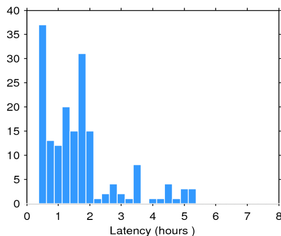
Figure 2. Histogram of the data latency for 24/12/2016. The y-axis denotes the number of files that are made available with a delay of x-hours with respect to the mean time of the records stored in the file.
