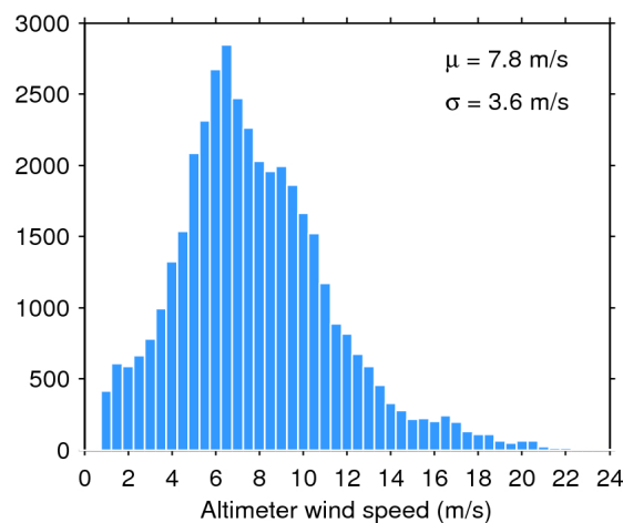
Figure 35. Histogram of science-valid wind over oceans and lakes for 24/12/2016. The mean ( \mu ) and standard deviation ( \sigma ) are also shown. Note that values larger than 24 m/s are excluded from the histogram for the sake of readability but not from the computation of \mu and \sigma .
