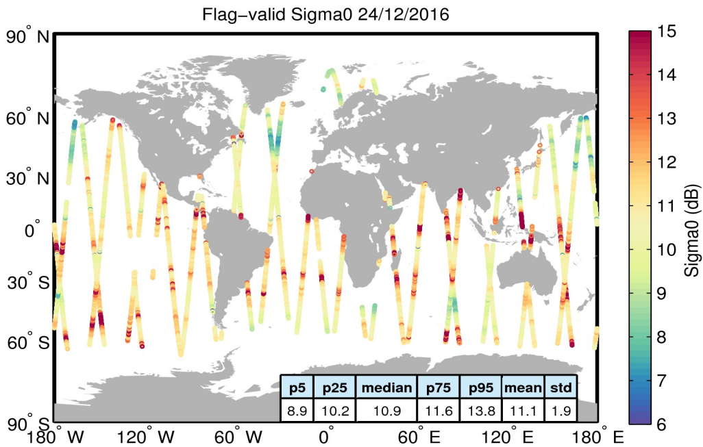
Figure 23. Geographical distribution of flag-valid sigma0 data over oceans and lakes for 24/12/2016. The statistical values shown in the table refer to the sigma0 in dB and are calculated over all measurements shown in the figure.
