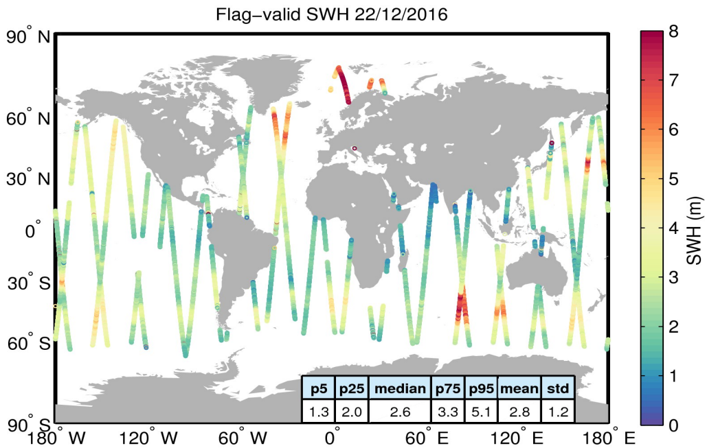
Figure 15. Geographical distribution of flag-valid SWH data over oceans and lakes for 22/12/2016. The statistical values shown in the table refer to the SWH in m and are calculated over all measurements shown in the figure.
