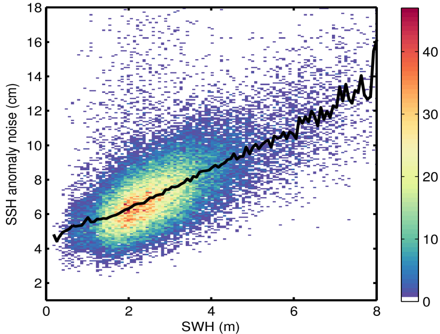
Figure 9. 2D histogram showing flag-valid SSH anomaly noise as a function of SWH for 22/12/2016. The black line denotes the median SSH anomaly noise as a function of SWH.
