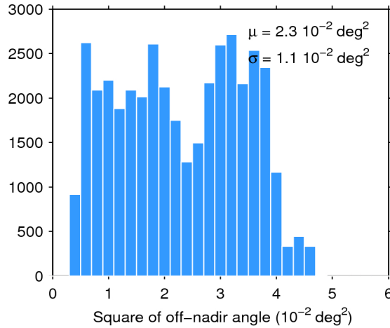
Figure 39. Histogram of flag-valid mispointing over oceans and lakes for 22/12/2016. The mean ( \mu ) and standard deviation ( \sigma ) are also shown. Note that values larger than 6 \cdot 10^{-2} \text{ deg}^2 are excluded from the histogram for the sake of readability but not from the computation of \mu and \sigma .
