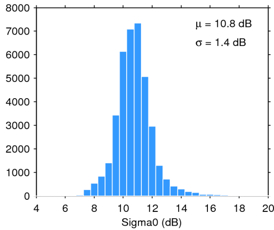
Figure 28. Histogram of science-valid sigma0 over oceans and lakes for 22/12/2016. The mean ( \mu ) and standard deviation ( \sigma ) are also shown. Note that values outside [4 20] dB are excluded from the histogram for the sake of readability but not from the computation of \mu and \sigma .
