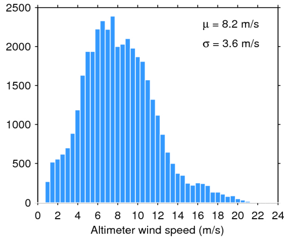
Figure 33. Histogram of flag-valid wind over oceans and lakes for 22/12/2016. The mean ( \mu ) and standard deviation ( \sigma ) are also shown. Note that values larger than 24 m/s are excluded from the histogram for the sake of readability but not from the computation of \mu and \sigma .
