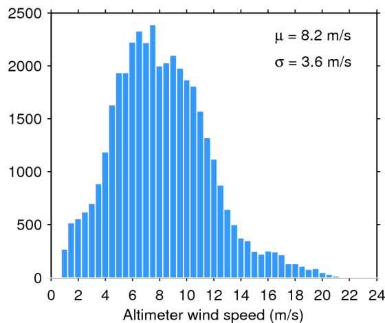
Figure 35. Histogram of science-valid wind over oceans and lakes for 22/12/2016. The mean ( \mu ) and standard deviation ( \sigma ) are also shown. Note that values larger than 24 m/s are excluded from the histogram for the sake of readability but not from the computation of \mu and \sigma .
