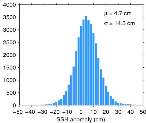
Figure 7. Histogram of flag-valid SSH anomaly over oceans and lakes for 22/12/2016. The mean ( \mu ) and standard deviation ( \sigma ) are also shown. Note that values outside [-50 50] cm are excluded from the histogram for the sake of readability but not from the computation of \mu and \sigma .
