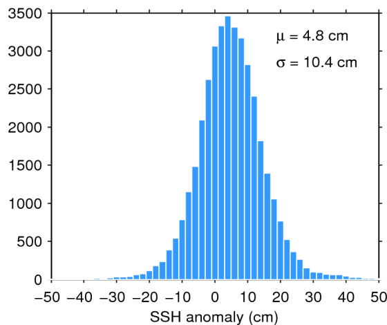
Figure 11. Histogram of science-valid SSH anomaly over oceans and lakes for 22/12/2016. The mean ( \mu ) and standard deviation ( \sigma ) are also shown. Note that values outside [-50 50] cm are excluded from the histogram for the sake of readability but not from the computation of \mu and \sigma .
