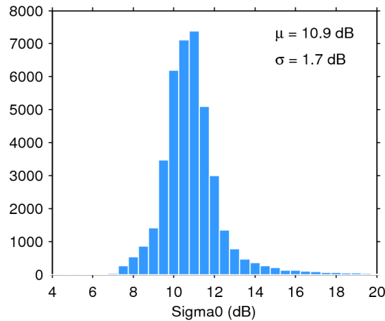
Figure 25. Histogram of flag-valid sigma0 over oceans and lakes for 22/12/2016. The mean ( \mu ) and standard deviation ( \sigma ) are also shown. Note that values outside [4 20] dB are excluded from the histogram for the sake of readability but not from the computation of \mu and \sigma .
