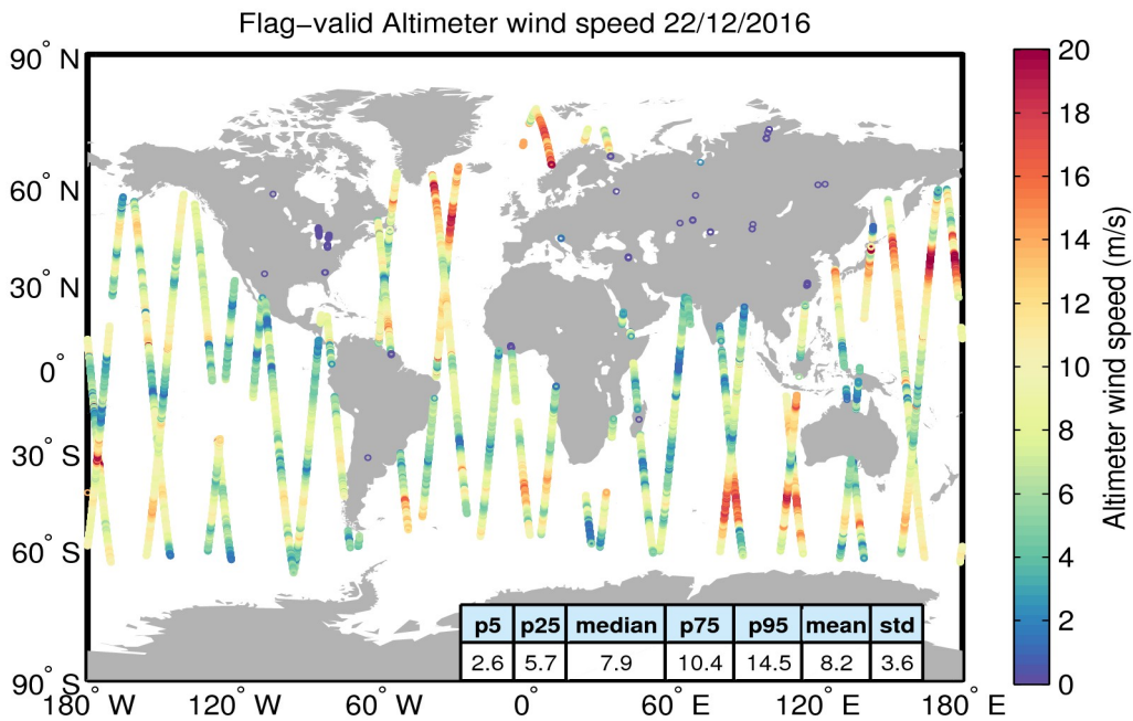
Figure 31. Geographical distribution of flag-valid wind data over oceans and lakes for 22/12/2016. The statistical values shown in the table refer to the wind in m/s and are calculated over all measurements shown in the figure.
