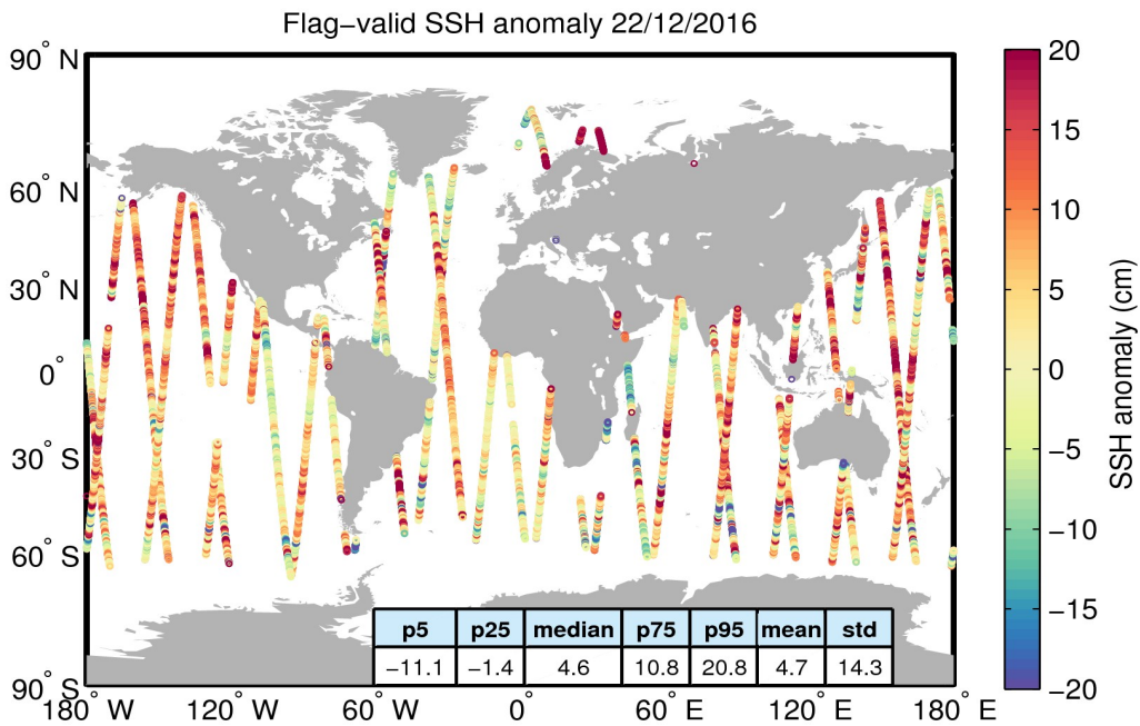
Figure 5. Geographical distribution of flag-valid 1-Hz SSH anomaly data over oceans and lakes for 22/12/2016. The statistical values shown in the table refer to the SSH anomaly in cm and are calculated over all measurements shown in the figure.
