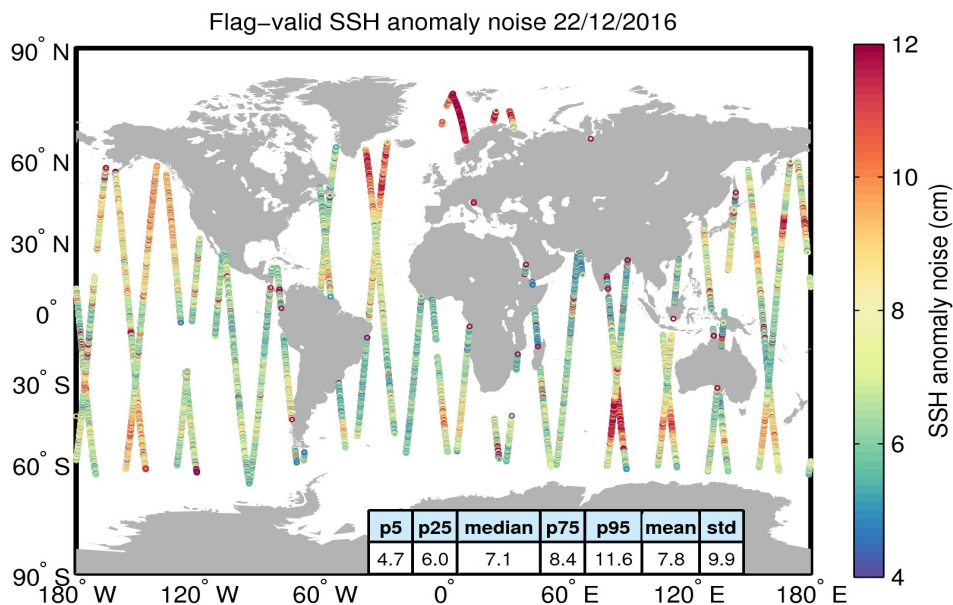
Figure 8. Geographical distribution of flag-valid 20-Hz SSH anomaly measurement noise over oceans and lakes for 22/12/2016. The statistical values shown in the table refer to the SSH anomaly noise and are calculated over all measurements shown in the figure.
