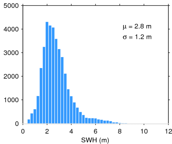
Figure 20. Histogram of science-valid SWH over oceans and lakes for 22/12/2016. The mean ( \mu ) and standard deviation ( \sigma ) are also shown. Note that values larger than 12 m are excluded from the histogram for the sake of readability but not from the computation of \mu and \sigma .
