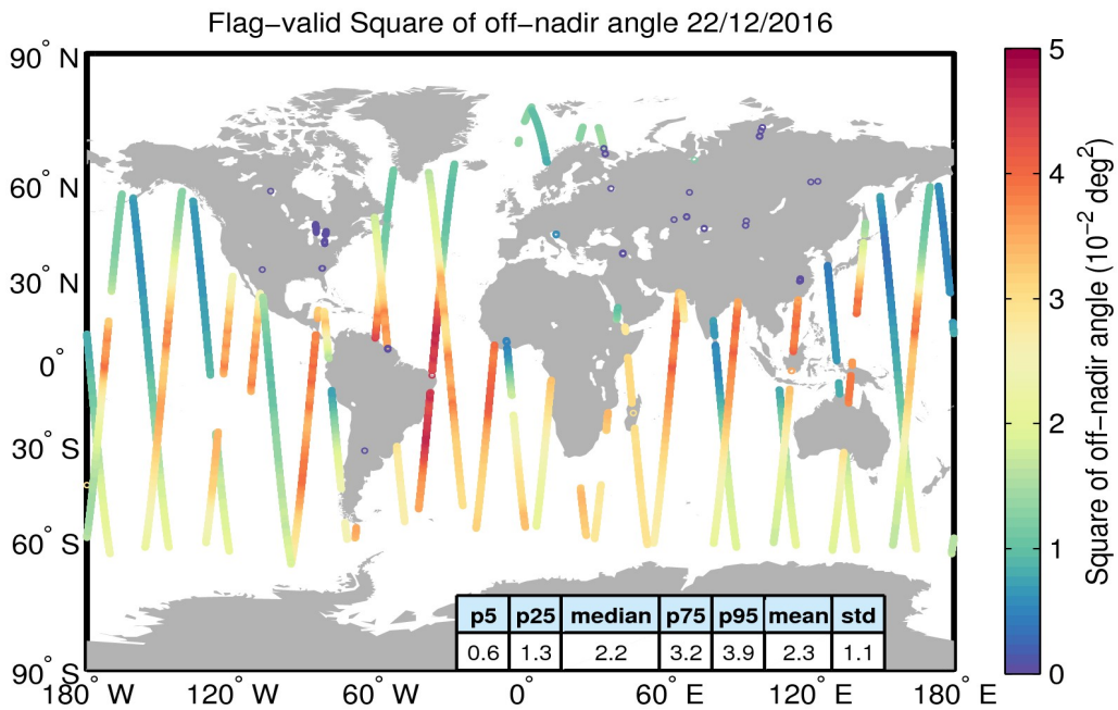
Figure 37. Geographical distribution of flag-valid mispointing data over oceans and lakes for 22/12/2016. The statistical values shown in the table refer to the mispointing in 10^{-2} deg 2 and are calculated over all measurements shown in the figure.
