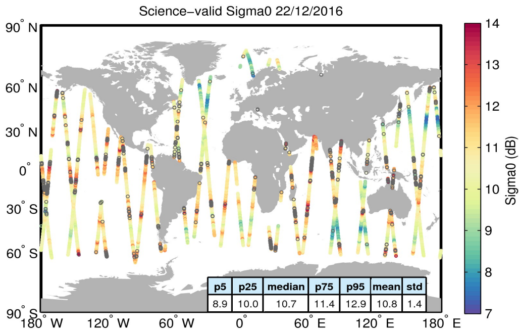
Figure 27. Geographical distribution of science-valid sigma0 data over oceans and lakes for 22/12/2016. The statistical values shown in the table refer to the sigma0 in dB and are calculated over all measurements shown in the figure. Gray circles denote records that have been rejected based on the editing criteria described in Table 4.
