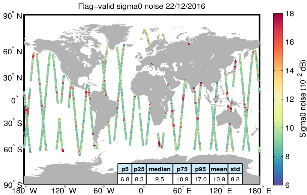
Figure 26. Geographical distribution of flag-valid 20-Hz sigma0 measurement noise over oceans and lakes for 22/12/2016. The statistical values shown in the table refer to the sigma0 noise and are calculated over all measurements shown in the figure.
