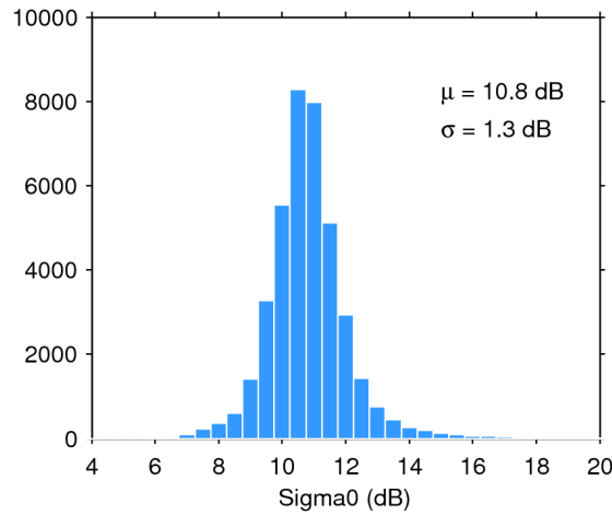
Figure 28. Histogram of science-valid sigma0 over oceans and lakes for 21/12/2016. The mean ( \mu ) and standard deviation ( \sigma ) are also shown. Note that values outside [4 20] dB are excluded from the histogram for the sake of readability but not from the computation of \mu and \sigma .
