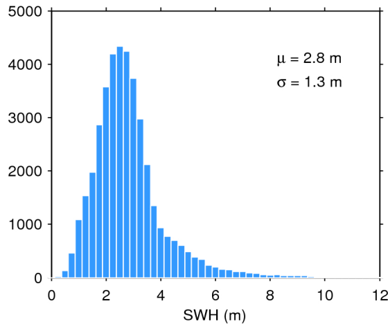
Figure 20. Histogram of science-valid SWH over oceans and lakes for 21/12/2016. The mean ( \mu ) and standard deviation ( \sigma ) are also shown. Note that values larger than 12 m are excluded from the histogram for the sake of readability but not from the computation of \mu and \sigma .
