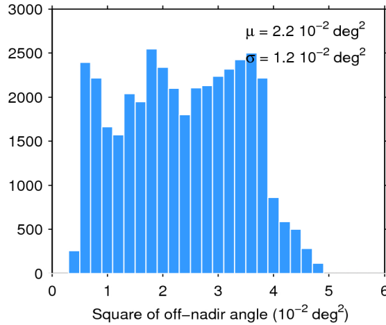
Figure 39. Histogram of flag-valid mispointing over oceans and lakes for 21/12/2016. The mean ( \mu ) and standard deviation ( \sigma ) are also shown. Note that values larger than 6 \cdot 10^{-2} \text{ deg}^2 are excluded from the histogram for the sake of readability but not from the computation of \mu and \sigma .
