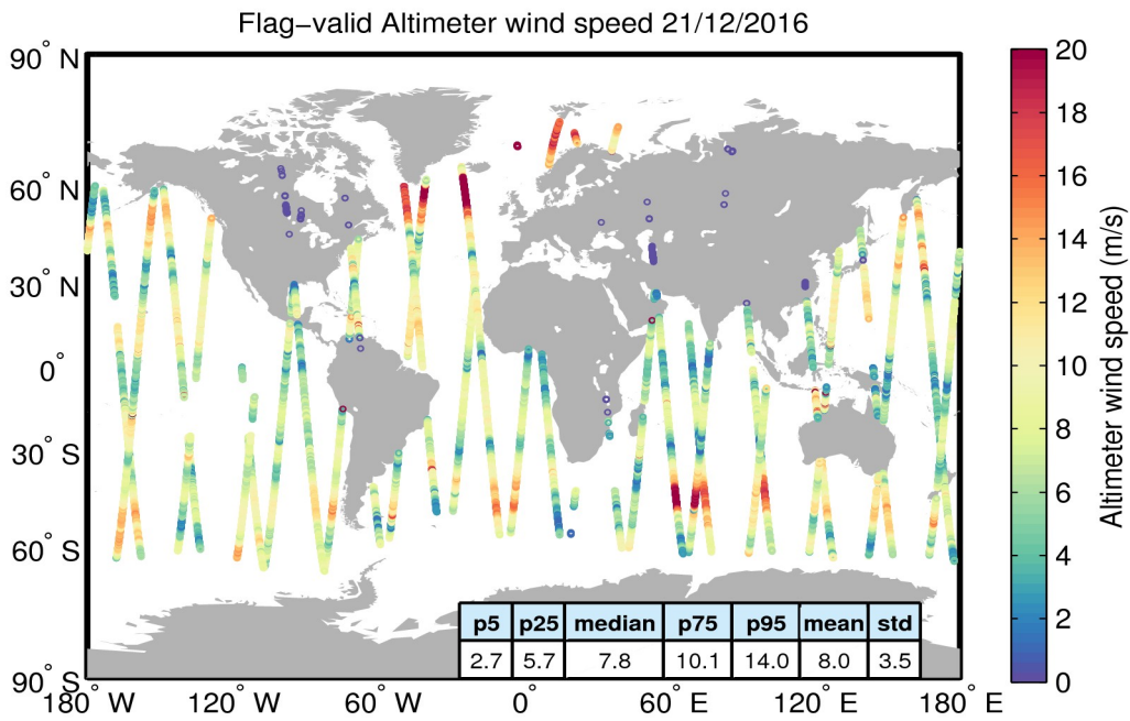
Figure 31. Geographical distribution of flag-valid wind data over oceans and lakes for 21/12/2016. The statistical values shown in the table refer to the wind in m/s and are calculated over all measurements shown in the figure.
