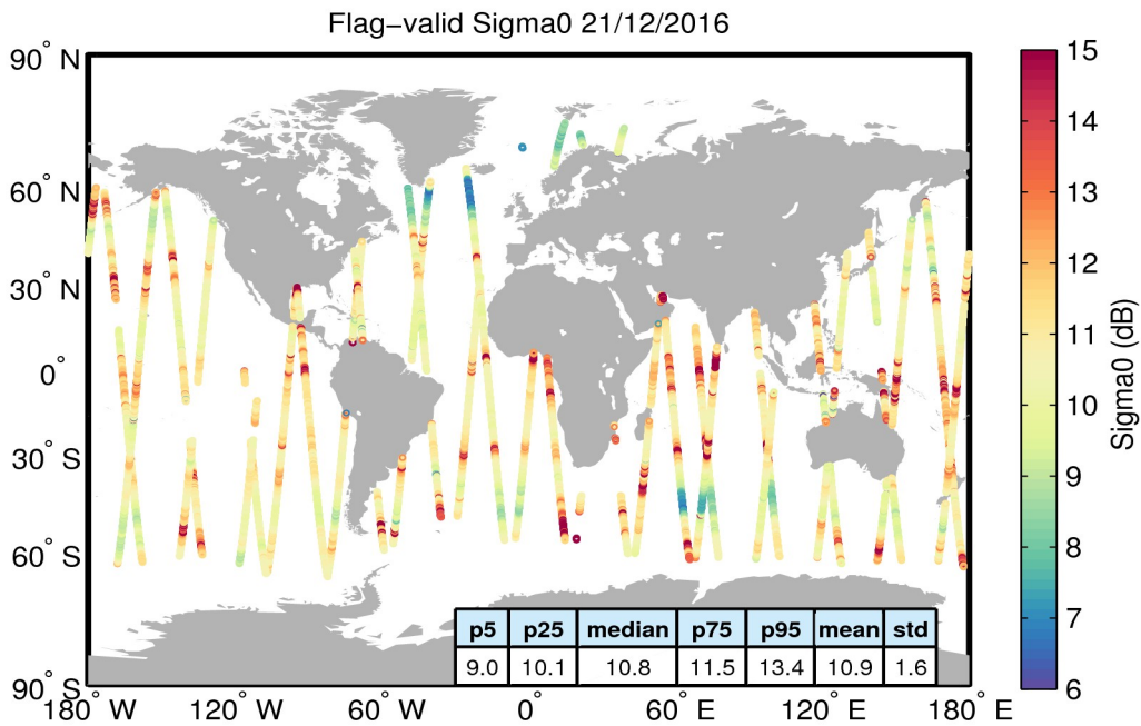
Figure 23. Geographical distribution of flag-valid sigma0 data over oceans and lakes for 21/12/2016. The statistical values shown in the table refer to the sigma0 in dB and are calculated over all measurements shown in the figure.
