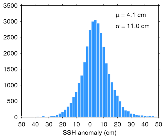
Figure 11. Histogram of science-valid SSH anomaly over oceans and lakes for 21/12/2016. The mean ( \mu ) and standard deviation ( \sigma ) are also shown. Note that values outside [-50 50] cm are excluded from the histogram for the sake of readability but not from the computation of \mu and \sigma .
