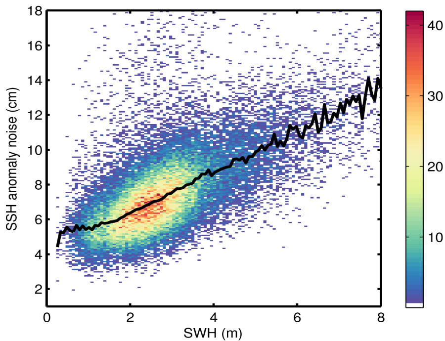
Figure 9. 2D histogram showing flag-valid SSH anomaly noise as a function of SWH for 21/12/2016. The black line denotes the median SSH anomaly noise as a function of SWH.
