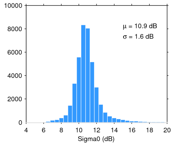
Figure 25. Histogram of flag-valid sigma0 over oceans and lakes for 21/12/2016. The mean ( \mu ) and standard deviation ( \sigma ) are also shown. Note that values outside [4 20] dB are excluded from the histogram for the sake of readability but not from the computation of \mu and \sigma .
