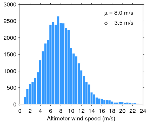
Figure 33. Histogram of flag-valid wind over oceans and lakes for 21/12/2016. The mean ( \mu ) and standard deviation ( \sigma ) are also shown. Note that values larger than 24 m/s are excluded from the histogram for the sake of readability but not from the computation of \mu and \sigma .
