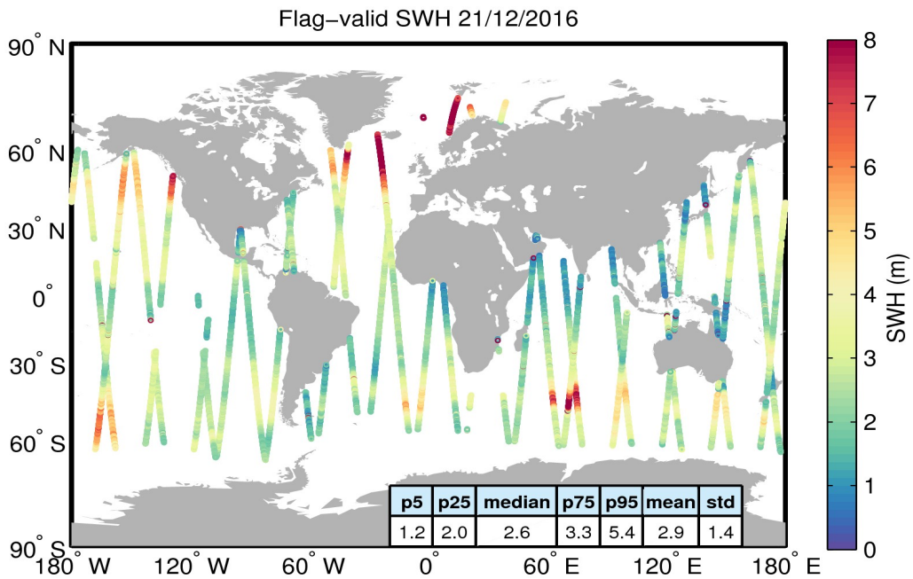
Figure 15. Geographical distribution of flag-valid SWH data over oceans and lakes for 21/12/2016. The statistical values shown in the table refer to the SWH in m and are calculated over all measurements shown in the figure.
