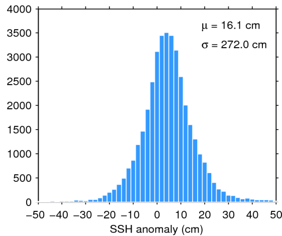
Figure 7. Histogram of flag-valid SSH anomaly over oceans and lakes for 21/12/2016. The mean ( \mu ) and standard deviation ( \sigma ) are also shown. Note that values outside [-50 50] cm are excluded from the histogram for the sake of readability but not from the computation of \mu and \sigma .
