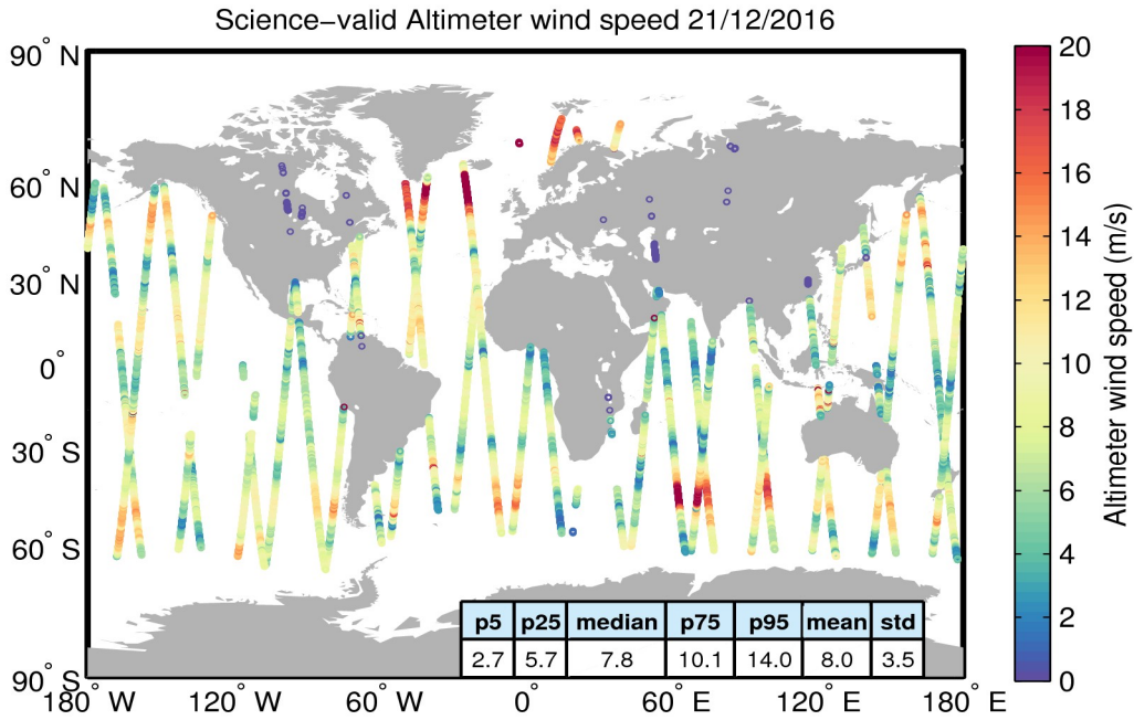
Figure 34. Geographical distribution of science-valid wind data over oceans and lakes for 21/12/2016. The statistical values shown in the table refer to the wind in m/s and are calculated over all measurements shown in the figure. Gray circles denote records that have been rejected based on the editing criteria described in Table 5.
