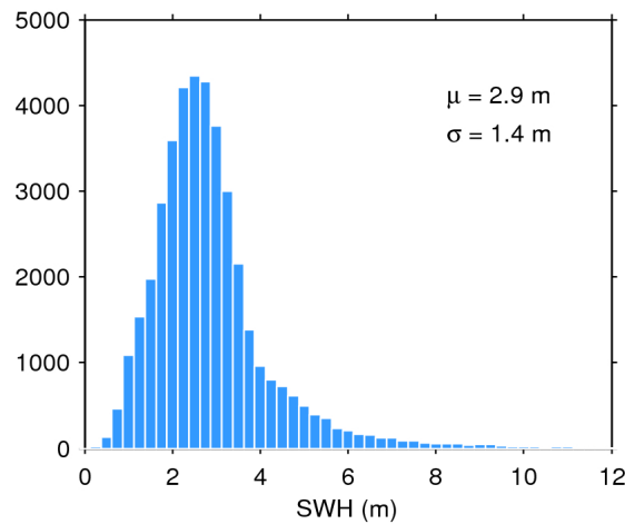
Figure 17. Histogram of flag-valid SWH over oceans and lakes for 21/12/2016. The mean ( \mu ) and standard deviation ( \sigma ) are also shown. Note that values larger than 12 m are excluded from the histogram for the sake of readability but not from the computation of \mu and \sigma .
