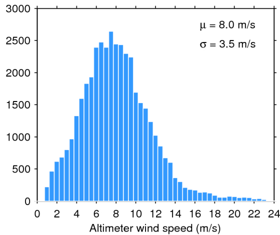
Figure 35. Histogram of science-valid wind over oceans and lakes for 21/12/2016. The mean ( \mu ) and standard deviation ( \sigma ) are also shown. Note that values larger than 24 m/s are excluded from the histogram for the sake of readability but not from the computation of \mu and \sigma .
