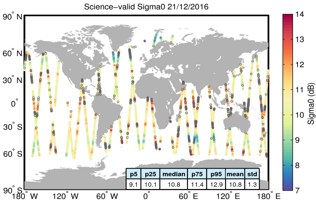
Figure 27. Geographical distribution of science-valid sigma0 data over oceans and lakes for 21/12/2016. The statistical values shown in the table refer to the sigma0 in dB and are calculated over all measurements shown in the figure. Gray circles denote records that have been rejected based on the editing criteria described in Table 4.
