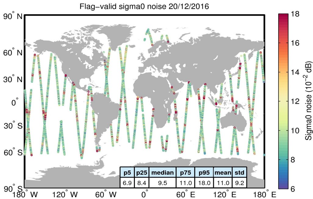
Figure 26. Geographical distribution of flag-valid 20-Hz sigma0 measurement noise over oceans and lakes for 20/12/2016. The statistical values shown in the table refer to the sigma0 noise and are calculated over all measurements shown in the figure.
