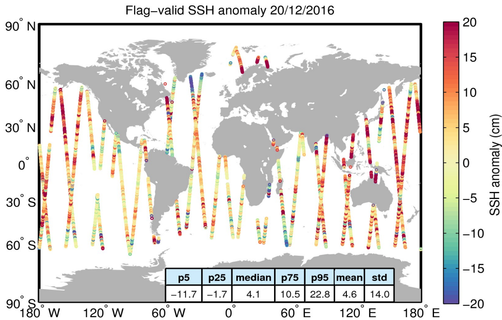
Figure 5. Geographical distribution of flag-valid 1-Hz SSH anomaly data over oceans and lakes for 20/12/2016. The statistical values shown in the table refer to the SSH anomaly in cm and are calculated over all measurements shown in the figure.
