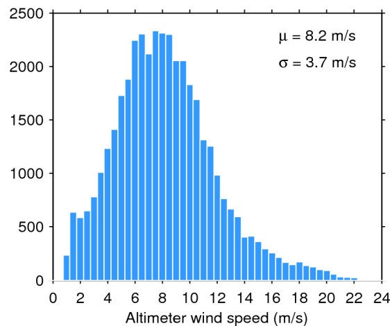
Figure 35. Histogram of science-valid wind over oceans and lakes for 20/12/2016. The mean ( \mu ) and standard deviation ( \sigma ) are also shown. Note that values larger than 24 m/s are excluded from the histogram for the sake of readability but not from the computation of \mu and \sigma .
