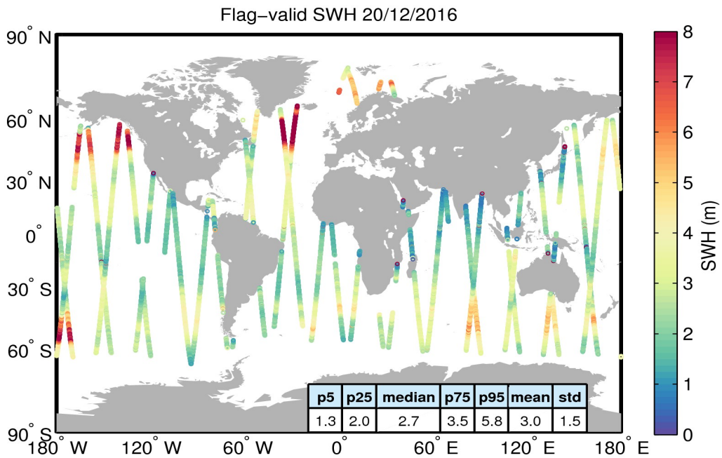
Figure 15. Geographical distribution of flag-valid SWH data over oceans and lakes for 20/12/2016. The statistical values shown in the table refer to the SWH in m and are calculated over all measurements shown in the figure.
