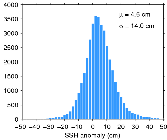
Figure 7. Histogram of flag-valid SSH anomaly over oceans and lakes for 20/12/2016. The mean ( \mu ) and standard deviation ( \sigma ) are also shown. Note that values outside [-50 50] cm are excluded from the histogram for the sake of readability but not from the computation of \mu and \sigma .
