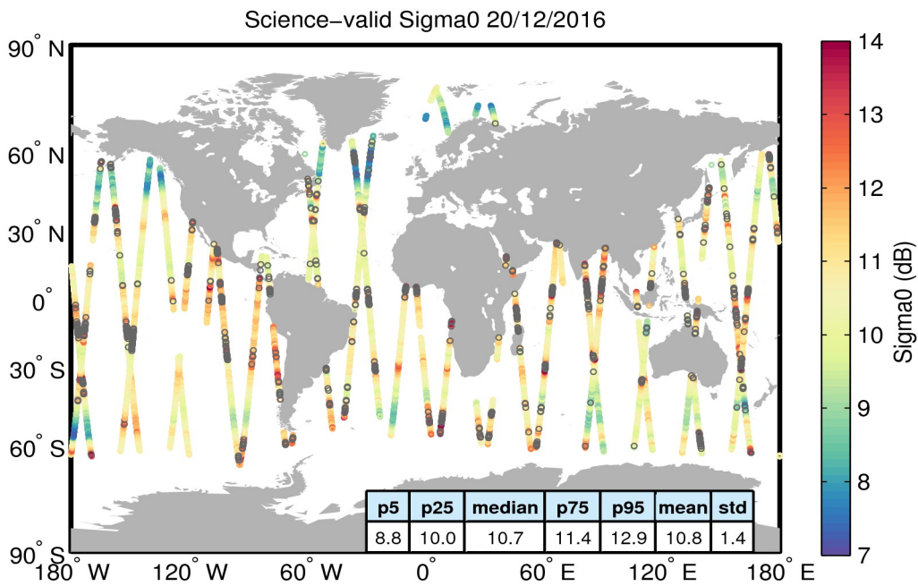
Figure 27. Geographical distribution of science-valid sigma0 data over oceans and lakes for 20/12/2016. The statistical values shown in the table refer to the sigma0 in dB and are calculated over all measurements shown in the figure. Gray circles denote records that have been rejected based on the editing criteria described in Table 4.
