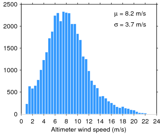
Figure 33. Histogram of flag-valid wind over oceans and lakes for 20/12/2016. The mean ( \mu ) and standard deviation ( \sigma ) are also shown. Note that values larger than 24 m/s are excluded from the histogram for the sake of readability but not from the computation of \mu and \sigma .
