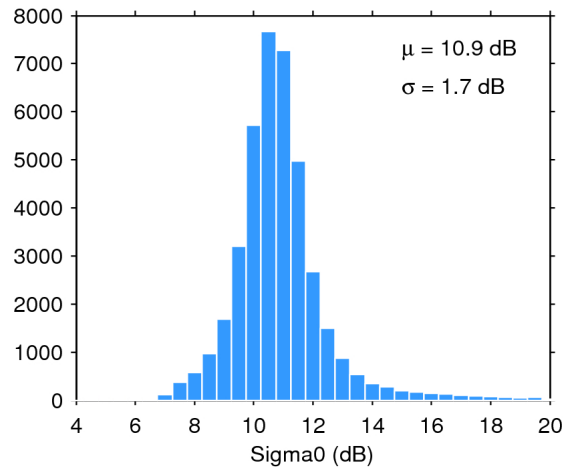
Figure 25. Histogram of flag-valid sigma0 over oceans and lakes for 20/12/2016. The mean ( \mu ) and standard deviation ( \sigma ) are also shown. Note that values outside [4 20] dB are excluded from the histogram for the sake of readability but not from the computation of \mu and \sigma .
