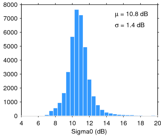
Figure 28. Histogram of science-valid sigma0 over oceans and lakes for 20/12/2016. The mean ( \mu ) and standard deviation ( \sigma ) are also shown. Note that values outside [4 20] dB are excluded from the histogram for the sake of readability but not from the computation of \mu and \sigma .
