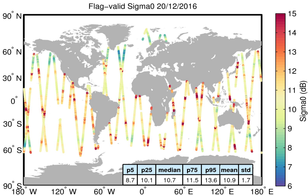
Figure 23. Geographical distribution of flag-valid sigma0 data over oceans and lakes for 20/12/2016. The statistical values shown in the table refer to the sigma0 in dB and are calculated over all measurements shown in the figure.
