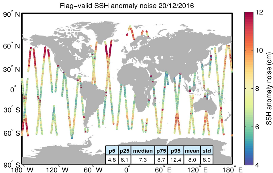
Figure 8. Geographical distribution of flag-valid 20-Hz SSH anomaly measurement noise over oceans and lakes for 20/12/2016. The statistical values shown in the table refer to the SSH anomaly noise and are calculated over all measurements shown in the figure.
