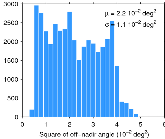
Figure 39. Histogram of flag-valid mispointing over oceans and lakes for 20/12/2016. The mean ( \mu ) and standard deviation ( \sigma ) are also shown. Note that values larger than 6 \cdot 10^{-2} \text{ deg}^2 are excluded from the histogram for the sake of readability but not from the computation of \mu and \sigma .
