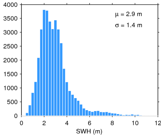
Figure 20. Histogram of science-valid SWH over oceans and lakes for 20/12/2016. The mean ( \mu ) and standard deviation ( \sigma ) are also shown. Note that values larger than 12 m are excluded from the histogram for the sake of readability but not from the computation of \mu and \sigma .
