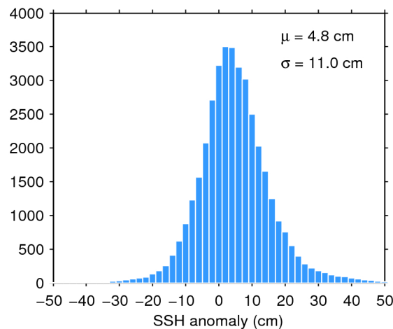
Figure 11. Histogram of science-valid SSH anomaly over oceans and lakes for 20/12/2016. The mean ( \mu ) and standard deviation ( \sigma ) are also shown. Note that values outside [-50 50] cm are excluded from the histogram for the sake of readability but not from the computation of \mu and \sigma .
