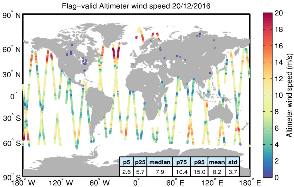
Figure 31. Geographical distribution of flag-valid wind data over oceans and lakes for 20/12/2016. The statistical values shown in the table refer to the wind in m/s and are calculated over all measurements shown in the figure.
