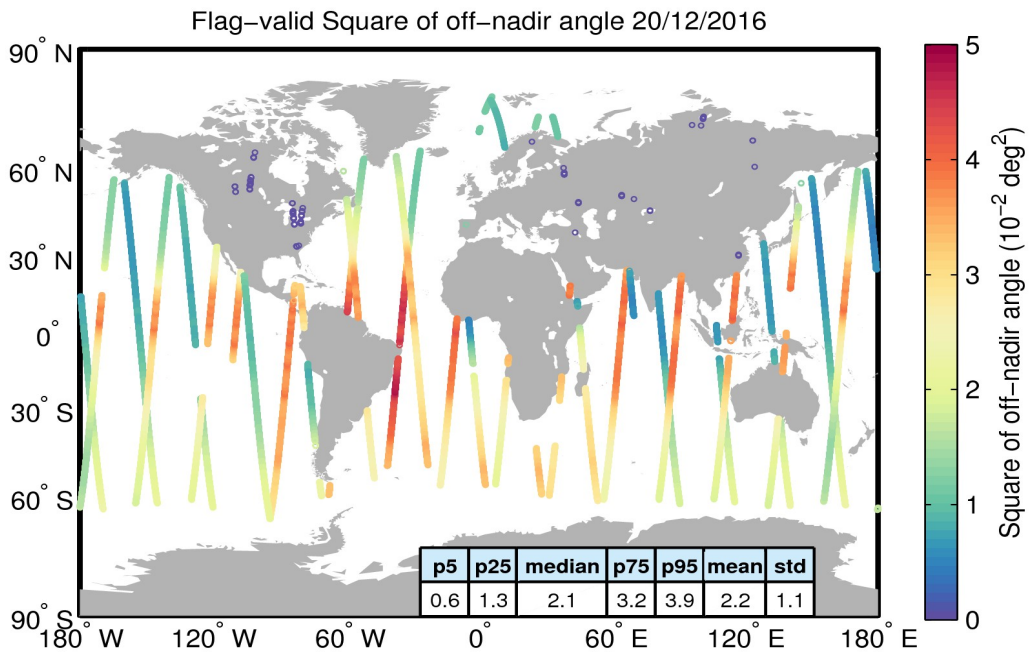
Figure 37. Geographical distribution of flag-valid mispointing data over oceans and lakes for 20/12/2016. The statistical values shown in the table refer to the mispointing in 10^{-2} deg 2 and are calculated over all measurements shown in the figure.
