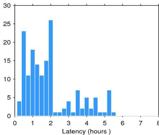
Figure 2. Histogram of the data latency for 20/12/2016. The y-axis denotes the number of files that are made available with a delay of x-hours with respect to the mean time of the records stored in the file.
