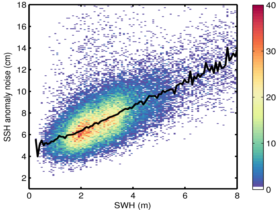
Figure 9. 2D histogram showing flag-valid SSH anomaly noise as a function of SWH for 20/12/2016. The black line denotes the median SSH anomaly noise as a function of SWH.
