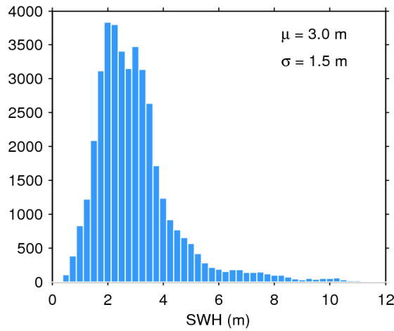
Figure 17. Histogram of flag-valid SWH over oceans and lakes for 20/12/2016. The mean ( \mu ) and standard deviation ( \sigma ) are also shown. Note that values larger than 12 m are excluded from the histogram for the sake of readability but not from the computation of \mu and \sigma .
