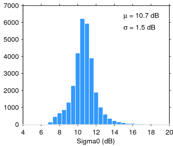
Figure 28. Histogram of science-valid sigma0 over oceans and lakes for 18/12/2016. The mean ( \mu ) and standard deviation ( \sigma ) are also shown. Note that values outside [4 20] dB are excluded from the histogram for the sake of readability but not from the computation of \mu and \sigma .
