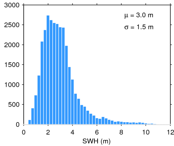
Figure 17. Histogram of flag-valid SWH over oceans and lakes for 18/12/2016. The mean ( \mu ) and standard deviation ( \sigma ) are also shown. Note that values larger than 12 m are excluded from the histogram for the sake of readability but not from the computation of \mu and \sigma .
