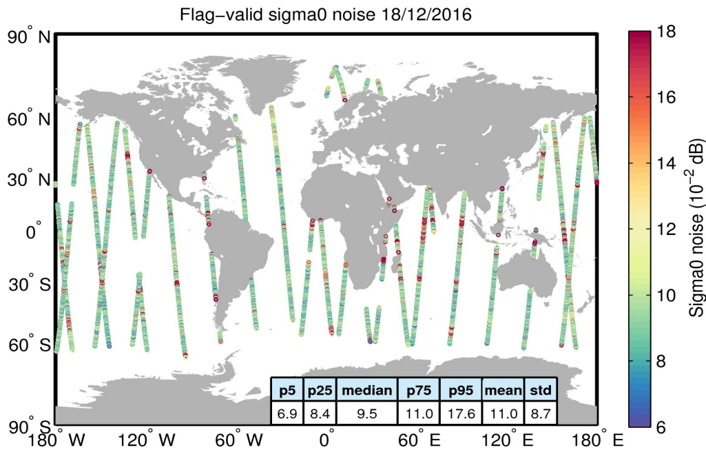
Figure 26. Geographical distribution of flag-valid 20-Hz sigma0 measurement noise over oceans and lakes for 18/12/2016. The statistical values shown in the table refer to the sigma0 noise and are calculated over all measurements shown in the figure.
