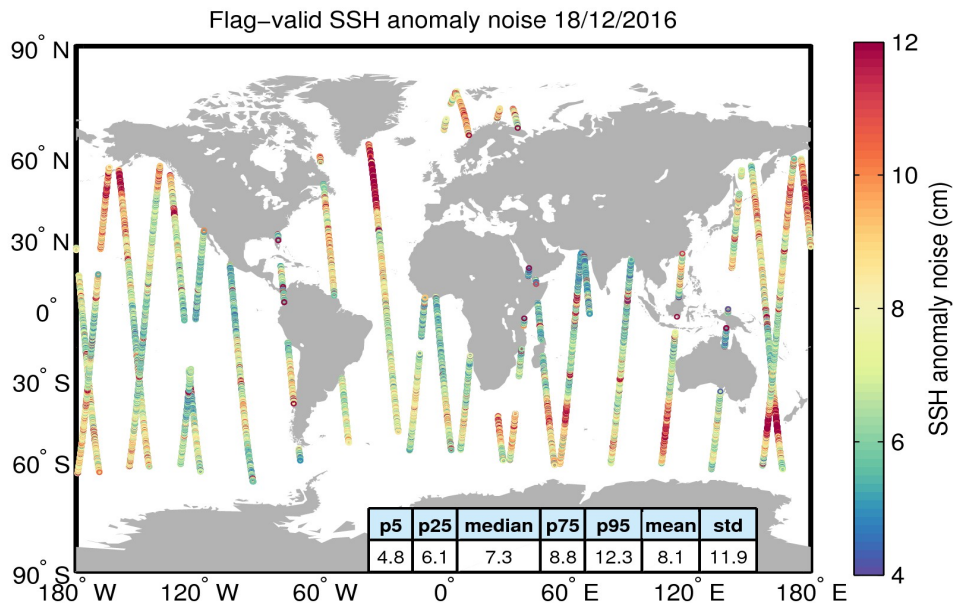
Figure 8. Geographical distribution of flag-valid 20-Hz SSH anomaly measurement noise over oceans and lakes for 18/12/2016. The statistical values shown in the table refer to the SSH anomaly noise and are calculated over all measurements shown in the figure.
