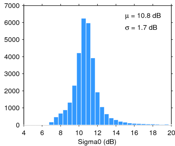
Figure 25. Histogram of flag-valid sigma0 over oceans and lakes for 18/12/2016. The mean ( \mu ) and standard deviation ( \sigma ) are also shown. Note that values outside [4 20] dB are excluded from the histogram for the sake of readability but not from the computation of \mu and \sigma .
