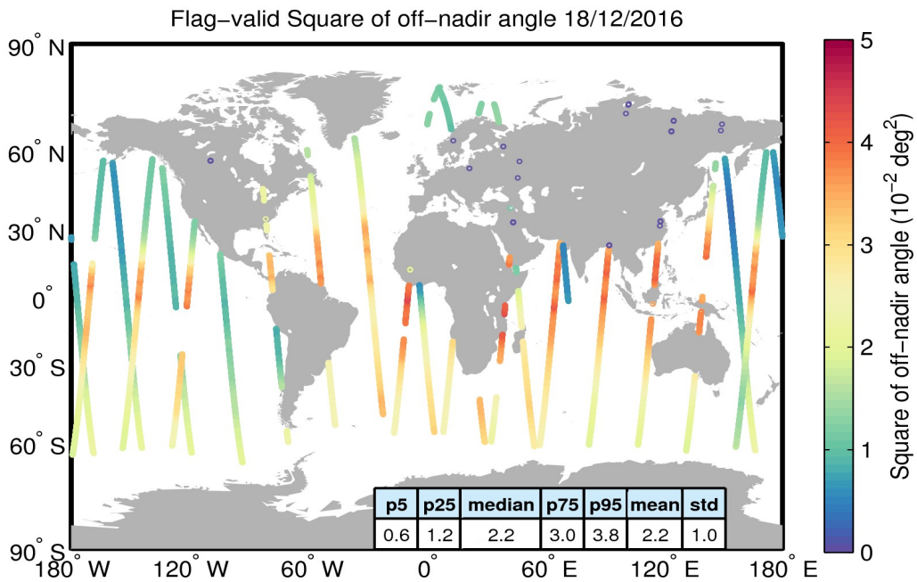
Figure 37. Geographical distribution of flag-valid mispointing data over oceans and lakes for 18/12/2016. The statistical values shown in the table refer to the mispointing in 10^{-2} deg 2 and are calculated over all measurements shown in the figure.
