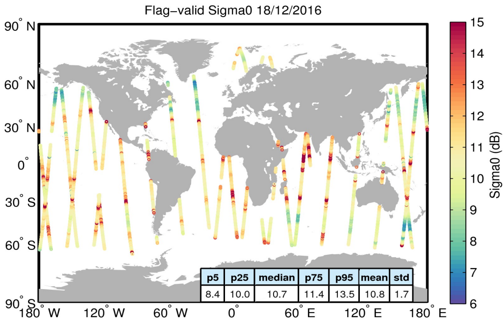
Figure 23. Geographical distribution of flag-valid sigma0 data over oceans and lakes for 18/12/2016. The statistical values shown in the table refer to the sigma0 in dB and are calculated over all measurements shown in the figure.
