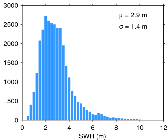
Figure 20. Histogram of science-valid SWH over oceans and lakes for 18/12/2016. The mean ( \mu ) and standard deviation ( \sigma ) are also shown. Note that values larger than 12 m are excluded from the histogram for the sake of readability but not from the computation of \mu and \sigma .
