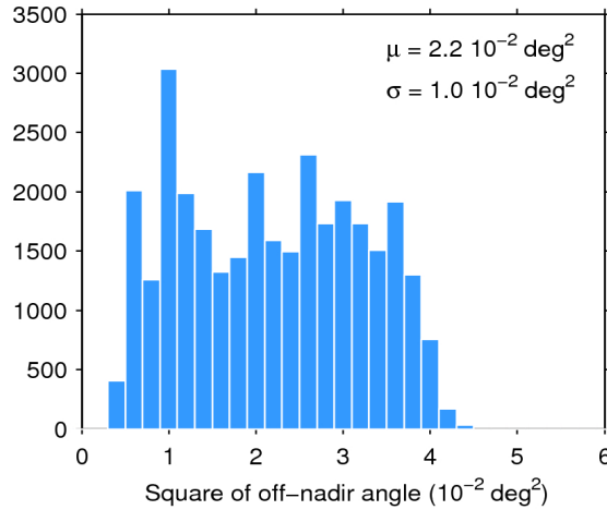
Figure 39. Histogram of flag-valid mispointing over oceans and lakes for 18/12/2016. The mean ( \mu ) and standard deviation ( \sigma ) are also shown. Note that values larger than 6 \cdot 10^{-2} \text{ deg}^2 are excluded from the histogram for the sake of readability but not from the computation of \mu and \sigma .
