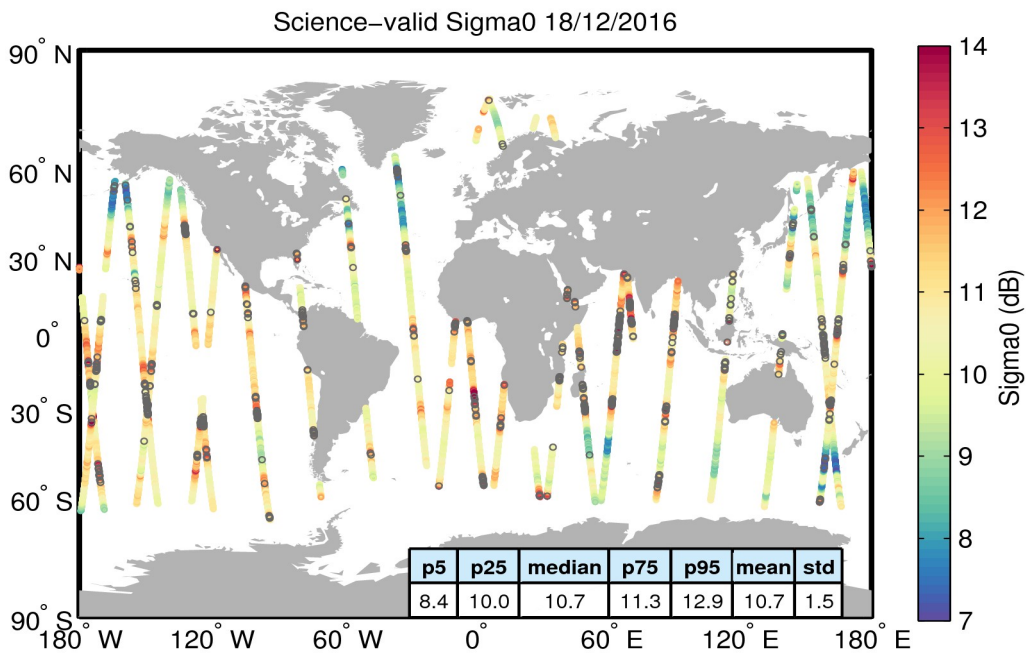
Figure 27. Geographical distribution of science-valid sigma0 data over oceans and lakes for 18/12/2016. The statistical values shown in the table refer to the sigma0 in dB and are calculated over all measurements shown in the figure. Gray circles denote records that have been rejected based on the editing criteria described in Table 4.
