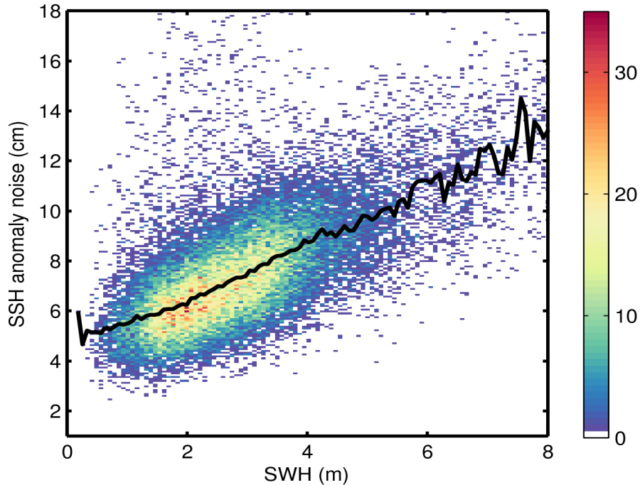
Figure 9. 2D histogram showing flag-valid SSH anomaly noise as a function of SWH for 18/12/2016. The black line denotes the median SSH anomaly noise as a function of SWH.
