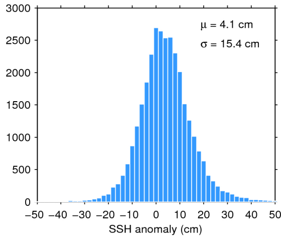
Figure 7. Histogram of flag-valid SSH anomaly over oceans and lakes for 18/12/2016. The mean ( \mu ) and standard deviation ( \sigma ) are also shown. Note that values outside [-50 50] cm are excluded from the histogram for the sake of readability but not from the computation of \mu and \sigma .
