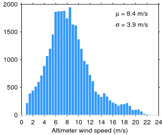
Figure 33. Histogram of flag-valid wind over oceans and lakes for 18/12/2016. The mean ( \mu ) and standard deviation ( \sigma ) are also shown. Note that values larger than 24 m/s are excluded from the histogram for the sake of readability but not from the computation of \mu and \sigma .
