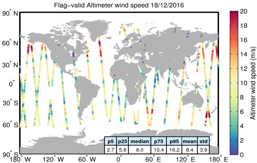
Figure 31. Geographical distribution of flag-valid wind data over oceans and lakes for 18/12/2016. The statistical values shown in the table refer to the wind in m/s and are calculated over all measurements shown in the figure.
