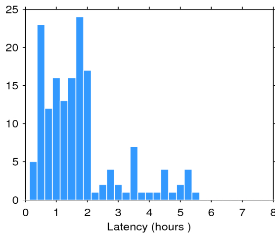
Figure 2. Histogram of the data latency for 18/12/2016. The y-axis denotes the number of files that are made available with a delay of x-hours with respect to the mean time of the records stored in the file.
