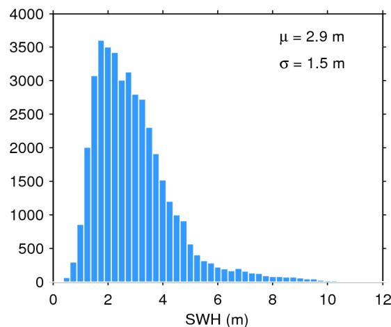
Figure 20. Histogram of science-valid SWH over oceans and lakes for 17/12/2016. The mean ( \mu ) and standard deviation ( \sigma ) are also shown. Note that values larger than 12 m are excluded from the histogram for the sake of readability but not from the computation of \mu and \sigma .
