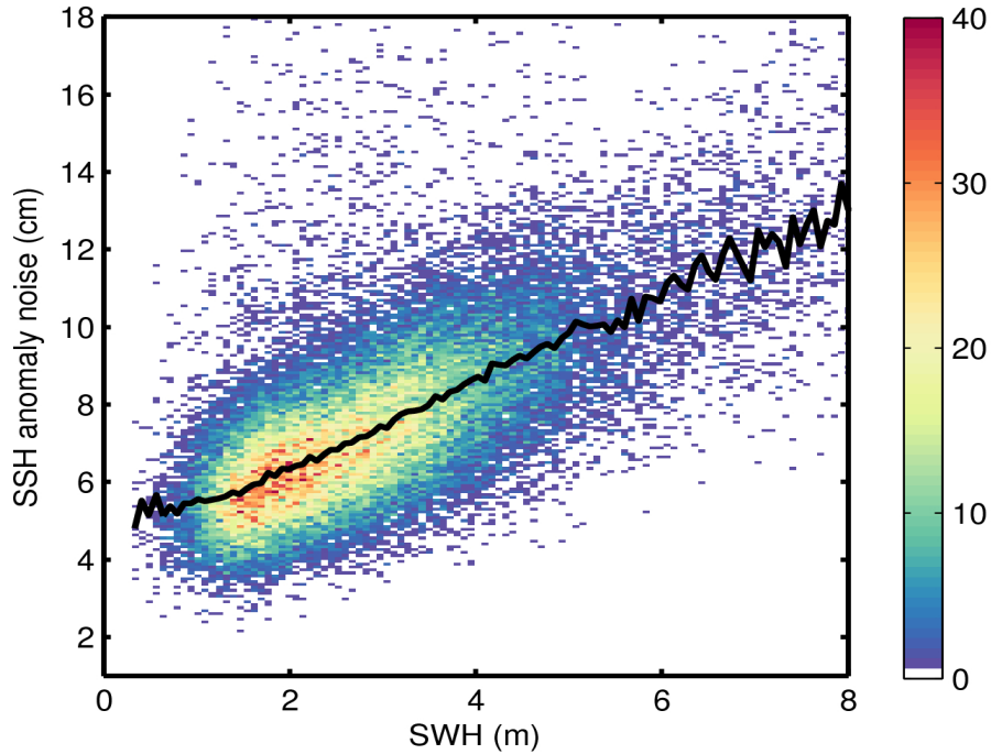
Figure 9. 2D histogram showing flag-valid SSH anomaly noise as a function of SWH for 17/12/2016. The black line denotes the median SSH anomaly noise as a function of SWH.
