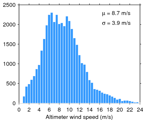
Figure 35. Histogram of science-valid wind over oceans and lakes for 17/12/2016. The mean ( \mu ) and standard deviation ( \sigma ) are also shown. Note that values larger than 24 m/s are excluded from the histogram for the sake of readability but not from the computation of \mu and \sigma .
