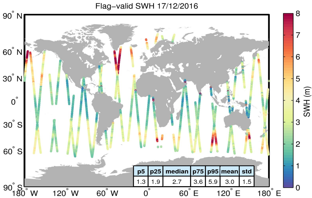
Figure 15. Geographical distribution of flag-valid SWH data over oceans and lakes for 17/12/2016. The statistical values shown in the table refer to the SWH in m and are calculated over all measurements shown in the figure.
