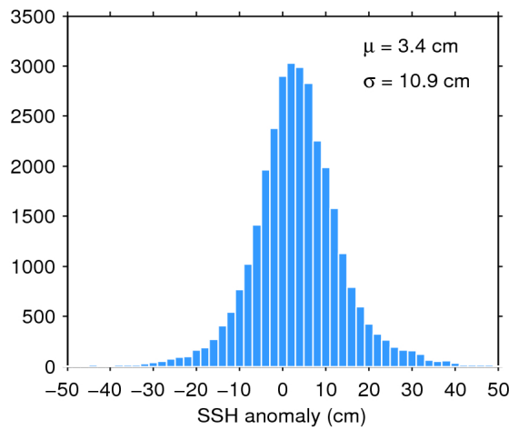
Figure 11. Histogram of science-valid SSH anomaly over oceans and lakes for 17/12/2016. The mean ( \mu ) and standard deviation ( \sigma ) are also shown. Note that values outside [-50 50] cm are excluded from the histogram for the sake of readability but not from the computation of \mu and \sigma .
