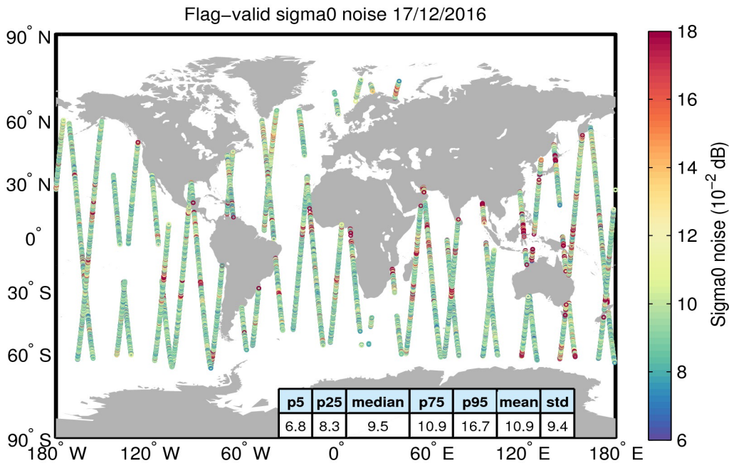
Figure 26. Geographical distribution of flag-valid 20-Hz sigma0 measurement noise over oceans and lakes for 17/12/2016. The statistical values shown in the table refer to the sigma0 noise and are calculated over all measurements shown in the figure.
