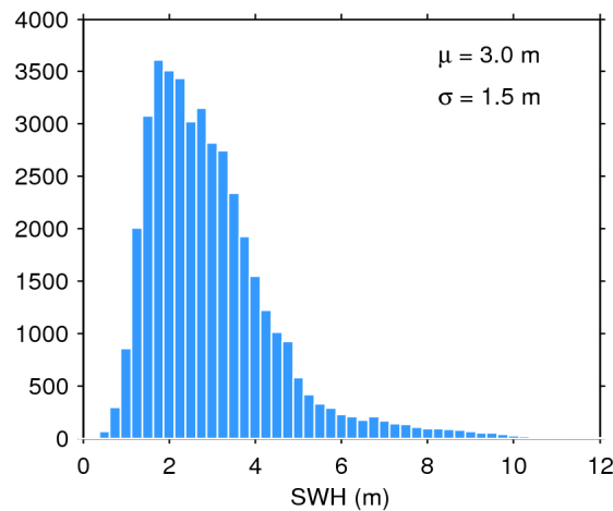
Figure 17. Histogram of flag-valid SWH over oceans and lakes for 17/12/2016. The mean ( \mu ) and standard deviation ( \sigma ) are also shown. Note that values larger than 12 m are excluded from the histogram for the sake of readability but not from the computation of \mu and \sigma .
