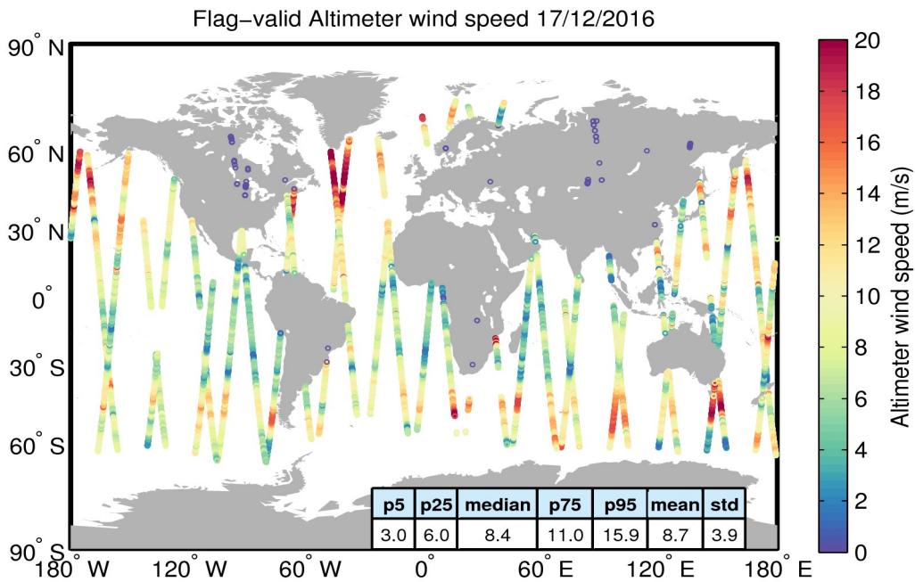
Figure 31. Geographical distribution of flag-valid wind data over oceans and lakes for 17/12/2016. The statistical values shown in the table refer to the wind in m/s and are calculated over all measurements shown in the figure.
