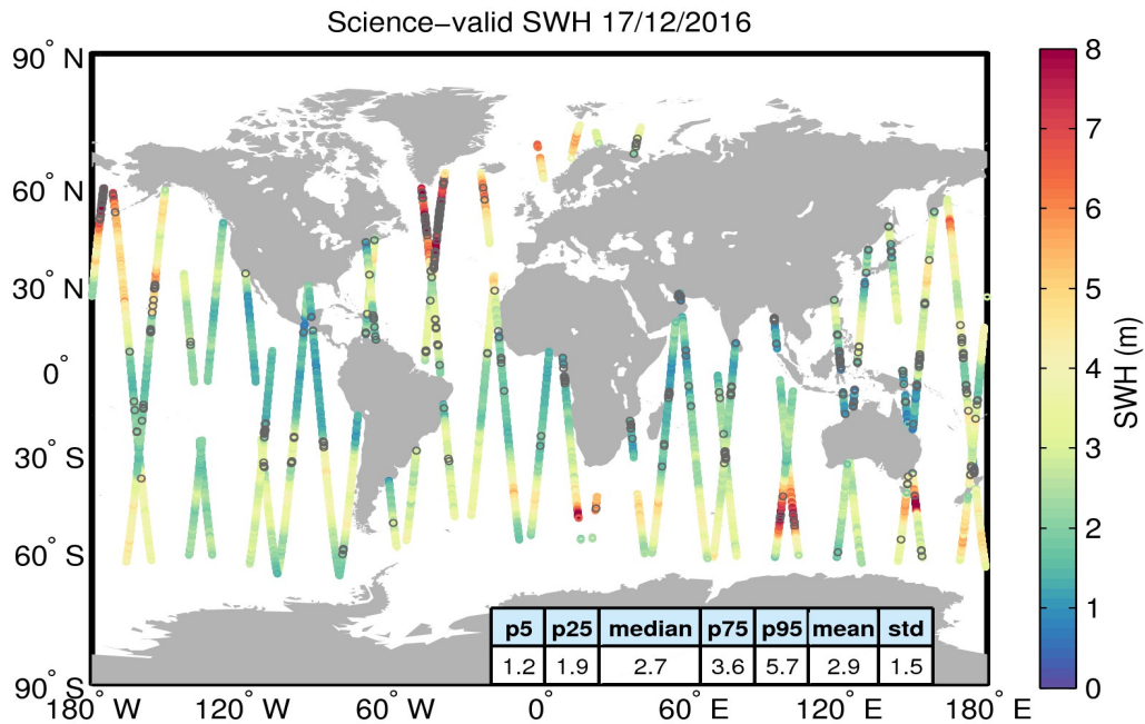
Figure 19. Geographical distribution of science-valid SWH data over oceans and lakes for 17/12/2016. The statistical values shown in the table refer to the SWH in m and are calculated over all measurements shown in the figure. Gray circles denote records that have been rejected based on the editing criteria described in Table 3.
