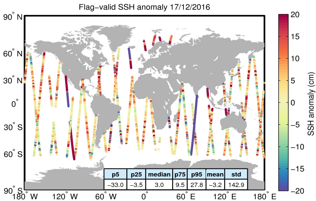
Figure 5. Geographical distribution of flag-valid 1-Hz SSH anomaly data over oceans and lakes for 17/12/2016. The statistical values shown in the table refer to the SSH anomaly in cm and are calculated over all measurements shown in the figure.
