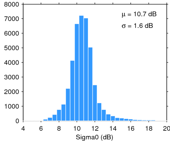
Figure 25. Histogram of flag-valid sigma0 over oceans and lakes for 17/12/2016. The mean ( \mu ) and standard deviation ( \sigma ) are also shown. Note that values outside [4 20] dB are excluded from the histogram for the sake of readability but not from the computation of \mu and \sigma .
