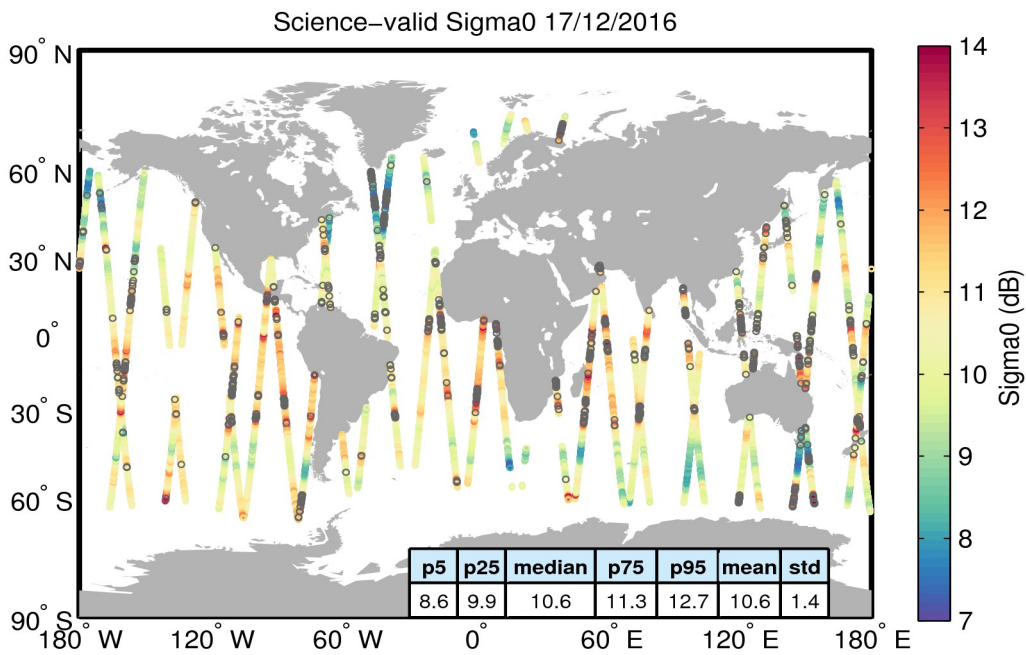
Figure 27. Geographical distribution of science-valid sigma0 data over oceans and lakes for 17/12/2016. The statistical values shown in the table refer to the sigma0 in dB and are calculated over all measurements shown in the figure. Gray circles denote records that have been rejected based on the editing criteria described in Table 4.
