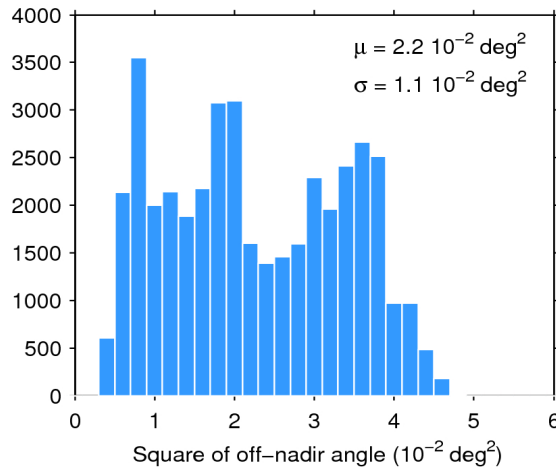
Figure 39. Histogram of flag-valid mispointing over oceans and lakes for 17/12/2016. The mean ( \mu ) and standard deviation ( \sigma ) are also shown. Note that values larger than 6 \cdot 10^{-2} \text{ deg}^2 are excluded from the histogram for the sake of readability but not from the computation of \mu and \sigma .
