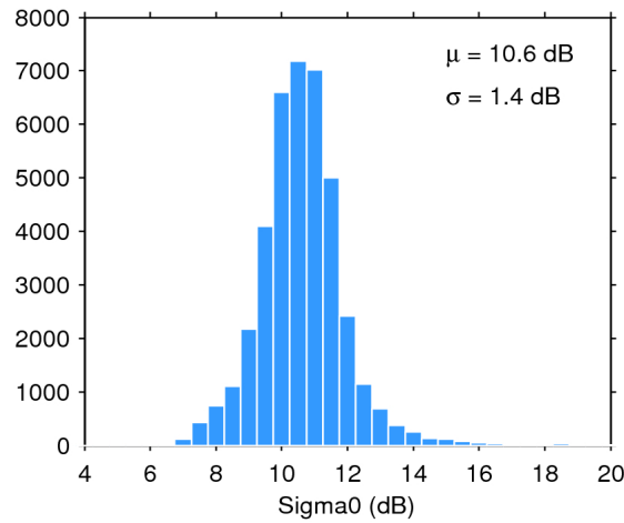
Figure 28. Histogram of science-valid sigma0 over oceans and lakes for 17/12/2016. The mean ( \mu ) and standard deviation ( \sigma ) are also shown. Note that values outside [4 20] dB are excluded from the histogram for the sake of readability but not from the computation of \mu and \sigma .
