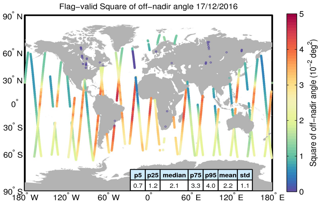
Figure 37. Geographical distribution of flag-valid mispointing data over oceans and lakes for 17/12/2016. The statistical values shown in the table refer to the mispointing in 10^{-2} deg 2 and are calculated over all measurements shown in the figure.
