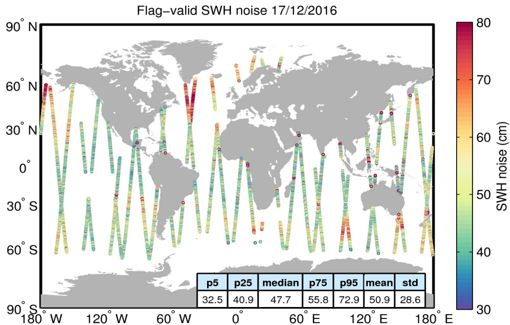
Figure 18. Geographical distribution of flag-valid 20-Hz SWH measurement noise over oceans and lakes for 17/12/2016. The statistical values shown in the table refer to the SWH noise and are calculated over all measurements shown in the figure.
