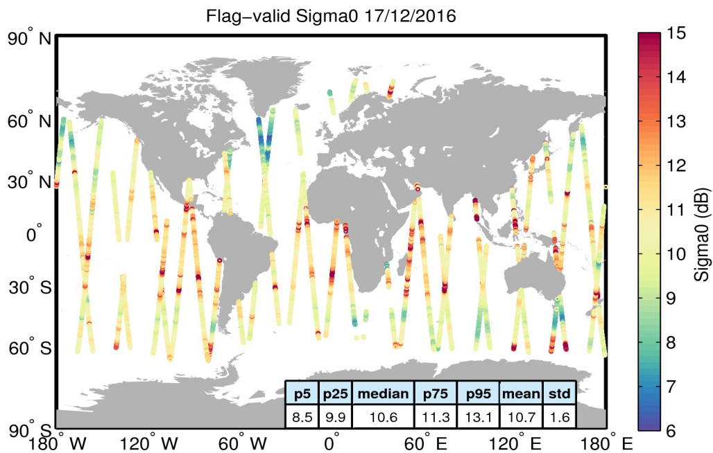
Figure 23. Geographical distribution of flag-valid sigma0 data over oceans and lakes for 17/12/2016. The statistical values shown in the table refer to the sigma0 in dB and are calculated over all measurements shown in the figure.
