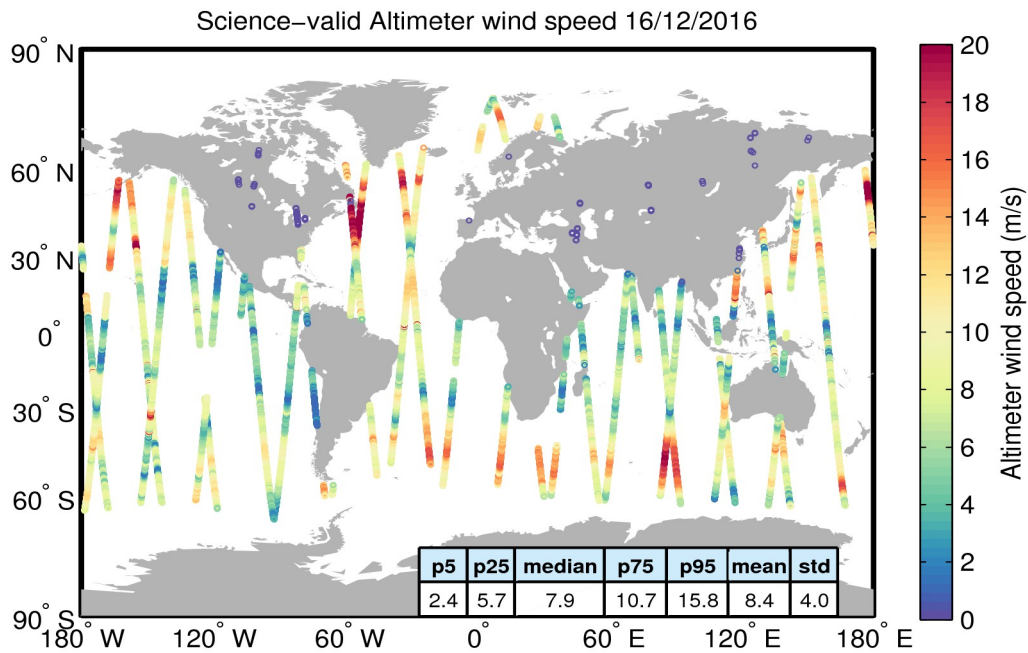
Figure 34. Geographical distribution of science-valid wind data over oceans and lakes for 16/12/2016. The statistical values shown in the table refer to the wind in m/s and are calculated over all measurements shown in the figure. Gray circles denote records that have been rejected based on the editing criteria described in Table 5.
