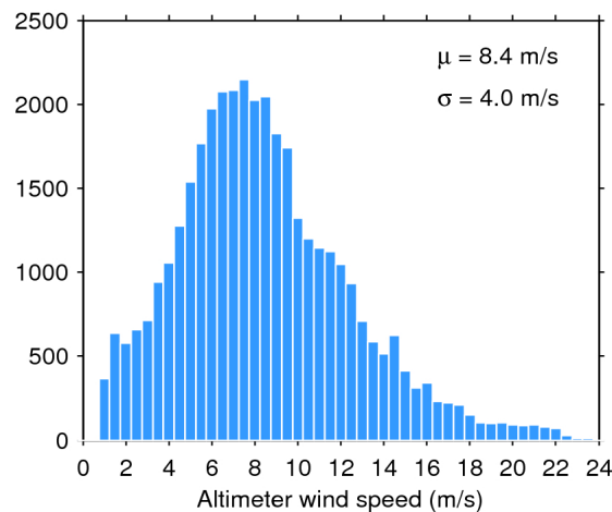
Figure 35. Histogram of science-valid wind over oceans and lakes for 16/12/2016. The mean ( \mu ) and standard deviation ( \sigma ) are also shown. Note that values larger than 24 m/s are excluded from the histogram for the sake of readability but not from the computation of \mu and \sigma .
