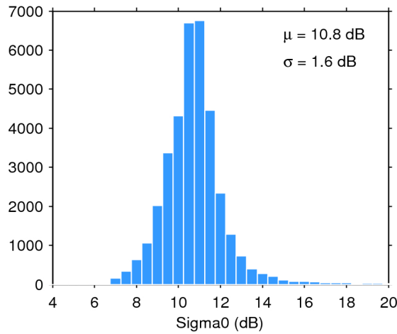
Figure 28. Histogram of science-valid sigma0 over oceans and lakes for 16/12/2016. The mean ( \mu ) and standard deviation ( \sigma ) are also shown. Note that values outside [4 20] dB are excluded from the histogram for the sake of readability but not from the computation of \mu and \sigma .
