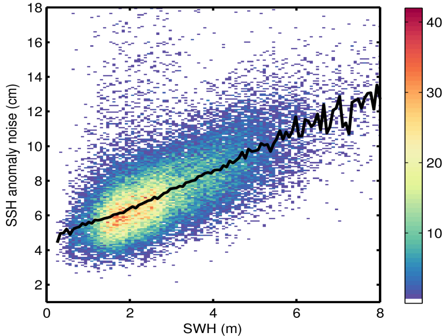
Figure 9. 2D histogram showing flag-valid SSH anomaly noise as a function of SWH for 16/12/2016. The black line denotes the median SSH anomaly noise as a function of SWH.
