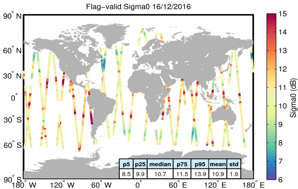
Figure 23. Geographical distribution of flag-valid sigma0 data over oceans and lakes for 16/12/2016. The statistical values shown in the table refer to the sigma0 in dB and are calculated over all measurements shown in the figure.
