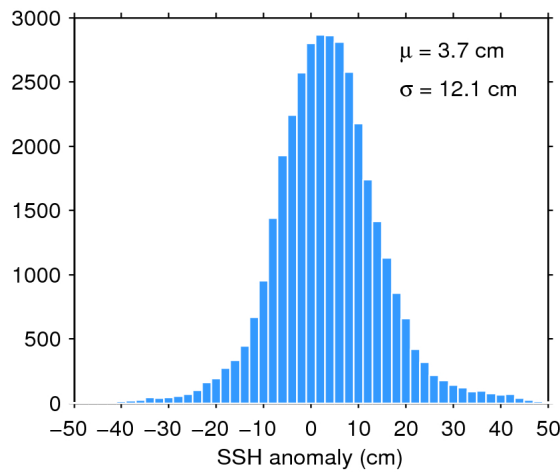
Figure 11. Histogram of science-valid SSH anomaly over oceans and lakes for 16/12/2016. The mean ( \mu ) and standard deviation ( \sigma ) are also shown. Note that values outside [-50 50] cm are excluded from the histogram for the sake of readability but not from the computation of \mu and \sigma .
