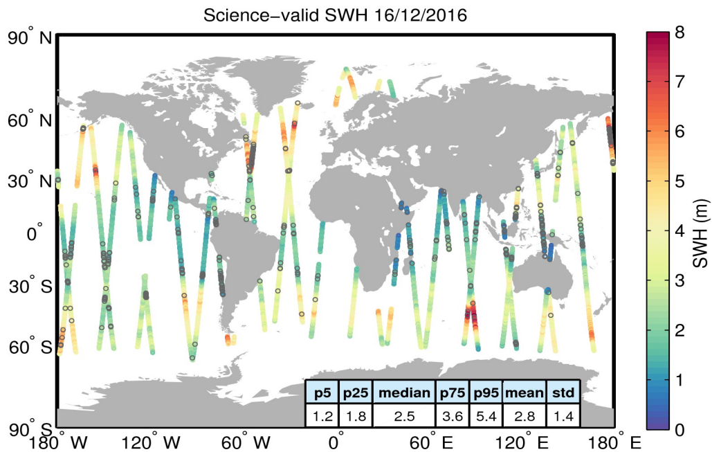
Figure 19. Geographical distribution of science-valid SWH data over oceans and lakes for 16/12/2016. The statistical values shown in the table refer to the SWH in m and are calculated over all measurements shown in the figure. Gray circles denote records that have been rejected based on the editing criteria described in Table 3.
