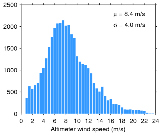
Figure 33. Histogram of flag-valid wind over oceans and lakes for 16/12/2016. The mean ( \mu ) and standard deviation ( \sigma ) are also shown. Note that values larger than 24 m/s are excluded from the histogram for the sake of readability but not from the computation of \mu and \sigma .
