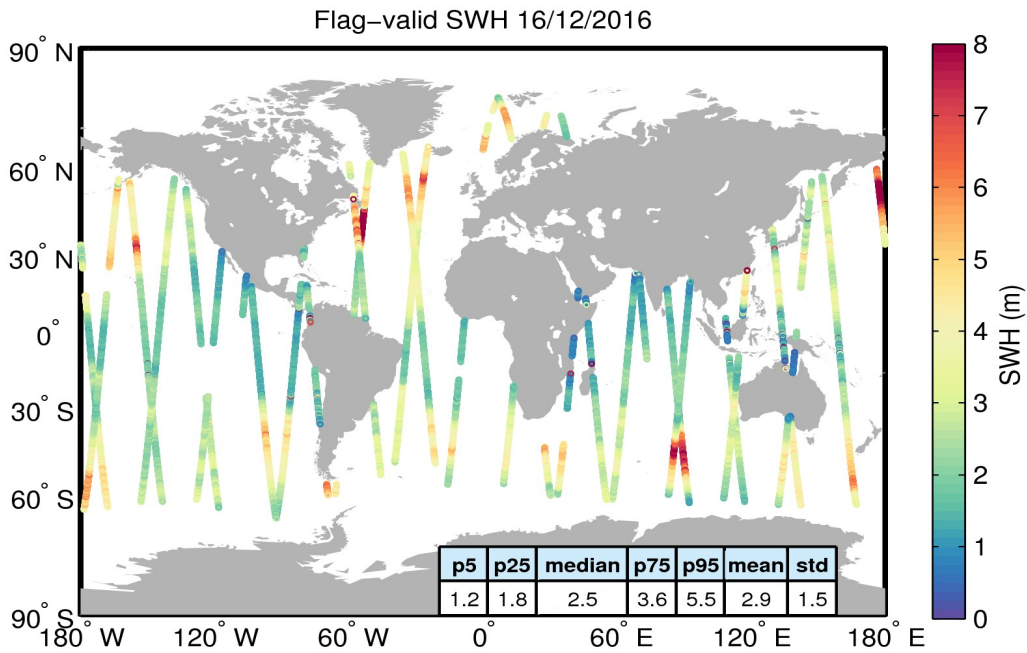
Figure 15. Geographical distribution of flag-valid SWH data over oceans and lakes for 16/12/2016. The statistical values shown in the table refer to the SWH in m and are calculated over all measurements shown in the figure.
