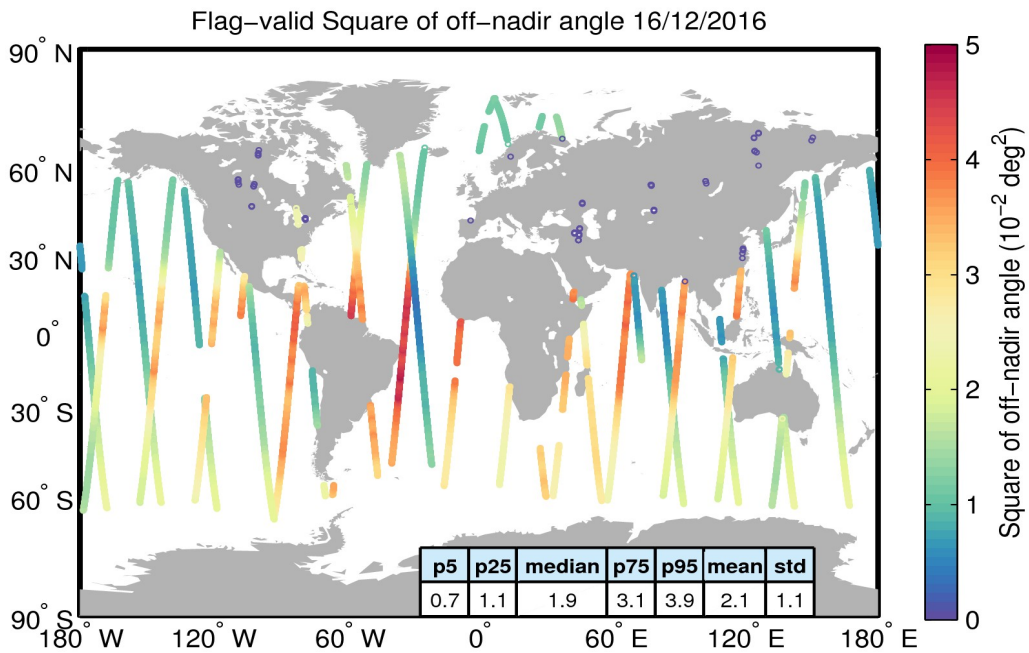
Figure 37. Geographical distribution of flag-valid mispointing data over oceans and lakes for 16/12/2016. The statistical values shown in the table refer to the mispointing in 10^{-2} deg 2 and are calculated over all measurements shown in the figure.
