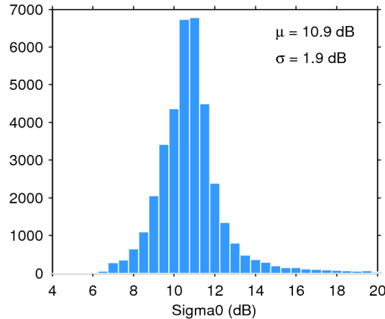
Figure 25. Histogram of flag-valid sigma0 over oceans and lakes for 16/12/2016. The mean ( \mu ) and standard deviation ( \sigma ) are also shown. Note that values outside [4 20] dB are excluded from the histogram for the sake of readability but not from the computation of \mu and \sigma .
