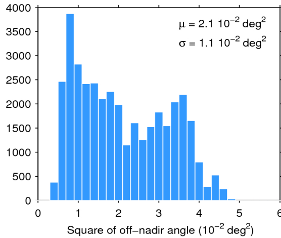
Figure 39. Histogram of flag-valid mispointing over oceans and lakes for 16/12/2016. The mean ( \mu ) and standard deviation ( \sigma ) are also shown. Note that values larger than 6 \cdot 10^{-2} \text{ deg}^2 are excluded from the histogram for the sake of readability but not from the computation of \mu and \sigma .
