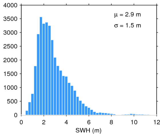
Figure 17. Histogram of flag-valid SWH over oceans and lakes for 16/12/2016. The mean ( \mu ) and standard deviation ( \sigma ) are also shown. Note that values larger than 12 m are excluded from the histogram for the sake of readability but not from the computation of \mu and \sigma .
