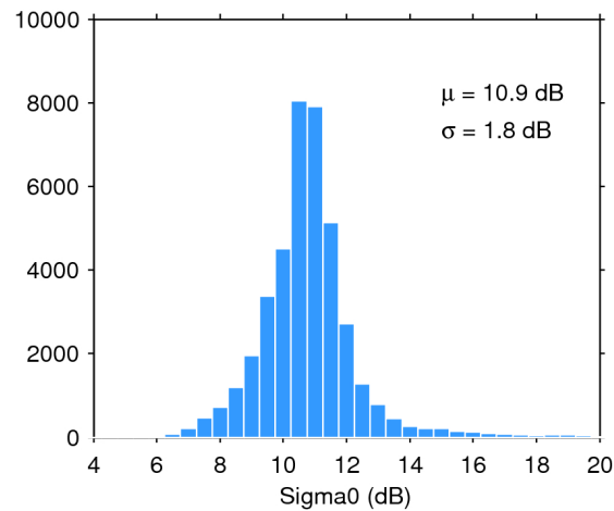
Figure 25. Histogram of flag-valid sigma0 over oceans and lakes for 14/12/2016. The mean ( \mu ) and standard deviation ( \sigma ) are also shown. Note that values outside [4 20] dB are excluded from the histogram for the sake of readability but not from the computation of \mu and \sigma .
