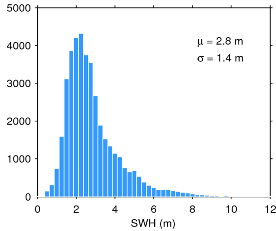
Figure 17. Histogram of flag-valid SWH over oceans and lakes for 14/12/2016. The mean ( \mu ) and standard deviation ( \sigma ) are also shown. Note that values larger than 12 m are excluded from the histogram for the sake of readability but not from the computation of \mu and \sigma .
