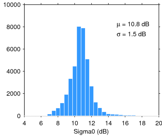
Figure 28. Histogram of science-valid sigma0 over oceans and lakes for 14/12/2016. The mean ( \mu ) and standard deviation ( \sigma ) are also shown. Note that values outside [4 20] dB are excluded from the histogram for the sake of readability but not from the computation of \mu and \sigma .
