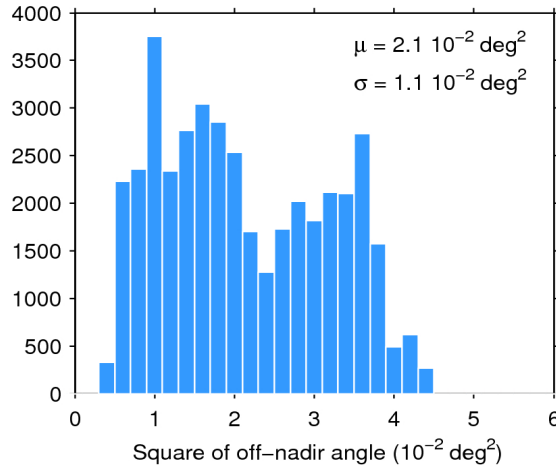
Figure 39. Histogram of flag-valid mispointing over oceans and lakes for 14/12/2016. The mean ( \mu ) and standard deviation ( \sigma ) are also shown. Note that values larger than 6 \cdot 10^{-2} \text{ deg}^2 are excluded from the histogram for the sake of readability but not from the computation of \mu and \sigma .
