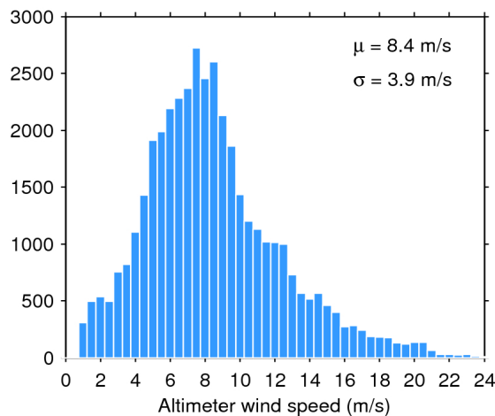
Figure 35. Histogram of science-valid wind over oceans and lakes for 14/12/2016. The mean ( \mu ) and standard deviation ( \sigma ) are also shown. Note that values larger than 24 m/s are excluded from the histogram for the sake of readability but not from the computation of \mu and \sigma .
