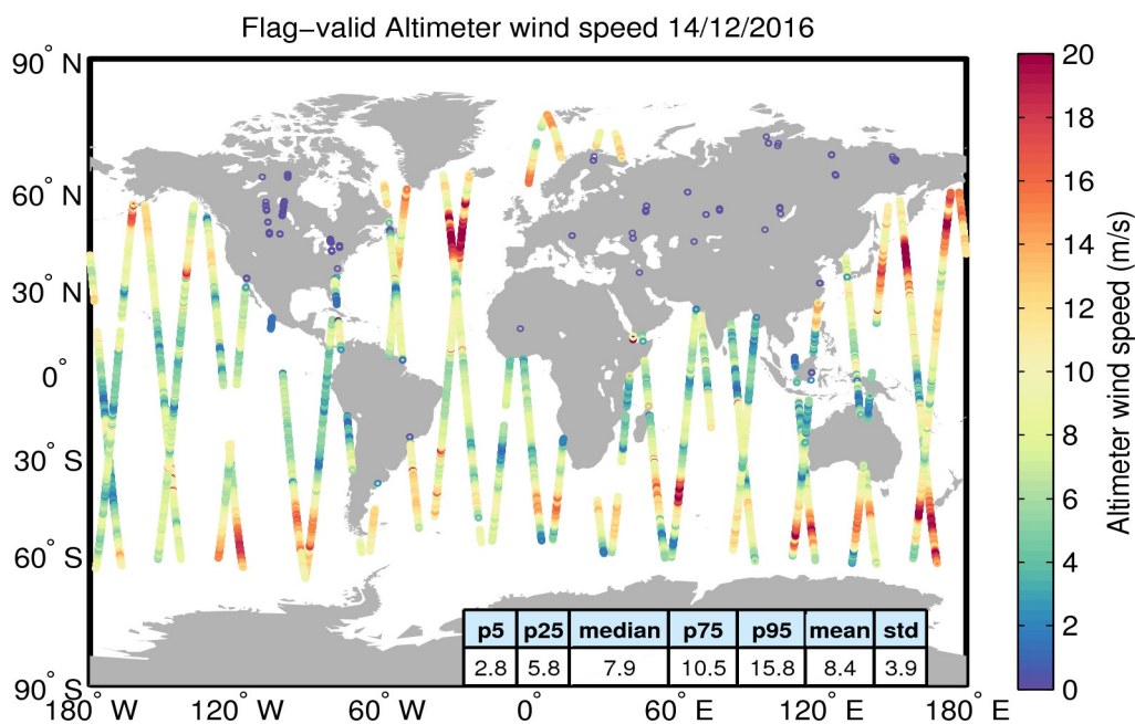
Figure 31. Geographical distribution of flag-valid wind data over oceans and lakes for 14/12/2016. The statistical values shown in the table refer to the wind in m/s and are calculated over all measurements shown in the figure.
