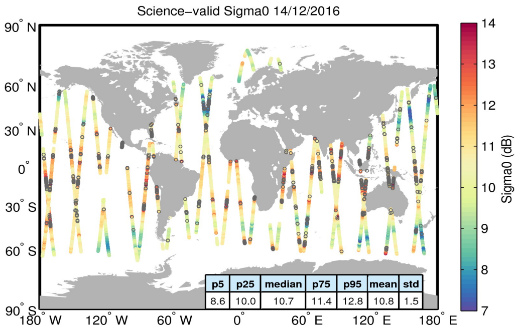
Figure 27. Geographical distribution of science-valid sigma0 data over oceans and lakes for 14/12/2016. The statistical values shown in the table refer to the sigma0 in dB and are calculated over all measurements shown in the figure. Gray circles denote records that have been rejected based on the editing criteria described in Table 4.
