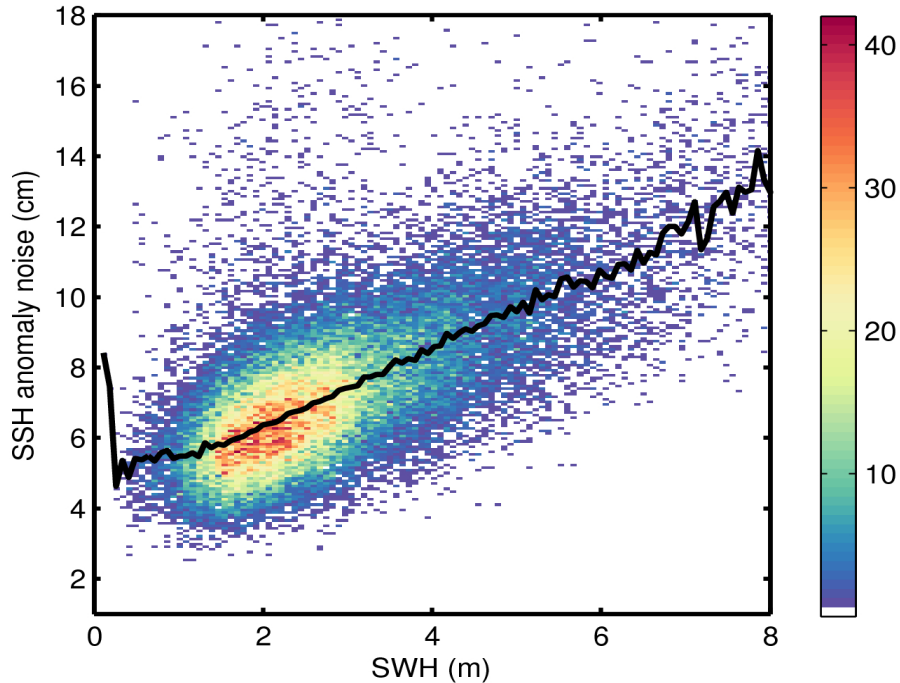
Figure 9. 2D histogram showing flag-valid SSH anomaly noise as a function of SWH for 14/12/2016. The black line denotes the median SSH anomaly noise as a function of SWH.
