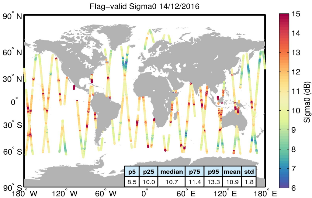
Figure 23. Geographical distribution of flag-valid sigma0 data over oceans and lakes for 14/12/2016. The statistical values shown in the table refer to the sigma0 in dB and are calculated over all measurements shown in the figure.
