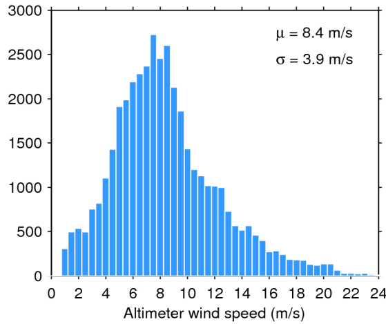
Figure 33. Histogram of flag-valid wind over oceans and lakes for 14/12/2016. The mean ( \mu ) and standard deviation ( \sigma ) are also shown. Note that values larger than 24 m/s are excluded from the histogram for the sake of readability but not from the computation of \mu and \sigma .
