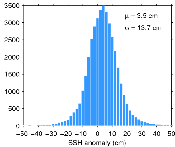
Figure 7. Histogram of flag-valid SSH anomaly over oceans and lakes for 14/12/2016. The mean ( \mu ) and standard deviation ( \sigma ) are also shown. Note that values outside [-50\ 50] cm are excluded from the histogram for the sake of readability but not from the computation of \mu and \sigma .
