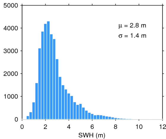
Figure 20. Histogram of science-valid SWH over oceans and lakes for 14/12/2016. The mean ( \mu ) and standard deviation ( \sigma ) are also shown. Note that values larger than 12 m are excluded from the histogram for the sake of readability but not from the computation of \mu and \sigma .
