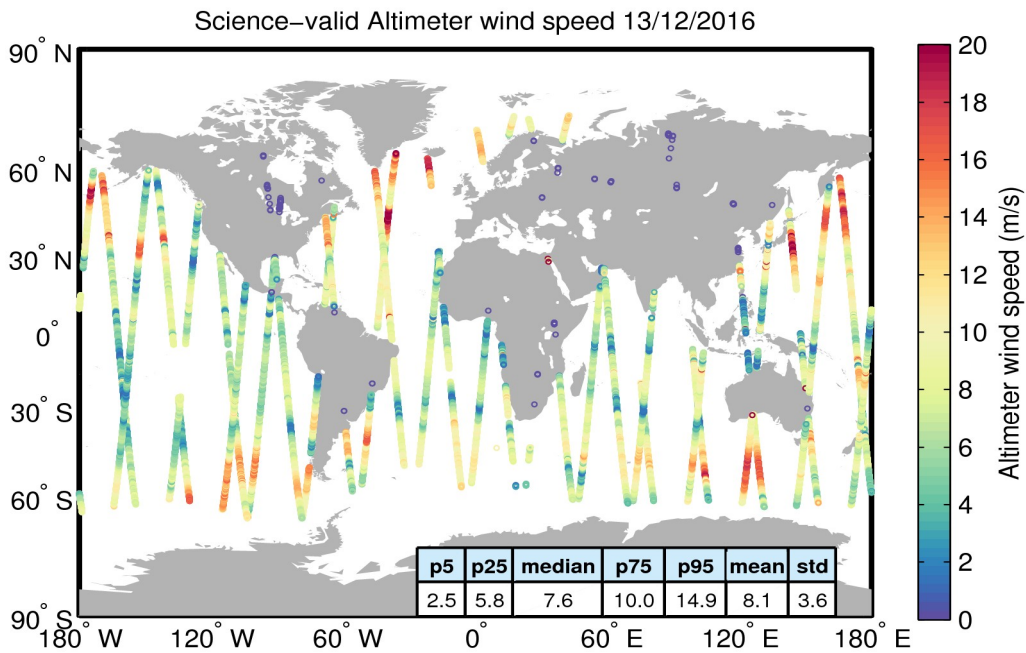
Figure 34. Geographical distribution of science-valid wind data over oceans and lakes for 13/12/2016. The statistical values shown in the table refer to the wind in m/s and are calculated over all measurements shown in the figure. Gray circles denote records that have been rejected based on the editing criteria described in Table 5.
