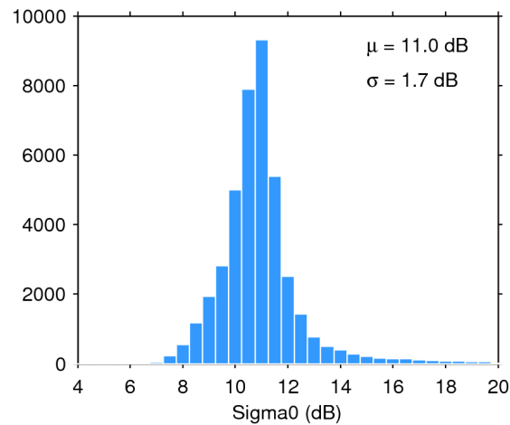
Figure 25. Histogram of flag-valid sigma0 over oceans and lakes for 13/12/2016. The mean ( \mu ) and standard deviation ( \sigma ) are also shown. Note that values outside [4 20] dB are excluded from the histogram for the sake of readability but not from the computation of \mu and \sigma .
