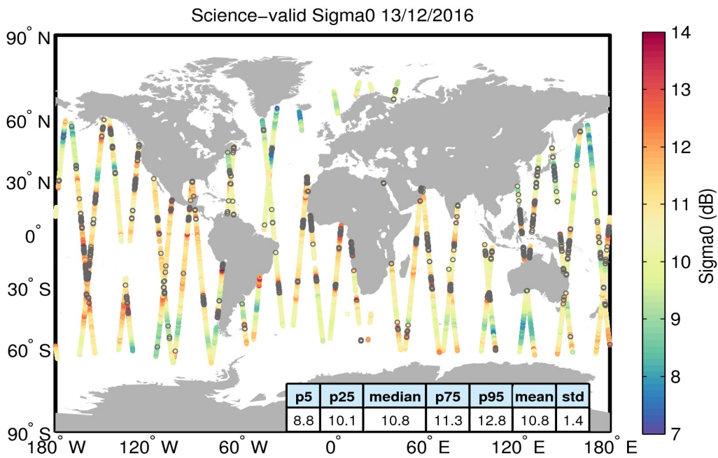
Figure 27. Geographical distribution of science-valid sigma0 data over oceans and lakes for 13/12/2016. The statistical values shown in the table refer to the sigma0 in dB and are calculated over all measurements shown in the figure. Gray circles denote records that have been rejected based on the editing criteria described in Table 4.
