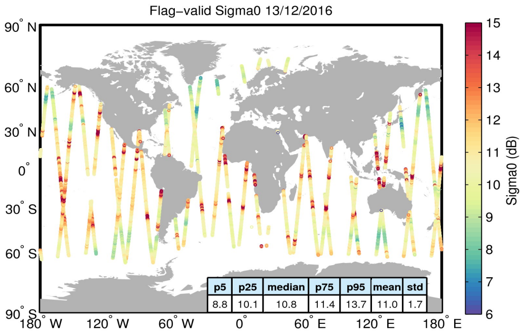
Figure 23. Geographical distribution of flag-valid sigma0 data over oceans and lakes for 13/12/2016. The statistical values shown in the table refer to the sigma0 in dB and are calculated over all measurements shown in the figure.
