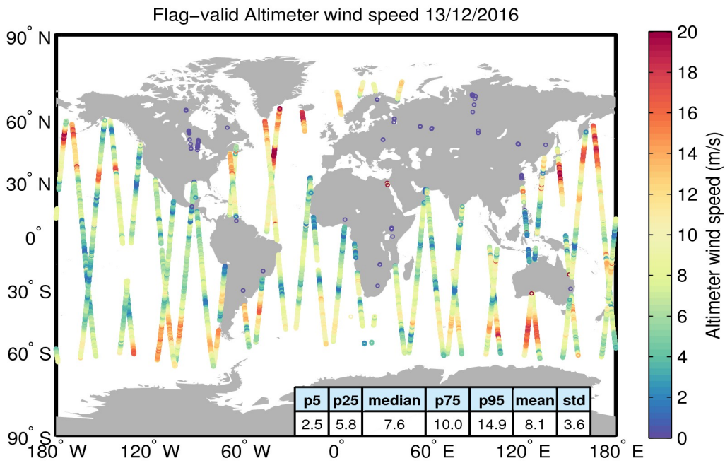
Figure 31. Geographical distribution of flag-valid wind data over oceans and lakes for 13/12/2016. The statistical values shown in the table refer to the wind in m/s and are calculated over all measurements shown in the figure.
