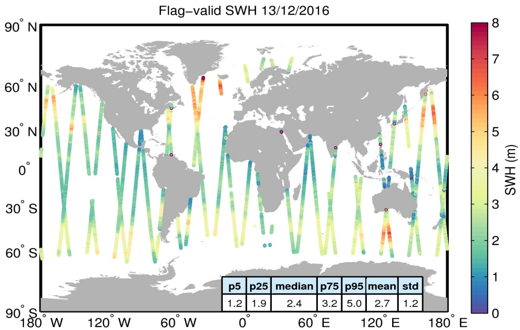
Figure 15. Geographical distribution of flag-valid SWH data over oceans and lakes for 13/12/2016. The statistical values shown in the table refer to the SWH in m and are calculated over all measurements shown in the figure.
