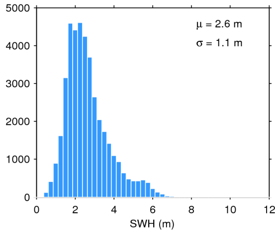
Figure 20. Histogram of science-valid SWH over oceans and lakes for 13/12/2016. The mean ( \mu ) and standard deviation ( \sigma ) are also shown. Note that values larger than 12 m are excluded from the histogram for the sake of readability but not from the computation of \mu and \sigma .
