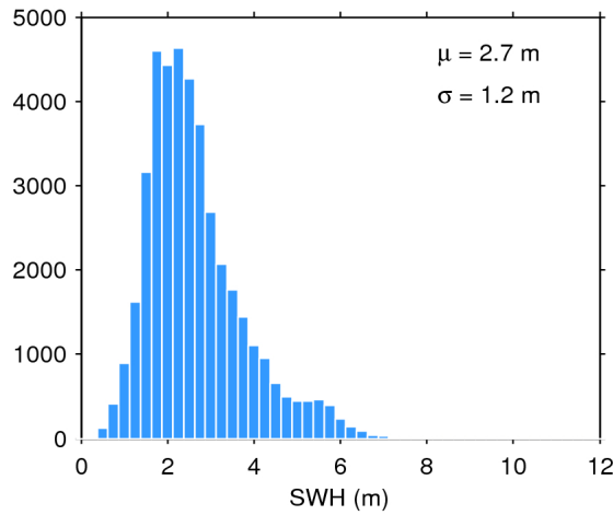
Figure 17. Histogram of flag-valid SWH over oceans and lakes for 13/12/2016. The mean ( \mu ) and standard deviation ( \sigma ) are also shown. Note that values larger than 12 m are excluded from the histogram for the sake of readability but not from the computation of \mu and \sigma .
