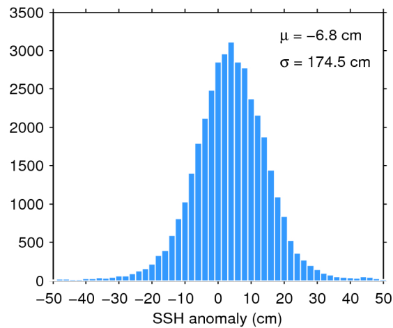
Figure 7. Histogram of flag-valid SSH anomaly over oceans and lakes for 13/12/2016. The mean ( \mu ) and standard deviation ( \sigma ) are also shown. Note that values outside [-50 50] cm are excluded from the histogram for the sake of readability but not from the computation of \mu and \sigma .
