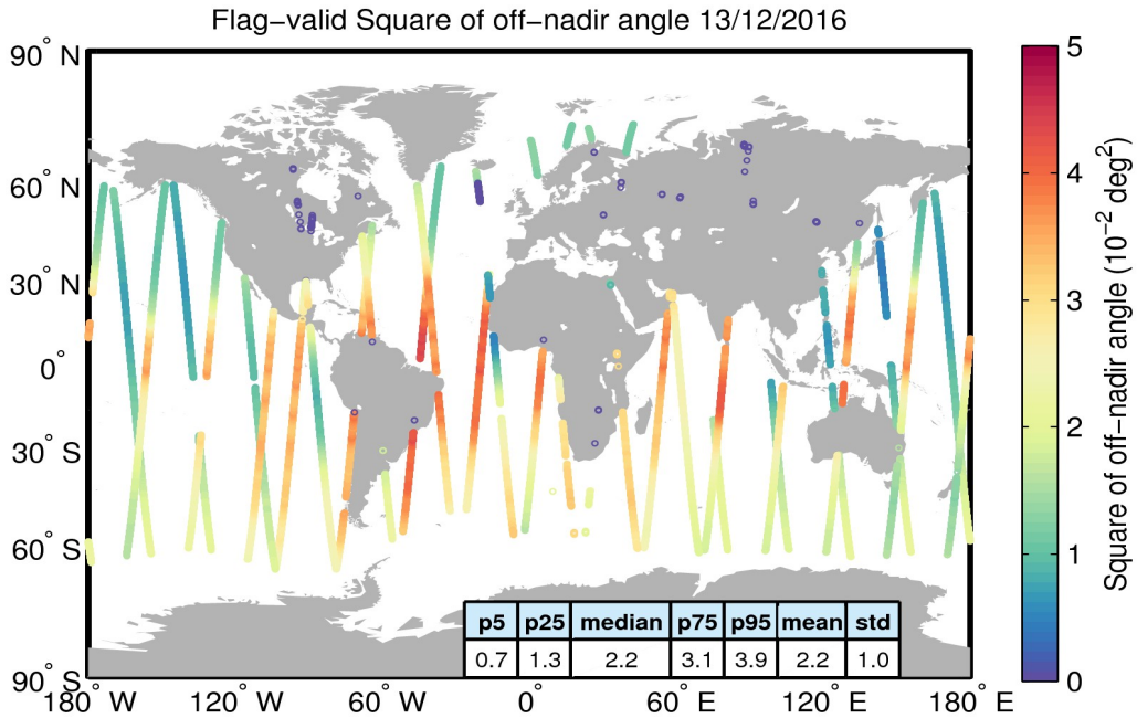
Figure 37. Geographical distribution of flag-valid mispointing data over oceans and lakes for 13/12/2016. The statistical values shown in the table refer to the mispointing in 10^{-2} deg 2 and are calculated over all measurements shown in the figure.
