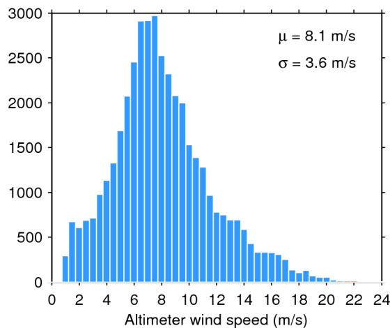
Figure 35. Histogram of science-valid wind over oceans and lakes for 13/12/2016. The mean ( \mu ) and standard deviation ( \sigma ) are also shown. Note that values larger than 24 m/s are excluded from the histogram for the sake of readability but not from the computation of \mu and \sigma .
