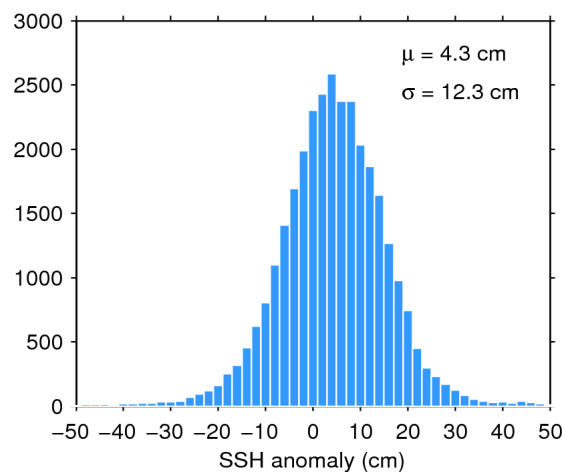
Figure 11. Histogram of science-valid SSH anomaly over oceans and lakes for 13/12/2016. The mean ( \mu ) and standard deviation ( \sigma ) are also shown. Note that values outside [-50 50] cm are excluded from the histogram for the sake of readability but not from the computation of \mu and \sigma .
