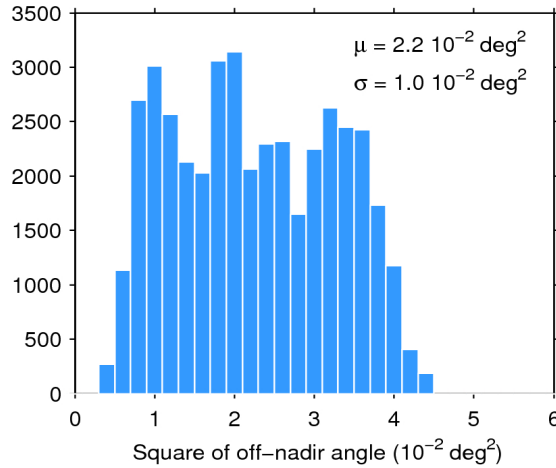
Figure 39. Histogram of flag-valid mispointing over oceans and lakes for 13/12/2016. The mean ( \mu ) and standard deviation ( \sigma ) are also shown. Note that values larger than 6 \cdot 10^{-2} \text{ deg}^2 are excluded from the histogram for the sake of readability but not from the computation of \mu and \sigma .
