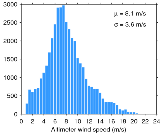
Figure 33. Histogram of flag-valid wind over oceans and lakes for 13/12/2016. The mean ( \mu ) and standard deviation ( \sigma ) are also shown. Note that values larger than 24 m/s are excluded from the histogram for the sake of readability but not from the computation of \mu and \sigma .
