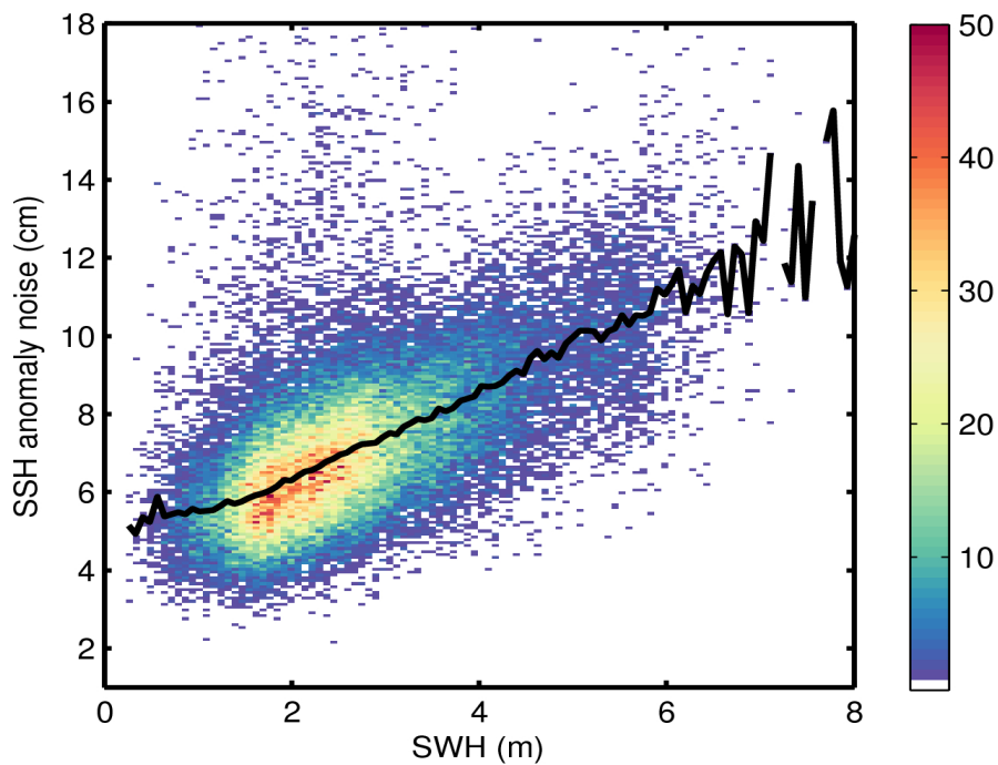
Figure 9. 2D histogram showing flag-valid SSH anomaly noise as a function of SWH for 13/12/2016. The black line denotes the median SSH anomaly noise as a function of SWH.
