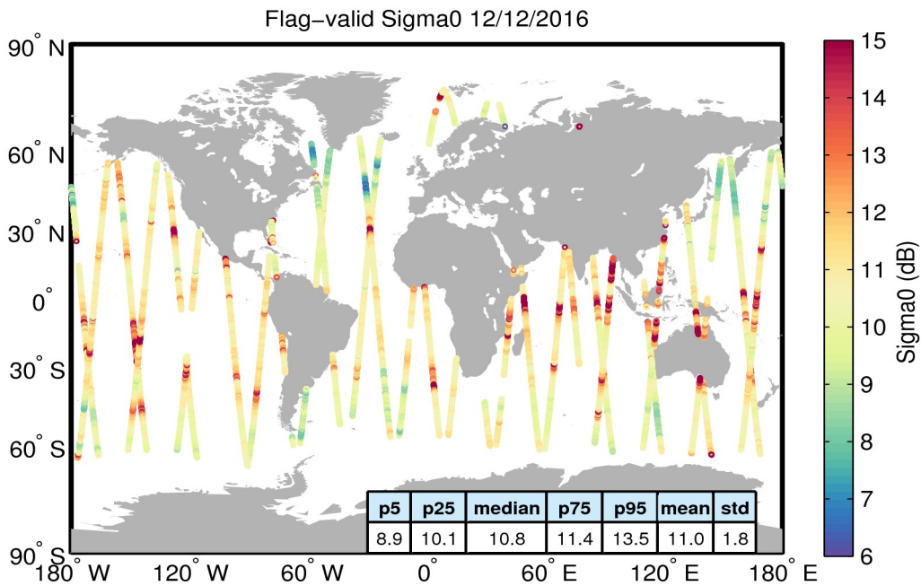
Figure 23. Geographical distribution of flag-valid sigma0 data over oceans and lakes for 12/12/2016. The statistical values shown in the table refer to the sigma0 in dB and are calculated over all measurements shown in the figure.
