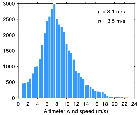
Figure 33. Histogram of flag-valid wind over oceans and lakes for 12/12/2016. The mean ( \mu ) and standard deviation ( \sigma ) are also shown. Note that values larger than 24 m/s are excluded from the histogram for the sake of readability but not from the computation of \mu and \sigma .
