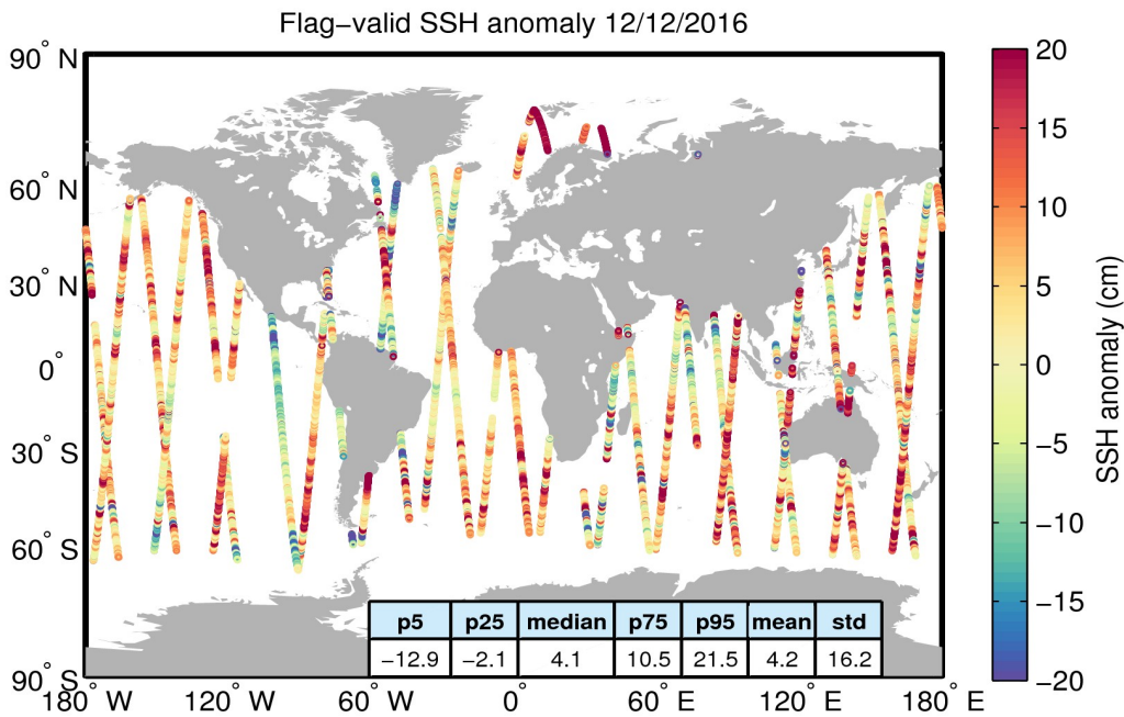
Figure 5. Geographical distribution of flag-valid 1-Hz SSH anomaly data over oceans and lakes for 12/12/2016. The statistical values shown in the table refer to the SSH anomaly in cm and are calculated over all measurements shown in the figure.
