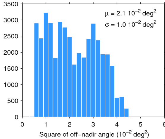
Figure 39. Histogram of flag-valid mispointing over oceans and lakes for 12/12/2016. The mean ( \mu ) and standard deviation ( \sigma ) are also shown. Note that values larger than 6 \cdot 10^{-2} \text{ deg}^2 are excluded from the histogram for the sake of readability but not from the computation of \mu and \sigma .
