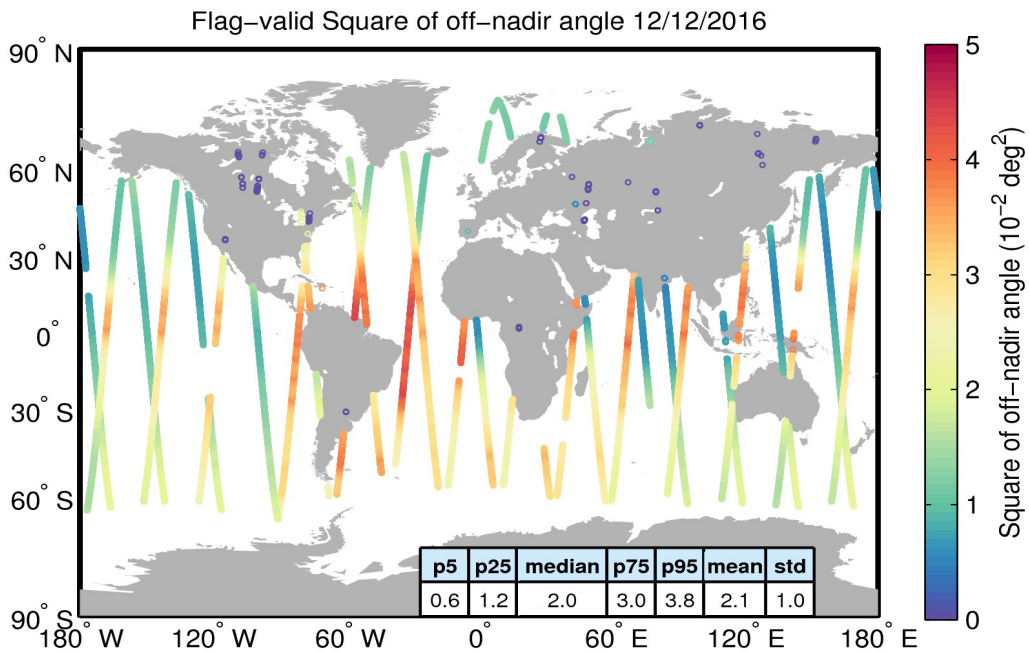
Figure 37. Geographical distribution of flag-valid mispointing data over oceans and lakes for 12/12/2016. The statistical values shown in the table refer to the mispointing in 10^{-2} deg 2 and are calculated over all measurements shown in the figure.
