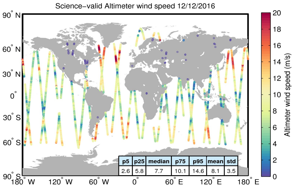
Figure 34. Geographical distribution of science-valid wind data over oceans and lakes for 12/12/2016. The statistical values shown in the table refer to the wind in m/s and are calculated over all measurements shown in the figure. Gray circles denote records that have been rejected based on the editing criteria described in Table 5.
