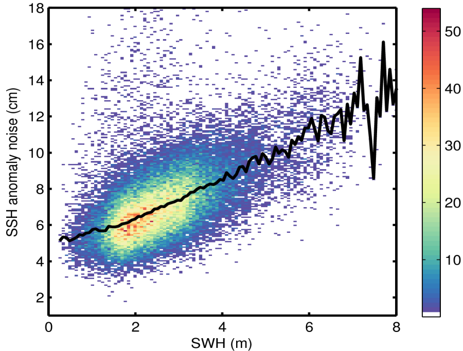
Figure 9. 2D histogram showing flag-valid SSH anomaly noise as a function of SWH for 12/12/2016. The black line denotes the median SSH anomaly noise as a function of SWH.
