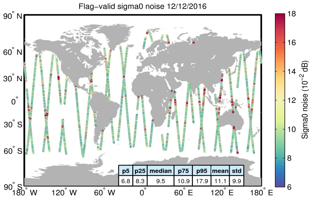
Figure 26. Geographical distribution of flag-valid 20-Hz sigma0 measurement noise over oceans and lakes for 12/12/2016. The statistical values shown in the table refer to the sigma0 noise and are calculated over all measurements shown in the figure.
