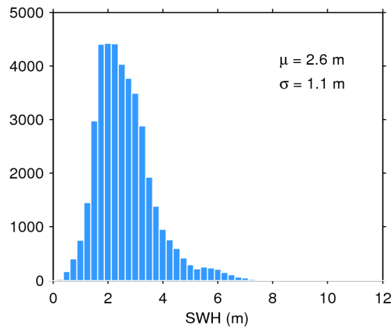
Figure 20. Histogram of science-valid SWH over oceans and lakes for 12/12/2016. The mean ( \mu ) and standard deviation ( \sigma ) are also shown. Note that values larger than 12 m are excluded from the histogram for the sake of readability but not from the computation of \mu and \sigma .
