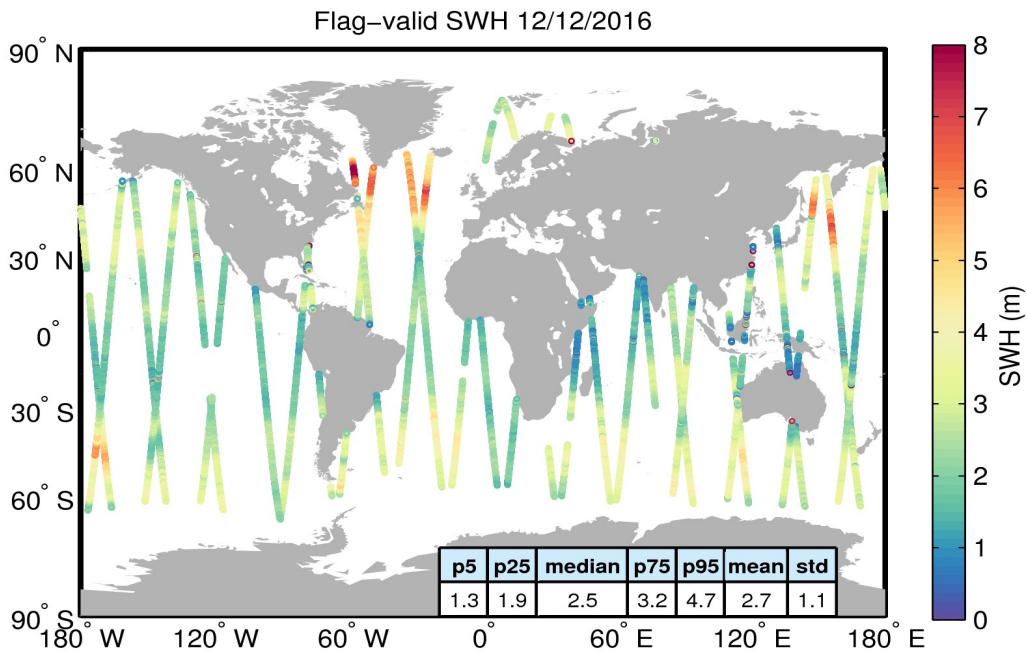
Figure 15. Geographical distribution of flag-valid SWH data over oceans and lakes for 12/12/2016. The statistical values shown in the table refer to the SWH in m and are calculated over all measurements shown in the figure.
