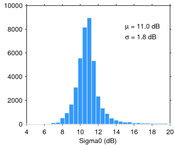
Figure 25. Histogram of flag-valid sigma0 over oceans and lakes for 12/12/2016. The mean ( \mu ) and standard deviation ( \sigma ) are also shown. Note that values outside [4 20] dB are excluded from the histogram for the sake of readability but not from the computation of \mu and \sigma .
