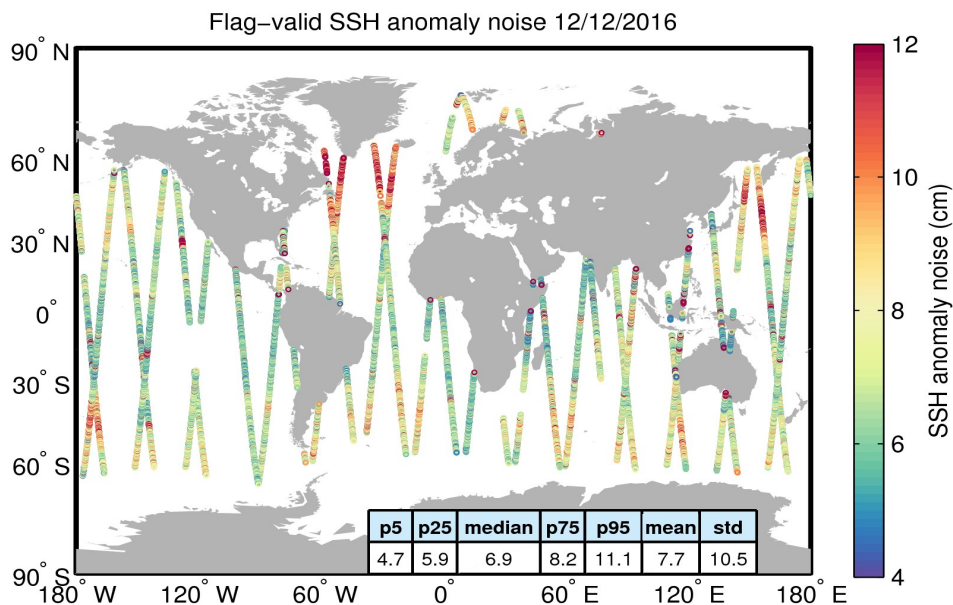
Figure 8. Geographical distribution of flag-valid 20-Hz SSH anomaly measurement noise over oceans and lakes for 12/12/2016. The statistical values shown in the table refer to the SSH anomaly noise and are calculated over all measurements shown in the figure.
