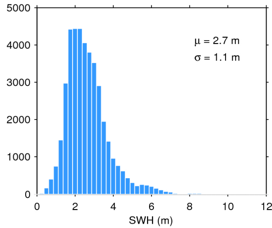
Figure 17. Histogram of flag-valid SWH over oceans and lakes for 12/12/2016. The mean ( \mu ) and standard deviation ( \sigma ) are also shown. Note that values larger than 12 m are excluded from the histogram for the sake of readability but not from the computation of \mu and \sigma .
