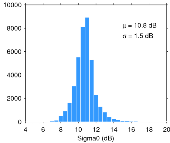
Figure 28. Histogram of science-valid sigma0 over oceans and lakes for 12/12/2016. The mean ( \mu ) and standard deviation ( \sigma ) are also shown. Note that values outside [4 20] dB are excluded from the histogram for the sake of readability but not from the computation of \mu and \sigma .
