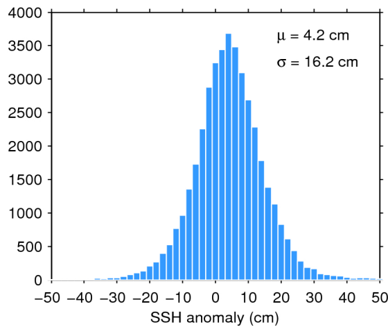
Figure 7. Histogram of flag-valid SSH anomaly over oceans and lakes for 12/12/2016. The mean ( \mu ) and standard deviation ( \sigma ) are also shown. Note that values outside [-50 50] cm are excluded from the histogram for the sake of readability but not from the computation of \mu and \sigma .
