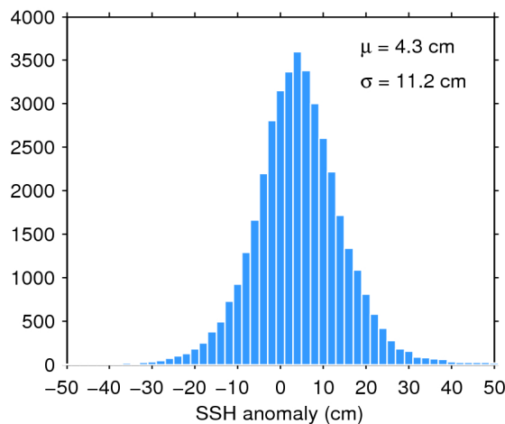
Figure 11. Histogram of science-valid SSH anomaly over oceans and lakes for 12/12/2016. The mean ( \mu ) and standard deviation ( \sigma ) are also shown. Note that values outside [-50 50] cm are excluded from the histogram for the sake of readability but not from the computation of \mu and \sigma .
