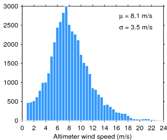
Figure 35. Histogram of science-valid wind over oceans and lakes for 12/12/2016. The mean ( \mu ) and standard deviation ( \sigma ) are also shown. Note that values larger than 24 m/s are excluded from the histogram for the sake of readability but not from the computation of \mu and \sigma .
