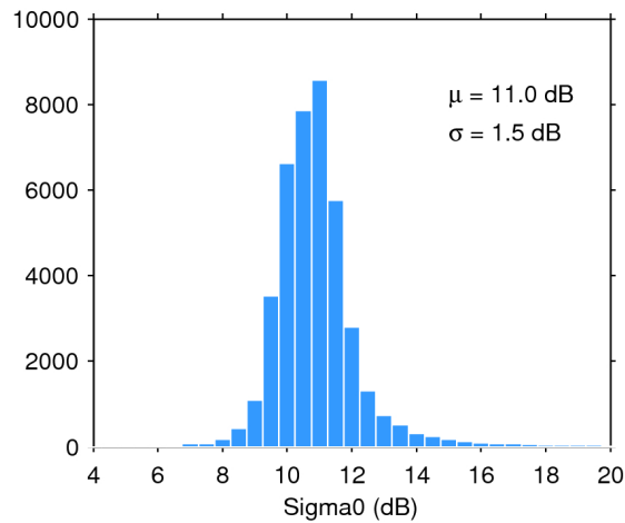
Figure 25. Histogram of flag-valid sigma0 over oceans and lakes for 11/12/2016. The mean ( \mu ) and standard deviation ( \sigma ) are also shown. Note that values outside [4 20] dB are excluded from the histogram for the sake of readability but not from the computation of \mu and \sigma .
