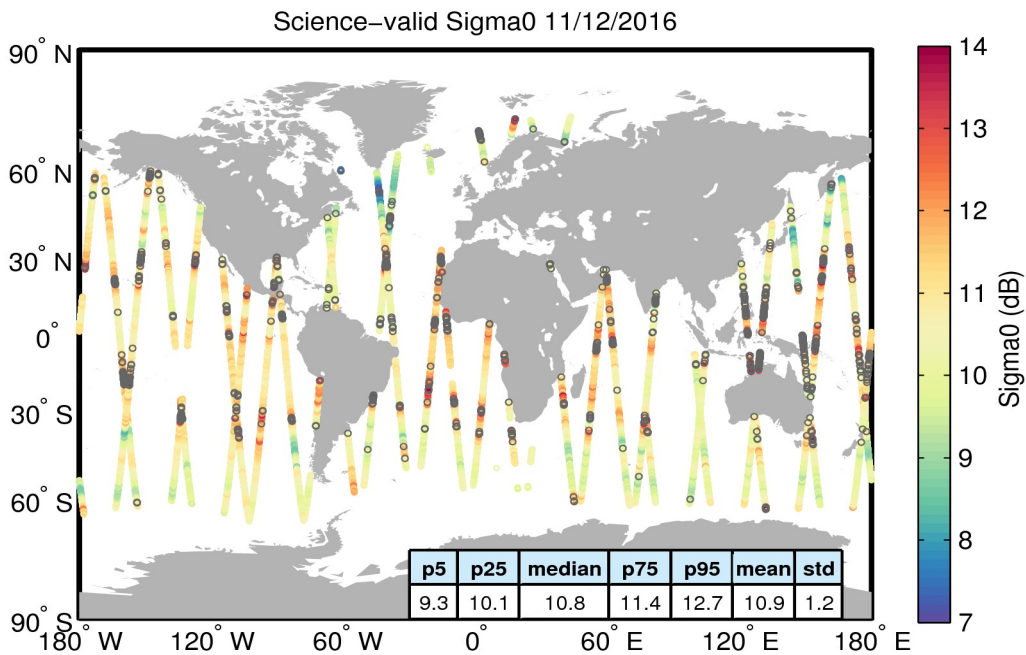
Figure 27. Geographical distribution of science-valid sigma0 data over oceans and lakes for 11/12/2016. The statistical values shown in the table refer to the sigma0 in dB and are calculated over all measurements shown in the figure. Gray circles denote records that have been rejected based on the editing criteria described in Table 4.
