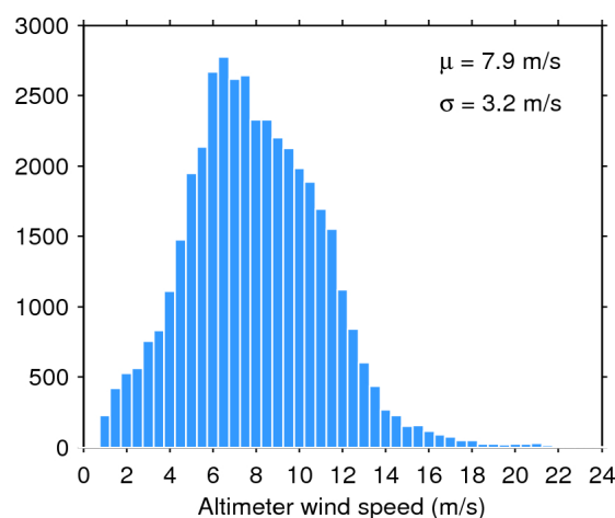
Figure 35. Histogram of science-valid wind over oceans and lakes for 11/12/2016. The mean ( \mu ) and standard deviation ( \sigma ) are also shown. Note that values larger than 24 m/s are excluded from the histogram for the sake of readability but not from the computation of \mu and \sigma .
