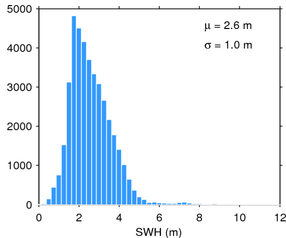
Figure 20. Histogram of science-valid SWH over oceans and lakes for 11/12/2016. The mean ( \mu ) and standard deviation ( \sigma ) are also shown. Note that values larger than 12 m are excluded from the histogram for the sake of readability but not from the computation of \mu and \sigma .
