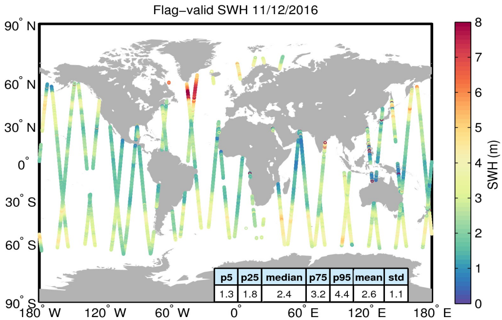
Figure 15. Geographical distribution of flag-valid SWH data over oceans and lakes for 11/12/2016. The statistical values shown in the table refer to the SWH in m and are calculated over all measurements shown in the figure.
