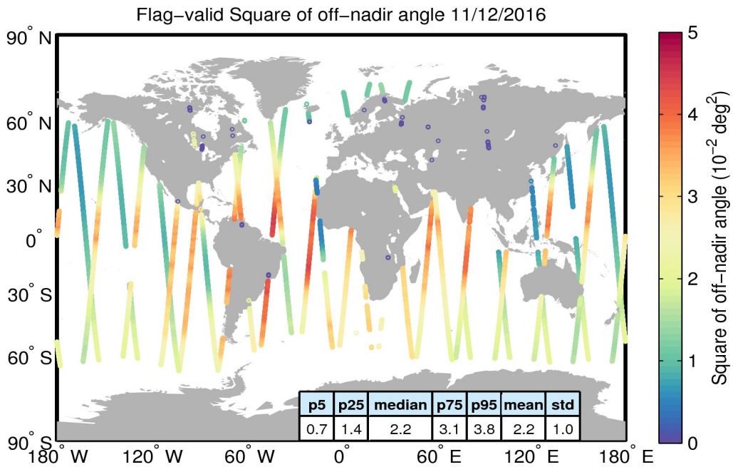
Figure 37. Geographical distribution of flag-valid mispointing data over oceans and lakes for 11/12/2016. The statistical values shown in the table refer to the mispointing in 10^{-2} deg 2 and are calculated over all measurements shown in the figure.
