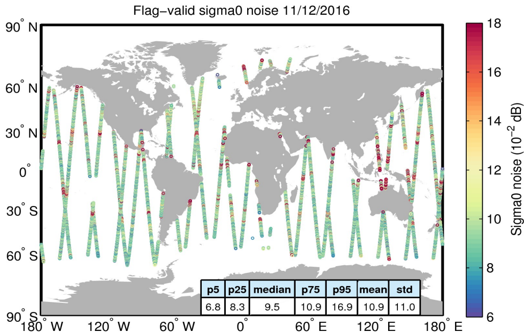
Figure 26. Geographical distribution of flag-valid 20-Hz sigma0 measurement noise over oceans and lakes for 11/12/2016. The statistical values shown in the table refer to the sigma0 noise and are calculated over all measurements shown in the figure.
