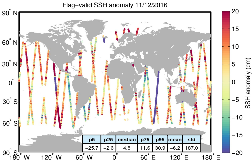
Figure 5. Geographical distribution of flag-valid 1-Hz SSH anomaly data over oceans and lakes for 11/12/2016. The statistical values shown in the table refer to the SSH anomaly in cm and are calculated over all measurements shown in the figure.
