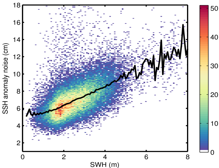
Figure 9. 2D histogram showing flag-valid SSH anomaly noise as a function of SWH for 11/12/2016. The black line denotes the median SSH anomaly noise as a function of SWH.
