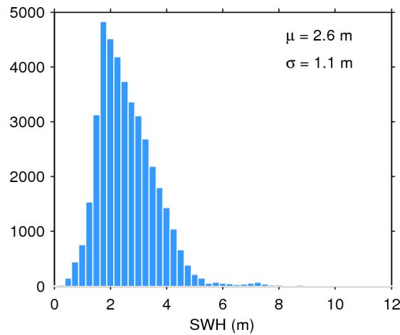
Figure 17. Histogram of flag-valid SWH over oceans and lakes for 11/12/2016. The mean ( \mu ) and standard deviation ( \sigma ) are also shown. Note that values larger than 12 m are excluded from the histogram for the sake of readability but not from the computation of \mu and \sigma .
