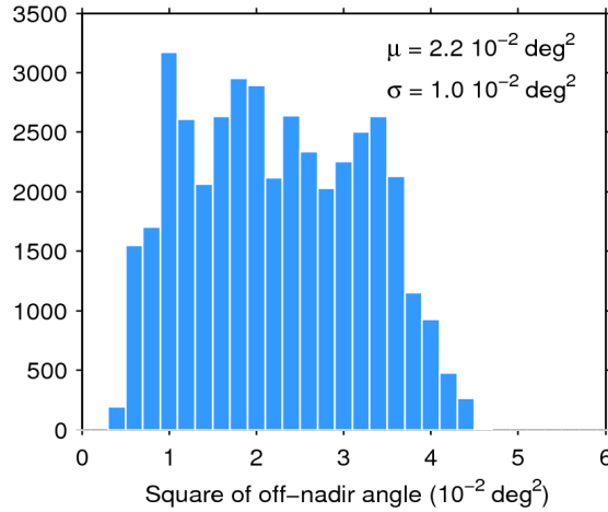
Figure 39. Histogram of flag-valid mispointing over oceans and lakes for 11/12/2016. The mean ( \mu ) and standard deviation ( \sigma ) are also shown. Note that values larger than 6 \cdot 10^{-2} \text{ deg}^2 are excluded from the histogram for the sake of readability but not from the computation of \mu and \sigma .
