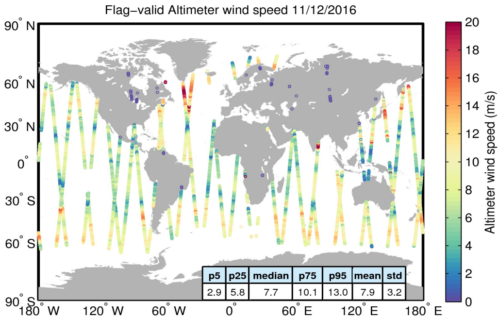
Figure 31. Geographical distribution of flag-valid wind data over oceans and lakes for 11/12/2016. The statistical values shown in the table refer to the wind in m/s and are calculated over all measurements shown in the figure.
