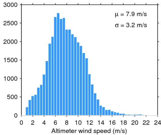
Figure 33. Histogram of flag-valid wind over oceans and lakes for 11/12/2016. The mean ( \mu ) and standard deviation ( \sigma ) are also shown. Note that values larger than 24 m/s are excluded from the histogram for the sake of readability but not from the computation of \mu and \sigma .
