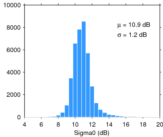
Figure 28. Histogram of science-valid sigma0 over oceans and lakes for 11/12/2016. The mean ( \mu ) and standard deviation ( \sigma ) are also shown. Note that values outside [4 20] dB are excluded from the histogram for the sake of readability but not from the computation of \mu and \sigma .
