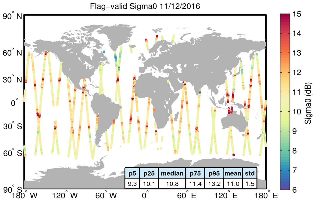
Figure 23. Geographical distribution of flag-valid sigma0 data over oceans and lakes for 11/12/2016. The statistical values shown in the table refer to the sigma0 in dB and are calculated over all measurements shown in the figure.
