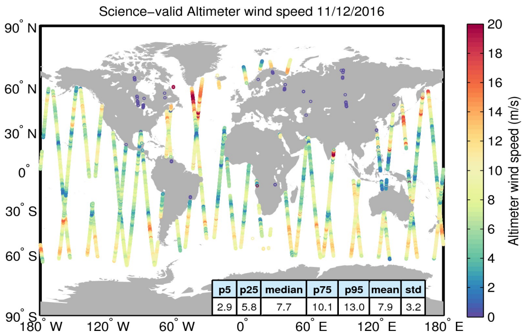
Figure 34. Geographical distribution of science-valid wind data over oceans and lakes for 11/12/2016. The statistical values shown in the table refer to the wind in m/s and are calculated over all measurements shown in the figure. Gray circles denote records that have been rejected based on the editing criteria described in Table 5.
