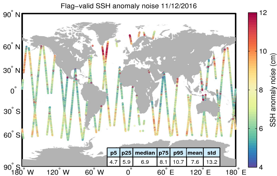
Figure 8. Geographical distribution of flag-valid 20-Hz SSH anomaly measurement noise over oceans and lakes for 11/12/2016. The statistical values shown in the table refer to the SSH anomaly noise and are calculated over all measurements shown in the figure.
