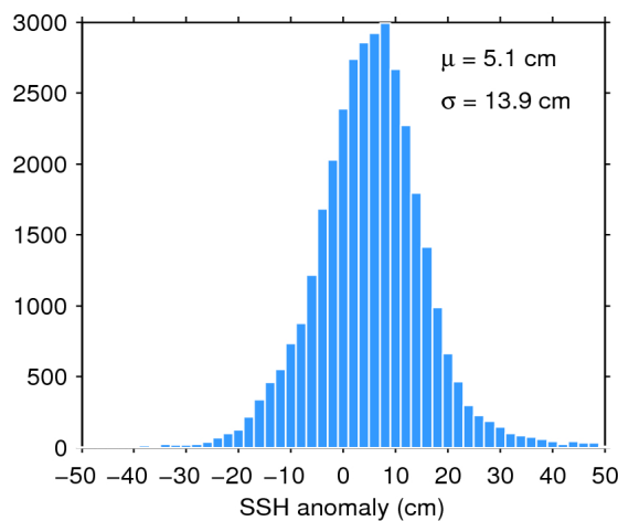
Figure 11. Histogram of science-valid SSH anomaly over oceans and lakes for 11/12/2016. The mean ( \mu ) and standard deviation ( \sigma ) are also shown. Note that values outside [-50 50] cm are excluded from the histogram for the sake of readability but not from the computation of \mu and \sigma .
