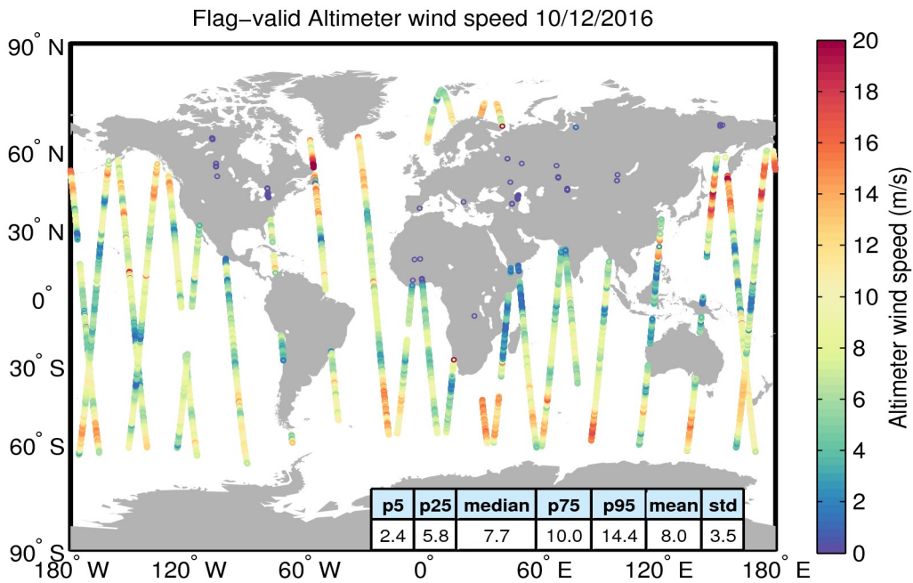
Figure 31. Geographical distribution of flag-valid wind data over oceans and lakes for 10/12/2016. The statistical values shown in the table refer to the wind in m/s and are calculated over all measurements shown in the figure.
