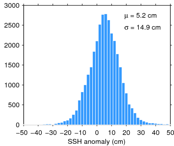
Figure 7. Histogram of flag-valid SSH anomaly over oceans and lakes for 10/12/2016. The mean ( \mu ) and standard deviation ( \sigma ) are also shown. Note that values outside [-50\ 50] cm are excluded from the histogram for the sake of readability but not from the computation of \mu and \sigma .
