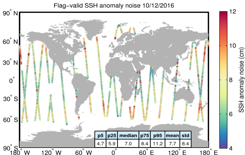
Figure 8. Geographical distribution of flag-valid 20-Hz SSH anomaly measurement noise over oceans and lakes for 10/12/2016. The statistical values shown in the table refer to the SSH anomaly noise and are calculated over all measurements shown in the figure.
