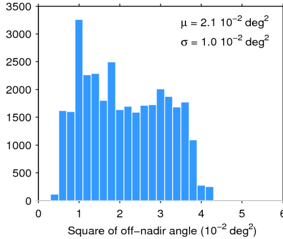
Figure 39. Histogram of flag-valid mispointing over oceans and lakes for 10/12/2016. The mean ( \mu ) and standard deviation ( \sigma ) are also shown. Note that values larger than 6 \cdot 10^{-2} \text{ deg}^2 are excluded from the histogram for the sake of readability but not from the computation of \mu and \sigma .
