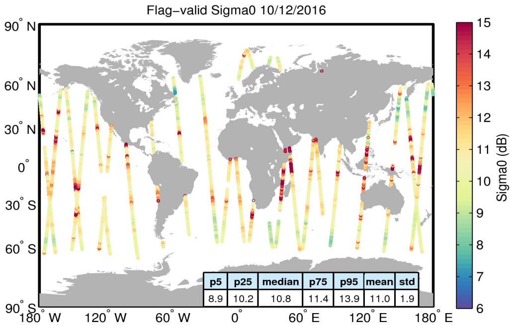
Figure 23. Geographical distribution of flag-valid sigma0 data over oceans and lakes for 10/12/2016. The statistical values shown in the table refer to the sigma0 in dB and are calculated over all measurements shown in the figure.
