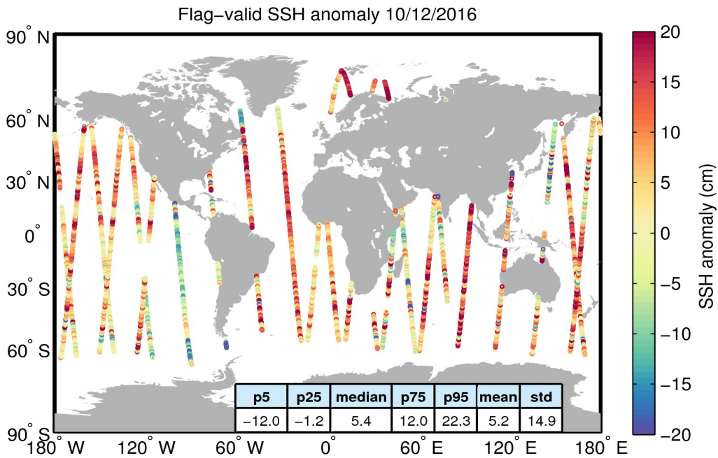
Figure 5. Geographical distribution of flag-valid 1-Hz SSH anomaly data over oceans and lakes for 10/12/2016. The statistical values shown in the table refer to the SSH anomaly in cm and are calculated over all measurements shown in the figure.
