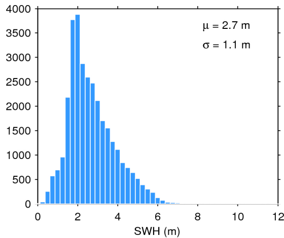
Figure 20. Histogram of science-valid SWH over oceans and lakes for 10/12/2016. The mean ( \mu ) and standard deviation ( \sigma ) are also shown. Note that values larger than 12 m are excluded from the histogram for the sake of readability but not from the computation of \mu and \sigma .
