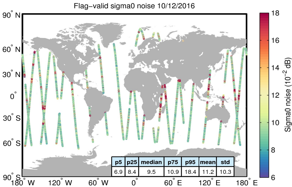
Figure 26. Geographical distribution of flag-valid 20-Hz sigma0 measurement noise over oceans and lakes for 10/12/2016. The statistical values shown in the table refer to the sigma0 noise and are calculated over all measurements shown in the figure.
