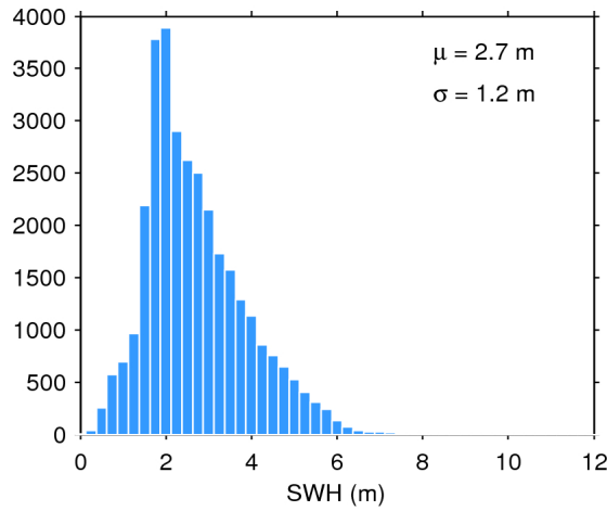
Figure 17. Histogram of flag-valid SWH over oceans and lakes for 10/12/2016. The mean ( \mu ) and standard deviation ( \sigma ) are also shown. Note that values larger than 12 m are excluded from the histogram for the sake of readability but not from the computation of \mu and \sigma .
