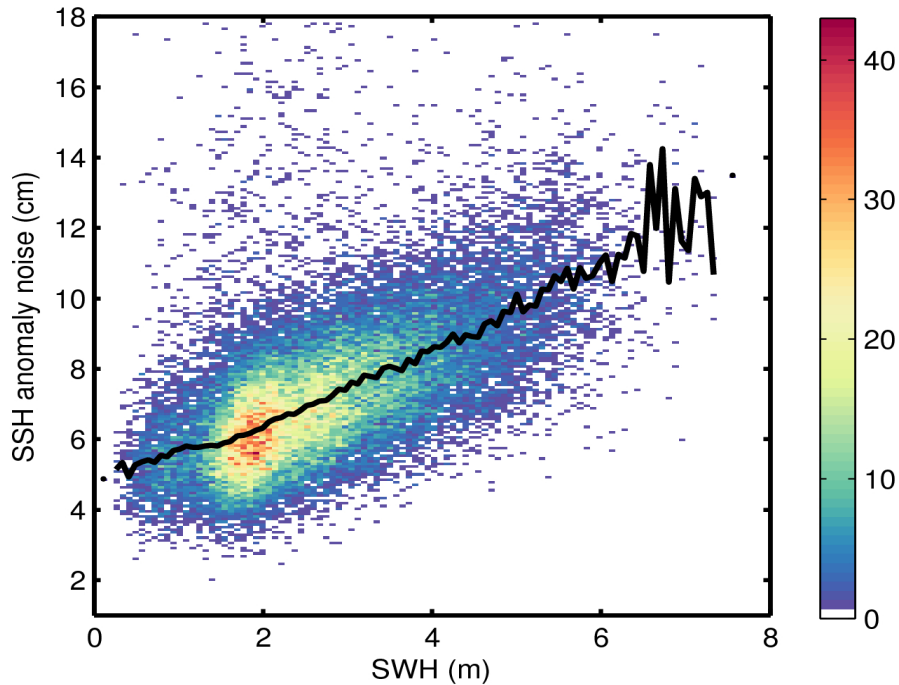
Figure 9. 2D histogram showing flag-valid SSH anomaly noise as a function of SWH for 10/12/2016. The black line denotes the median SSH anomaly noise as a function of SWH.
