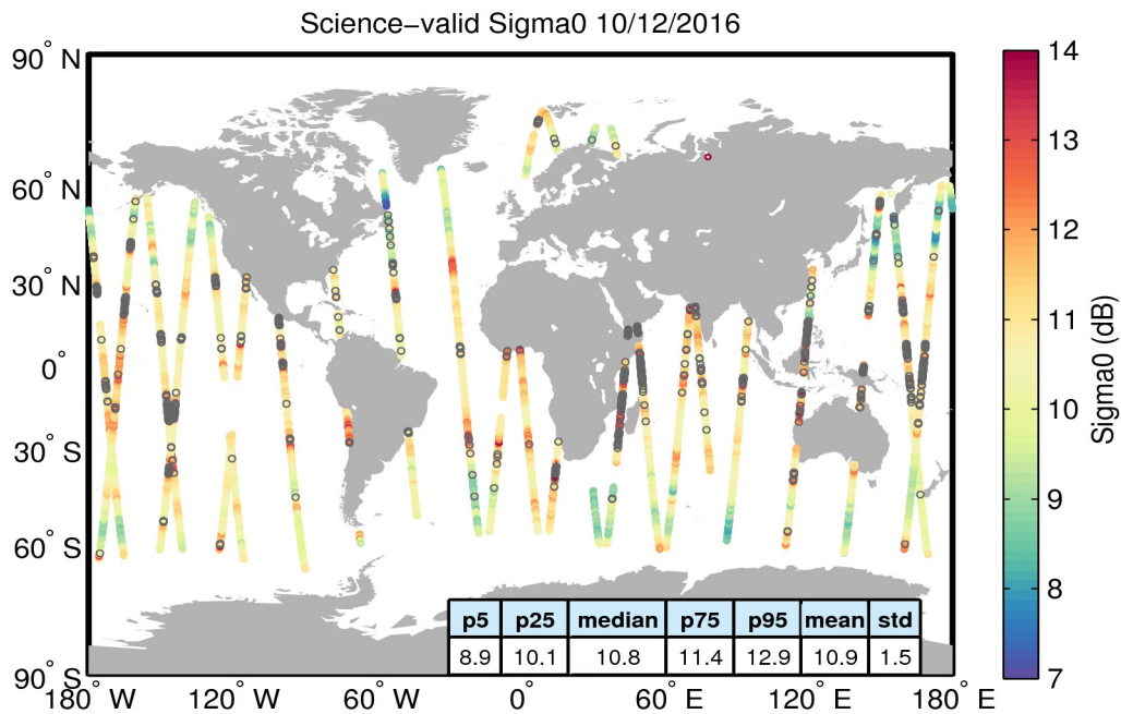
Figure 27. Geographical distribution of science-valid sigma0 data over oceans and lakes for 10/12/2016. The statistical values shown in the table refer to the sigma0 in dB and are calculated over all measurements shown in the figure. Gray circles denote records that have been rejected based on the editing criteria described in Table 4.
