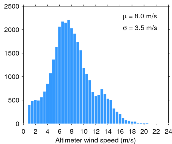
Figure 35. Histogram of science-valid wind over oceans and lakes for 10/12/2016. The mean ( \mu ) and standard deviation ( \sigma ) are also shown. Note that values larger than 24 m/s are excluded from the histogram for the sake of readability but not from the computation of \mu and \sigma .
