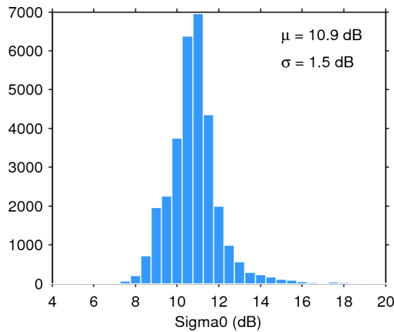
Figure 28. Histogram of science-valid sigma0 over oceans and lakes for 10/12/2016. The mean ( \mu ) and standard deviation ( \sigma ) are also shown. Note that values outside [4 20] dB are excluded from the histogram for the sake of readability but not from the computation of \mu and \sigma .
