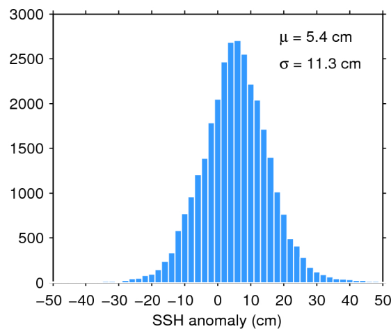
Figure 11. Histogram of science-valid SSH anomaly over oceans and lakes for 10/12/2016. The mean ( \mu ) and standard deviation ( \sigma ) are also shown. Note that values outside [-50 50] cm are excluded from the histogram for the sake of readability but not from the computation of \mu and \sigma .
