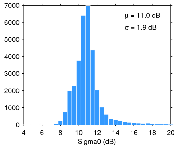
Figure 25. Histogram of flag-valid sigma0 over oceans and lakes for 10/12/2016. The mean ( \mu ) and standard deviation ( \sigma ) are also shown. Note that values outside [4 20] dB are excluded from the histogram for the sake of readability but not from the computation of \mu and \sigma .
