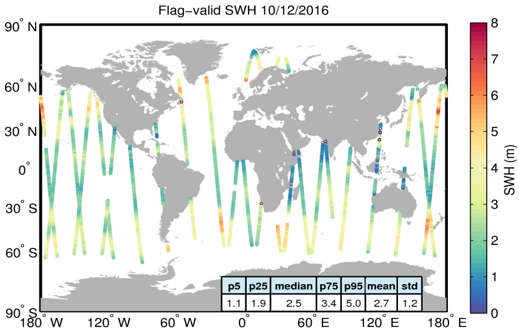
Figure 15. Geographical distribution of flag-valid SWH data over oceans and lakes for 10/12/2016. The statistical values shown in the table refer to the SWH in m and are calculated over all measurements shown in the figure.
