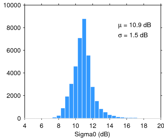
Figure 28. Histogram of science-valid sigma0 over oceans and lakes for 09/12/2016. The mean ( \mu ) and standard deviation ( \sigma ) are also shown. Note that values outside [4 20] dB are excluded from the histogram for the sake of readability but not from the computation of \mu and \sigma .
