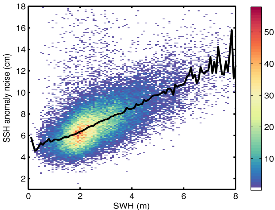
Figure 9. 2D histogram showing flag-valid SSH anomaly noise as a function of SWH for 09/12/2016. The black line denotes the median SSH anomaly noise as a function of SWH.
