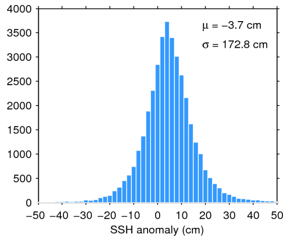
Figure 7. Histogram of flag-valid SSH anomaly over oceans and lakes for 09/12/2016. The mean ( \mu ) and standard deviation ( \sigma ) are also shown. Note that values outside [-50 50] cm are excluded from the histogram for the sake of readability but not from the computation of \mu and \sigma .
