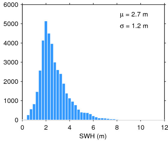
Figure 17. Histogram of flag-valid SWH over oceans and lakes for 09/12/2016. The mean ( \mu ) and standard deviation ( \sigma ) are also shown. Note that values larger than 12 m are excluded from the histogram for the sake of readability but not from the computation of \mu and \sigma .
