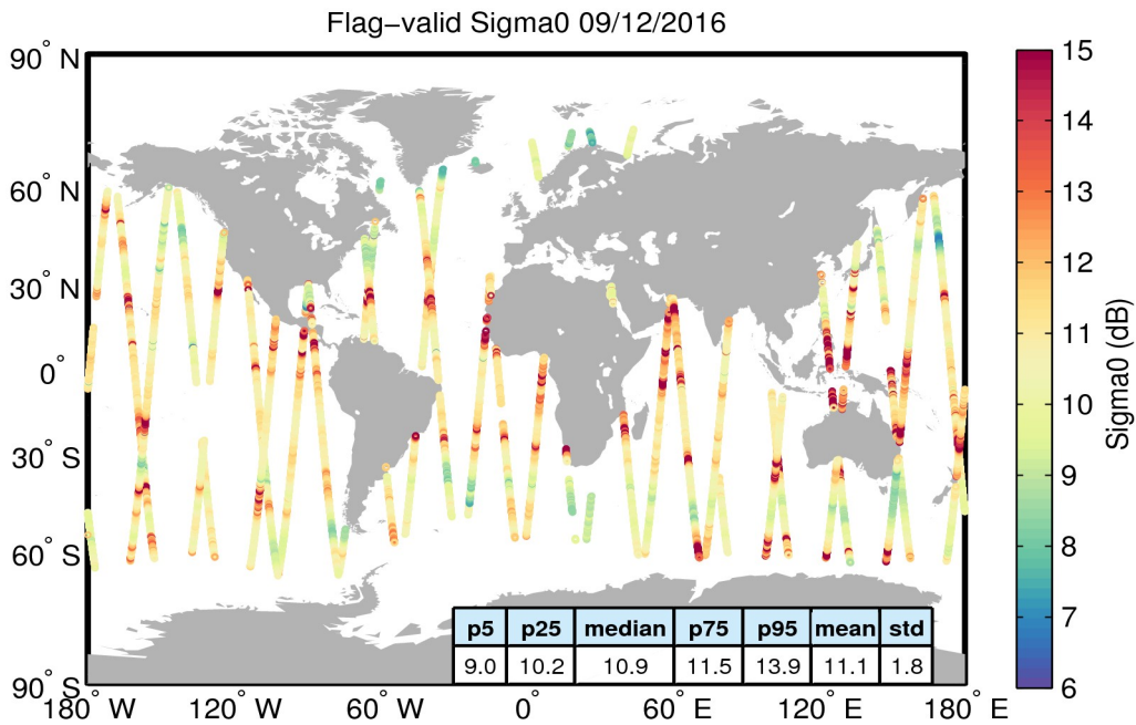
Figure 23. Geographical distribution of flag-valid sigma0 data over oceans and lakes for 09/12/2016. The statistical values shown in the table refer to the sigma0 in dB and are calculated over all measurements shown in the figure.
