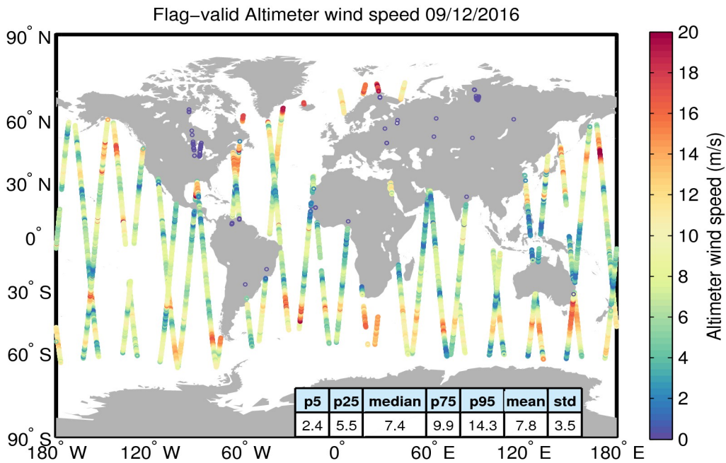
Figure 31. Geographical distribution of flag-valid wind data over oceans and lakes for 09/12/2016. The statistical values shown in the table refer to the wind in m/s and are calculated over all measurements shown in the figure.
