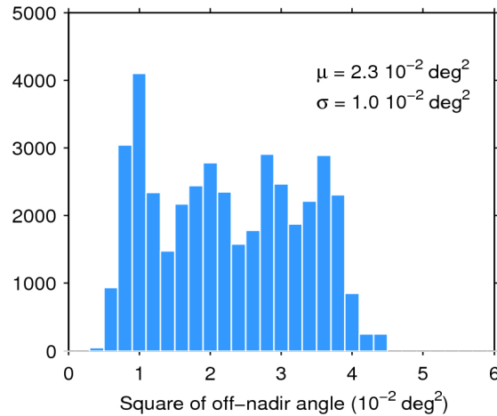
Figure 39. Histogram of flag-valid mispointing over oceans and lakes for 09/12/2016. The mean ( \mu ) and standard deviation ( \sigma ) are also shown. Note that values larger than 6 \cdot 10^{-2} \text{ deg}^2 are excluded from the histogram for the sake of readability but not from the computation of \mu and \sigma .
