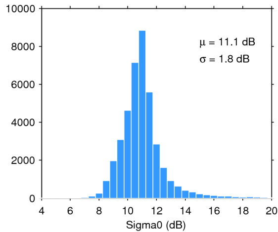
Figure 25. Histogram of flag-valid sigma0 over oceans and lakes for 09/12/2016. The mean ( \mu ) and standard deviation ( \sigma ) are also shown. Note that values outside [4 20] dB are excluded from the histogram for the sake of readability but not from the computation of \mu and \sigma .
