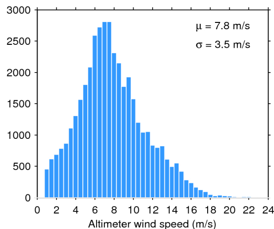
Figure 35. Histogram of science-valid wind over oceans and lakes for 09/12/2016. The mean ( \mu ) and standard deviation ( \sigma ) are also shown. Note that values larger than 24 m/s are excluded from the histogram for the sake of readability but not from the computation of \mu and \sigma .
