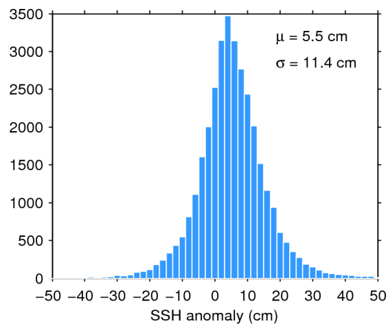
Figure 11. Histogram of science-valid SSH anomaly over oceans and lakes for 09/12/2016. The mean ( \mu ) and standard deviation ( \sigma ) are also shown. Note that values outside [-50 50] cm are excluded from the histogram for the sake of readability but not from the computation of \mu and \sigma .
