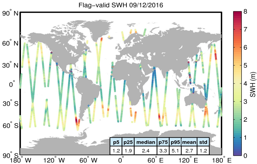
Figure 15. Geographical distribution of flag-valid SWH data over oceans and lakes for 09/12/2016. The statistical values shown in the table refer to the SWH in m and are calculated over all measurements shown in the figure.
