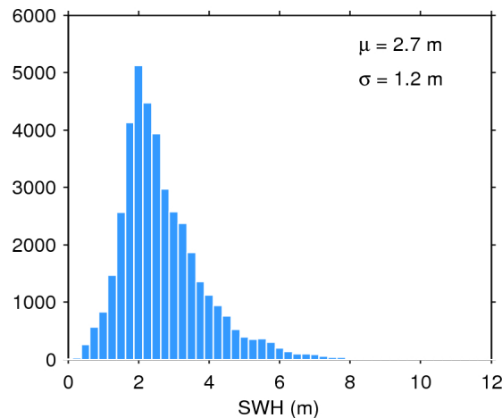
Figure 20. Histogram of science-valid SWH over oceans and lakes for 09/12/2016. The mean ( \mu ) and standard deviation ( \sigma ) are also shown. Note that values larger than 12 m are excluded from the histogram for the sake of readability but not from the computation of \mu and \sigma .
