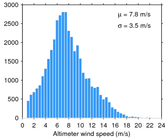
Figure 33. Histogram of flag-valid wind over oceans and lakes for 09/12/2016. The mean ( \mu ) and standard deviation ( \sigma ) are also shown. Note that values larger than 24 m/s are excluded from the histogram for the sake of readability but not from the computation of \mu and \sigma .
