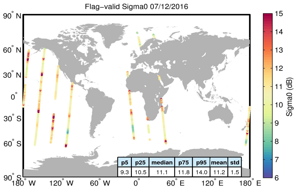
Figure 23. Geographical distribution of flag-valid sigma0 data over oceans and lakes for 07/12/2016. The statistical values shown in the table refer to the sigma0 in dB and are calculated over all measurements shown in the figure.
