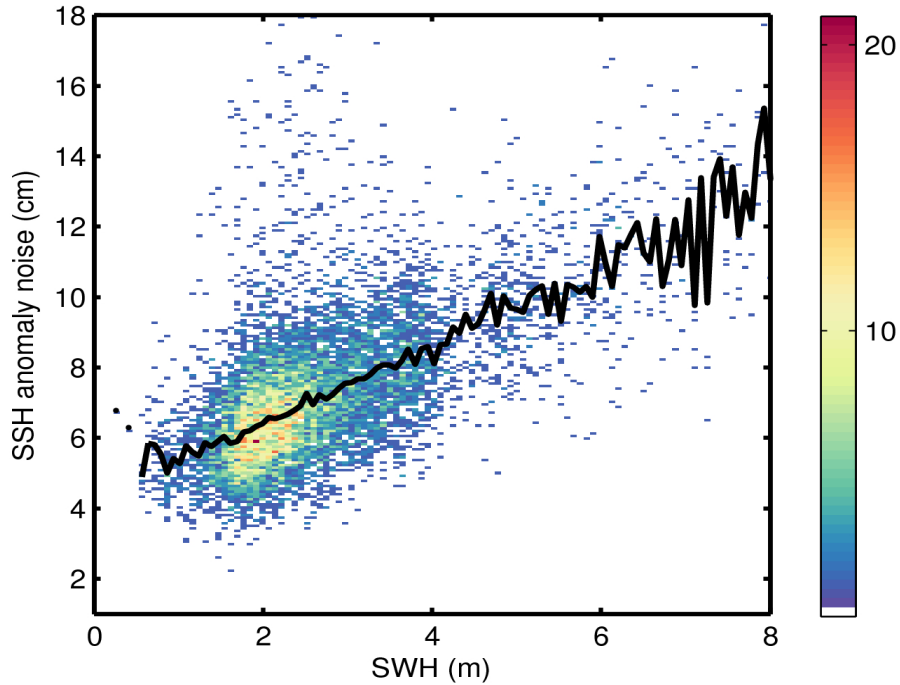
Figure 9. 2D histogram showing flag-valid SSH anomaly noise as a function of SWH for 07/12/2016. The black line denotes the median SSH anomaly noise as a function of SWH.
