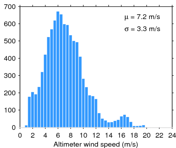
Figure 35. Histogram of science-valid wind over oceans and lakes for 07/12/2016. The mean ( \mu ) and standard deviation ( \sigma ) are also shown. Note that values larger than 24 m/s are excluded from the histogram for the sake of readability but not from the computation of \mu and \sigma .
