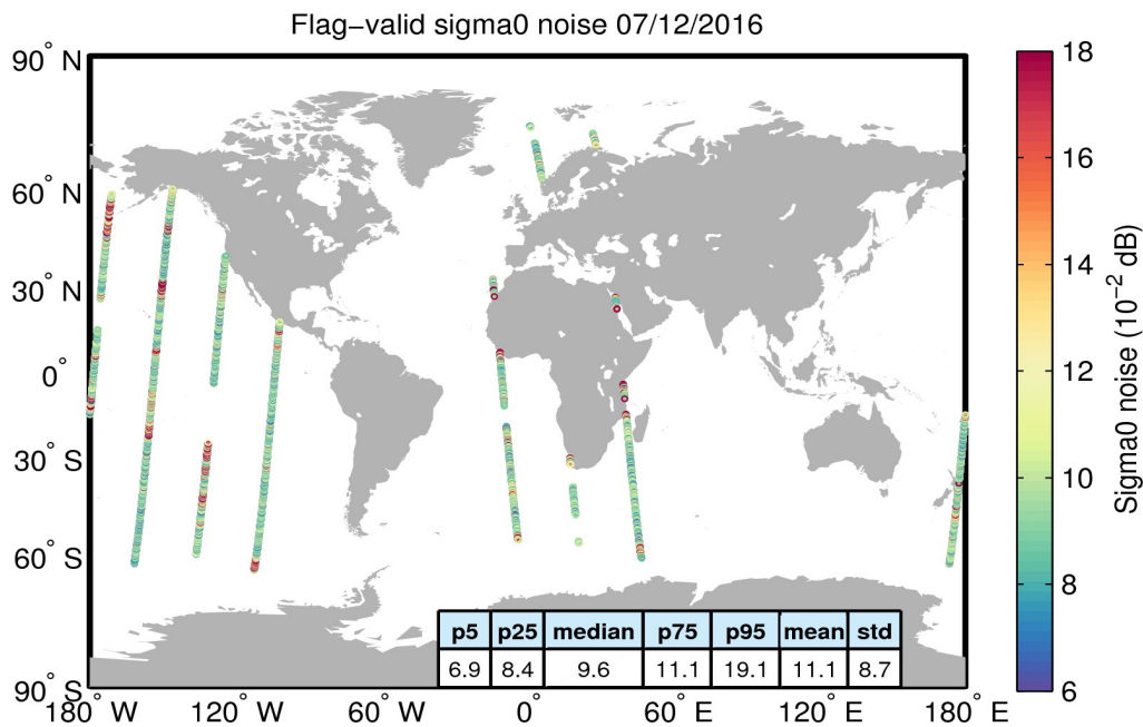
Figure 26. Geographical distribution of flag-valid 20-Hz sigma0 measurement noise over oceans and lakes for 07/12/2016. The statistical values shown in the table refer to the sigma0 noise and are calculated over all measurements shown in the figure.
