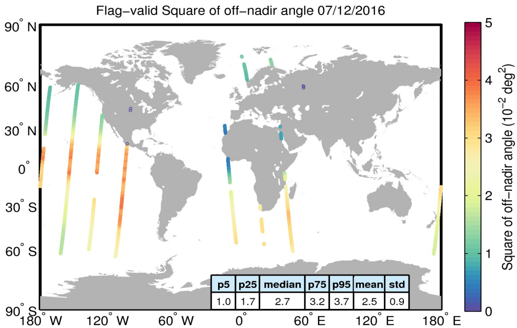
Figure 37. Geographical distribution of flag-valid mispointing data over oceans and lakes for 07/12/2016. The statistical values shown in the table refer to the mispointing in 10^{-2} deg 2 and are calculated over all measurements shown in the figure.
