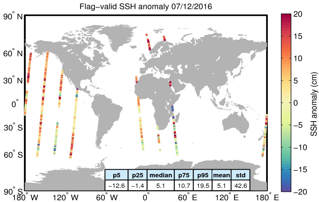
Figure 5. Geographical distribution of flag-valid 1-Hz SSH anomaly data over oceans and lakes for 07/12/2016. The statistical values shown in the table refer to the SSH anomaly in cm and are calculated over all measurements shown in the figure.
