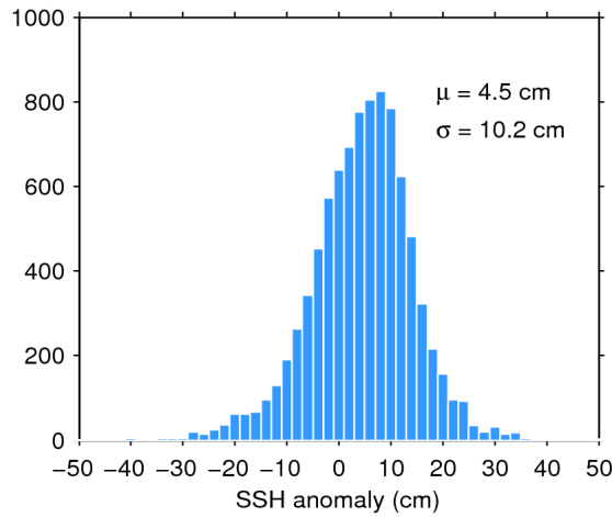
Figure 11. Histogram of science-valid SSH anomaly over oceans and lakes for 07/12/2016. The mean ( \mu ) and standard deviation ( \sigma ) are also shown. Note that values outside [-50 50] cm are excluded from the histogram for the sake of readability but not from the computation of \mu and \sigma .
