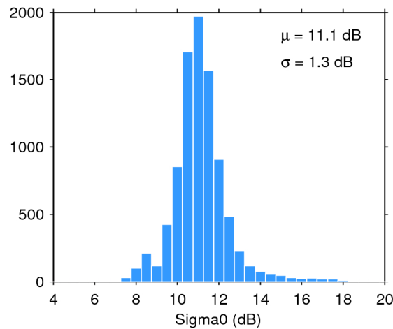
Figure 28. Histogram of science-valid sigma0 over oceans and lakes for 07/12/2016. The mean ( \mu ) and standard deviation ( \sigma ) are also shown. Note that values outside [4 20] dB are excluded from the histogram for the sake of readability but not from the computation of \mu and \sigma .
