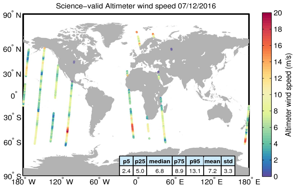
Figure 34. Geographical distribution of science-valid wind data over oceans and lakes for 07/12/2016. The statistical values shown in the table refer to the wind in m/s and are calculated over all measurements shown in the figure. Gray circles denote records that have been rejected based on the editing criteria described in Table 5.
