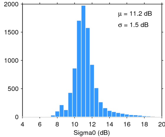
Figure 25. Histogram of flag-valid sigma0 over oceans and lakes for 07/12/2016. The mean ( \mu ) and standard deviation ( \sigma ) are also shown. Note that values outside [4 20] dB are excluded from the histogram for the sake of readability but not from the computation of \mu and \sigma .
