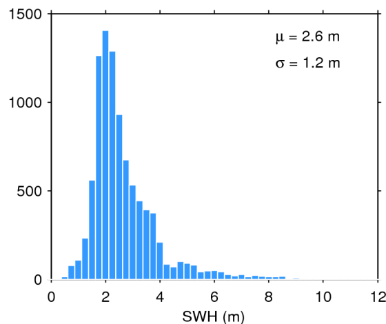
Figure 20. Histogram of science-valid SWH over oceans and lakes for 07/12/2016. The mean ( \mu ) and standard deviation ( \sigma ) are also shown. Note that values larger than 12 m are excluded from the histogram for the sake of readability but not from the computation of \mu and \sigma .
