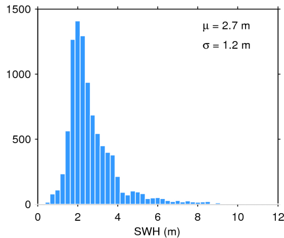
Figure 17. Histogram of flag-valid SWH over oceans and lakes for 07/12/2016. The mean ( \mu ) and standard deviation ( \sigma ) are also shown. Note that values larger than 12 m are excluded from the histogram for the sake of readability but not from the computation of \mu and \sigma .
