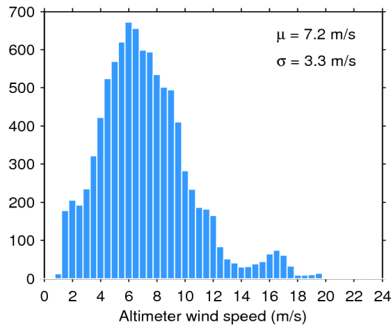
Figure 33. Histogram of flag-valid wind over oceans and lakes for 07/12/2016. The mean ( \mu ) and standard deviation ( \sigma ) are also shown. Note that values larger than 24 m/s are excluded from the histogram for the sake of readability but not from the computation of \mu and \sigma .
