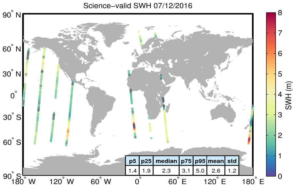
Figure 19. Geographical distribution of science-valid SWH data over oceans and lakes for 07/12/2016. The statistical values shown in the table refer to the SWH in m and are calculated over all measurements shown in the figure. Gray circles denote records that have been rejected based on the editing criteria described in Table 3.
