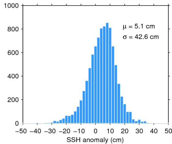
Figure 7. Histogram of flag-valid SSH anomaly over oceans and lakes for 07/12/2016. The mean ( \mu ) and standard deviation ( \sigma ) are also shown. Note that values outside [-50\ 50] cm are excluded from the histogram for the sake of readability but not from the computation of \mu and \sigma .
