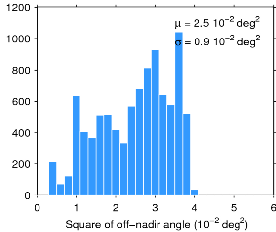
Figure 39. Histogram of flag-valid mispointing over oceans and lakes for 07/12/2016. The mean ( \mu ) and standard deviation ( \sigma ) are also shown. Note that values larger than 6 \cdot 10^{-2} \text{ deg}^2 are excluded from the histogram for the sake of readability but not from the computation of \mu and \sigma .
