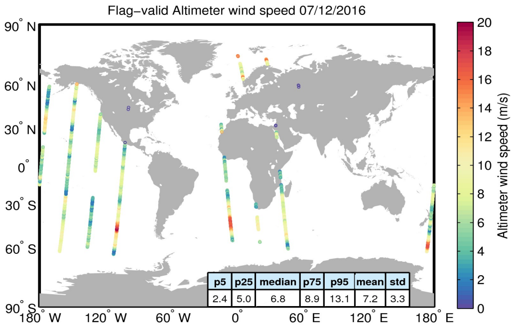
Figure 31. Geographical distribution of flag-valid wind data over oceans and lakes for 07/12/2016. The statistical values shown in the table refer to the wind in m/s and are calculated over all measurements shown in the figure.
