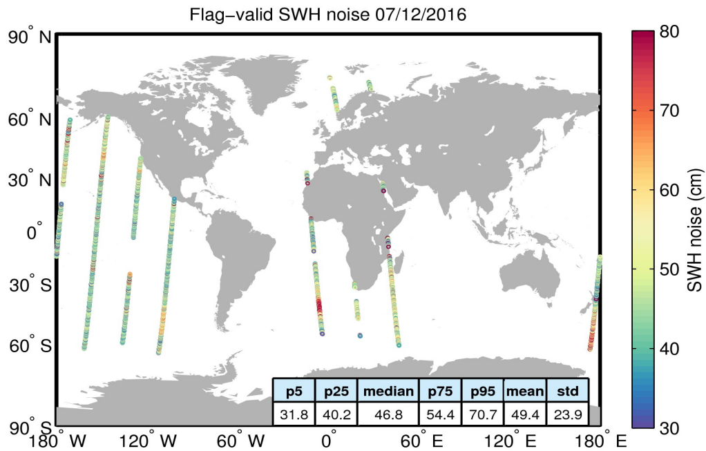
Figure 18. Geographical distribution of flag-valid 20-Hz SWH measurement noise over oceans and lakes for 07/12/2016. The statistical values shown in the table refer to the SWH noise and are calculated over all measurements shown in the figure.
