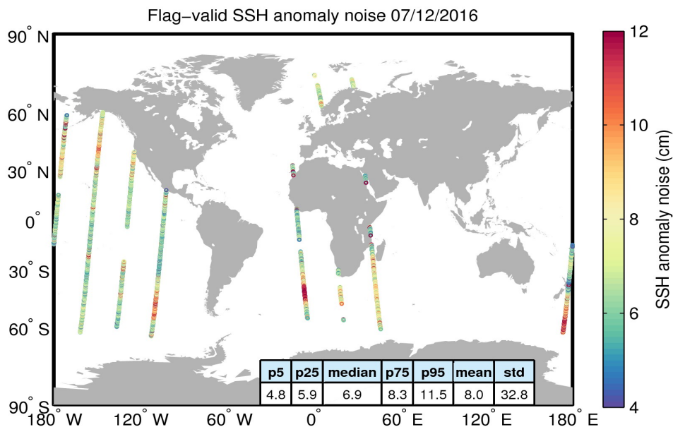
Figure 8. Geographical distribution of flag-valid 20-Hz SSH anomaly measurement noise over oceans and lakes for 07/12/2016. The statistical values shown in the table refer to the SSH anomaly noise and are calculated over all measurements shown in the figure.
