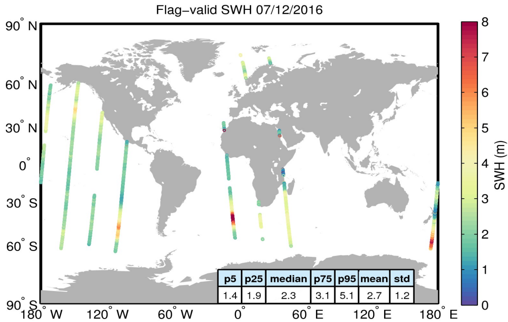
Figure 15. Geographical distribution of flag-valid SWH data over oceans and lakes for 07/12/2016. The statistical values shown in the table refer to the SWH in m and are calculated over all measurements shown in the figure.
