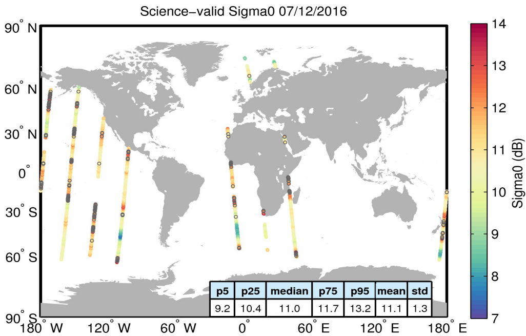
Figure 27. Geographical distribution of science-valid sigma0 data over oceans and lakes for 07/12/2016. The statistical values shown in the table refer to the sigma0 in dB and are calculated over all measurements shown in the figure. Gray circles denote records that have been rejected based on the editing criteria described in Table 4.
