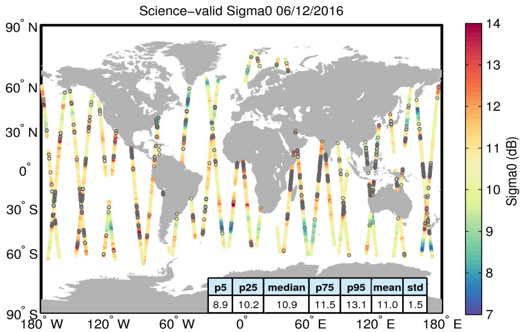
Figure 27. Geographical distribution of science-valid sigma0 data over oceans and lakes for 06/12/2016. The statistical values shown in the table refer to the sigma0 in dB and are calculated over all measurements shown in the figure. Gray circles denote records that have been rejected based on the editing criteria described in Table 4.
