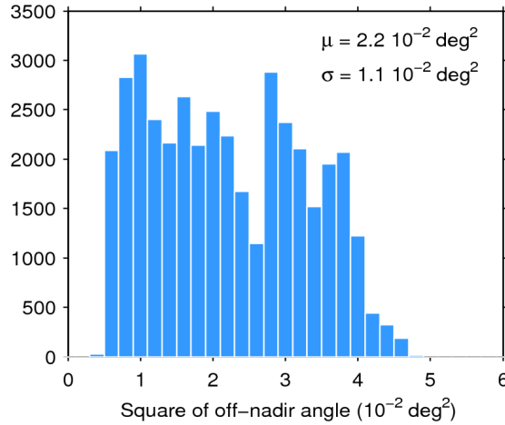
Figure 39. Histogram of flag-valid mispointing over oceans and lakes for 06/12/2016. The mean ( \mu ) and standard deviation ( \sigma ) are also shown. Note that values larger than 6 \cdot 10^{-2} \text{ deg}^2 are excluded from the histogram for the sake of readability but not from the computation of \mu and \sigma .
