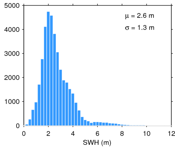
Figure 17. Histogram of flag-valid SWH over oceans and lakes for 06/12/2016. The mean ( \mu ) and standard deviation ( \sigma ) are also shown. Note that values larger than 12 m are excluded from the histogram for the sake of readability but not from the computation of \mu and \sigma .
