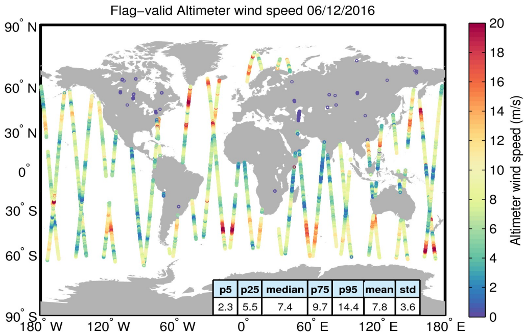
Figure 31. Geographical distribution of flag-valid wind data over oceans and lakes for 06/12/2016. The statistical values shown in the table refer to the wind in m/s and are calculated over all measurements shown in the figure.
