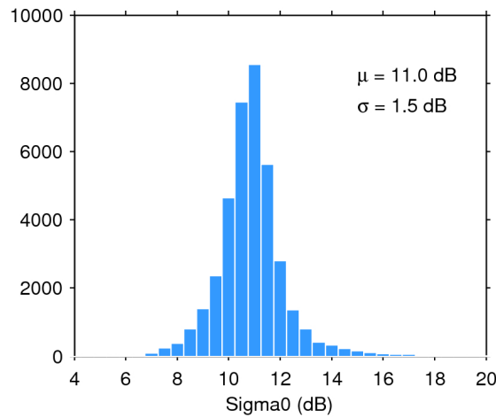
Figure 28. Histogram of science-valid sigma0 over oceans and lakes for 06/12/2016. The mean ( \mu ) and standard deviation ( \sigma ) are also shown. Note that values outside [4 20] dB are excluded from the histogram for the sake of readability but not from the computation of \mu and \sigma .
