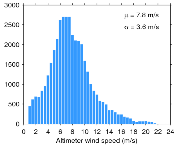
Figure 33. Histogram of flag-valid wind over oceans and lakes for 06/12/2016. The mean ( \mu ) and standard deviation ( \sigma ) are also shown. Note that values larger than 24 m/s are excluded from the histogram for the sake of readability but not from the computation of \mu and \sigma .
