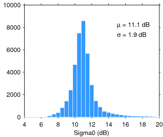
Figure 25. Histogram of flag-valid sigma0 over oceans and lakes for 06/12/2016. The mean ( \mu ) and standard deviation ( \sigma ) are also shown. Note that values outside [4 20] dB are excluded from the histogram for the sake of readability but not from the computation of \mu and \sigma .
