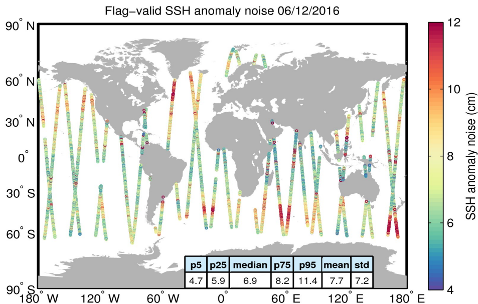
Figure 8. Geographical distribution of flag-valid 20-Hz SSH anomaly measurement noise over oceans and lakes for 06/12/2016. The statistical values shown in the table refer to the SSH anomaly noise and are calculated over all measurements shown in the figure.
