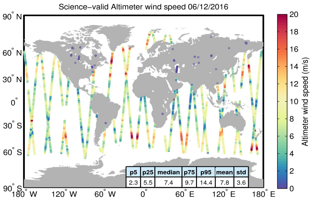
Figure 34. Geographical distribution of science-valid wind data over oceans and lakes for 06/12/2016. The statistical values shown in the table refer to the wind in m/s and are calculated over all measurements shown in the figure. Gray circles denote records that have been rejected based on the editing criteria described in Table 5.
