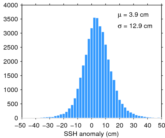
Figure 7. Histogram of flag-valid SSH anomaly over oceans and lakes for 06/12/2016. The mean ( \mu ) and standard deviation ( \sigma ) are also shown. Note that values outside [-50\ 50] cm are excluded from the histogram for the sake of readability but not from the computation of \mu and \sigma .
