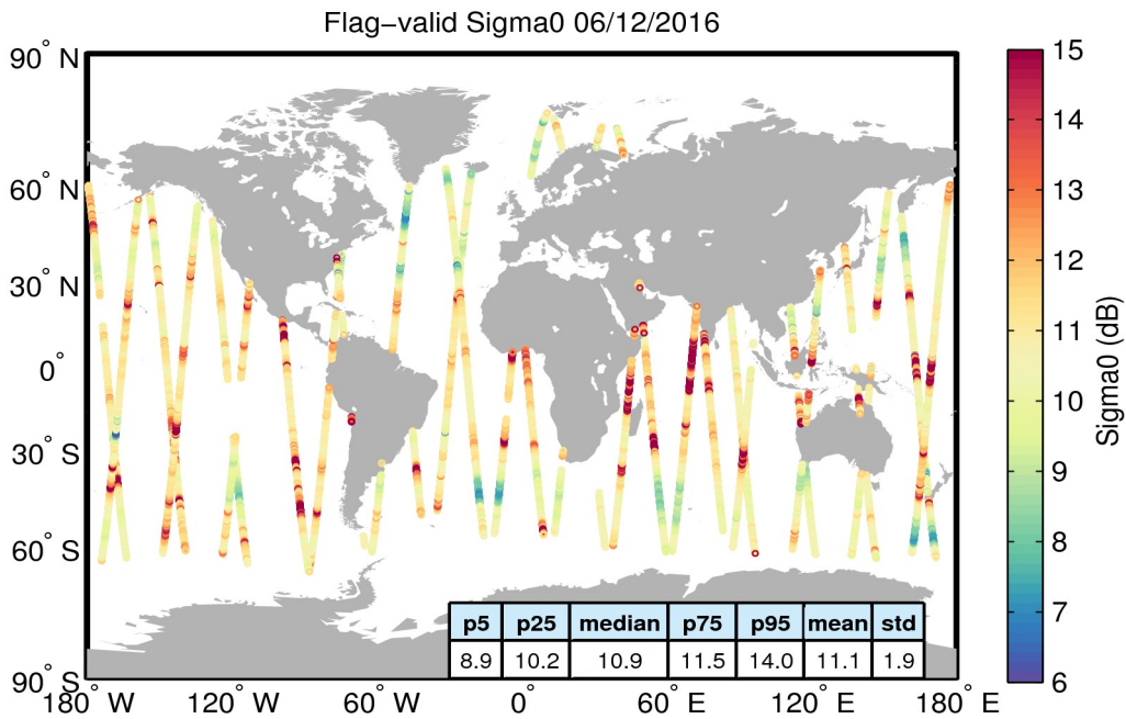
Figure 23. Geographical distribution of flag-valid sigma0 data over oceans and lakes for 06/12/2016. The statistical values shown in the table refer to the sigma0 in dB and are calculated over all measurements shown in the figure.
