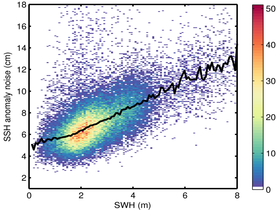
Figure 9. 2D histogram showing flag-valid SSH anomaly noise as a function of SWH for 06/12/2016. The black line denotes the median SSH anomaly noise as a function of SWH.
