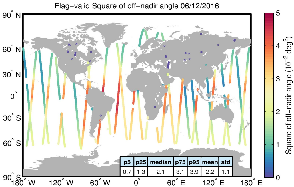
Figure 37. Geographical distribution of flag-valid mispointing data over oceans and lakes for 06/12/2016. The statistical values shown in the table refer to the mispointing in 10^{-2} deg 2 and are calculated over all measurements shown in the figure.
