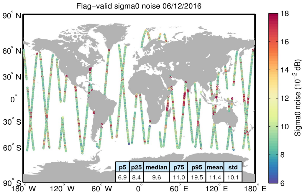
Figure 26. Geographical distribution of flag-valid 20-Hz sigma0 measurement noise over oceans and lakes for 06/12/2016. The statistical values shown in the table refer to the sigma0 noise and are calculated over all measurements shown in the figure.
