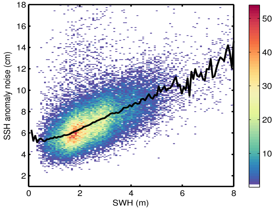
Figure 9. 2D histogram showing flag-valid SSH anomaly noise as a function of SWH for 05/12/2016. The black line denotes the median SSH anomaly noise as a function of SWH.
