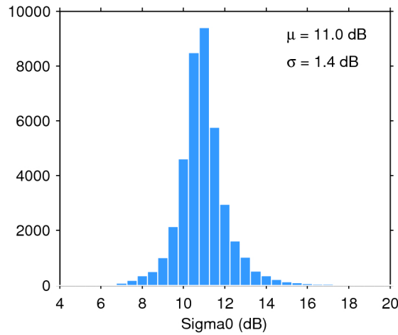
Figure 28. Histogram of science-valid sigma0 over oceans and lakes for 05/12/2016. The mean ( \mu ) and standard deviation ( \sigma ) are also shown. Note that values outside [4 20] dB are excluded from the histogram for the sake of readability but not from the computation of \mu and \sigma .
