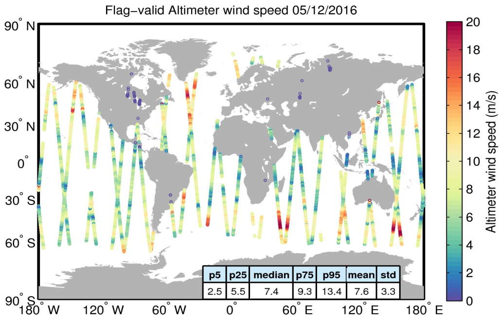
Figure 31. Geographical distribution of flag-valid wind data over oceans and lakes for 05/12/2016. The statistical values shown in the table refer to the wind in m/s and are calculated over all measurements shown in the figure.
