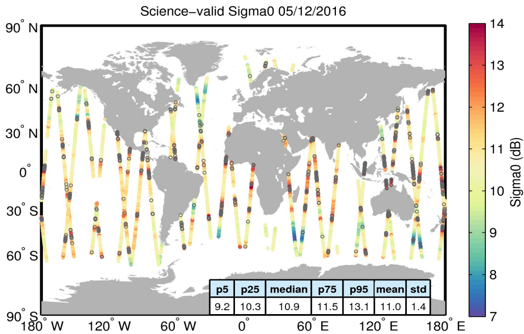
Figure 27. Geographical distribution of science-valid sigma0 data over oceans and lakes for 05/12/2016. The statistical values shown in the table refer to the sigma0 in dB and are calculated over all measurements shown in the figure. Gray circles denote records that have been rejected based on the editing criteria described in Table 4.
