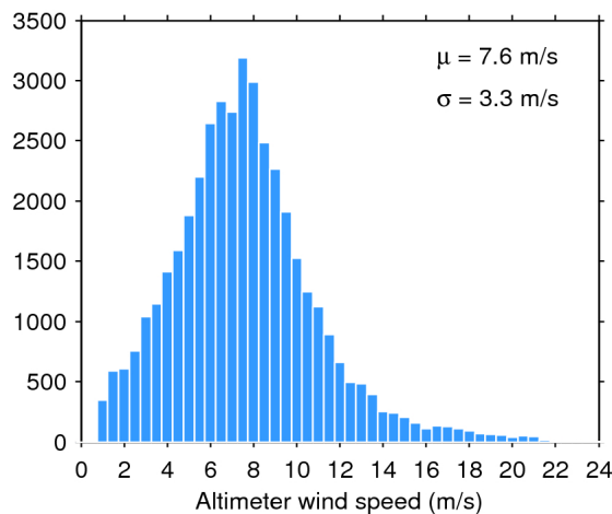
Figure 35. Histogram of science-valid wind over oceans and lakes for 05/12/2016. The mean ( \mu ) and standard deviation ( \sigma ) are also shown. Note that values larger than 24 m/s are excluded from the histogram for the sake of readability but not from the computation of \mu and \sigma .
