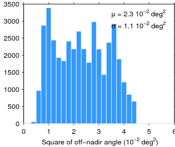
Figure 39. Histogram of flag-valid mispointing over oceans and lakes for 05/12/2016. The mean ( \mu ) and standard deviation ( \sigma ) are also shown. Note that values larger than 6 \cdot 10^{-2} \text{ deg}^2 are excluded from the histogram for the sake of readability but not from the computation of \mu and \sigma .
