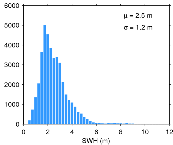
Figure 17. Histogram of flag-valid SWH over oceans and lakes for 05/12/2016. The mean ( \mu ) and standard deviation ( \sigma ) are also shown. Note that values larger than 12 m are excluded from the histogram for the sake of readability but not from the computation of \mu and \sigma .
