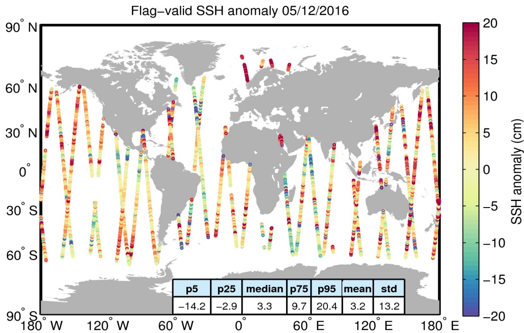
Figure 5. Geographical distribution of flag-valid 1-Hz SSH anomaly data over oceans and lakes for 05/12/2016. The statistical values shown in the table refer to the SSH anomaly in cm and are calculated over all measurements shown in the figure.
