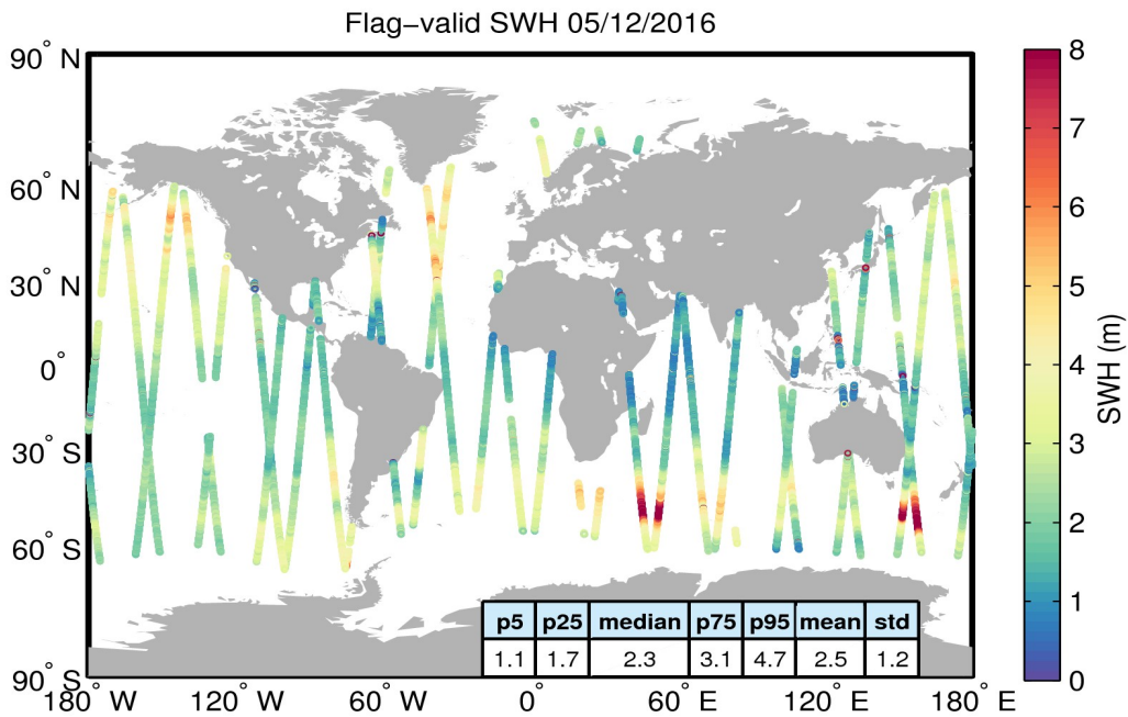
Figure 15. Geographical distribution of flag-valid SWH data over oceans and lakes for 05/12/2016. The statistical values shown in the table refer to the SWH in m and are calculated over all measurements shown in the figure.
