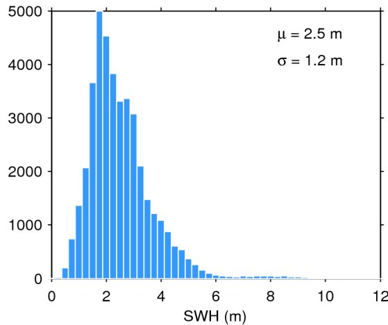
Figure 20. Histogram of science-valid SWH over oceans and lakes for 05/12/2016. The mean ( \mu ) and standard deviation ( \sigma ) are also shown. Note that values larger than 12 m are excluded from the histogram for the sake of readability but not from the computation of \mu and \sigma .
