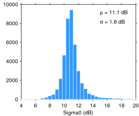
Figure 25. Histogram of flag-valid sigma0 over oceans and lakes for 05/12/2016. The mean ( \mu ) and standard deviation ( \sigma ) are also shown. Note that values outside [4 20] dB are excluded from the histogram for the sake of readability but not from the computation of \mu and \sigma .
