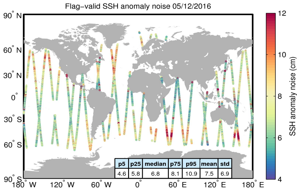
Figure 8. Geographical distribution of flag-valid 20-Hz SSH anomaly measurement noise over oceans and lakes for 05/12/2016. The statistical values shown in the table refer to the SSH anomaly noise and are calculated over all measurements shown in the figure.
