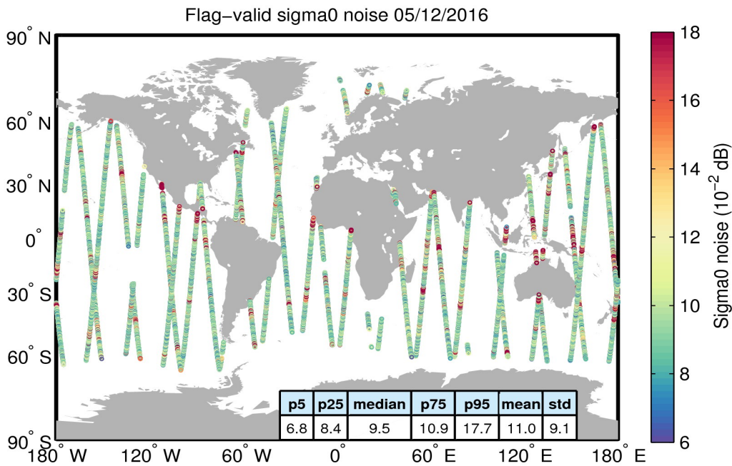
Figure 26. Geographical distribution of flag-valid 20-Hz sigma0 measurement noise over oceans and lakes for 05/12/2016. The statistical values shown in the table refer to the sigma0 noise and are calculated over all measurements shown in the figure.
