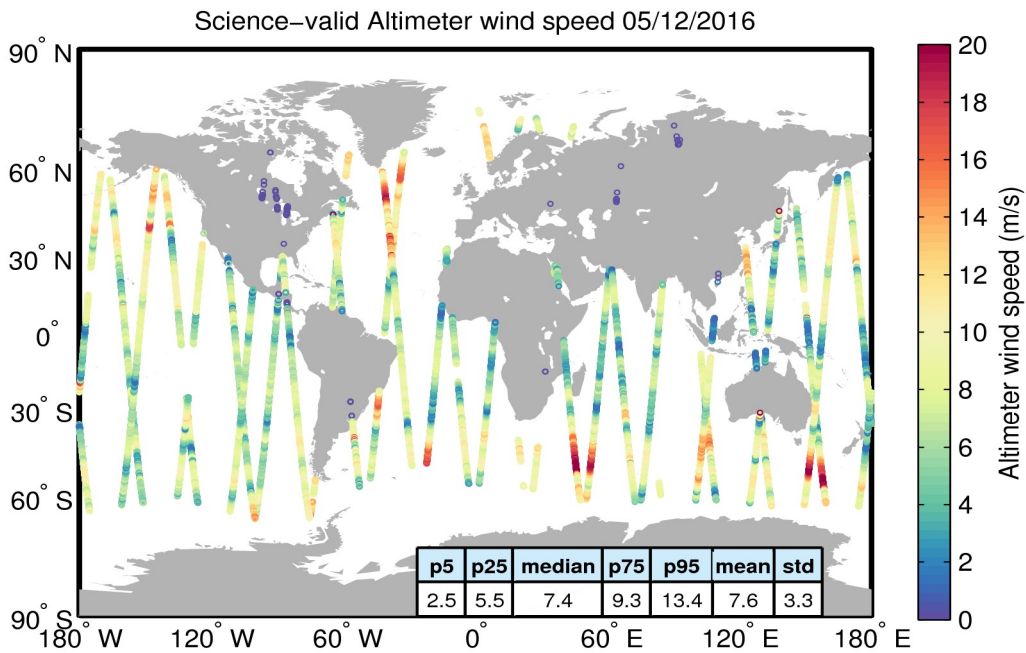
Figure 34. Geographical distribution of science-valid wind data over oceans and lakes for 05/12/2016. The statistical values shown in the table refer to the wind in m/s and are calculated over all measurements shown in the figure. Gray circles denote records that have been rejected based on the editing criteria described in Table 5.
