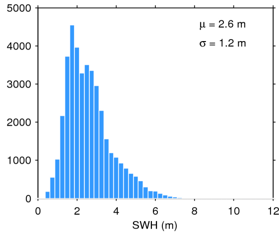
Figure 17. Histogram of flag-valid SWH over oceans and lakes for 04/12/2016. The mean ( \mu ) and standard deviation ( \sigma ) are also shown. Note that values larger than 12 m are excluded from the histogram for the sake of readability but not from the computation of \mu and \sigma .
