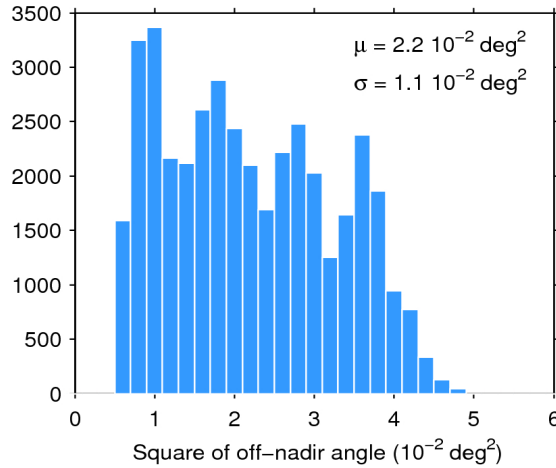
Figure 39. Histogram of flag-valid mispointing over oceans and lakes for 04/12/2016. The mean ( \mu ) and standard deviation ( \sigma ) are also shown. Note that values larger than 6 \cdot 10^{-2} \text{ deg}^2 are excluded from the histogram for the sake of readability but not from the computation of \mu and \sigma .
