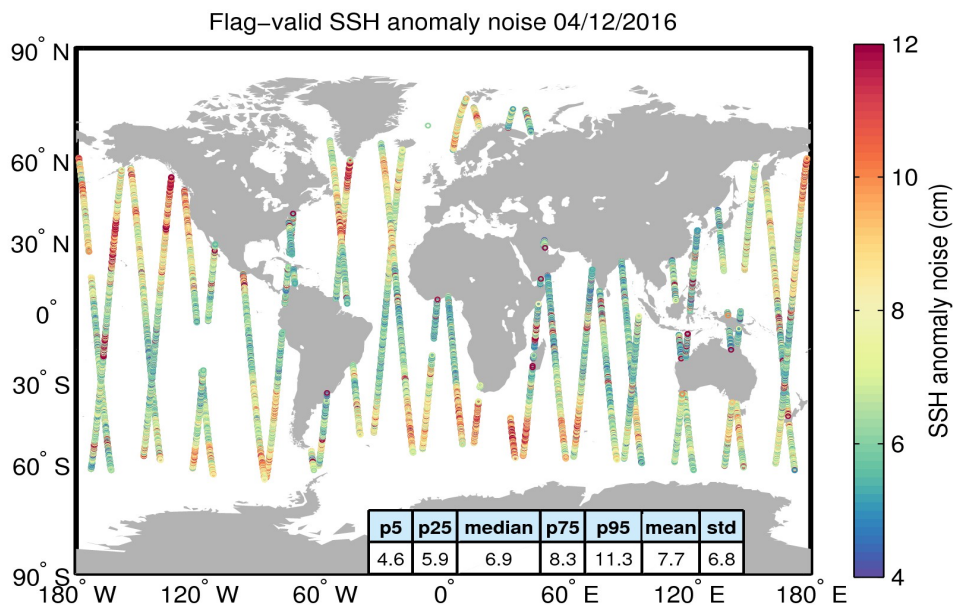
Figure 8. Geographical distribution of flag-valid 20-Hz SSH anomaly measurement noise over oceans and lakes for 04/12/2016. The statistical values shown in the table refer to the SSH anomaly noise and are calculated over all measurements shown in the figure.
