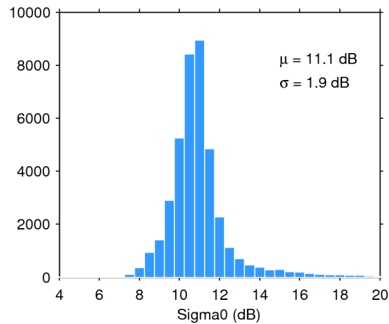
Figure 25. Histogram of flag-valid sigma0 over oceans and lakes for 04/12/2016. The mean ( \mu ) and standard deviation ( \sigma ) are also shown. Note that values outside [4 20] dB are excluded from the histogram for the sake of readability but not from the computation of \mu and \sigma .
