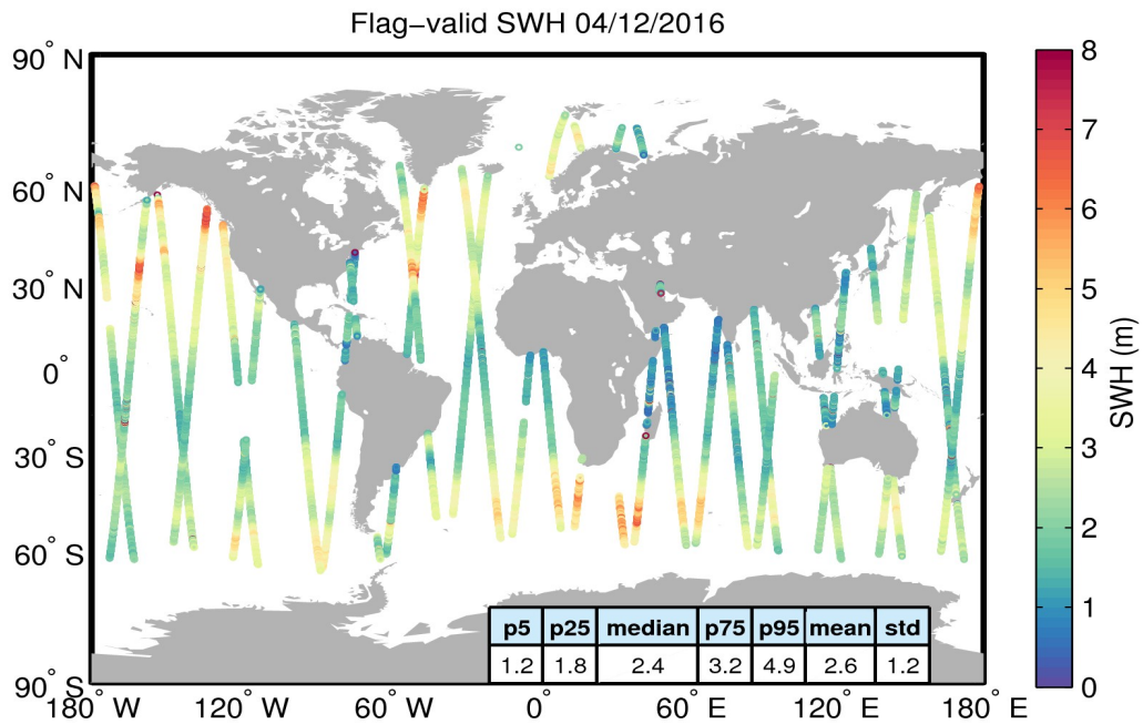
Figure 15. Geographical distribution of flag-valid SWH data over oceans and lakes for 04/12/2016. The statistical values shown in the table refer to the SWH in m and are calculated over all measurements shown in the figure.
