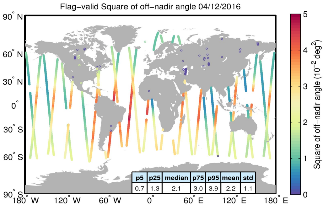
Figure 37. Geographical distribution of flag-valid mispointing data over oceans and lakes for 04/12/2016. The statistical values shown in the table refer to the mispointing in 10^{-2} deg 2 and are calculated over all measurements shown in the figure.
