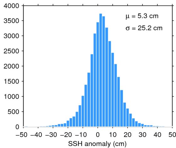
Figure 7. Histogram of flag-valid SSH anomaly over oceans and lakes for 04/12/2016. The mean ( \mu ) and standard deviation ( \sigma ) are also shown. Note that values outside [-50 50] cm are excluded from the histogram for the sake of readability but not from the computation of \mu and \sigma .
