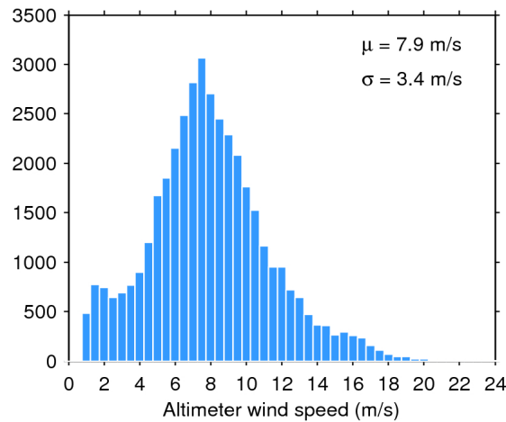
Figure 33. Histogram of flag-valid wind over oceans and lakes for 04/12/2016. The mean ( \mu ) and standard deviation ( \sigma ) are also shown. Note that values larger than 24 m/s are excluded from the histogram for the sake of readability but not from the computation of \mu and \sigma .
