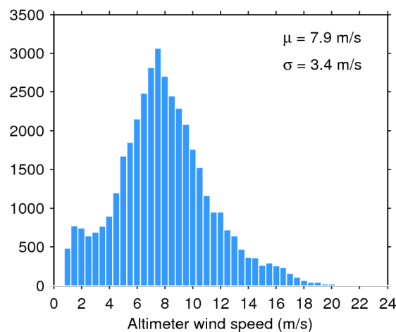
Figure 35. Histogram of science-valid wind over oceans and lakes for 04/12/2016. The mean ( \mu ) and standard deviation ( \sigma ) are also shown. Note that values larger than 24 m/s are excluded from the histogram for the sake of readability but not from the computation of \mu and \sigma .
