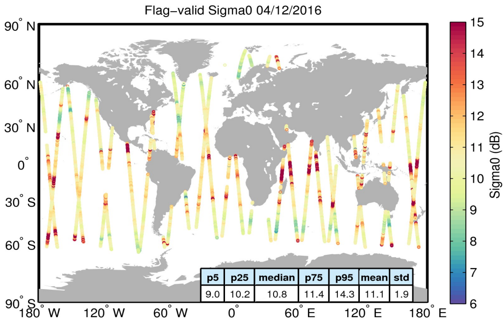
Figure 23. Geographical distribution of flag-valid sigma0 data over oceans and lakes for 04/12/2016. The statistical values shown in the table refer to the sigma0 in dB and are calculated over all measurements shown in the figure.
