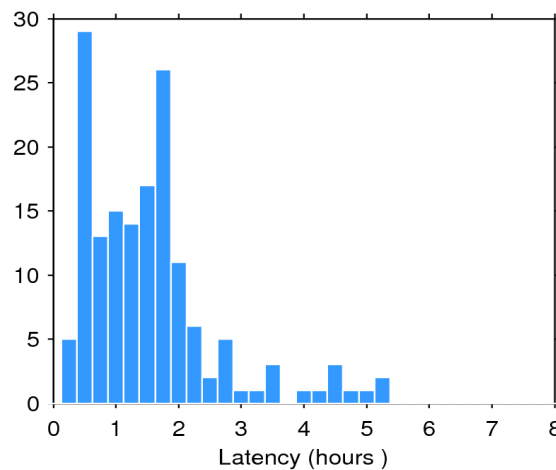
Figure 2. Histogram of the data latency for 04/12/2016. The y-axis denotes the number of files that are made available with a delay of x-hours with respect to the mean time of the records stored in the file.
