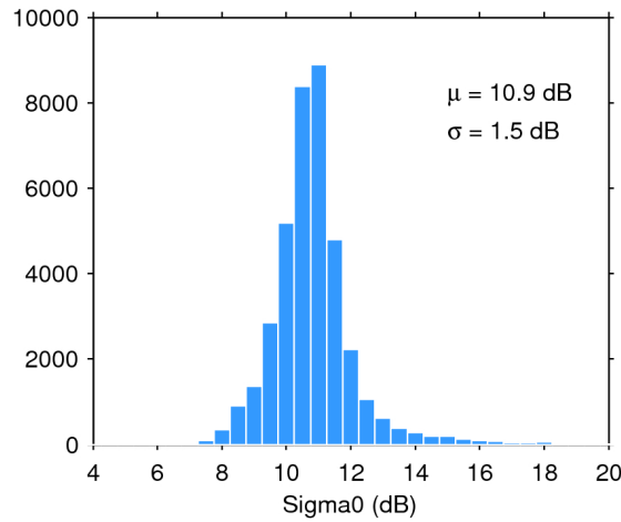
Figure 28. Histogram of science-valid sigma0 over oceans and lakes for 04/12/2016. The mean ( \mu ) and standard deviation ( \sigma ) are also shown. Note that values outside [4 20] dB are excluded from the histogram for the sake of readability but not from the computation of \mu and \sigma .
