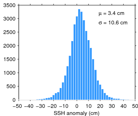
Figure 11. Histogram of science-valid SSH anomaly over oceans and lakes for 04/12/2016. The mean ( \mu ) and standard deviation ( \sigma ) are also shown. Note that values outside [-50 50] cm are excluded from the histogram for the sake of readability but not from the computation of \mu and \sigma .
