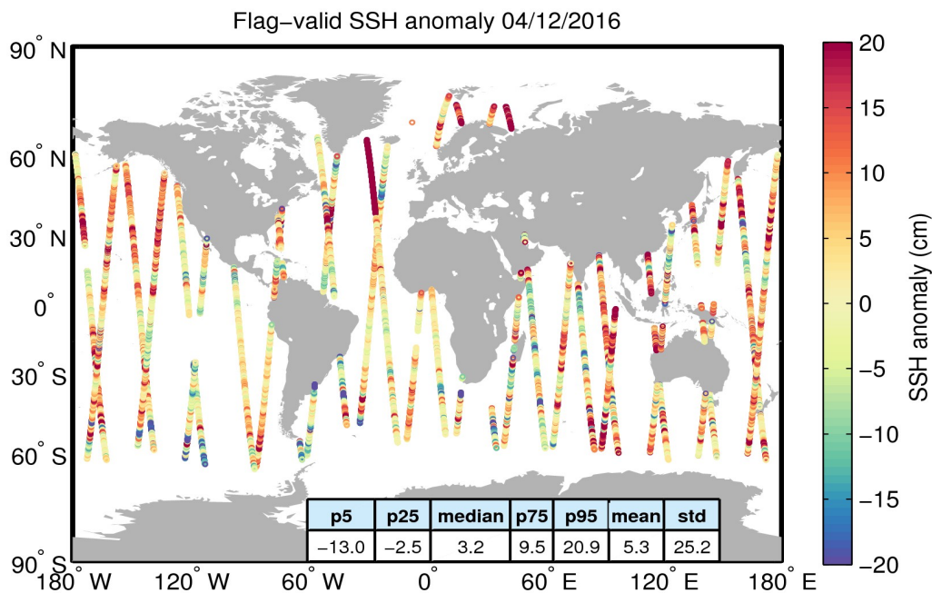
Figure 5. Geographical distribution of flag-valid 1-Hz SSH anomaly data over oceans and lakes for 04/12/2016. The statistical values shown in the table refer to the SSH anomaly in cm and are calculated over all measurements shown in the figure.
