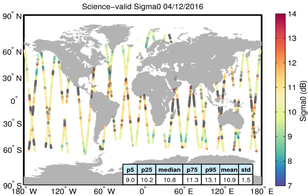
Figure 27. Geographical distribution of science-valid sigma0 data over oceans and lakes for 04/12/2016. The statistical values shown in the table refer to the sigma0 in dB and are calculated over all measurements shown in the figure. Gray circles denote records that have been rejected based on the editing criteria described in Table 4.
