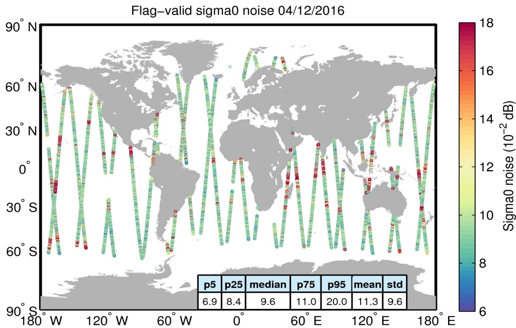
Figure 26. Geographical distribution of flag-valid 20-Hz sigma0 measurement noise over oceans and lakes for 04/12/2016. The statistical values shown in the table refer to the sigma0 noise and are calculated over all measurements shown in the figure.
