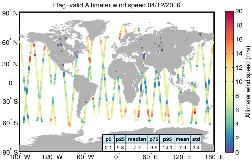
Figure 31. Geographical distribution of flag-valid wind data over oceans and lakes for 04/12/2016. The statistical values shown in the table refer to the wind in m/s and are calculated over all measurements shown in the figure.
