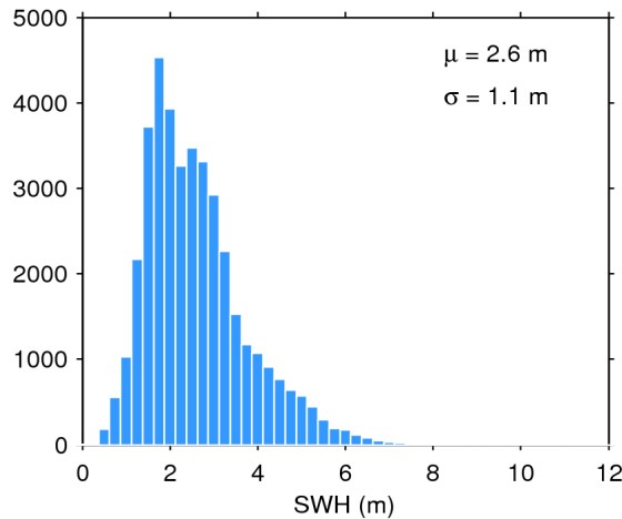
Figure 20. Histogram of science-valid SWH over oceans and lakes for 04/12/2016. The mean ( \mu ) and standard deviation ( \sigma ) are also shown. Note that values larger than 12 m are excluded from the histogram for the sake of readability but not from the computation of \mu and \sigma .
