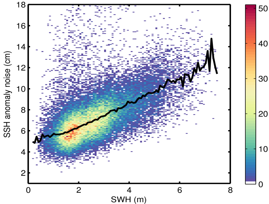
Figure 9. 2D histogram showing flag-valid SSH anomaly noise as a function of SWH for 04/12/2016. The black line denotes the median SSH anomaly noise as a function of SWH.
