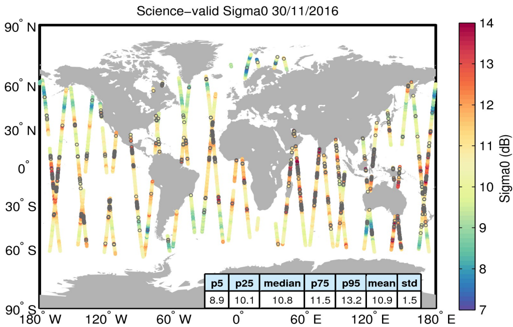
Figure 27. Geographical distribution of science-valid sigma0 data over oceans and lakes for 30/11/2016. The statistical values shown in the table refer to the sigma0 in dB and are calculated over all measurements shown in the figure. Gray circles denote records that have been rejected based on the editing criteria described in Table 4.
