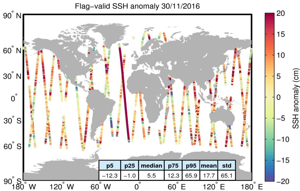
Figure 5. Geographical distribution of flag-valid 1-Hz SSH anomaly data over oceans and lakes for 30/11/2016. The statistical values shown in the table refer to the SSH anomaly in cm and are calculated over all measurements shown in the figure.
