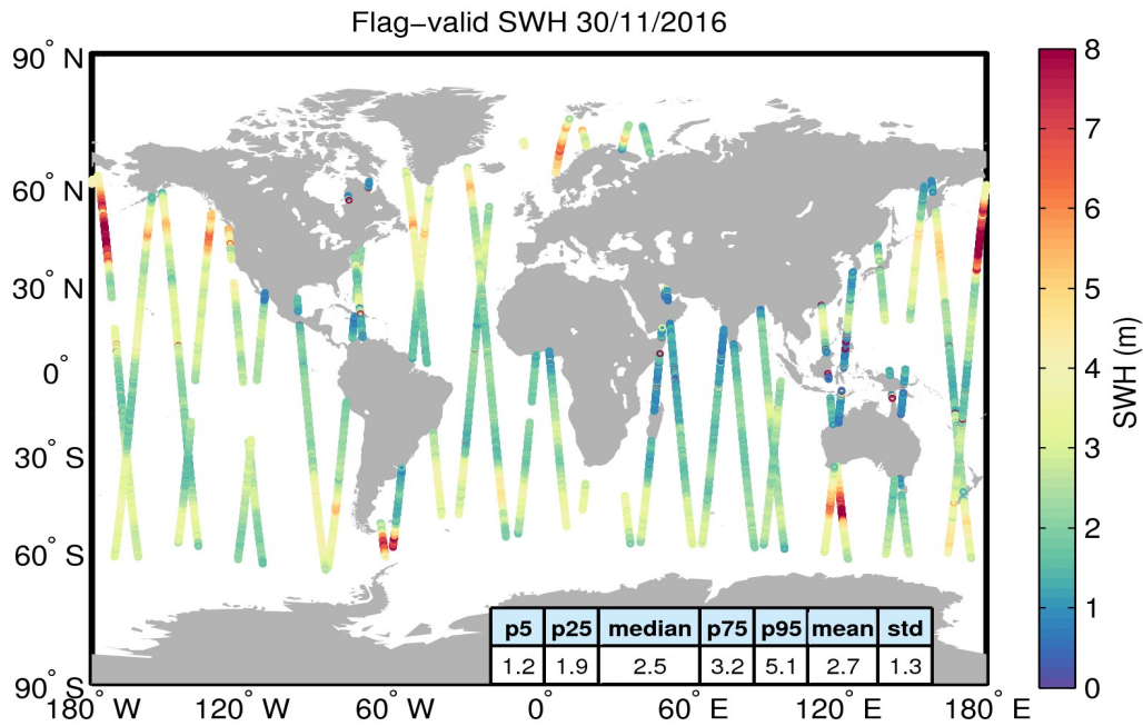
Figure 15. Geographical distribution of flag-valid SWH data over oceans and lakes for 30/11/2016. The statistical values shown in the table refer to the SWH in m and are calculated over all measurements shown in the figure.
