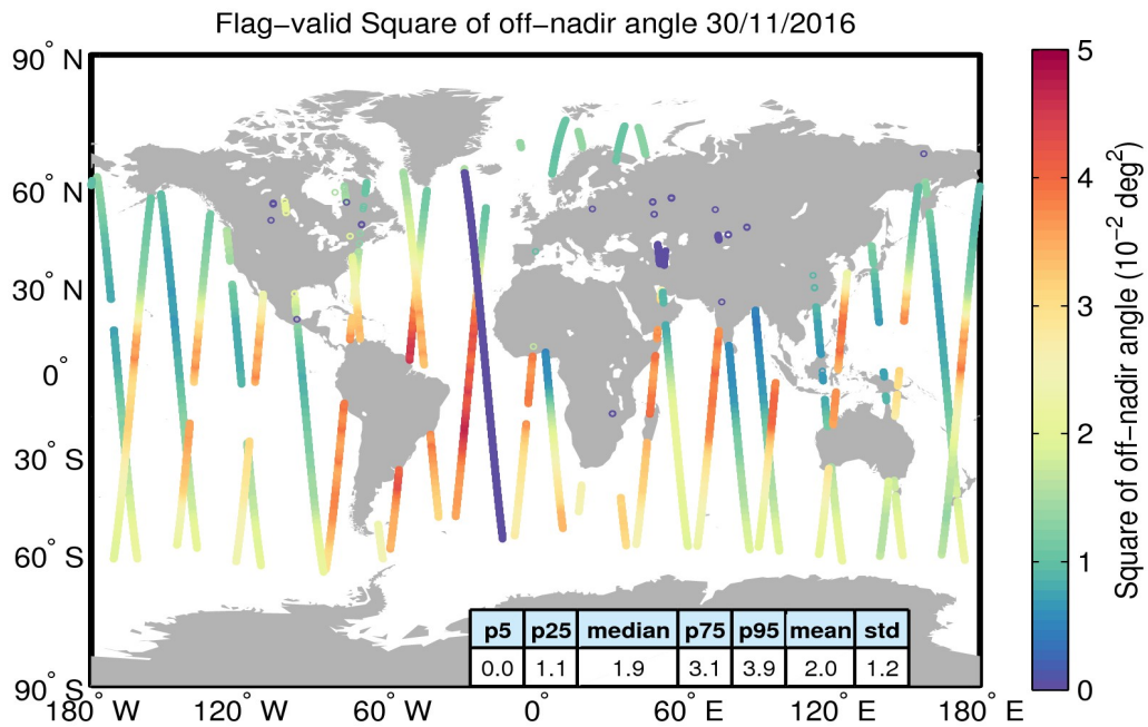
Figure 37. Geographical distribution of flag-valid mispointing data over oceans and lakes for 30/11/2016. The statistical values shown in the table refer to the mispointing in 10^{-2} deg 2 and are calculated over all measurements shown in the figure.
