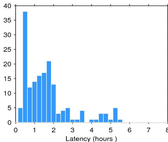
Figure 2. Histogram of the data latency for 30/11/2016. The y-axis denotes the number of files that are made available with a delay of x-hours with respect to the mean time of the records stored in the file.
