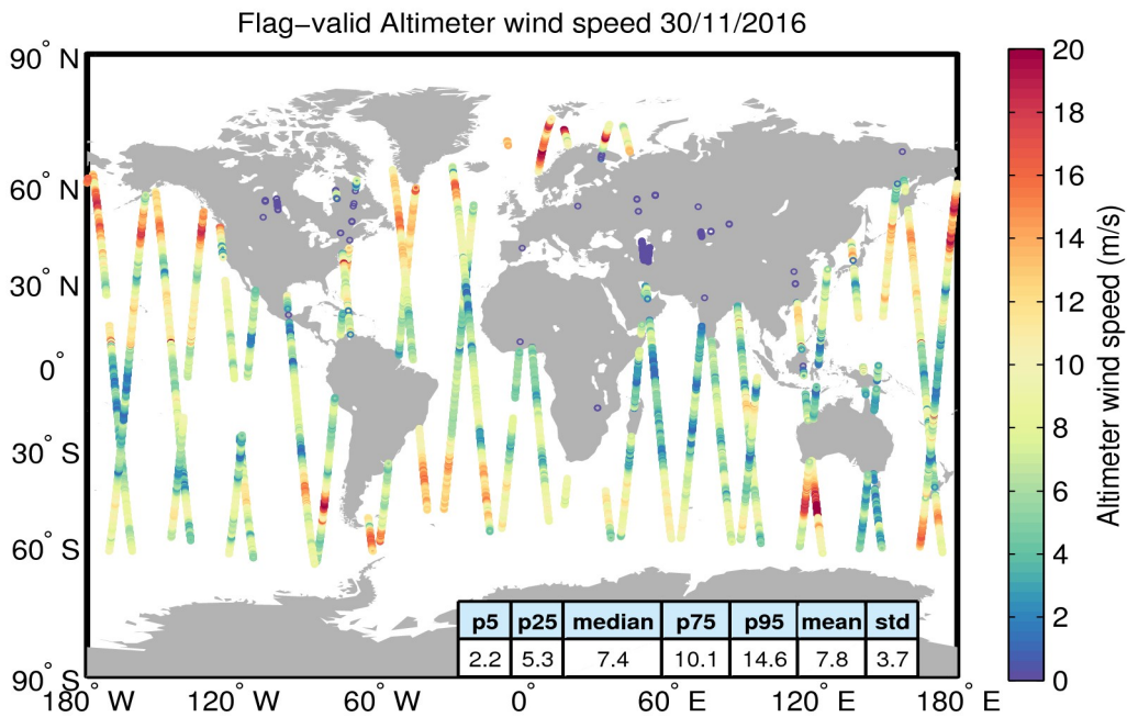
Figure 31. Geographical distribution of flag-valid wind data over oceans and lakes for 30/11/2016. The statistical values shown in the table refer to the wind in m/s and are calculated over all measurements shown in the figure.
