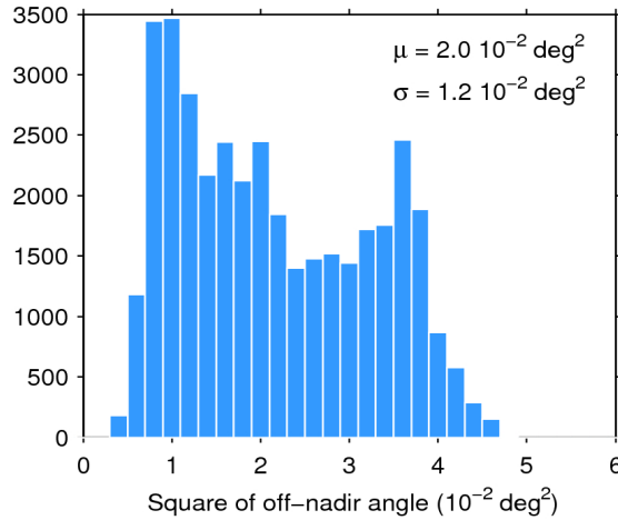
Figure 39. Histogram of flag-valid mispointing over oceans and lakes for 30/11/2016. The mean ( \mu ) and standard deviation ( \sigma ) are also shown. Note that values larger than 6 \cdot 10^{-2} \text{ deg}^2 are excluded from the histogram for the sake of readability but not from the computation of \mu and \sigma .
