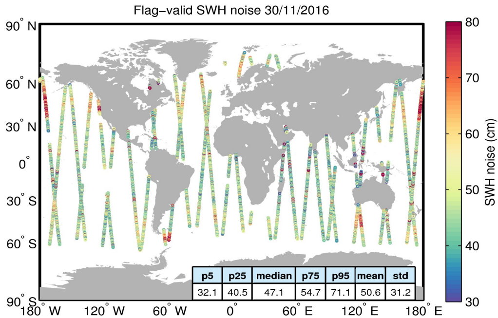
Figure 18. Geographical distribution of flag-valid 20-Hz SWH measurement noise over oceans and lakes for 30/11/2016. The statistical values shown in the table refer to the SWH noise and are calculated over all measurements shown in the figure.
