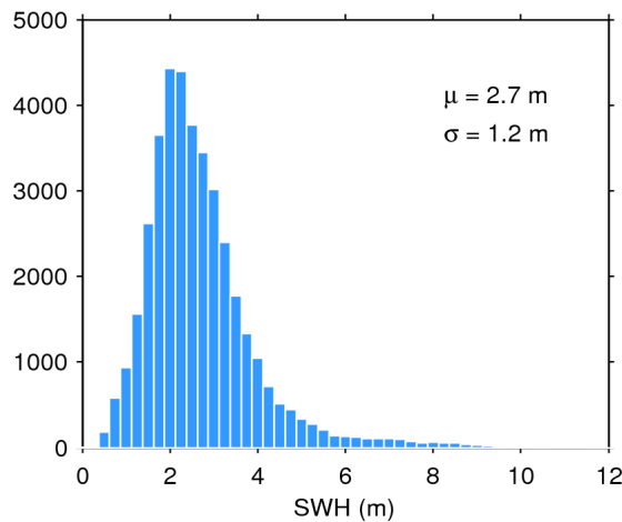
Figure 20. Histogram of science-valid SWH over oceans and lakes for 30/11/2016. The mean ( \mu ) and standard deviation ( \sigma ) are also shown. Note that values larger than 12 m are excluded from the histogram for the sake of readability but not from the computation of \mu and \sigma .
