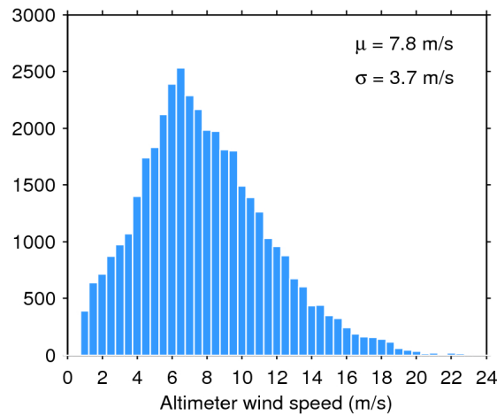
Figure 33. Histogram of flag-valid wind over oceans and lakes for 30/11/2016. The mean ( \mu ) and standard deviation ( \sigma ) are also shown. Note that values larger than 24 m/s are excluded from the histogram for the sake of readability but not from the computation of \mu and \sigma .
