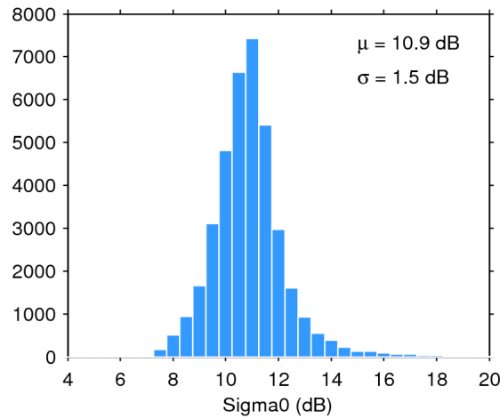
Figure 28. Histogram of science-valid sigma0 over oceans and lakes for 30/11/2016. The mean ( \mu ) and standard deviation ( \sigma ) are also shown. Note that values outside [4 20] dB are excluded from the histogram for the sake of readability but not from the computation of \mu and \sigma .
