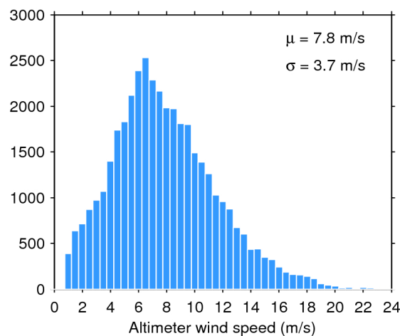
Figure 35. Histogram of science-valid wind over oceans and lakes for 30/11/2016. The mean ( \mu ) and standard deviation ( \sigma ) are also shown. Note that values larger than 24 m/s are excluded from the histogram for the sake of readability but not from the computation of \mu and \sigma .
