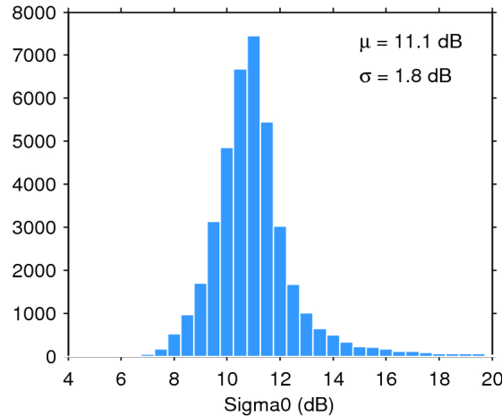
Figure 25. Histogram of flag-valid sigma0 over oceans and lakes for 30/11/2016. The mean ( \mu ) and standard deviation ( \sigma ) are also shown. Note that values outside [4 20] dB are excluded from the histogram for the sake of readability but not from the computation of \mu and \sigma .
