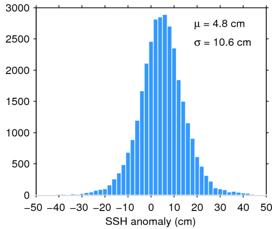
Figure 11. Histogram of science-valid SSH anomaly over oceans and lakes for 30/11/2016. The mean ( \mu ) and standard deviation ( \sigma ) are also shown. Note that values outside [-50 50] cm are excluded from the histogram for the sake of readability but not from the computation of \mu and \sigma .
