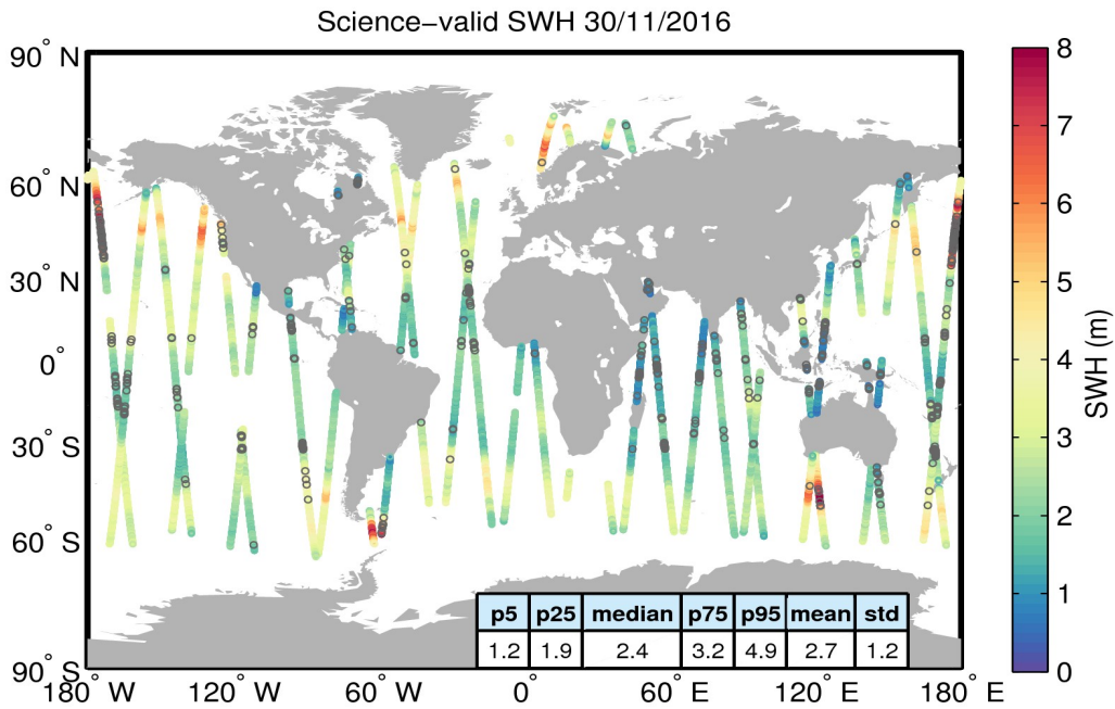
Figure 19. Geographical distribution of science-valid SWH data over oceans and lakes for 30/11/2016. The statistical values shown in the table refer to the SWH in m and are calculated over all measurements shown in the figure. Gray circles denote records that have been rejected based on the editing criteria described in Table 3.
