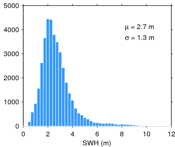
Figure 17. Histogram of flag-valid SWH over oceans and lakes for 30/11/2016. The mean ( \mu ) and standard deviation ( \sigma ) are also shown. Note that values larger than 12 m are excluded from the histogram for the sake of readability but not from the computation of \mu and \sigma .
