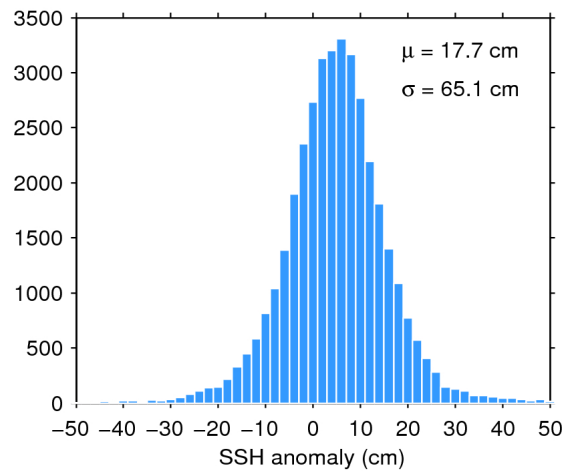
Figure 7. Histogram of flag-valid SSH anomaly over oceans and lakes for 30/11/2016. The mean ( \mu ) and standard deviation ( \sigma ) are also shown. Note that values outside [-50 50] cm are excluded from the histogram for the sake of readability but not from the computation of \mu and \sigma .
