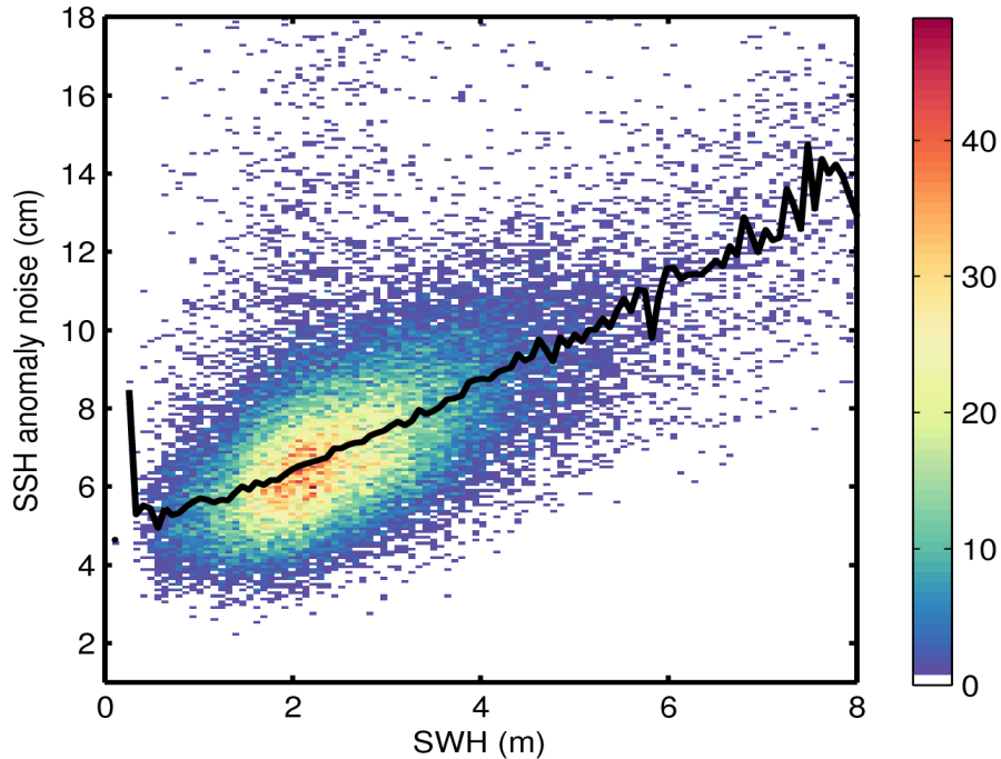
Figure 9. 2D histogram showing flag-valid SSH anomaly noise as a function of SWH for 30/11/2016. The black line denotes the median SSH anomaly noise as a function of SWH.
