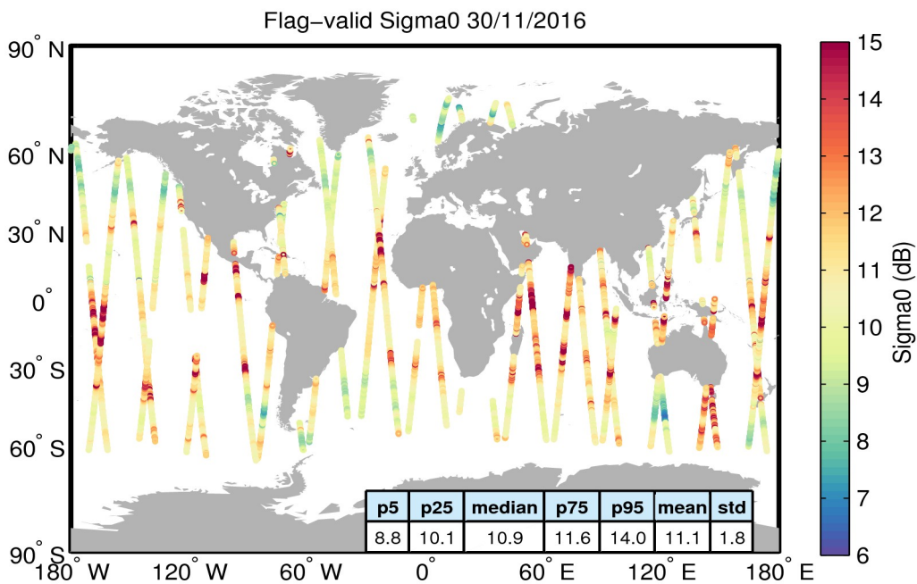
Figure 23. Geographical distribution of flag-valid sigma0 data over oceans and lakes for 30/11/2016. The statistical values shown in the table refer to the sigma0 in dB and are calculated over all measurements shown in the figure.
