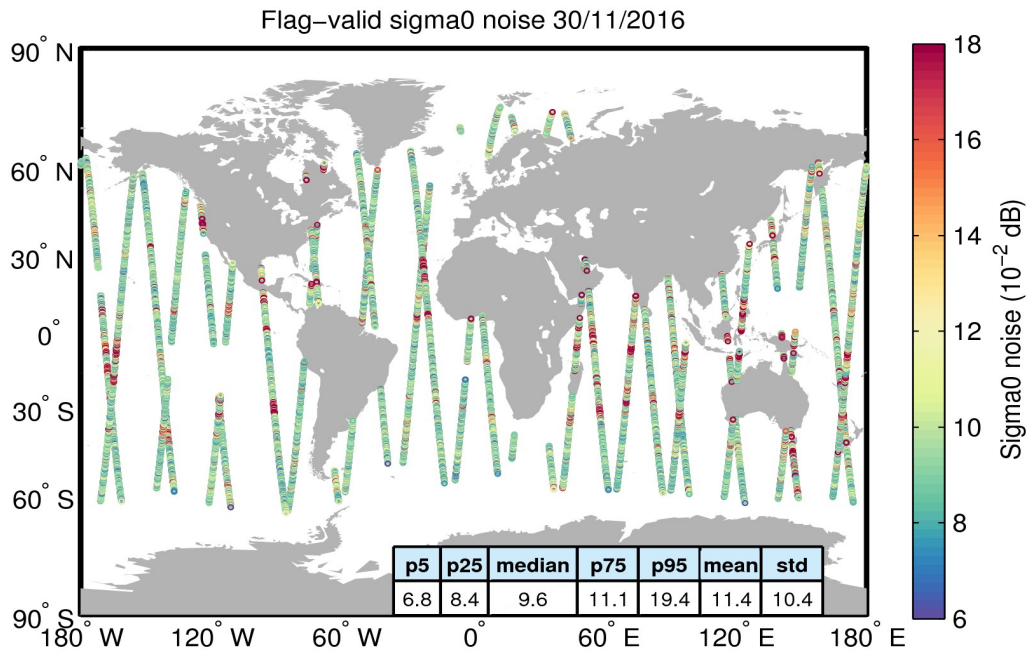
Figure 26. Geographical distribution of flag-valid 20-Hz sigma0 measurement noise over oceans and lakes for 30/11/2016. The statistical values shown in the table refer to the sigma0 noise and are calculated over all measurements shown in the figure.
