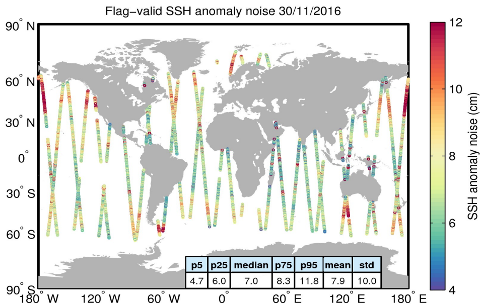
Figure 8. Geographical distribution of flag-valid 20-Hz SSH anomaly measurement noise over oceans and lakes for 30/11/2016. The statistical values shown in the table refer to the SSH anomaly noise and are calculated over all measurements shown in the figure.
