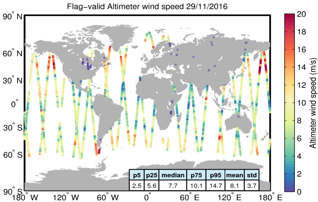
Figure 31. Geographical distribution of flag-valid wind data over oceans and lakes for 29/11/2016. The statistical values shown in the table refer to the wind in m/s and are calculated over all measurements shown in the figure.
