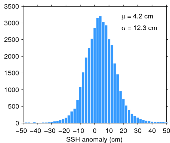
Figure 11. Histogram of science-valid SSH anomaly over oceans and lakes for 29/11/2016. The mean ( \mu ) and standard deviation ( \sigma ) are also shown. Note that values outside [-50 50] cm are excluded from the histogram for the sake of readability but not from the computation of \mu and \sigma .
