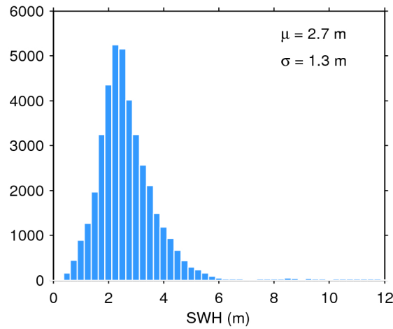
Figure 17. Histogram of flag-valid SWH over oceans and lakes for 29/11/2016. The mean ( \mu ) and standard deviation ( \sigma ) are also shown. Note that values larger than 12 m are excluded from the histogram for the sake of readability but not from the computation of \mu and \sigma .
