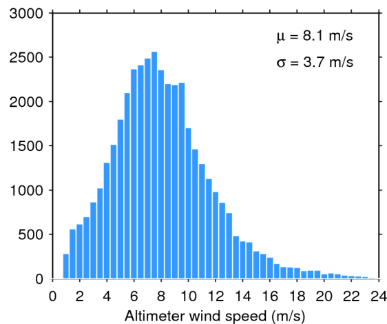
Figure 35. Histogram of science-valid wind over oceans and lakes for 29/11/2016. The mean ( \mu ) and standard deviation ( \sigma ) are also shown. Note that values larger than 24 m/s are excluded from the histogram for the sake of readability but not from the computation of \mu and \sigma .
