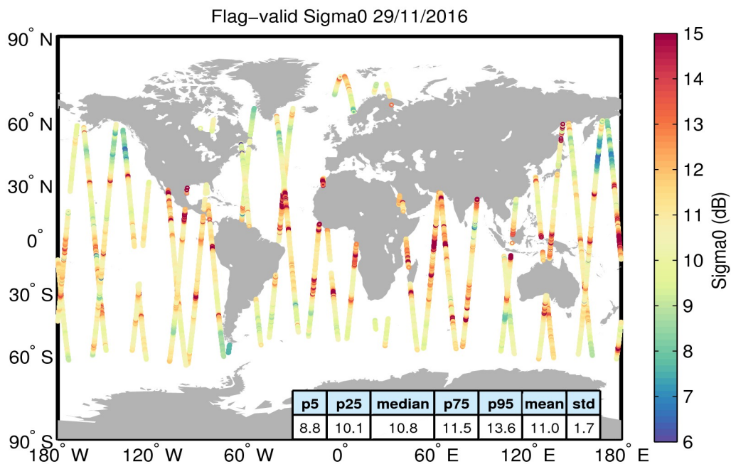
Figure 23. Geographical distribution of flag-valid sigma0 data over oceans and lakes for 29/11/2016. The statistical values shown in the table refer to the sigma0 in dB and are calculated over all measurements shown in the figure.
