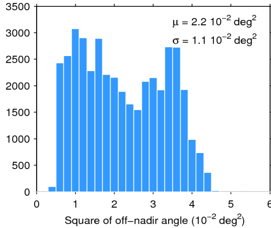
Figure 39. Histogram of flag-valid mispointing over oceans and lakes for 29/11/2016. The mean ( \mu ) and standard deviation ( \sigma ) are also shown. Note that values larger than 6 \cdot 10^{-2} \text{ deg}^2 are excluded from the histogram for the sake of readability but not from the computation of \mu and \sigma .
