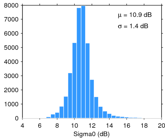
Figure 28. Histogram of science-valid sigma0 over oceans and lakes for 29/11/2016. The mean ( \mu ) and standard deviation ( \sigma ) are also shown. Note that values outside [4 20] dB are excluded from the histogram for the sake of readability but not from the computation of \mu and \sigma .
