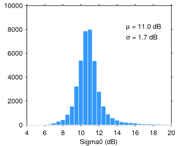
Figure 25. Histogram of flag-valid sigma0 over oceans and lakes for 29/11/2016. The mean ( \mu ) and standard deviation ( \sigma ) are also shown. Note that values outside [4 20] dB are excluded from the histogram for the sake of readability but not from the computation of \mu and \sigma .
