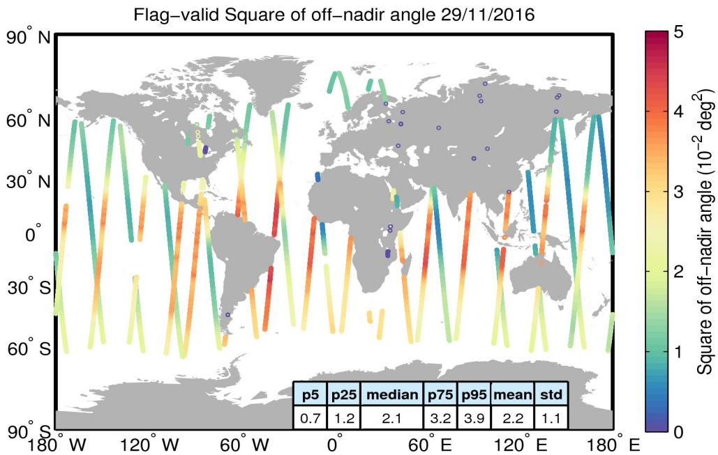
Figure 37. Geographical distribution of flag-valid mispointing data over oceans and lakes for 29/11/2016. The statistical values shown in the table refer to the mispointing in 10^{-2} deg 2 and are calculated over all measurements shown in the figure.
