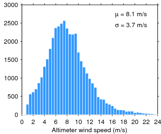
Figure 33. Histogram of flag-valid wind over oceans and lakes for 29/11/2016. The mean ( \mu ) and standard deviation ( \sigma ) are also shown. Note that values larger than 24 m/s are excluded from the histogram for the sake of readability but not from the computation of \mu and \sigma .
