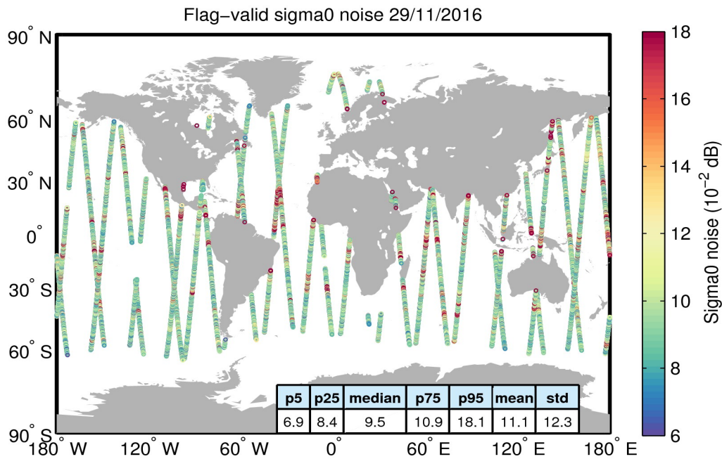
Figure 26. Geographical distribution of flag-valid 20-Hz sigma0 measurement noise over oceans and lakes for 29/11/2016. The statistical values shown in the table refer to the sigma0 noise and are calculated over all measurements shown in the figure.
