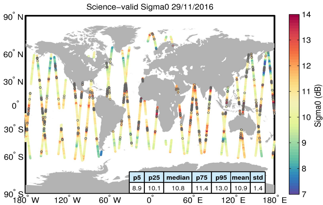
Figure 27. Geographical distribution of science-valid sigma0 data over oceans and lakes for 29/11/2016. The statistical values shown in the table refer to the sigma0 in dB and are calculated over all measurements shown in the figure. Gray circles denote records that have been rejected based on the editing criteria described in Table 4.
