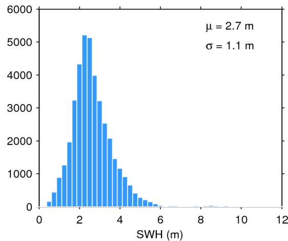
Figure 20. Histogram of science-valid SWH over oceans and lakes for 29/11/2016. The mean ( \mu ) and standard deviation ( \sigma ) are also shown. Note that values larger than 12 m are excluded from the histogram for the sake of readability but not from the computation of \mu and \sigma .
