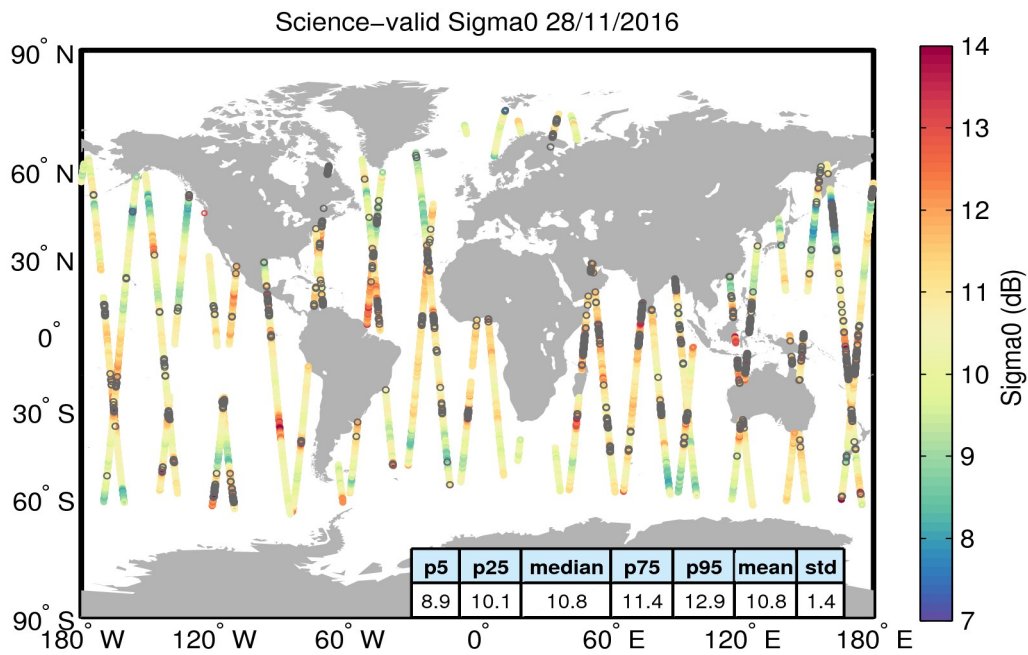
Figure 27. Geographical distribution of science-valid sigma0 data over oceans and lakes for 28/11/2016. The statistical values shown in the table refer to the sigma0 in dB and are calculated over all measurements shown in the figure. Gray circles denote records that have been rejected based on the editing criteria described in Table 4.
