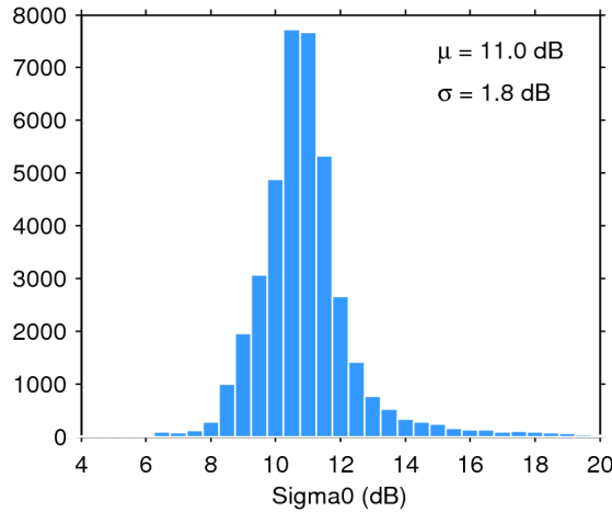
Figure 25. Histogram of flag-valid sigma0 over oceans and lakes for 28/11/2016. The mean ( \mu ) and standard deviation ( \sigma ) are also shown. Note that values outside [4 20] dB are excluded from the histogram for the sake of readability but not from the computation of \mu and \sigma .
