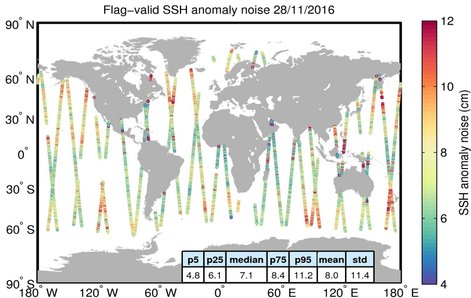
Figure 8. Geographical distribution of flag-valid 20-Hz SSH anomaly measurement noise over oceans and lakes for 28/11/2016. The statistical values shown in the table refer to the SSH anomaly noise and are calculated over all measurements shown in the figure.
