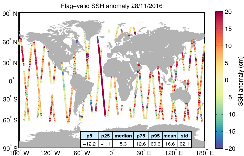
Figure 5. Geographical distribution of flag-valid 1-Hz SSH anomaly data over oceans and lakes for 28/11/2016. The statistical values shown in the table refer to the SSH anomaly in cm and are calculated over all measurements shown in the figure.
