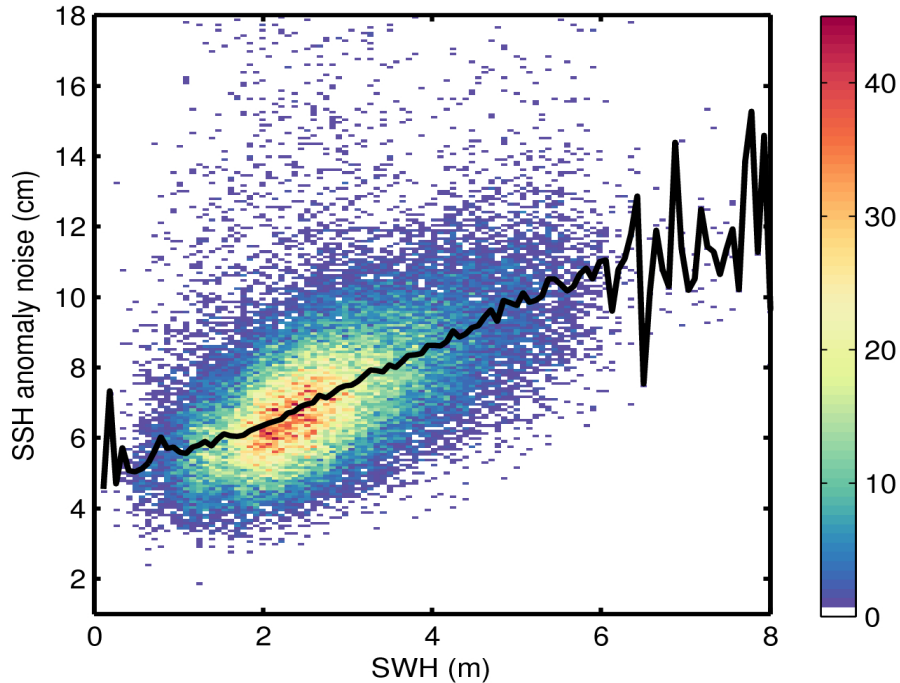
Figure 9. 2D histogram showing flag-valid SSH anomaly noise as a function of SWH for 28/11/2016. The black line denotes the median SSH anomaly noise as a function of SWH.
