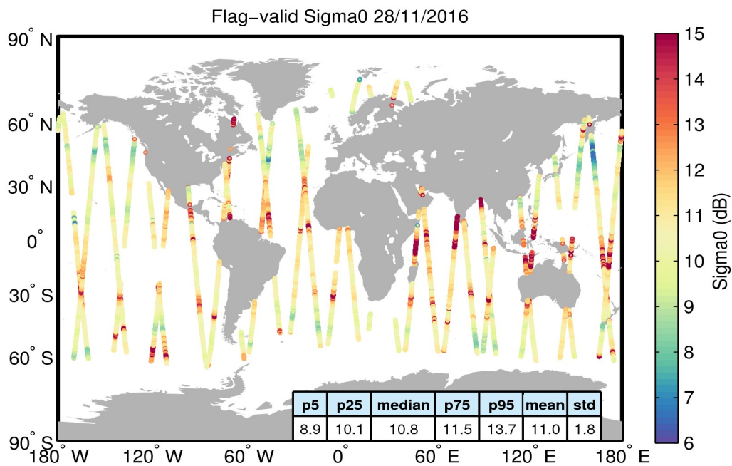
Figure 23. Geographical distribution of flag-valid sigma0 data over oceans and lakes for 28/11/2016. The statistical values shown in the table refer to the sigma0 in dB and are calculated over all measurements shown in the figure.
