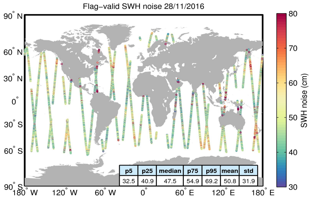
Figure 18. Geographical distribution of flag-valid 20-Hz SWH measurement noise over oceans and lakes for 28/11/2016. The statistical values shown in the table refer to the SWH noise and are calculated over all measurements shown in the figure.
