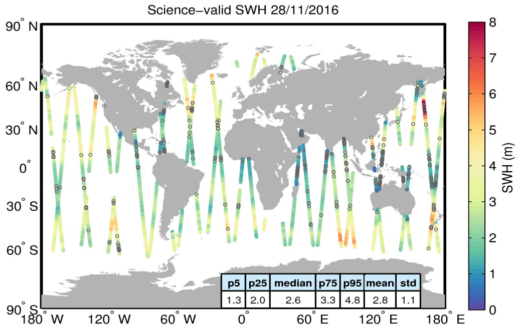
Figure 19. Geographical distribution of science-valid SWH data over oceans and lakes for 28/11/2016. The statistical values shown in the table refer to the SWH in m and are calculated over all measurements shown in the figure. Gray circles denote records that have been rejected based on the editing criteria described in Table 3.
