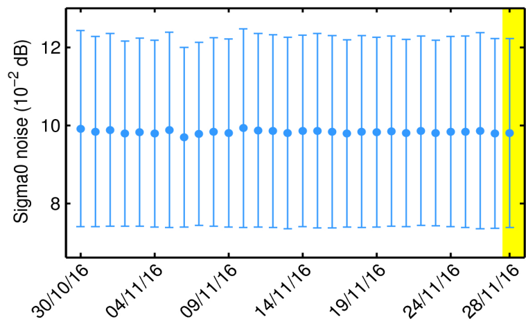
Figure 30. Average science-valid sigma0 noise (blue dot) and the corresponding standard deviation (error bar) for each day in last 30-day window. The yellow shading highlights the day analyzed in this report.
