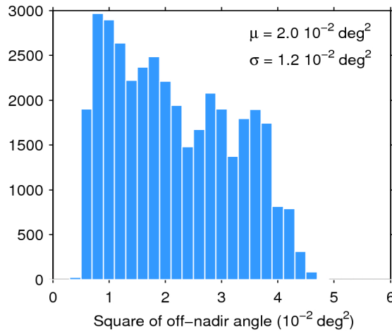
Figure 39. Histogram of flag-valid mispointing over oceans and lakes for 28/11/2016. The mean ( \mu ) and standard deviation ( \sigma ) are also shown. Note that values larger than 6 \cdot 10^{-2} \text{ deg}^2 are excluded from the histogram for the sake of readability but not from the computation of \mu and \sigma .
