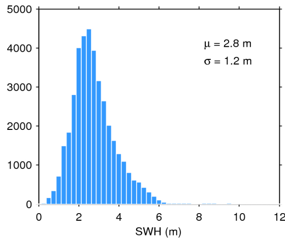
Figure 17. Histogram of flag-valid SWH over oceans and lakes for 28/11/2016. The mean ( \mu ) and standard deviation ( \sigma ) are also shown. Note that values larger than 12 m are excluded from the histogram for the sake of readability but not from the computation of \mu and \sigma .
