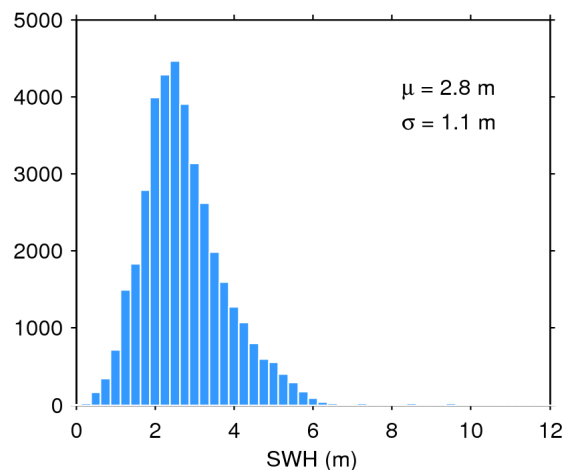
Figure 20. Histogram of science-valid SWH over oceans and lakes for 28/11/2016. The mean ( \mu ) and standard deviation ( \sigma ) are also shown. Note that values larger than 12 m are excluded from the histogram for the sake of readability but not from the computation of \mu and \sigma .
