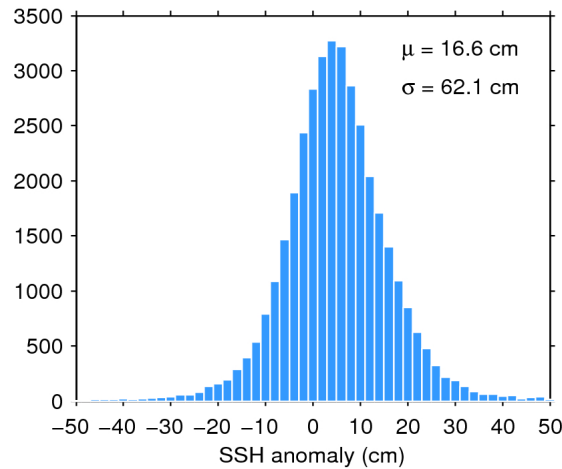
Figure 7. Histogram of flag-valid SSH anomaly over oceans and lakes for 28/11/2016. The mean ( \mu ) and standard deviation ( \sigma ) are also shown. Note that values outside [-50 50] cm are excluded from the histogram for the sake of readability but not from the computation of \mu and \sigma .
