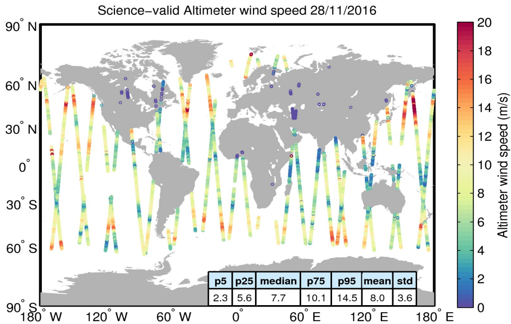
Figure 34. Geographical distribution of science-valid wind data over oceans and lakes for 28/11/2016. The statistical values shown in the table refer to the wind in m/s and are calculated over all measurements shown in the figure. Gray circles denote records that have been rejected based on the editing criteria described in Table 5.
