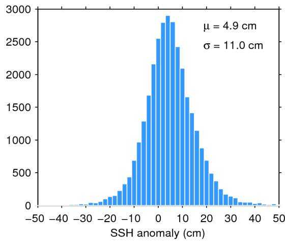
Figure 11. Histogram of science-valid SSH anomaly over oceans and lakes for 28/11/2016. The mean ( \mu ) and standard deviation ( \sigma ) are also shown. Note that values outside [-50 50] cm are excluded from the histogram for the sake of readability but not from the computation of \mu and \sigma .
