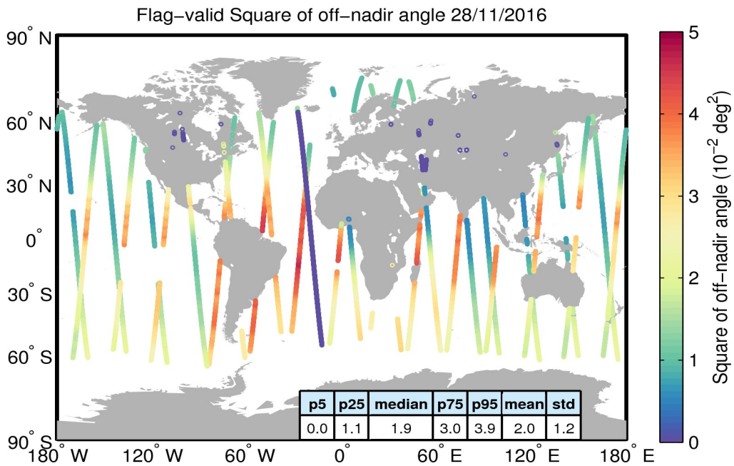
Figure 37. Geographical distribution of flag-valid mispointing data over oceans and lakes for 28/11/2016. The statistical values shown in the table refer to the mispointing in 10^{-2} deg 2 and are calculated over all measurements shown in the figure.
