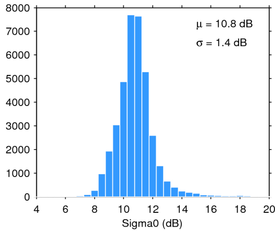
Figure 28. Histogram of science-valid sigma0 over oceans and lakes for 28/11/2016. The mean ( \mu ) and standard deviation ( \sigma ) are also shown. Note that values outside [4 20] dB are excluded from the histogram for the sake of readability but not from the computation of \mu and \sigma .
