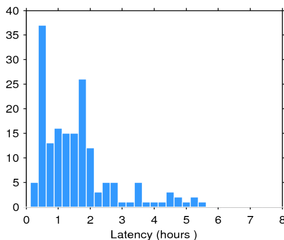
Figure 2. Histogram of the data latency for 28/11/2016. The y-axis denotes the number of files that are made available with a delay of x-hours with respect to the mean time of the records stored in the file.
