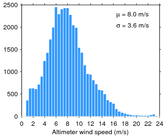
Figure 33. Histogram of flag-valid wind over oceans and lakes for 28/11/2016. The mean ( \mu ) and standard deviation ( \sigma ) are also shown. Note that values larger than 24 m/s are excluded from the histogram for the sake of readability but not from the computation of \mu and \sigma .
