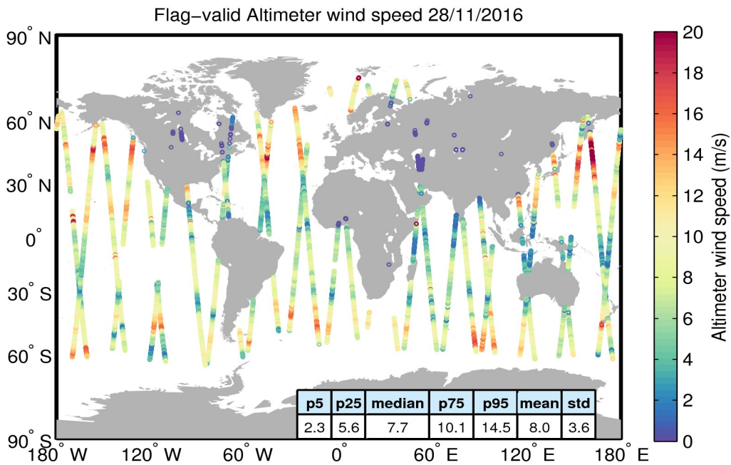
Figure 31. Geographical distribution of flag-valid wind data over oceans and lakes for 28/11/2016. The statistical values shown in the table refer to the wind in m/s and are calculated over all measurements shown in the figure.
