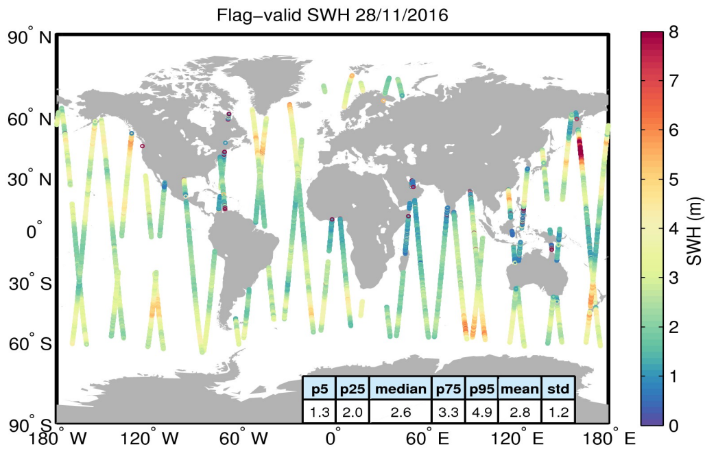
Figure 15. Geographical distribution of flag-valid SWH data over oceans and lakes for 28/11/2016. The statistical values shown in the table refer to the SWH in m and are calculated over all measurements shown in the figure.
