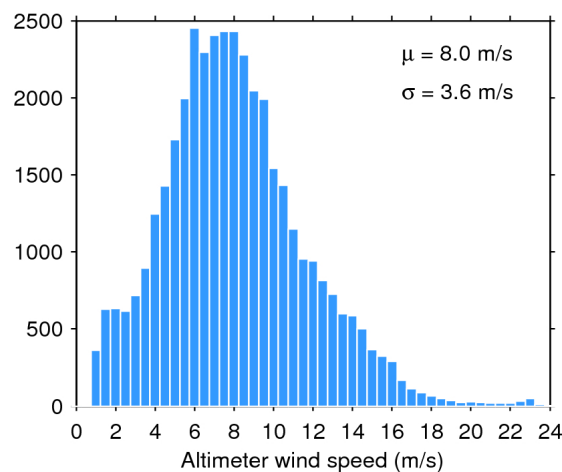
Figure 35. Histogram of science-valid wind over oceans and lakes for 28/11/2016. The mean ( \mu ) and standard deviation ( \sigma ) are also shown. Note that values larger than 24 m/s are excluded from the histogram for the sake of readability but not from the computation of \mu and \sigma .
