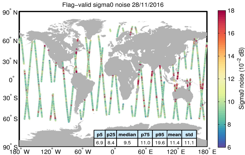
Figure 26. Geographical distribution of flag-valid 20-Hz sigma0 measurement noise over oceans and lakes for 28/11/2016. The statistical values shown in the table refer to the sigma0 noise and are calculated over all measurements shown in the figure.
