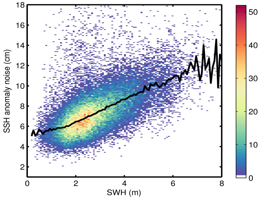
Figure 9. 2D histogram showing flag-valid SSH anomaly noise as a function of SWH for 27/11/2016. The black line denotes the median SSH anomaly noise as a function of SWH.
