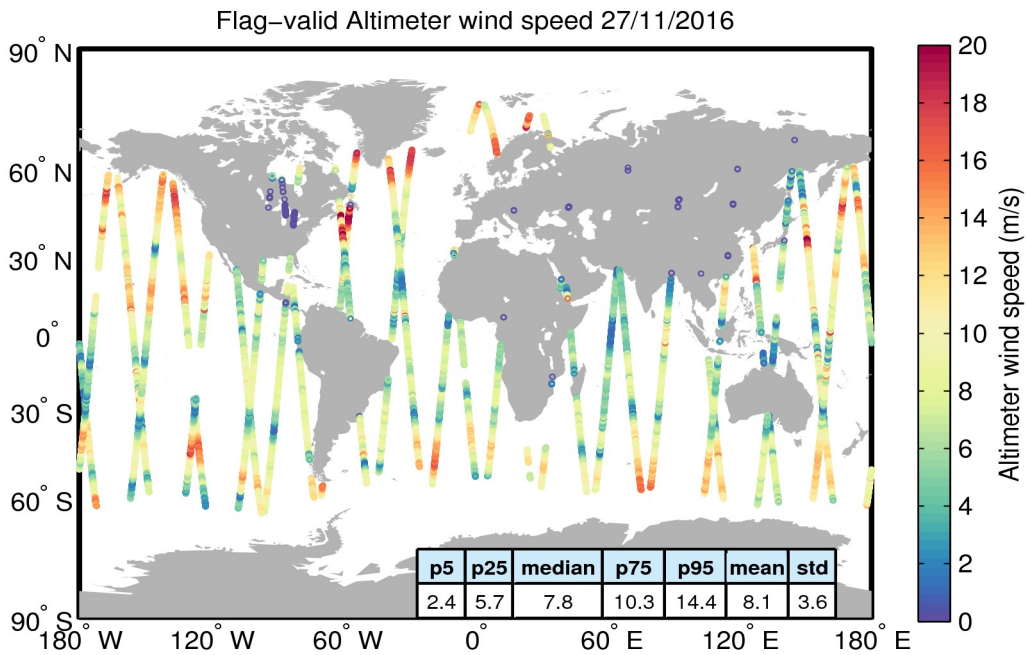
Figure 31. Geographical distribution of flag-valid wind data over oceans and lakes for 27/11/2016. The statistical values shown in the table refer to the wind in m/s and are calculated over all measurements shown in the figure.
