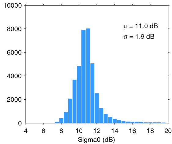
Figure 25. Histogram of flag-valid sigma0 over oceans and lakes for 27/11/2016. The mean ( \mu ) and standard deviation ( \sigma ) are also shown. Note that values outside [4 20] dB are excluded from the histogram for the sake of readability but not from the computation of \mu and \sigma .
