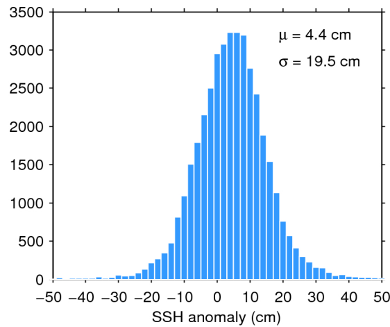
Figure 7. Histogram of flag-valid SSH anomaly over oceans and lakes for 27/11/2016. The mean ( \mu ) and standard deviation ( \sigma ) are also shown. Note that values outside [-50\ 50] cm are excluded from the histogram for the sake of readability but not from the computation of \mu and \sigma .
