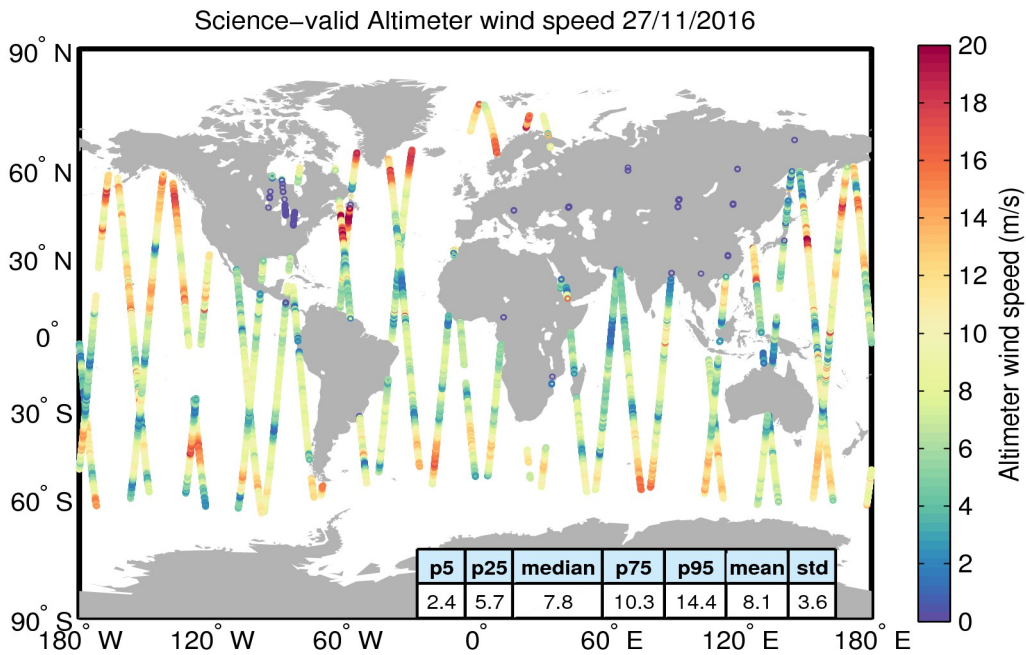
Figure 34. Geographical distribution of science-valid wind data over oceans and lakes for 27/11/2016. The statistical values shown in the table refer to the wind in m/s and are calculated over all measurements shown in the figure. Gray circles denote records that have been rejected based on the editing criteria described in Table 5.
