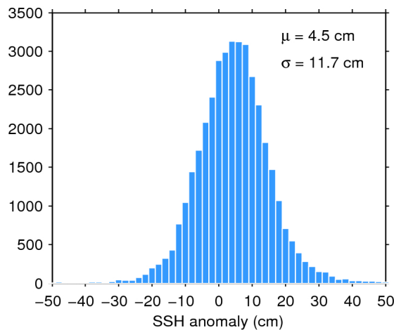
Figure 11. Histogram of science-valid SSH anomaly over oceans and lakes for 27/11/2016. The mean ( \mu ) and standard deviation ( \sigma ) are also shown. Note that values outside [-50 50] cm are excluded from the histogram for the sake of readability but not from the computation of \mu and \sigma .
