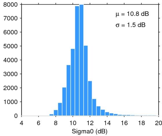
Figure 28. Histogram of science-valid sigma0 over oceans and lakes for 27/11/2016. The mean ( \mu ) and standard deviation ( \sigma ) are also shown. Note that values outside [4 20] dB are excluded from the histogram for the sake of readability but not from the computation of \mu and \sigma .
