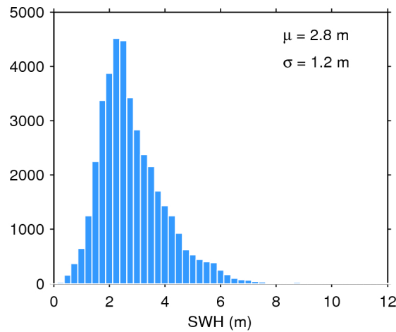
Figure 17. Histogram of flag-valid SWH over oceans and lakes for 27/11/2016. The mean ( \mu ) and standard deviation ( \sigma ) are also shown. Note that values larger than 12 m are excluded from the histogram for the sake of readability but not from the computation of \mu and \sigma .
