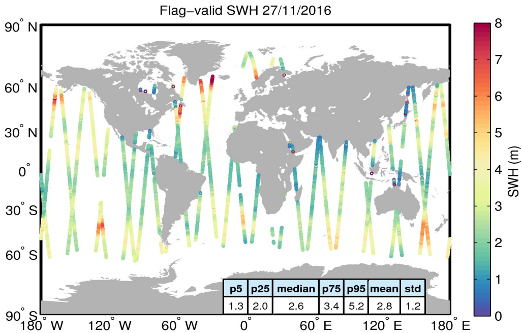
Figure 15. Geographical distribution of flag-valid SWH data over oceans and lakes for 27/11/2016. The statistical values shown in the table refer to the SWH in m and are calculated over all measurements shown in the figure.
