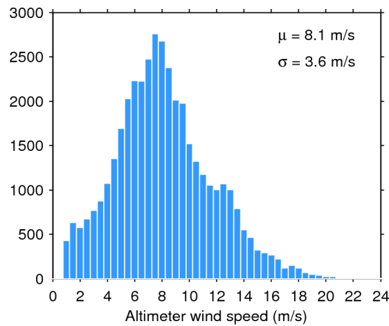
Figure 33. Histogram of flag-valid wind over oceans and lakes for 27/11/2016. The mean ( \mu ) and standard deviation ( \sigma ) are also shown. Note that values larger than 24 m/s are excluded from the histogram for the sake of readability but not from the computation of \mu and \sigma .
