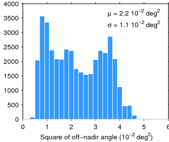
Figure 39. Histogram of flag-valid mispointing over oceans and lakes for 27/11/2016. The mean ( \mu ) and standard deviation ( \sigma ) are also shown. Note that values larger than 6 \cdot 10^{-2} \text{ deg}^2 are excluded from the histogram for the sake of readability but not from the computation of \mu and \sigma .
