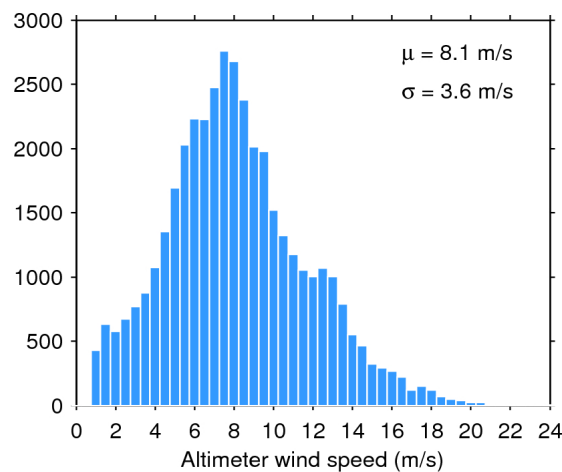
Figure 35. Histogram of science-valid wind over oceans and lakes for 27/11/2016. The mean ( \mu ) and standard deviation ( \sigma ) are also shown. Note that values larger than 24 m/s are excluded from the histogram for the sake of readability but not from the computation of \mu and \sigma .
