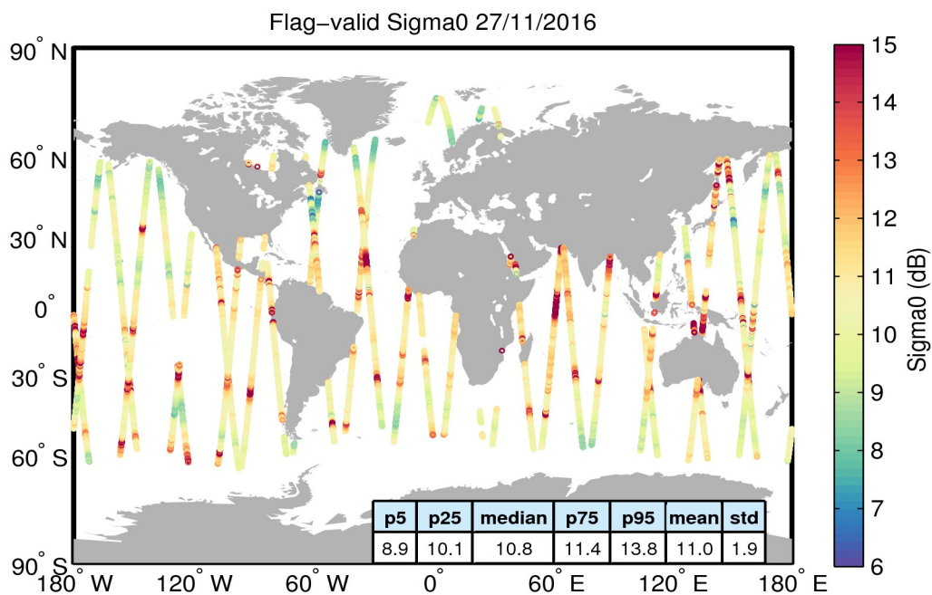
Figure 23. Geographical distribution of flag-valid sigma0 data over oceans and lakes for 27/11/2016. The statistical values shown in the table refer to the sigma0 in dB and are calculated over all measurements shown in the figure.
