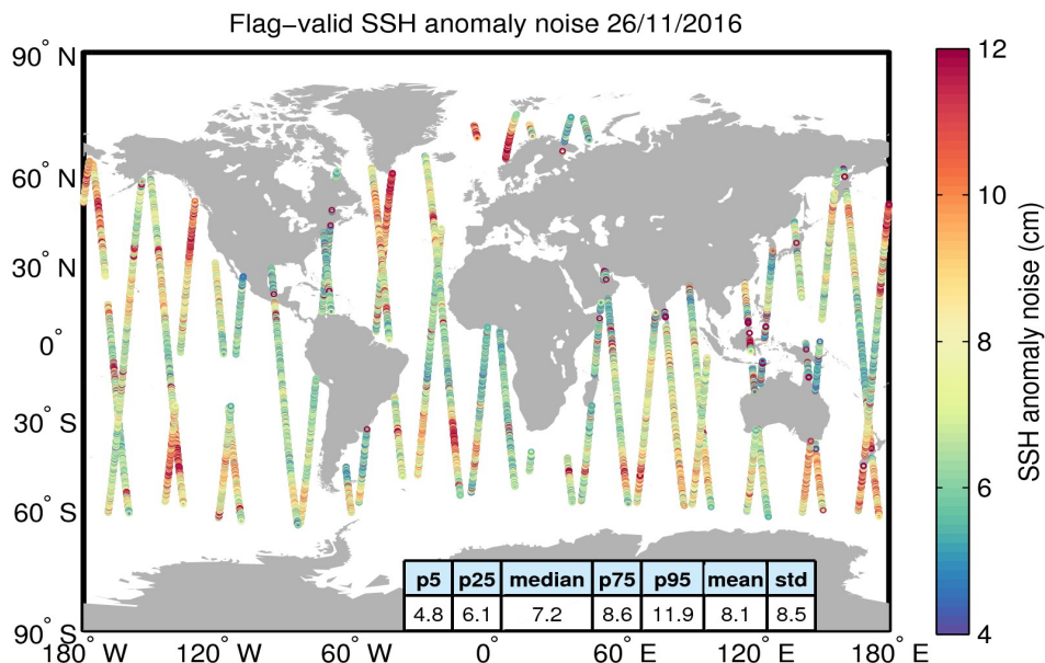
Figure 8. Geographical distribution of flag-valid 20-Hz SSH anomaly measurement noise over oceans and lakes for 26/11/2016. The statistical values shown in the table refer to the SSH anomaly noise and are calculated over all measurements shown in the figure.
