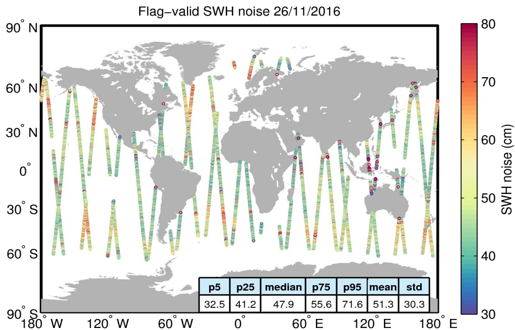
Figure 18. Geographical distribution of flag-valid 20-Hz SWH measurement noise over oceans and lakes for 26/11/2016. The statistical values shown in the table refer to the SWH noise and are calculated over all measurements shown in the figure.
