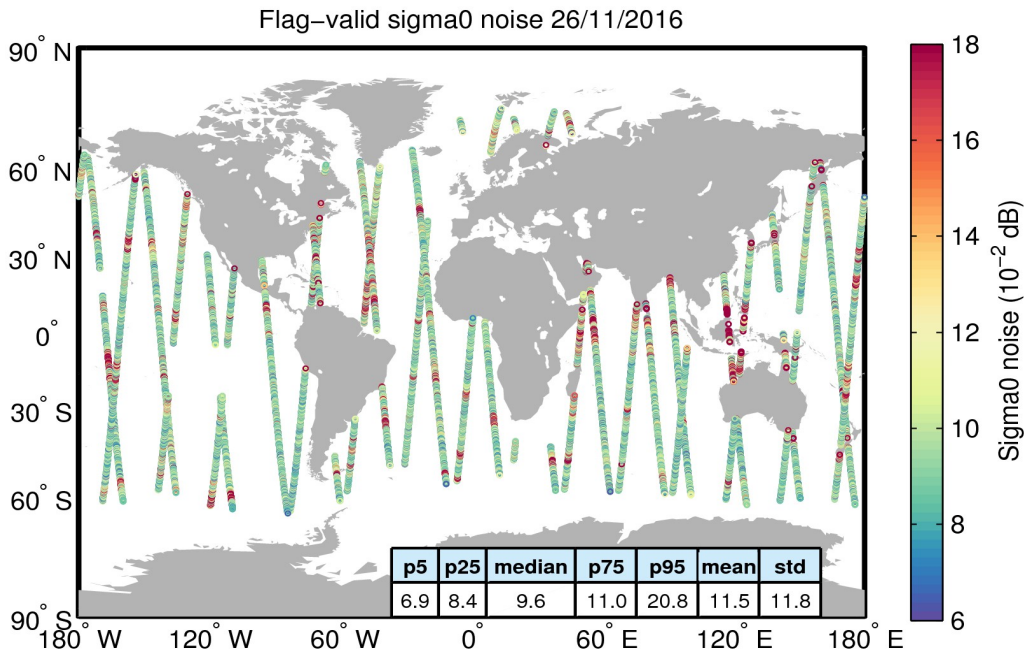
Figure 26. Geographical distribution of flag-valid 20-Hz sigma0 measurement noise over oceans and lakes for 26/11/2016. The statistical values shown in the table refer to the sigma0 noise and are calculated over all measurements shown in the figure.
