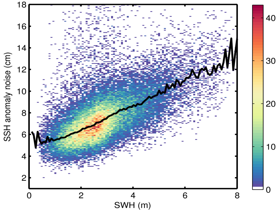
Figure 9. 2D histogram showing flag-valid SSH anomaly noise as a function of SWH for 26/11/2016. The black line denotes the median SSH anomaly noise as a function of SWH.
