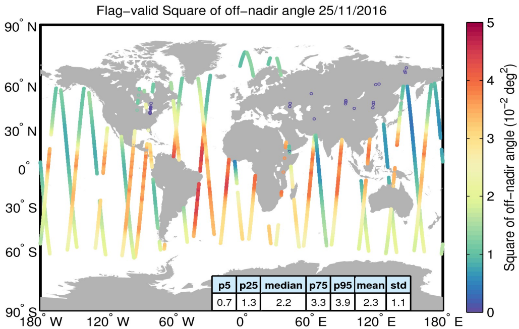
Figure 37. Geographical distribution of flag-valid mispointing data over oceans and lakes for 25/11/2016. The statistical values shown in the table refer to the mispointing in 10^{-2} deg 2 and are calculated over all measurements shown in the figure.
