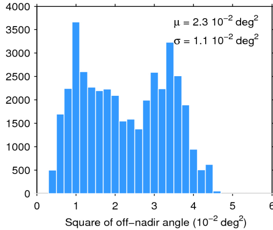
Figure 39. Histogram of flag-valid mispointing over oceans and lakes for 25/11/2016. The mean ( \mu ) and standard deviation ( \sigma ) are also shown. Note that values larger than 6 \cdot 10^{-2} \text{ deg}^2 are excluded from the histogram for the sake of readability but not from the computation of \mu and \sigma .
