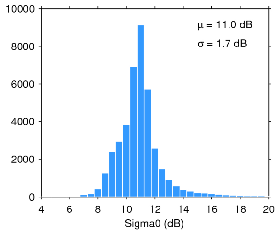
Figure 25. Histogram of flag-valid sigma0 over oceans and lakes for 25/11/2016. The mean ( \mu ) and standard deviation ( \sigma ) are also shown. Note that values outside [4 20] dB are excluded from the histogram for the sake of readability but not from the computation of \mu and \sigma .
