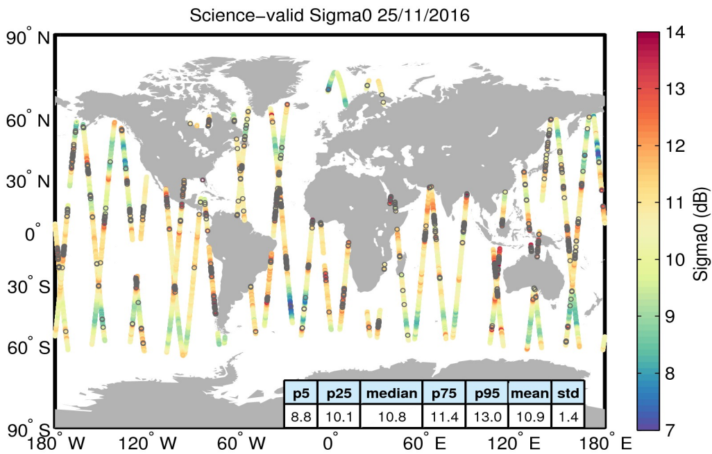
Figure 27. Geographical distribution of science-valid sigma0 data over oceans and lakes for 25/11/2016. The statistical values shown in the table refer to the sigma0 in dB and are calculated over all measurements shown in the figure. Gray circles denote records that have been rejected based on the editing criteria described in Table 4.
