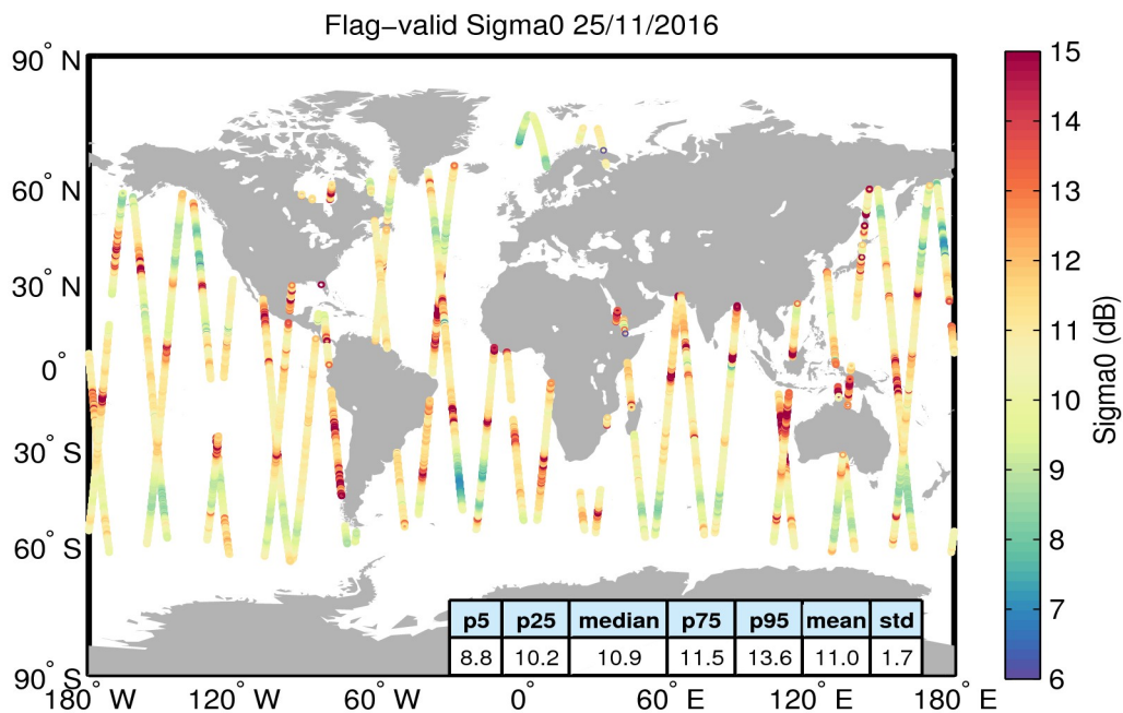
Figure 23. Geographical distribution of flag-valid sigma0 data over oceans and lakes for 25/11/2016. The statistical values shown in the table refer to the sigma0 in dB and are calculated over all measurements shown in the figure.
