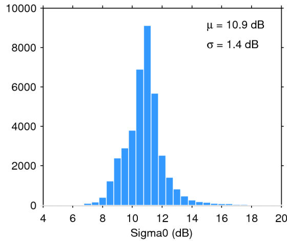
Figure 28. Histogram of science-valid sigma0 over oceans and lakes for 25/11/2016. The mean ( \mu ) and standard deviation ( \sigma ) are also shown. Note that values outside [4 20] dB are excluded from the histogram for the sake of readability but not from the computation of \mu and \sigma .
