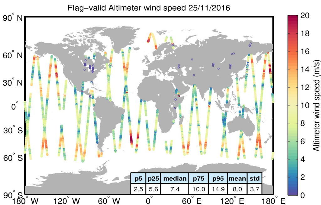
Figure 31. Geographical distribution of flag-valid wind data over oceans and lakes for 25/11/2016. The statistical values shown in the table refer to the wind in m/s and are calculated over all measurements shown in the figure.
