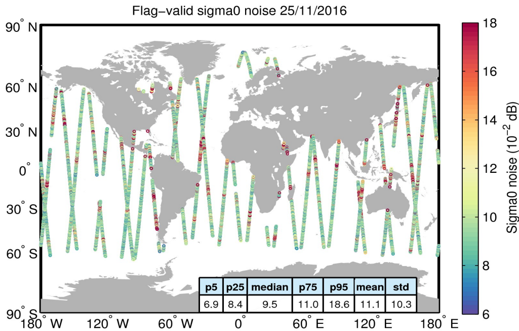
Figure 26. Geographical distribution of flag-valid 20-Hz sigma0 measurement noise over oceans and lakes for 25/11/2016. The statistical values shown in the table refer to the sigma0 noise and are calculated over all measurements shown in the figure.
