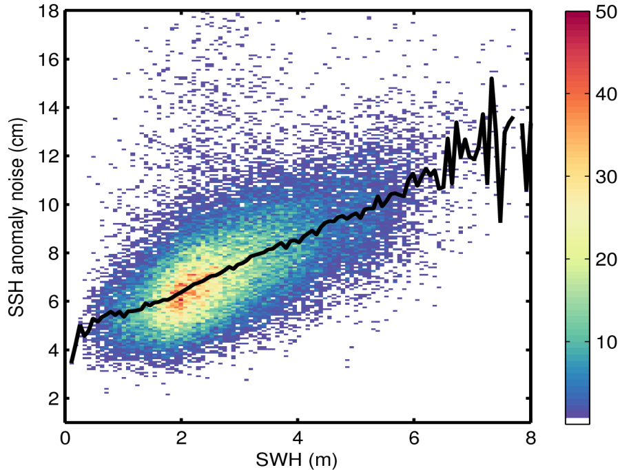
Figure 9. 2D histogram showing flag-valid SSH anomaly noise as a function of SWH for 25/11/2016. The black line denotes the median SSH anomaly noise as a function of SWH.
