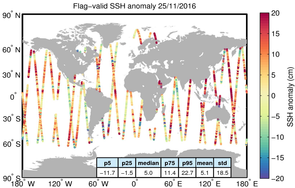
Figure 5. Geographical distribution of flag-valid 1-Hz SSH anomaly data over oceans and lakes for 25/11/2016. The statistical values shown in the table refer to the SSH anomaly in cm and are calculated over all measurements shown in the figure.
