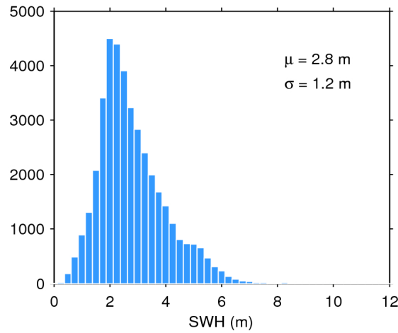
Figure 17. Histogram of flag-valid SWH over oceans and lakes for 25/11/2016. The mean ( \mu ) and standard deviation ( \sigma ) are also shown. Note that values larger than 12 m are excluded from the histogram for the sake of readability but not from the computation of \mu and \sigma .
