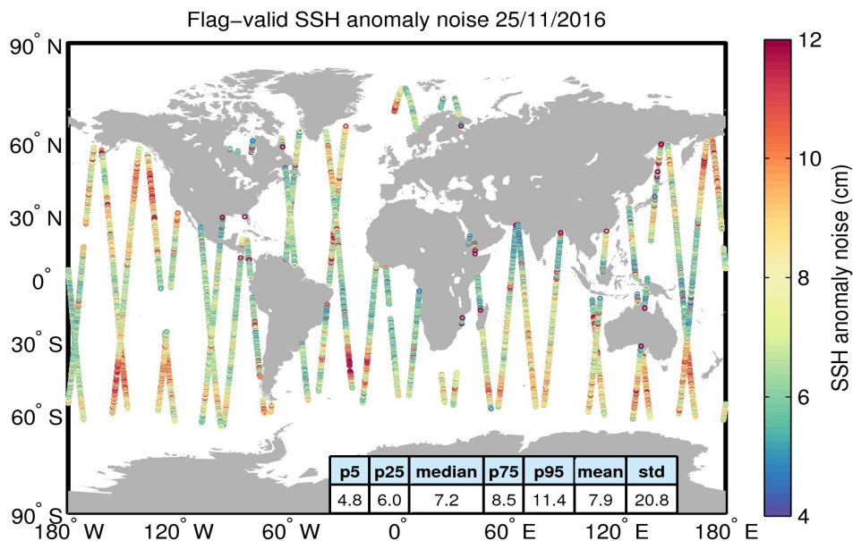
Figure 8. Geographical distribution of flag-valid 20-Hz SSH anomaly measurement noise over oceans and lakes for 25/11/2016. The statistical values shown in the table refer to the SSH anomaly noise and are calculated over all measurements shown in the figure.
