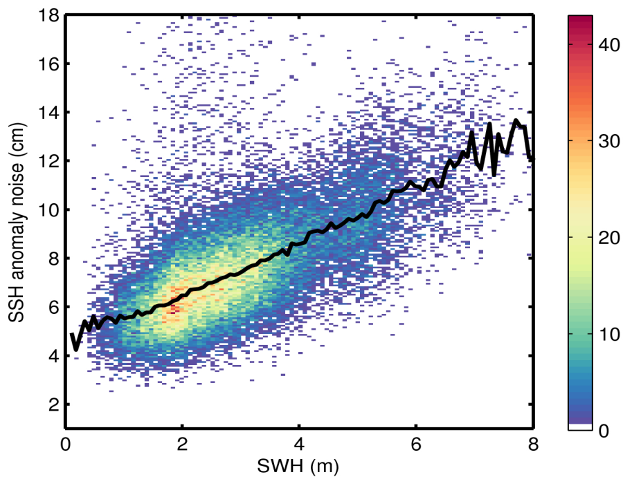
Figure 9. 2D histogram showing flag-valid SSH anomaly noise as a function of SWH for 23/11/2016. The black line denotes the median SSH anomaly noise as a function of SWH.
