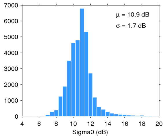
Figure 25. Histogram of flag-valid sigma0 over oceans and lakes for 23/11/2016. The mean ( \mu ) and standard deviation ( \sigma ) are also shown. Note that values outside [4 20] dB are excluded from the histogram for the sake of readability but not from the computation of \mu and \sigma .
