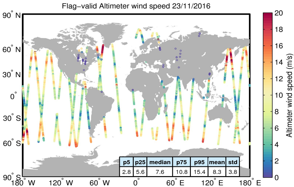
Figure 31. Geographical distribution of flag-valid wind data over oceans and lakes for 23/11/2016. The statistical values shown in the table refer to the wind in m/s and are calculated over all measurements shown in the figure.
