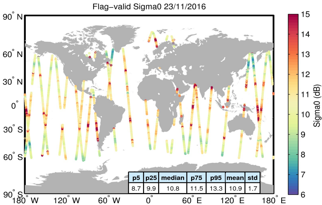
Figure 23. Geographical distribution of flag-valid sigma0 data over oceans and lakes for 23/11/2016. The statistical values shown in the table refer to the sigma0 in dB and are calculated over all measurements shown in the figure.
