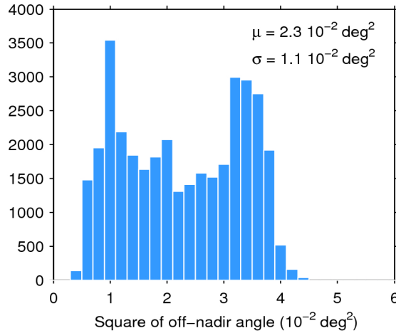
Figure 39. Histogram of flag-valid mispointing over oceans and lakes for 23/11/2016. The mean ( \mu ) and standard deviation ( \sigma ) are also shown. Note that values larger than 6 \cdot 10^{-2} \text{ deg}^2 are excluded from the histogram for the sake of readability but not from the computation of \mu and \sigma .
