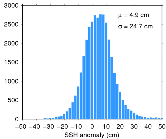
Figure 7. Histogram of flag-valid SSH anomaly over oceans and lakes for 23/11/2016. The mean ( \mu ) and standard deviation ( \sigma ) are also shown. Note that values outside [-50 50] cm are excluded from the histogram for the sake of readability but not from the computation of \mu and \sigma .
