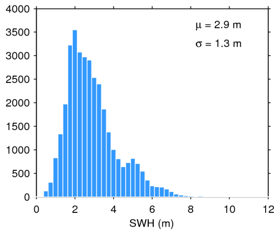
Figure 17. Histogram of flag-valid SWH over oceans and lakes for 23/11/2016. The mean ( \mu ) and standard deviation ( \sigma ) are also shown. Note that values larger than 12 m are excluded from the histogram for the sake of readability but not from the computation of \mu and \sigma .
