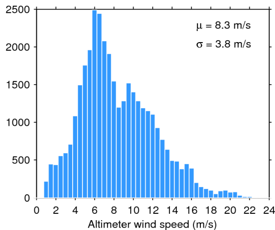
Figure 35. Histogram of science-valid wind over oceans and lakes for 23/11/2016. The mean ( \mu ) and standard deviation ( \sigma ) are also shown. Note that values larger than 24 m/s are excluded from the histogram for the sake of readability but not from the computation of \mu and \sigma .
