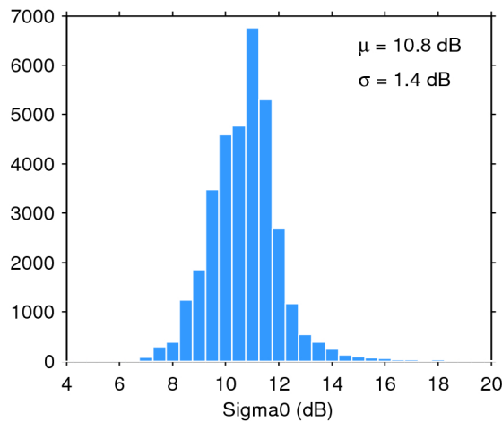
Figure 28. Histogram of science-valid sigma0 over oceans and lakes for 23/11/2016. The mean ( \mu ) and standard deviation ( \sigma ) are also shown. Note that values outside [4 20] dB are excluded from the histogram for the sake of readability but not from the computation of \mu and \sigma .
