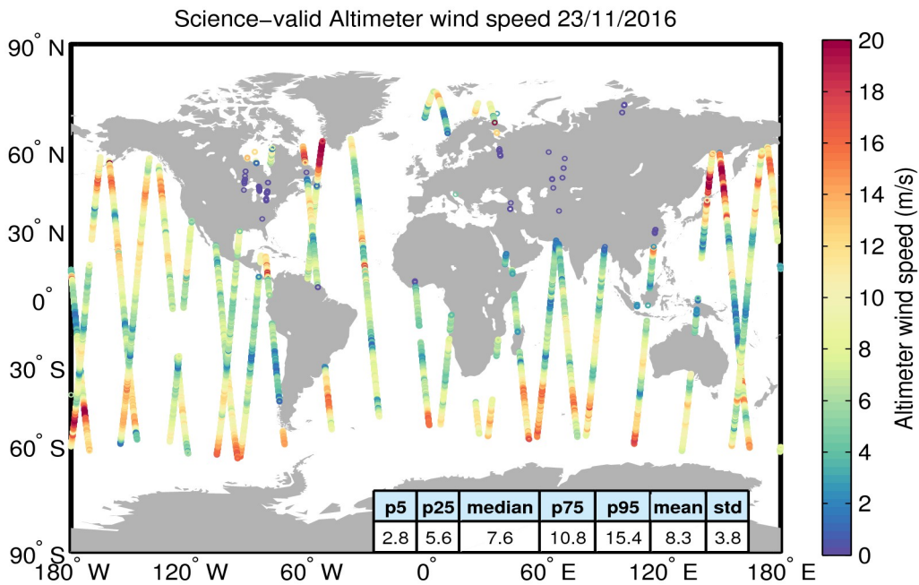
Figure 34. Geographical distribution of science-valid wind data over oceans and lakes for 23/11/2016. The statistical values shown in the table refer to the wind in m/s and are calculated over all measurements shown in the figure. Gray circles denote records that have been rejected based on the editing criteria described in Table 5.
