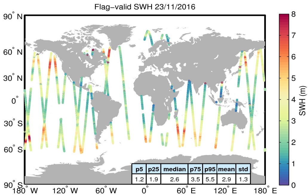
Figure 15. Geographical distribution of flag-valid SWH data over oceans and lakes for 23/11/2016. The statistical values shown in the table refer to the SWH in m and are calculated over all measurements shown in the figure.
