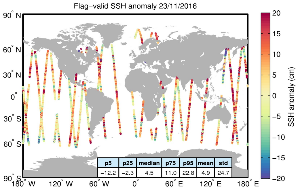
Figure 5. Geographical distribution of flag-valid 1-Hz SSH anomaly data over oceans and lakes for 23/11/2016. The statistical values shown in the table refer to the SSH anomaly in cm and are calculated over all measurements shown in the figure.
