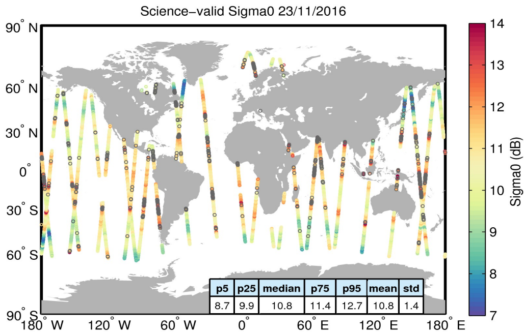
Figure 27. Geographical distribution of science-valid sigma0 data over oceans and lakes for 23/11/2016. The statistical values shown in the table refer to the sigma0 in dB and are calculated over all measurements shown in the figure. Gray circles denote records that have been rejected based on the editing criteria described in Table 4.
