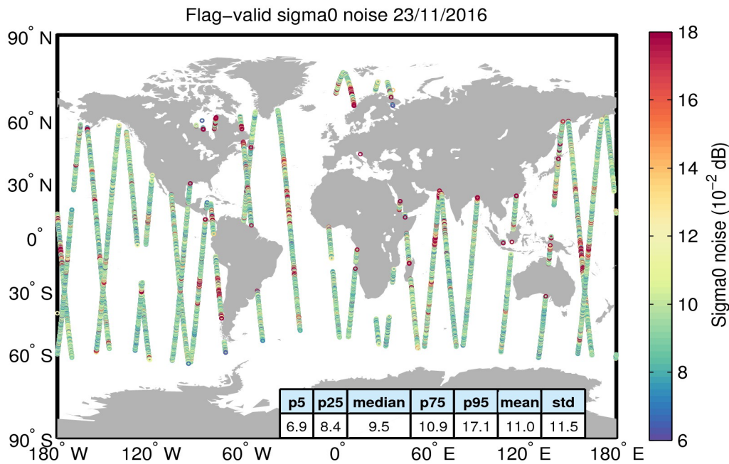
Figure 26. Geographical distribution of flag-valid 20-Hz sigma0 measurement noise over oceans and lakes for 23/11/2016. The statistical values shown in the table refer to the sigma0 noise and are calculated over all measurements shown in the figure.
