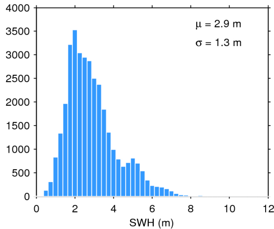
Figure 20. Histogram of science-valid SWH over oceans and lakes for 23/11/2016. The mean ( \mu ) and standard deviation ( \sigma ) are also shown. Note that values larger than 12 m are excluded from the histogram for the sake of readability but not from the computation of \mu and \sigma .
