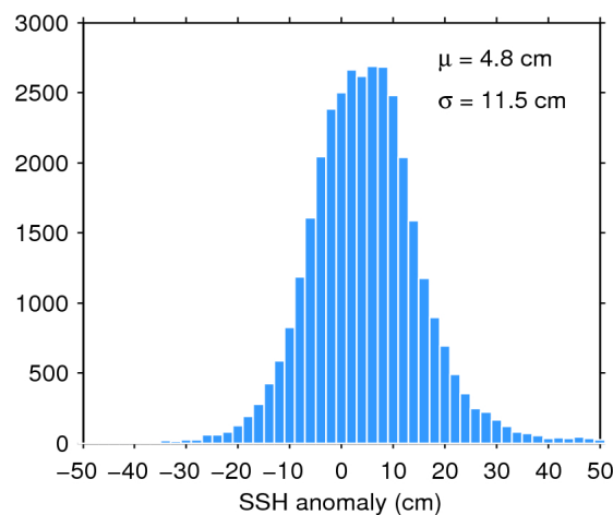
Figure 11. Histogram of science-valid SSH anomaly over oceans and lakes for 23/11/2016. The mean ( \mu ) and standard deviation ( \sigma ) are also shown. Note that values outside [-50 50] cm are excluded from the histogram for the sake of readability but not from the computation of \mu and \sigma .
