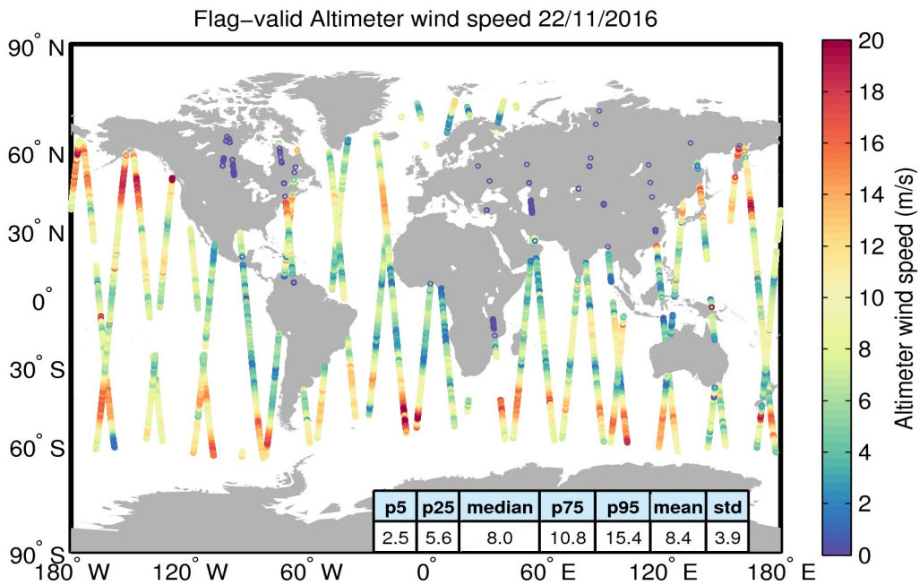
Figure 31. Geographical distribution of flag-valid wind data over oceans and lakes for 22/11/2016. The statistical values shown in the table refer to the wind in m/s and are calculated over all measurements shown in the figure.
