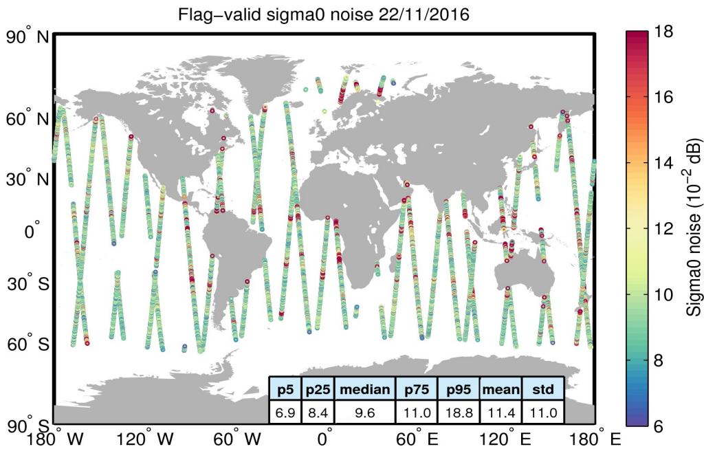
Figure 26. Geographical distribution of flag-valid 20-Hz sigma0 measurement noise over oceans and lakes for 22/11/2016. The statistical values shown in the table refer to the sigma0 noise and are calculated over all measurements shown in the figure.
