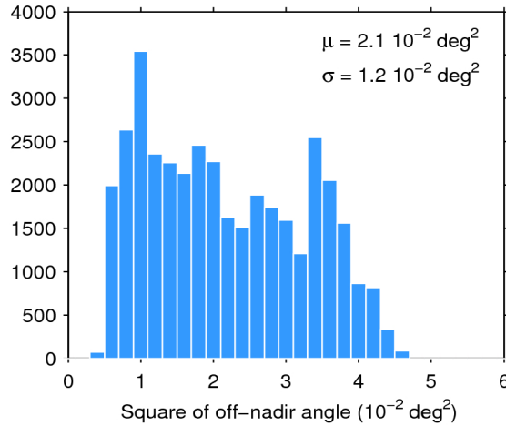
Figure 39. Histogram of flag-valid mispointing over oceans and lakes for 22/11/2016. The mean ( \mu ) and standard deviation ( \sigma ) are also shown. Note that values larger than 6 \cdot 10^{-2} \text{ deg}^2 are excluded from the histogram for the sake of readability but not from the computation of \mu and \sigma .
