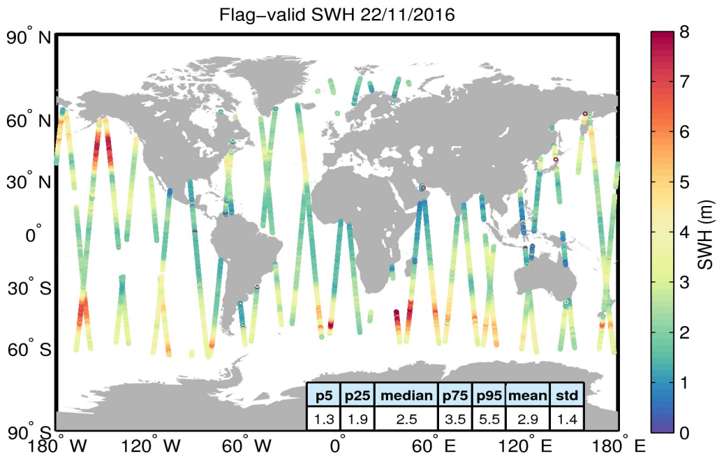
Figure 15. Geographical distribution of flag-valid SWH data over oceans and lakes for 22/11/2016. The statistical values shown in the table refer to the SWH in m and are calculated over all measurements shown in the figure.
