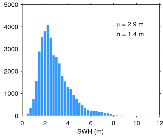
Figure 17. Histogram of flag-valid SWH over oceans and lakes for 22/11/2016. The mean ( \mu ) and standard deviation ( \sigma ) are also shown. Note that values larger than 12 m are excluded from the histogram for the sake of readability but not from the computation of \mu and \sigma .
