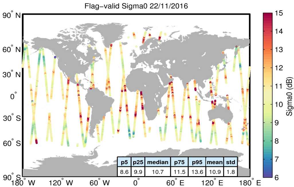
Figure 23. Geographical distribution of flag-valid sigma0 data over oceans and lakes for 22/11/2016. The statistical values shown in the table refer to the sigma0 in dB and are calculated over all measurements shown in the figure.
