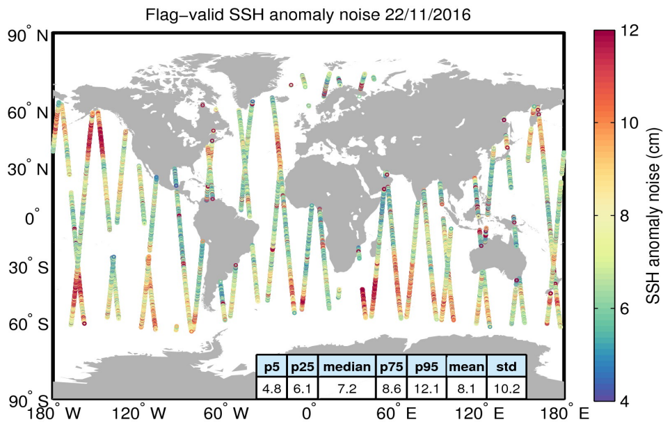
Figure 8. Geographical distribution of flag-valid 20-Hz SSH anomaly measurement noise over oceans and lakes for 22/11/2016. The statistical values shown in the table refer to the SSH anomaly noise and are calculated over all measurements shown in the figure.
