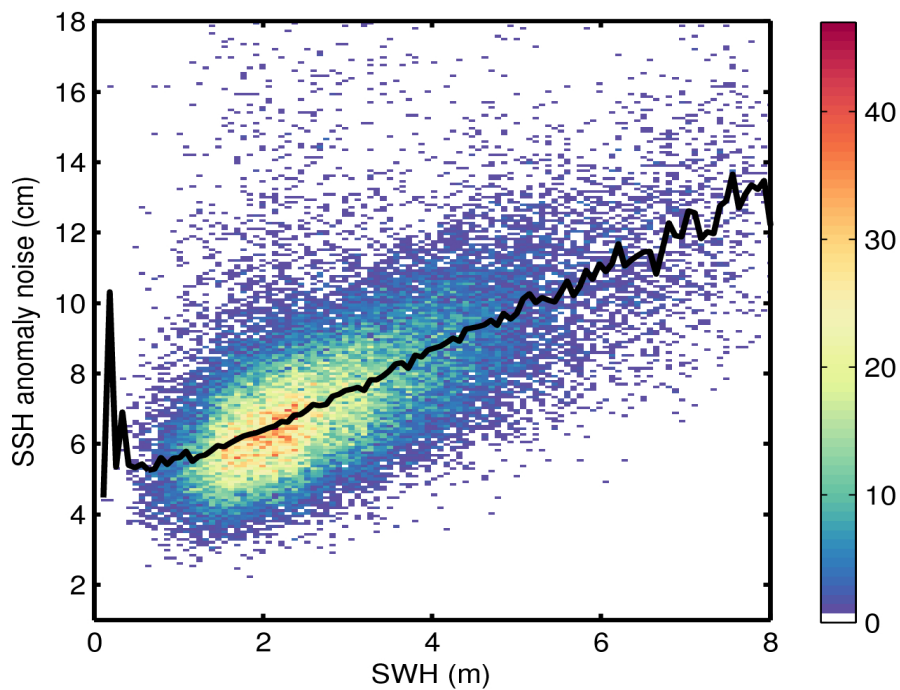
Figure 9. 2D histogram showing flag-valid SSH anomaly noise as a function of SWH for 22/11/2016. The black line denotes the median SSH anomaly noise as a function of SWH.
