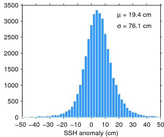
Figure 7. Histogram of flag-valid SSH anomaly over oceans and lakes for 22/11/2016. The mean ( \mu ) and standard deviation ( \sigma ) are also shown. Note that values outside [-50 50] cm are excluded from the histogram for the sake of readability but not from the computation of \mu and \sigma .
