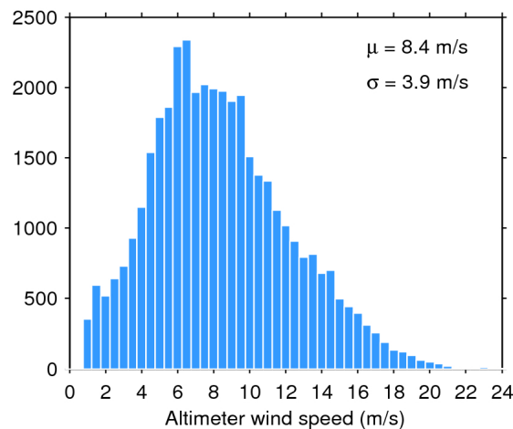
Figure 35. Histogram of science-valid wind over oceans and lakes for 22/11/2016. The mean ( \mu ) and standard deviation ( \sigma ) are also shown. Note that values larger than 24 m/s are excluded from the histogram for the sake of readability but not from the computation of \mu and \sigma .
