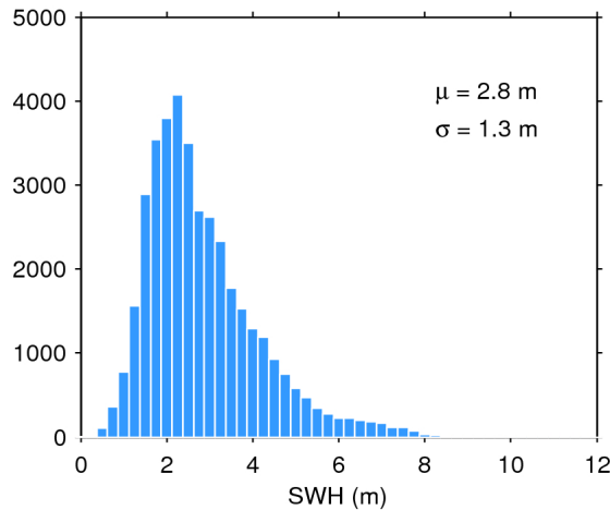
Figure 20. Histogram of science-valid SWH over oceans and lakes for 22/11/2016. The mean ( \mu ) and standard deviation ( \sigma ) are also shown. Note that values larger than 12 m are excluded from the histogram for the sake of readability but not from the computation of \mu and \sigma .
