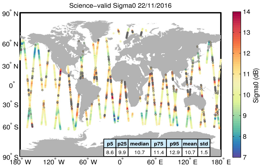
Figure 27. Geographical distribution of science-valid sigma0 data over oceans and lakes for 22/11/2016. The statistical values shown in the table refer to the sigma0 in dB and are calculated over all measurements shown in the figure. Gray circles denote records that have been rejected based on the editing criteria described in Table 4.
