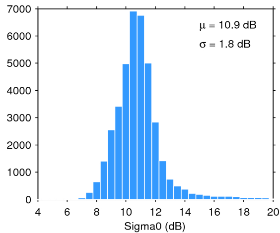
Figure 25. Histogram of flag-valid sigma0 over oceans and lakes for 22/11/2016. The mean ( \mu ) and standard deviation ( \sigma ) are also shown. Note that values outside [4 20] dB are excluded from the histogram for the sake of readability but not from the computation of \mu and \sigma .
