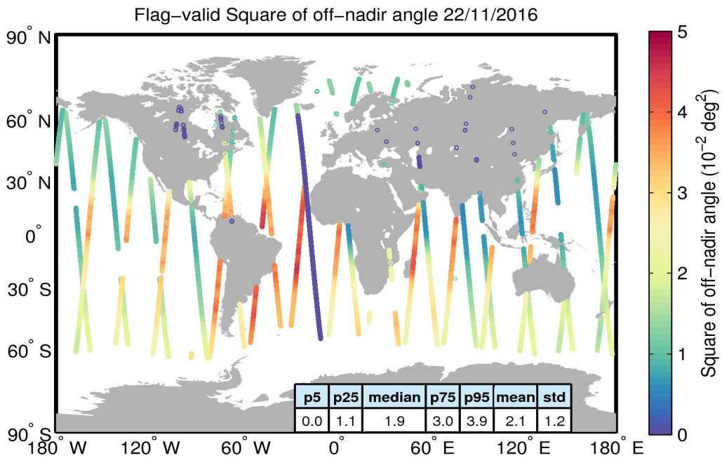
Figure 37. Geographical distribution of flag-valid mispointing data over oceans and lakes for 22/11/2016. The statistical values shown in the table refer to the mispointing in 10^{-2} \text{deg}^2 and are calculated over all measurements shown in the figure.
