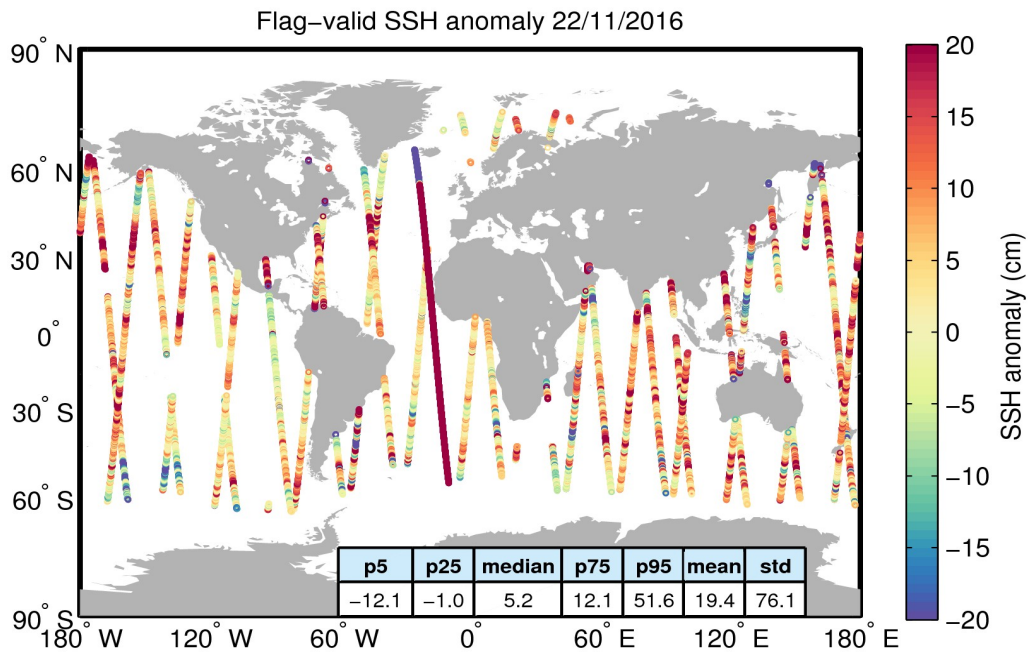
Figure 5. Geographical distribution of flag-valid 1-Hz SSH anomaly data over oceans and lakes for 22/11/2016. The statistical values shown in the table refer to the SSH anomaly in cm and are calculated over all measurements shown in the figure.
