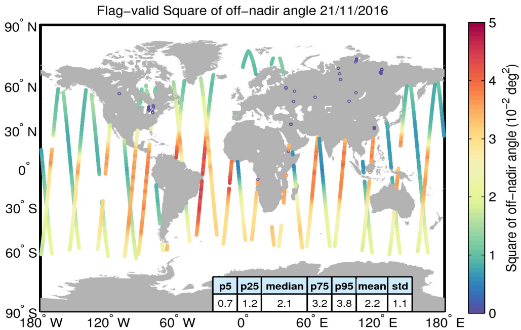
Figure 37. Geographical distribution of flag-valid mispointing data over oceans and lakes for 21/11/2016. The statistical values shown in the table refer to the mispointing in 10^{-2} deg 2 and are calculated over all measurements shown in the figure.
