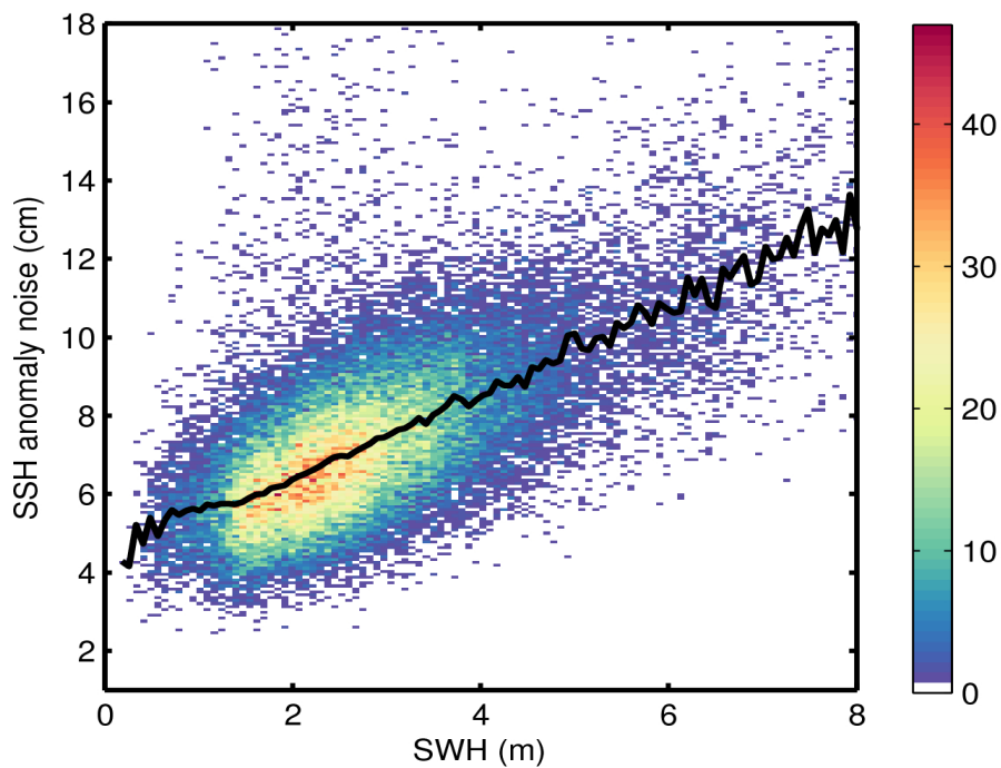
Figure 9. 2D histogram showing flag-valid SSH anomaly noise as a function of SWH for 21/11/2016. The black line denotes the median SSH anomaly noise as a function of SWH.
