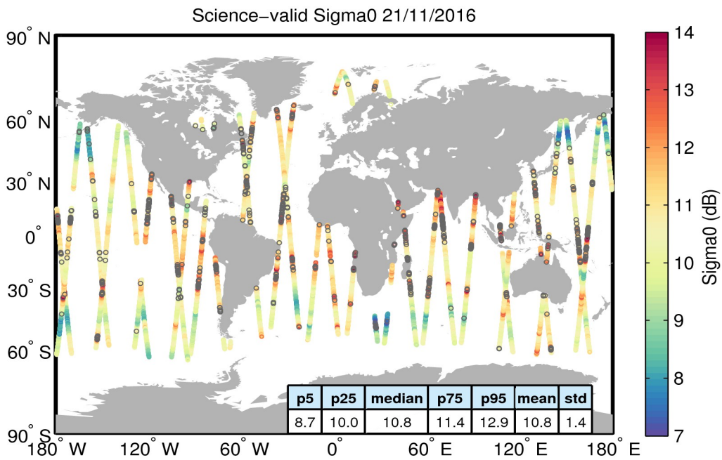
Figure 27. Geographical distribution of science-valid sigma0 data over oceans and lakes for 21/11/2016. The statistical values shown in the table refer to the sigma0 in dB and are calculated over all measurements shown in the figure. Gray circles denote records that have been rejected based on the editing criteria described in Table 4.
