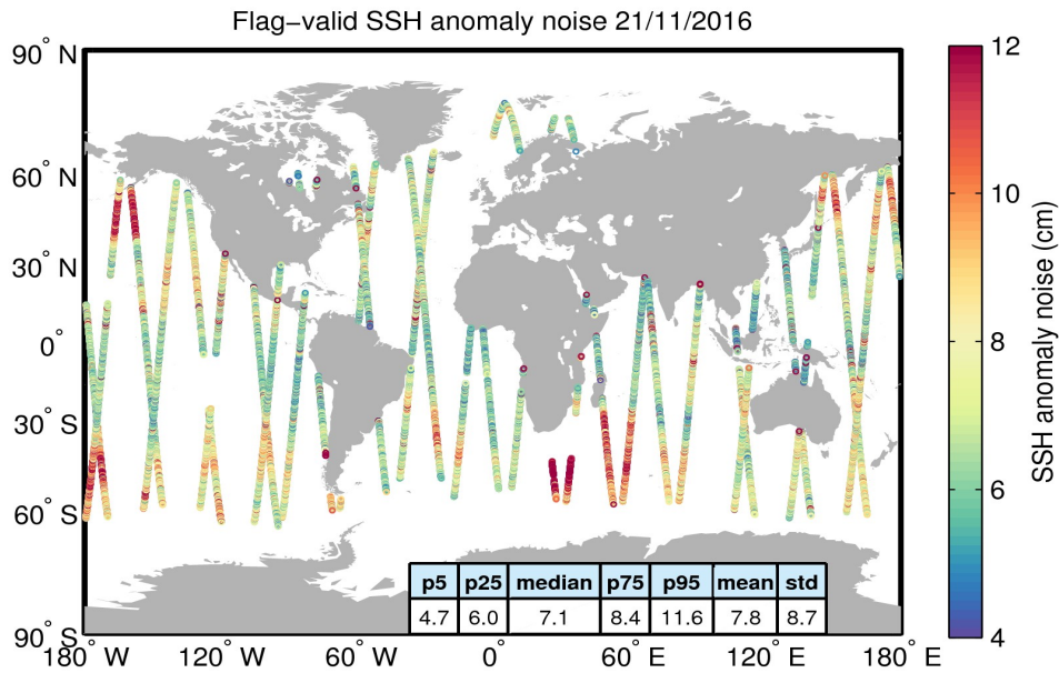
Figure 8. Geographical distribution of flag-valid 20-Hz SSH anomaly measurement noise over oceans and lakes for 21/11/2016. The statistical values shown in the table refer to the SSH anomaly noise and are calculated over all measurements shown in the figure.
