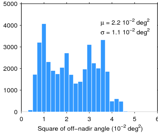
Figure 39. Histogram of flag-valid mispointing over oceans and lakes for 21/11/2016. The mean ( \mu ) and standard deviation ( \sigma ) are also shown. Note that values larger than 6 \cdot 10^{-2} \text{ deg}^2 are excluded from the histogram for the sake of readability but not from the computation of \mu and \sigma .
