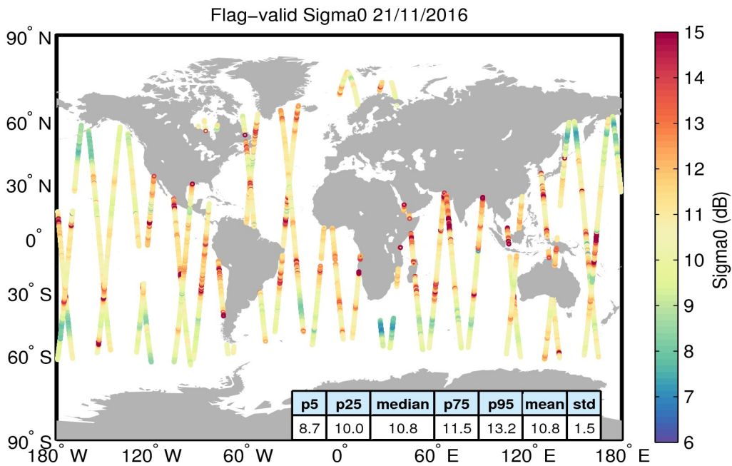
Figure 23. Geographical distribution of flag-valid sigma0 data over oceans and lakes for 21/11/2016. The statistical values shown in the table refer to the sigma0 in dB and are calculated over all measurements shown in the figure.
