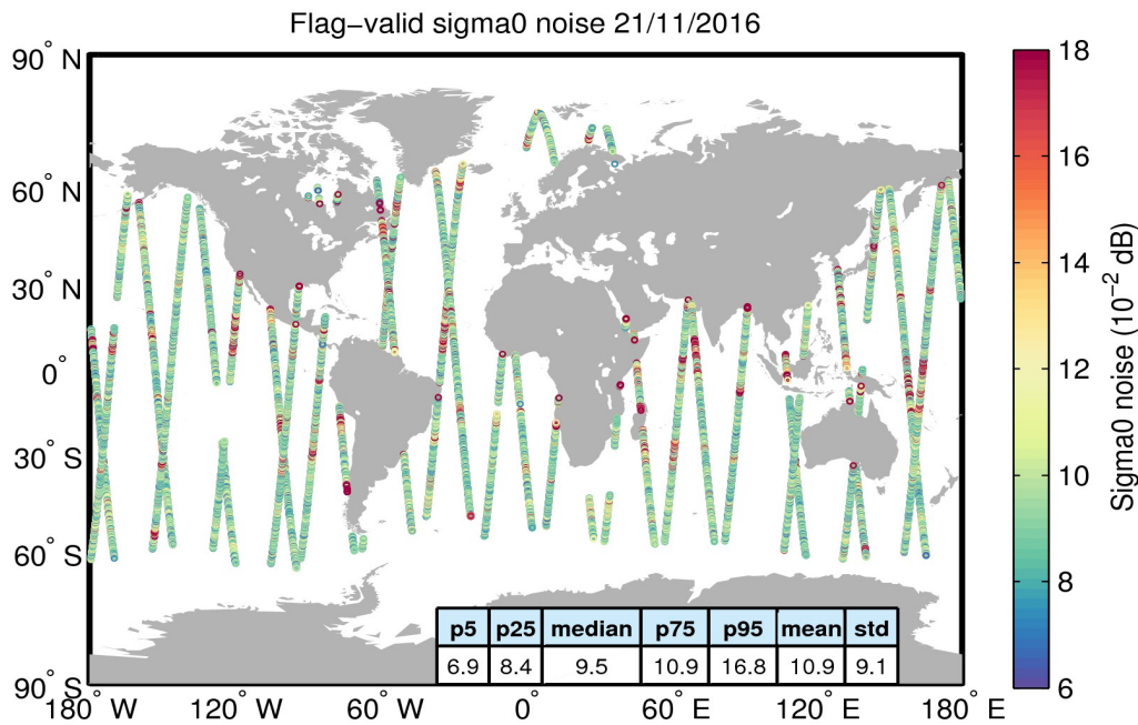
Figure 26. Geographical distribution of flag-valid 20-Hz sigma0 measurement noise over oceans and lakes for 21/11/2016. The statistical values shown in the table refer to the sigma0 noise and are calculated over all measurements shown in the figure.
