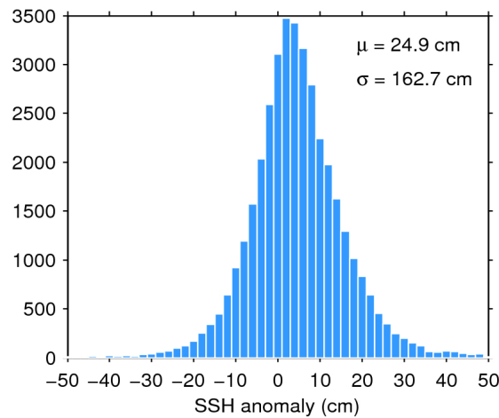
Figure 7. Histogram of flag-valid SSH anomaly over oceans and lakes for 21/11/2016. The mean ( \mu ) and standard deviation ( \sigma ) are also shown. Note that values outside [-50 50] cm are excluded from the histogram for the sake of readability but not from the computation of \mu and \sigma .
