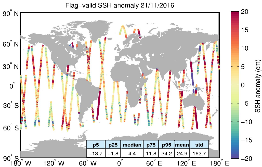
Figure 5. Geographical distribution of flag-valid 1-Hz SSH anomaly data over oceans and lakes for 21/11/2016. The statistical values shown in the table refer to the SSH anomaly in cm and are calculated over all measurements shown in the figure.
