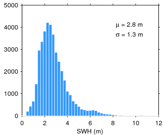
Figure 20. Histogram of science-valid SWH over oceans and lakes for 21/11/2016. The mean ( \mu ) and standard deviation ( \sigma ) are also shown. Note that values larger than 12 m are excluded from the histogram for the sake of readability but not from the computation of \mu and \sigma .
