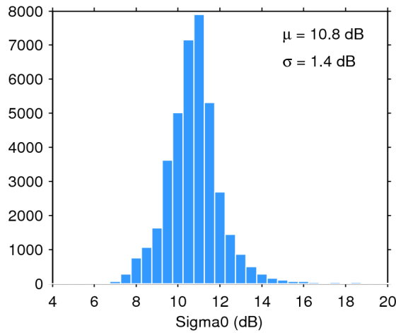
Figure 28. Histogram of science-valid sigma0 over oceans and lakes for 21/11/2016. The mean ( \mu ) and standard deviation ( \sigma ) are also shown. Note that values outside [4 20] dB are excluded from the histogram for the sake of readability but not from the computation of \mu and \sigma .
