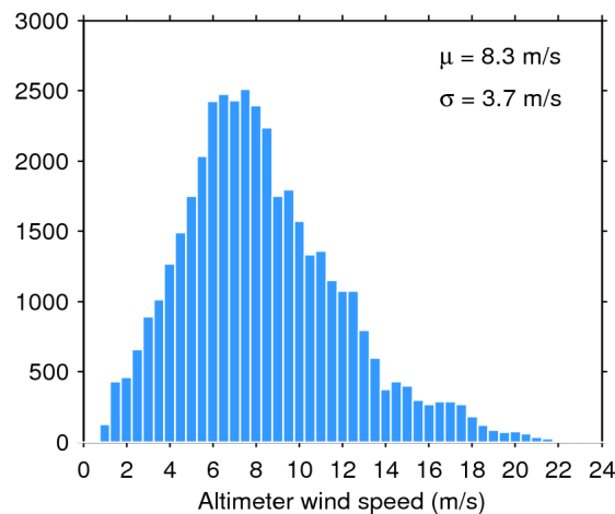
Figure 35. Histogram of science-valid wind over oceans and lakes for 21/11/2016. The mean ( \mu ) and standard deviation ( \sigma ) are also shown. Note that values larger than 24 m/s are excluded from the histogram for the sake of readability but not from the computation of \mu and \sigma .
