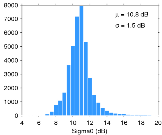
Figure 25. Histogram of flag-valid sigma0 over oceans and lakes for 21/11/2016. The mean ( \mu ) and standard deviation ( \sigma ) are also shown. Note that values outside [4 20] dB are excluded from the histogram for the sake of readability but not from the computation of \mu and \sigma .
