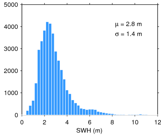
Figure 17. Histogram of flag-valid SWH over oceans and lakes for 21/11/2016. The mean ( \mu ) and standard deviation ( \sigma ) are also shown. Note that values larger than 12 m are excluded from the histogram for the sake of readability but not from the computation of \mu and \sigma .
