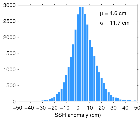
Figure 11. Histogram of science-valid SSH anomaly over oceans and lakes for 21/11/2016. The mean ( \mu ) and standard deviation ( \sigma ) are also shown. Note that values outside [-50 50] cm are excluded from the histogram for the sake of readability but not from the computation of \mu and \sigma .
