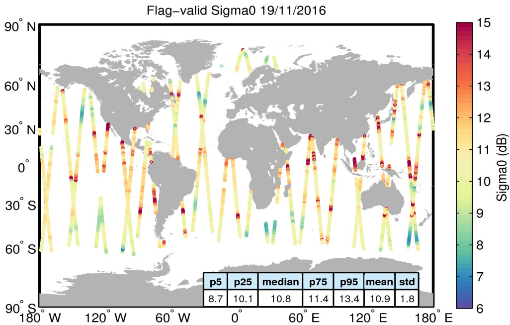
Figure 23. Geographical distribution of flag-valid sigma0 data over oceans and lakes for 19/11/2016. The statistical values shown in the table refer to the sigma0 in dB and are calculated over all measurements shown in the figure.
