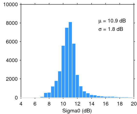
Figure 25. Histogram of flag-valid sigma0 over oceans and lakes for 19/11/2016. The mean ( \mu ) and standard deviation ( \sigma ) are also shown. Note that values outside [4 20] dB are excluded from the histogram for the sake of readability but not from the computation of \mu and \sigma .
