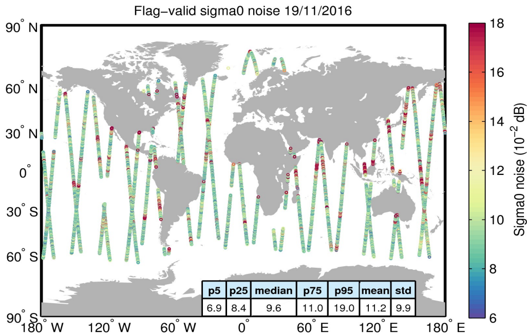
Figure 26. Geographical distribution of flag-valid 20-Hz sigma0 measurement noise over oceans and lakes for 19/11/2016. The statistical values shown in the table refer to the sigma0 noise and are calculated over all measurements shown in the figure.
