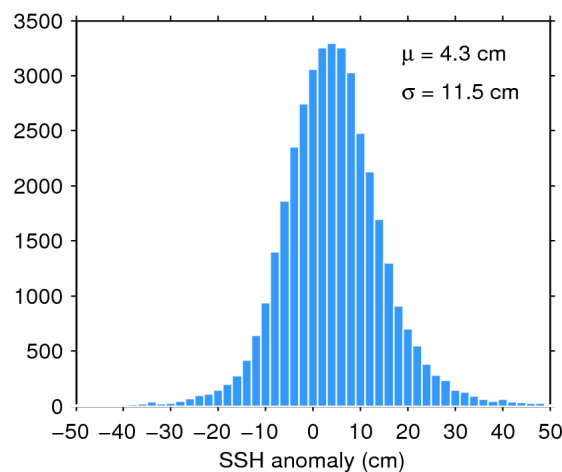
Figure 11. Histogram of science-valid SSH anomaly over oceans and lakes for 19/11/2016. The mean ( \mu ) and standard deviation ( \sigma ) are also shown. Note that values outside [-50 50] cm are excluded from the histogram for the sake of readability but not from the computation of \mu and \sigma .
