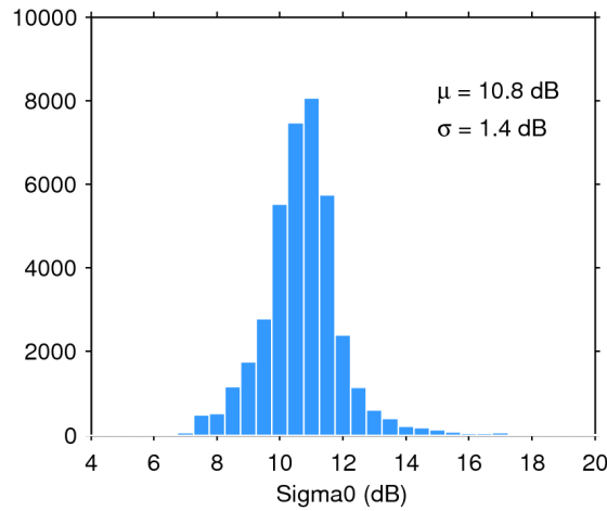
Figure 28. Histogram of science-valid sigma0 over oceans and lakes for 19/11/2016. The mean ( \mu ) and standard deviation ( \sigma ) are also shown. Note that values outside [4 20] dB are excluded from the histogram for the sake of readability but not from the computation of \mu and \sigma .
