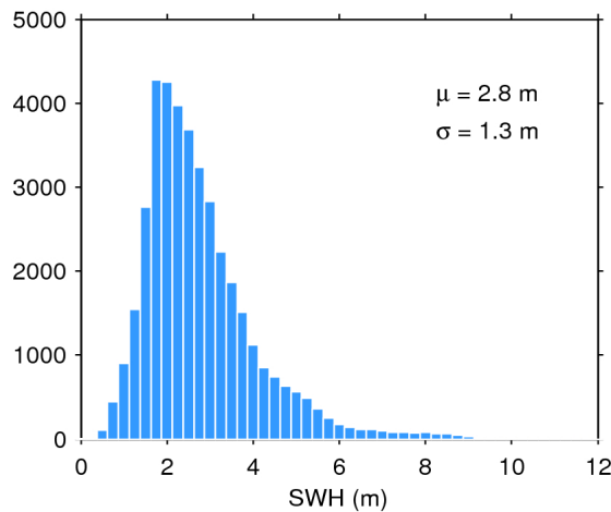
Figure 20. Histogram of science-valid SWH over oceans and lakes for 19/11/2016. The mean ( \mu ) and standard deviation ( \sigma ) are also shown. Note that values larger than 12 m are excluded from the histogram for the sake of readability but not from the computation of \mu and \sigma .
