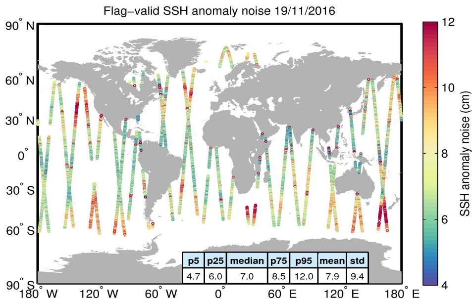
Figure 8. Geographical distribution of flag-valid 20-Hz SSH anomaly measurement noise over oceans and lakes for 19/11/2016. The statistical values shown in the table refer to the SSH anomaly noise and are calculated over all measurements shown in the figure.
