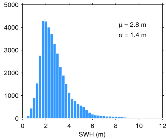
Figure 17. Histogram of flag-valid SWH over oceans and lakes for 19/11/2016. The mean ( \mu ) and standard deviation ( \sigma ) are also shown. Note that values larger than 12 m are excluded from the histogram for the sake of readability but not from the computation of \mu and \sigma .
