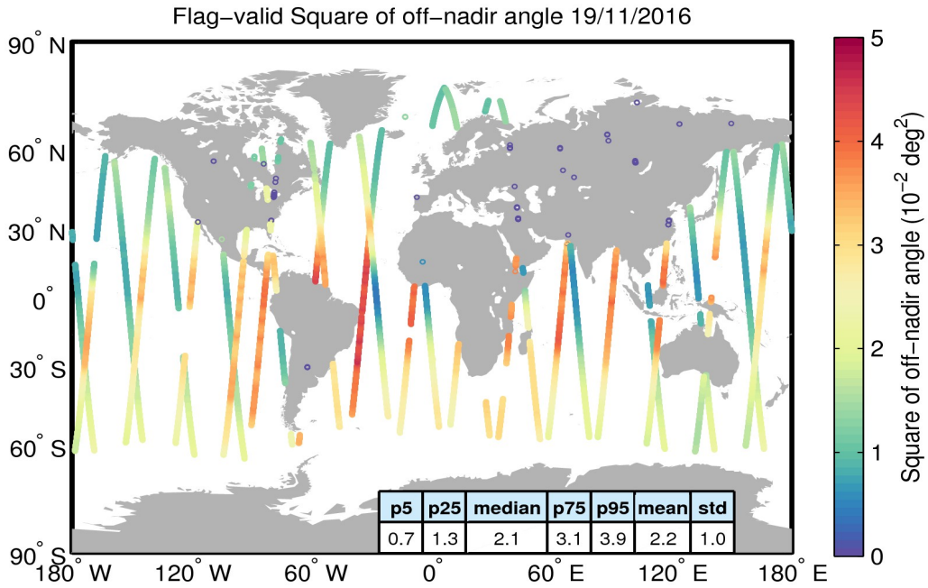
Figure 37. Geographical distribution of flag-valid mispointing data over oceans and lakes for 19/11/2016. The statistical values shown in the table refer to the mispointing in 10^{-2} deg 2 and are calculated over all measurements shown in the figure.
