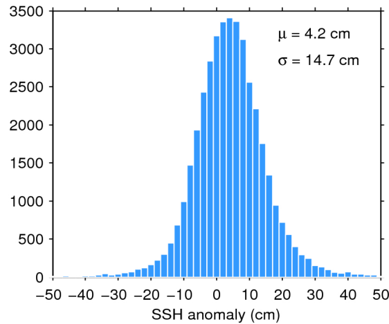
Figure 7. Histogram of flag-valid SSH anomaly over oceans and lakes for 19/11/2016. The mean ( \mu ) and standard deviation ( \sigma ) are also shown. Note that values outside [-50\ 50] cm are excluded from the histogram for the sake of readability but not from the computation of \mu and \sigma .
