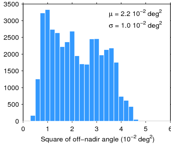
Figure 39. Histogram of flag-valid mispointing over oceans and lakes for 19/11/2016. The mean ( \mu ) and standard deviation ( \sigma ) are also shown. Note that values larger than 6 \cdot 10^{-2} \text{ deg}^2 are excluded from the histogram for the sake of readability but not from the computation of \mu and \sigma .
