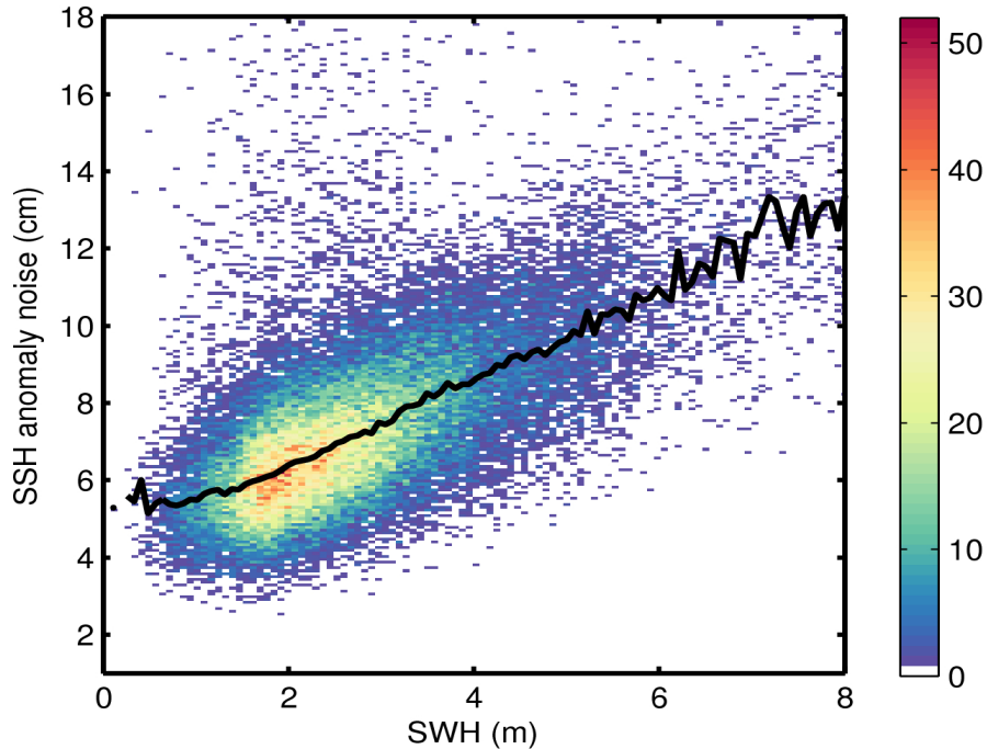
Figure 9. 2D histogram showing flag-valid SSH anomaly noise as a function of SWH for 19/11/2016. The black line denotes the median SSH anomaly noise as a function of SWH.
