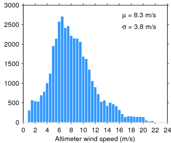
Figure 33. Histogram of flag-valid wind over oceans and lakes for 19/11/2016. The mean ( \mu ) and standard deviation ( \sigma ) are also shown. Note that values larger than 24 m/s are excluded from the histogram for the sake of readability but not from the computation of \mu and \sigma .
