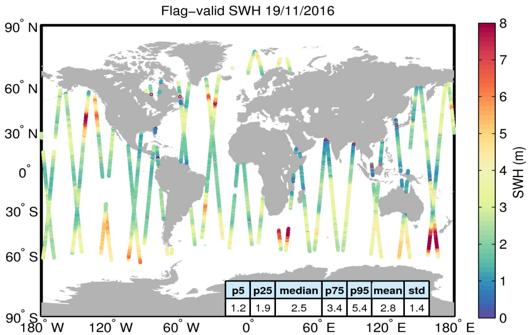
Figure 15. Geographical distribution of flag-valid SWH data over oceans and lakes for 19/11/2016. The statistical values shown in the table refer to the SWH in m and are calculated over all measurements shown in the figure.
