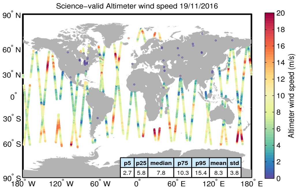
Figure 34. Geographical distribution of science-valid wind data over oceans and lakes for 19/11/2016. The statistical values shown in the table refer to the wind in m/s and are calculated over all measurements shown in the figure. Gray circles denote records that have been rejected based on the editing criteria described in Table 5.
