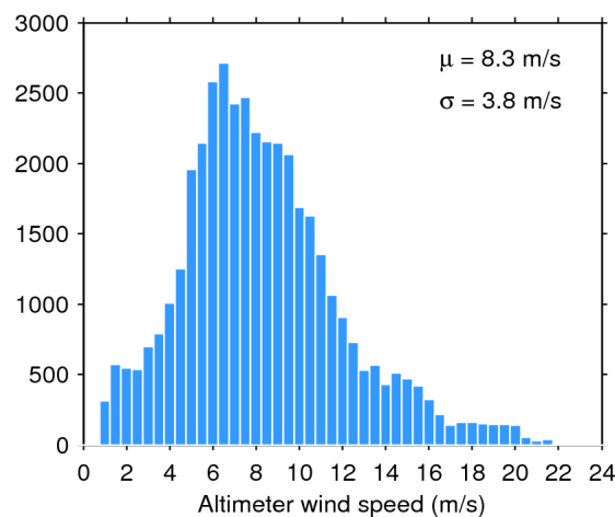
Figure 35. Histogram of science-valid wind over oceans and lakes for 19/11/2016. The mean ( \mu ) and standard deviation ( \sigma ) are also shown. Note that values larger than 24 m/s are excluded from the histogram for the sake of readability but not from the computation of \mu and \sigma .
