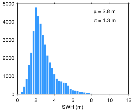
Figure 20. Histogram of science-valid SWH over oceans and lakes for 18/11/2016. The mean ( \mu ) and standard deviation ( \sigma ) are also shown. Note that values larger than 12 m are excluded from the histogram for the sake of readability but not from the computation of \mu and \sigma .
