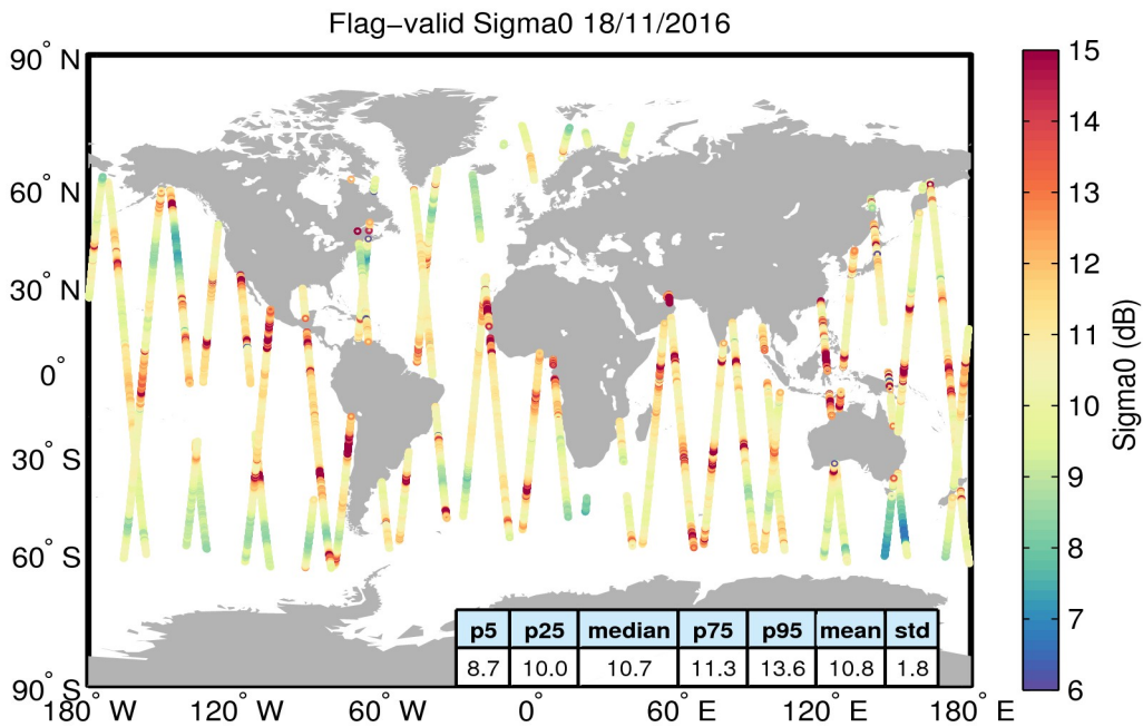
Figure 23. Geographical distribution of flag-valid sigma0 data over oceans and lakes for 18/11/2016. The statistical values shown in the table refer to the sigma0 in dB and are calculated over all measurements shown in the figure.
