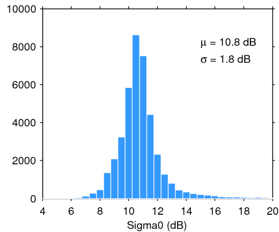
Figure 25. Histogram of flag-valid sigma0 over oceans and lakes for 18/11/2016. The mean ( \mu ) and standard deviation ( \sigma ) are also shown. Note that values outside [4 20] dB are excluded from the histogram for the sake of readability but not from the computation of \mu and \sigma .
