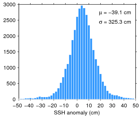
Figure 7. Histogram of flag-valid SSH anomaly over oceans and lakes for 18/11/2016. The mean ( \mu ) and standard deviation ( \sigma ) are also shown. Note that values outside [-50 50] cm are excluded from the histogram for the sake of readability but not from the computation of \mu and \sigma .
