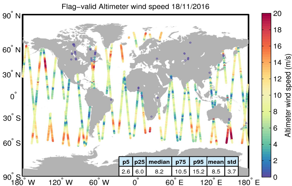
Figure 31. Geographical distribution of flag-valid wind data over oceans and lakes for 18/11/2016. The statistical values shown in the table refer to the wind in m/s and are calculated over all measurements shown in the figure.
