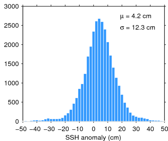
Figure 11. Histogram of science-valid SSH anomaly over oceans and lakes for 18/11/2016. The mean ( \mu ) and standard deviation ( \sigma ) are also shown. Note that values outside [-50 50] cm are excluded from the histogram for the sake of readability but not from the computation of \mu and \sigma .
