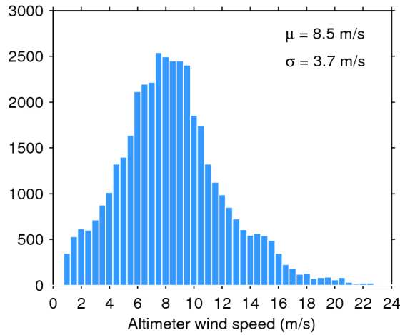
Figure 33. Histogram of flag-valid wind over oceans and lakes for 18/11/2016. The mean ( \mu ) and standard deviation ( \sigma ) are also shown. Note that values larger than 24 m/s are excluded from the histogram for the sake of readability but not from the computation of \mu and \sigma .
