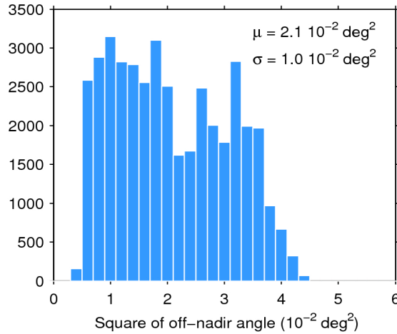
Figure 39. Histogram of flag-valid mispointing over oceans and lakes for 18/11/2016. The mean ( \mu ) and standard deviation ( \sigma ) are also shown. Note that values larger than 6 \cdot 10^{-2} \text{ deg}^2 are excluded from the histogram for the sake of readability but not from the computation of \mu and \sigma .
