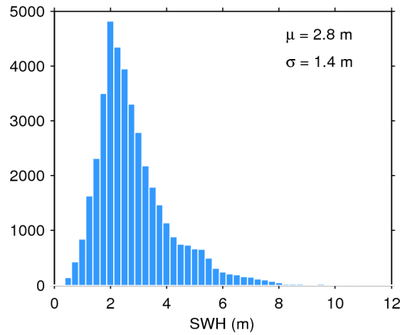
Figure 17. Histogram of flag-valid SWH over oceans and lakes for 18/11/2016. The mean ( \mu ) and standard deviation ( \sigma ) are also shown. Note that values larger than 12 m are excluded from the histogram for the sake of readability but not from the computation of \mu and \sigma .
