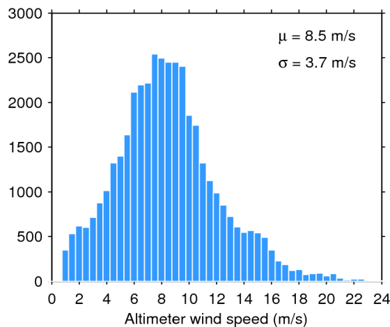
Figure 35. Histogram of science-valid wind over oceans and lakes for 18/11/2016. The mean ( \mu ) and standard deviation ( \sigma ) are also shown. Note that values larger than 24 m/s are excluded from the histogram for the sake of readability but not from the computation of \mu and \sigma .
