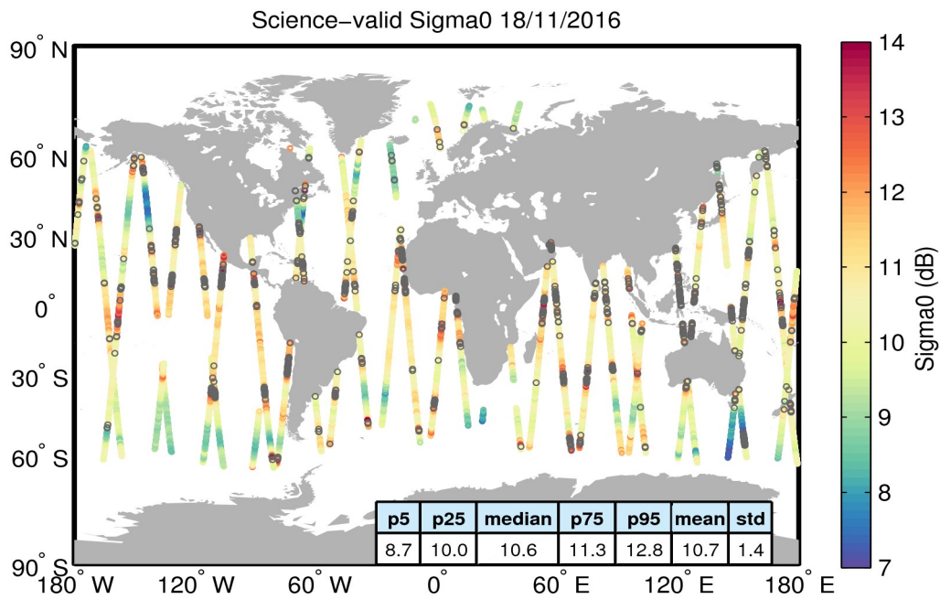
Figure 27. Geographical distribution of science-valid sigma0 data over oceans and lakes for 18/11/2016. The statistical values shown in the table refer to the sigma0 in dB and are calculated over all measurements shown in the figure. Gray circles denote records that have been rejected based on the editing criteria described in Table 4.
