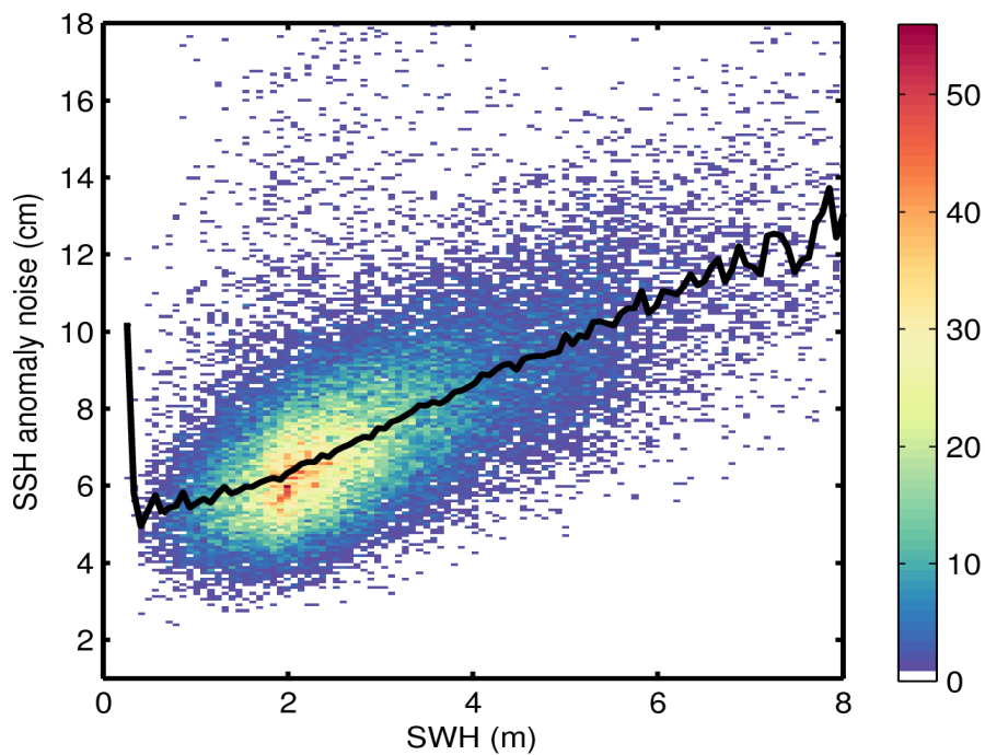
Figure 9. 2D histogram showing flag-valid SSH anomaly noise as a function of SWH for 18/11/2016. The black line denotes the median SSH anomaly noise as a function of SWH.
