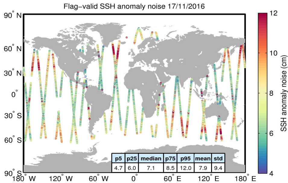
Figure 8. Geographical distribution of flag-valid 20-Hz SSH anomaly measurement noise over oceans and lakes for 17/11/2016. The statistical values shown in the table refer to the SSH anomaly noise and are calculated over all measurements shown in the figure.
