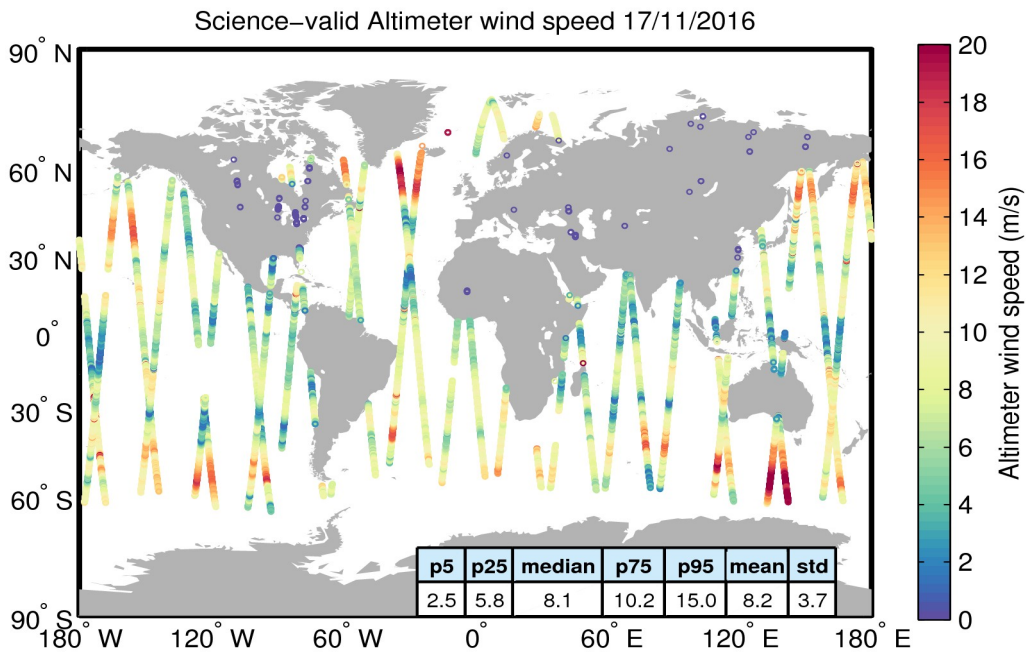
Figure 34. Geographical distribution of science-valid wind data over oceans and lakes for 17/11/2016. The statistical values shown in the table refer to the wind in m/s and are calculated over all measurements shown in the figure. Gray circles denote records that have been rejected based on the editing criteria described in Table 5.
