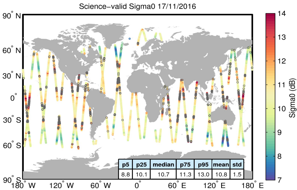
Figure 27. Geographical distribution of science-valid sigma0 data over oceans and lakes for 17/11/2016. The statistical values shown in the table refer to the sigma0 in dB and are calculated over all measurements shown in the figure. Gray circles denote records that have been rejected based on the editing criteria described in Table 4.
