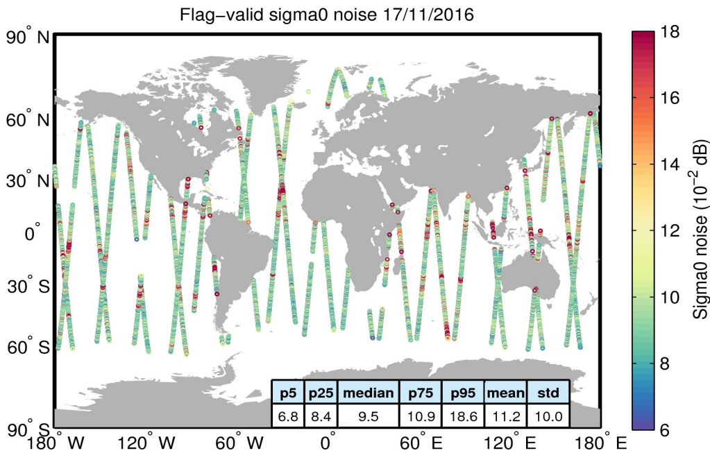
Figure 26. Geographical distribution of flag-valid 20-Hz sigma0 measurement noise over oceans and lakes for 17/11/2016. The statistical values shown in the table refer to the sigma0 noise and are calculated over all measurements shown in the figure.
