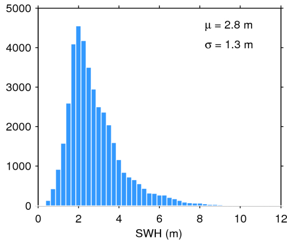
Figure 20. Histogram of science-valid SWH over oceans and lakes for 17/11/2016. The mean ( \mu ) and standard deviation ( \sigma ) are also shown. Note that values larger than 12 m are excluded from the histogram for the sake of readability but not from the computation of \mu and \sigma .
