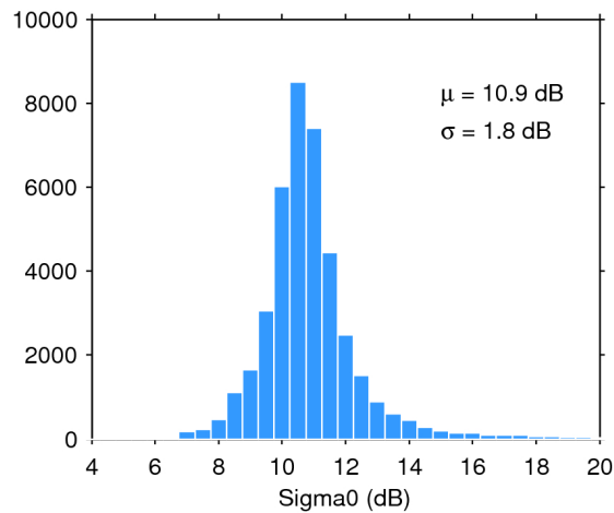
Figure 25. Histogram of flag-valid sigma0 over oceans and lakes for 17/11/2016. The mean ( \mu ) and standard deviation ( \sigma ) are also shown. Note that values outside [4 20] dB are excluded from the histogram for the sake of readability but not from the computation of \mu and \sigma .
