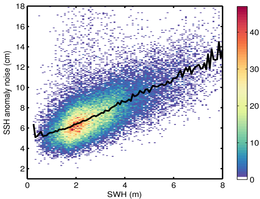
Figure 9. 2D histogram showing flag-valid SSH anomaly noise as a function of SWH for 17/11/2016. The black line denotes the median SSH anomaly noise as a function of SWH.
