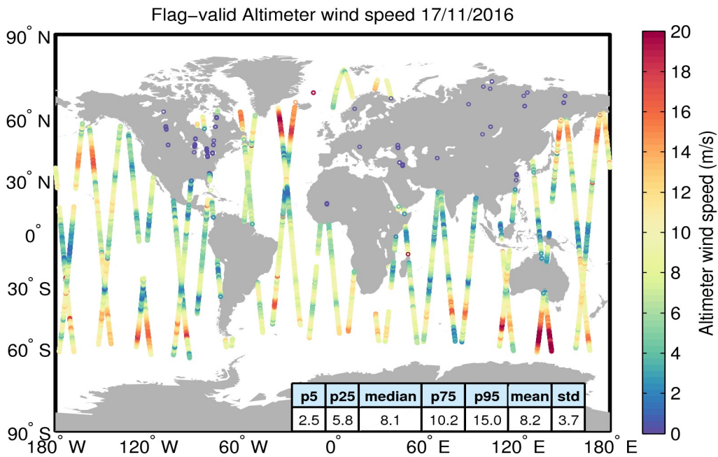
Figure 31. Geographical distribution of flag-valid wind data over oceans and lakes for 17/11/2016. The statistical values shown in the table refer to the wind in m/s and are calculated over all measurements shown in the figure.
