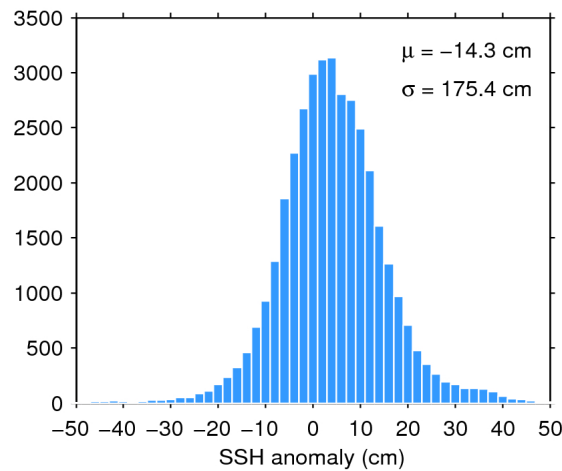
Figure 7. Histogram of flag-valid SSH anomaly over oceans and lakes for 17/11/2016. The mean ( \mu ) and standard deviation ( \sigma ) are also shown. Note that values outside [-50 50] cm are excluded from the histogram for the sake of readability but not from the computation of \mu and \sigma .
