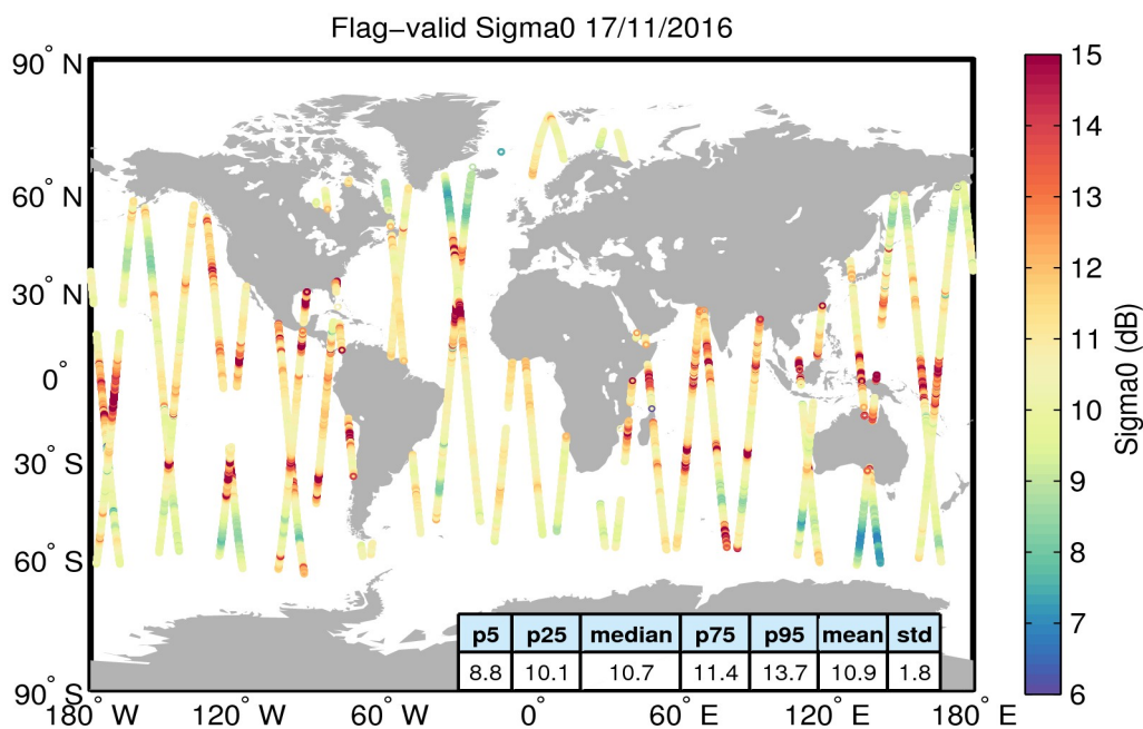
Figure 23. Geographical distribution of flag-valid sigma0 data over oceans and lakes for 17/11/2016. The statistical values shown in the table refer to the sigma0 in dB and are calculated over all measurements shown in the figure.
