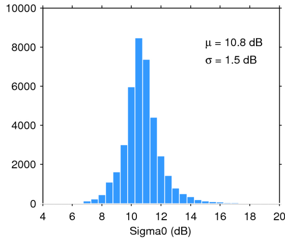
Figure 28. Histogram of science-valid sigma0 over oceans and lakes for 17/11/2016. The mean ( \mu ) and standard deviation ( \sigma ) are also shown. Note that values outside [4 20] dB are excluded from the histogram for the sake of readability but not from the computation of \mu and \sigma .
