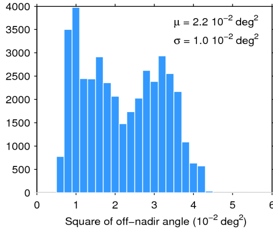
Figure 39. Histogram of flag-valid mispointing over oceans and lakes for 17/11/2016. The mean ( \mu ) and standard deviation ( \sigma ) are also shown. Note that values larger than 6 \cdot 10^{-2} \text{ deg}^2 are excluded from the histogram for the sake of readability but not from the computation of \mu and \sigma .
