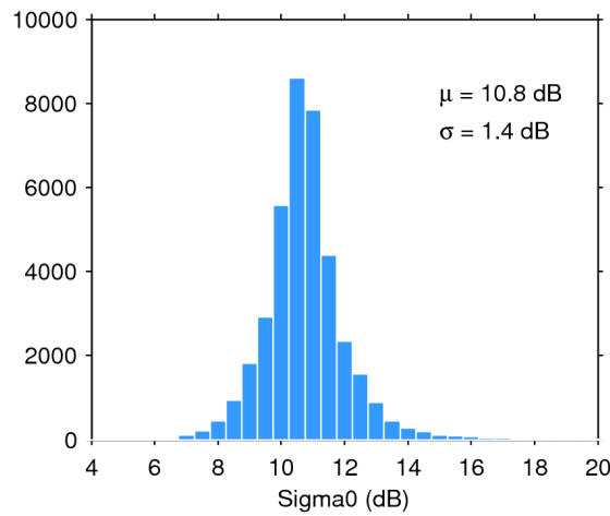
Figure 28. Histogram of science-valid sigma0 over oceans and lakes for 16/11/2016. The mean ( \mu ) and standard deviation ( \sigma ) are also shown. Note that values outside [4 20] dB are excluded from the histogram for the sake of readability but not from the computation of \mu and \sigma .
