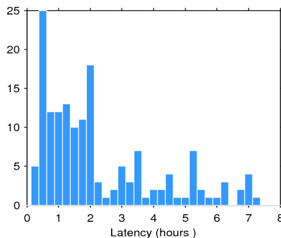
Figure 2. Histogram of the data latency for 16/11/2016. The y-axis denotes the number of files that are made available with a delay of x-hours with respect to the mean time of the records stored in the file.
