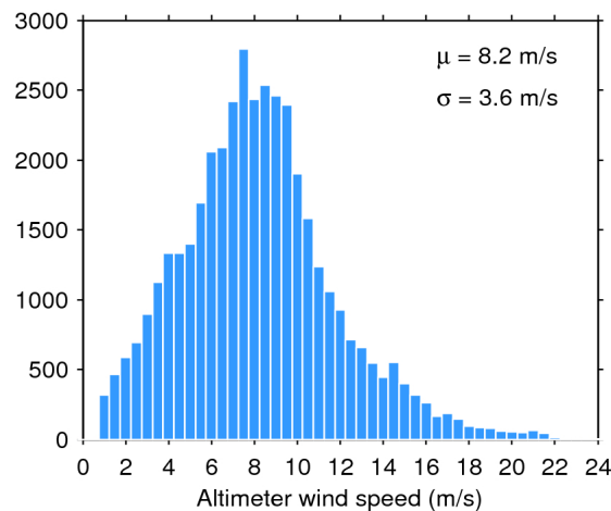
Figure 35. Histogram of science-valid wind over oceans and lakes for 16/11/2016. The mean ( \mu ) and standard deviation ( \sigma ) are also shown. Note that values larger than 24 m/s are excluded from the histogram for the sake of readability but not from the computation of \mu and \sigma .
