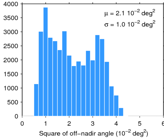
Figure 39. Histogram of flag-valid mispointing over oceans and lakes for 16/11/2016. The mean ( \mu ) and standard deviation ( \sigma ) are also shown. Note that values larger than 6 \cdot 10^{-2} \text{ deg}^2 are excluded from the histogram for the sake of readability but not from the computation of \mu and \sigma .
