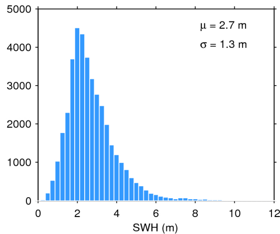
Figure 20. Histogram of science-valid SWH over oceans and lakes for 16/11/2016. The mean ( \mu ) and standard deviation ( \sigma ) are also shown. Note that values larger than 12 m are excluded from the histogram for the sake of readability but not from the computation of \mu and \sigma .
