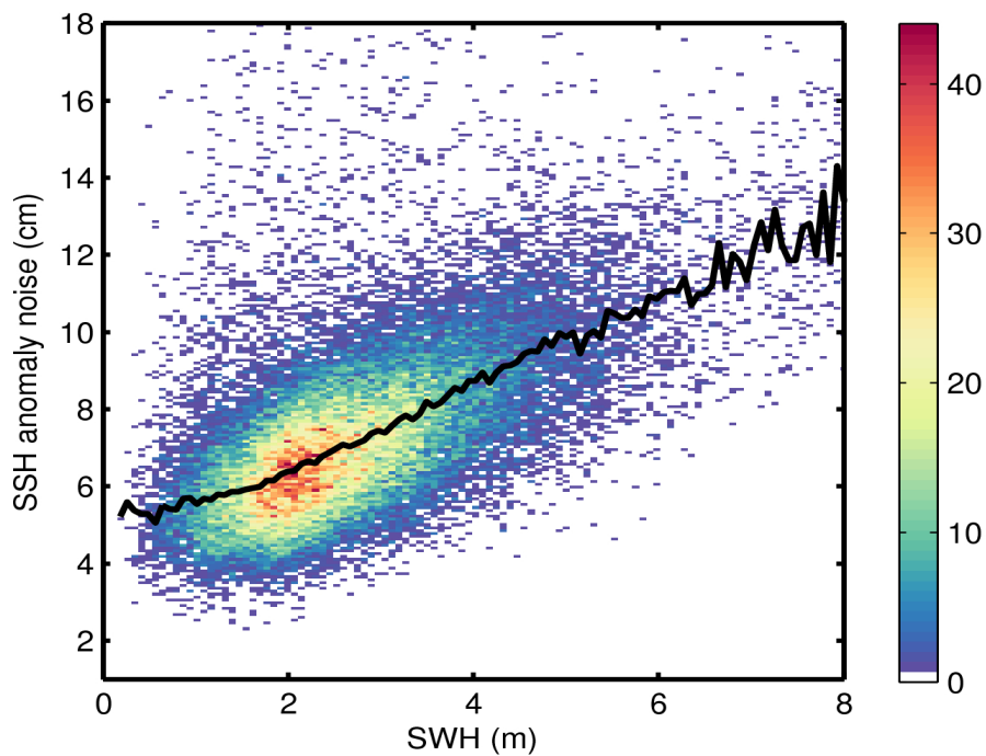
Figure 9. 2D histogram showing flag-valid SSH anomaly noise as a function of SWH for 16/11/2016. The black line denotes the median SSH anomaly noise as a function of SWH.
