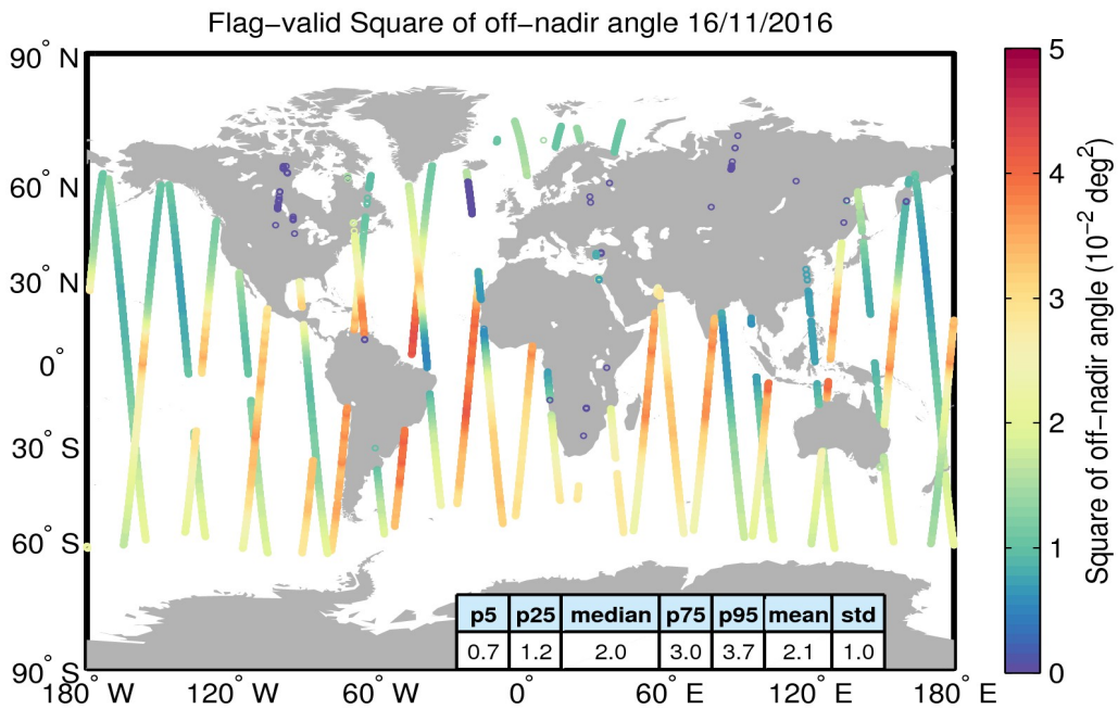
Figure 37. Geographical distribution of flag-valid mispointing data over oceans and lakes for 16/11/2016. The statistical values shown in the table refer to the mispointing in 10^{-2} deg 2 and are calculated over all measurements shown in the figure.
