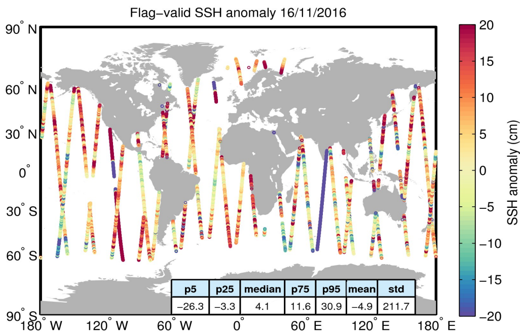
Figure 5. Geographical distribution of flag-valid 1-Hz SSH anomaly data over oceans and lakes for 16/11/2016. The statistical values shown in the table refer to the SSH anomaly in cm and are calculated over all measurements shown in the figure.
