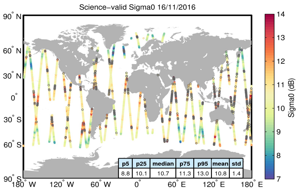
Figure 27. Geographical distribution of science-valid sigma0 data over oceans and lakes for 16/11/2016. The statistical values shown in the table refer to the sigma0 in dB and are calculated over all measurements shown in the figure. Gray circles denote records that have been rejected based on the editing criteria described in Table 4.
