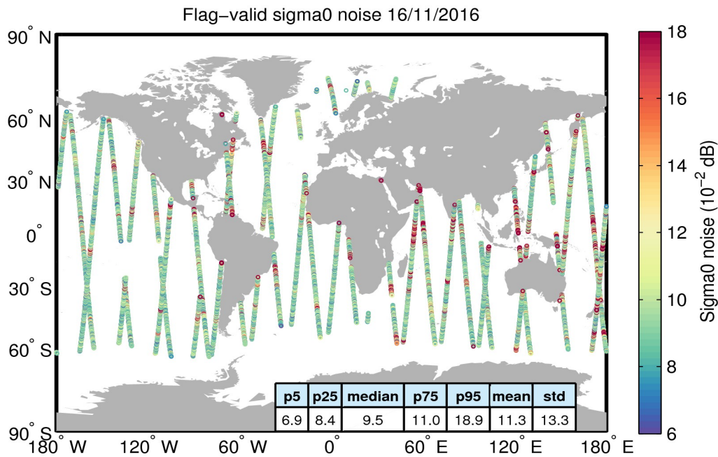
Figure 26. Geographical distribution of flag-valid 20-Hz sigma0 measurement noise over oceans and lakes for 16/11/2016. The statistical values shown in the table refer to the sigma0 noise and are calculated over all measurements shown in the figure.
