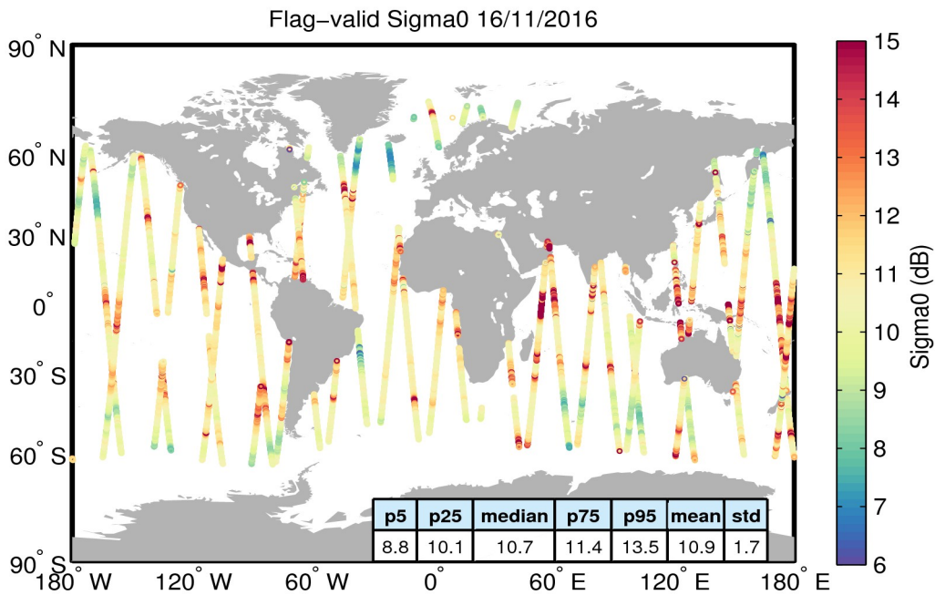
Figure 23. Geographical distribution of flag-valid sigma0 data over oceans and lakes for 16/11/2016. The statistical values shown in the table refer to the sigma0 in dB and are calculated over all measurements shown in the figure.
