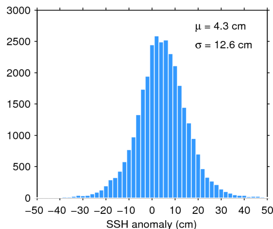
Figure 11. Histogram of science-valid SSH anomaly over oceans and lakes for 16/11/2016. The mean ( \mu ) and standard deviation ( \sigma ) are also shown. Note that values outside [-50 50] cm are excluded from the histogram for the sake of readability but not from the computation of \mu and \sigma .
