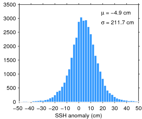
Figure 7. Histogram of flag-valid SSH anomaly over oceans and lakes for 16/11/2016. The mean ( \mu ) and standard deviation ( \sigma ) are also shown. Note that values outside [-50 50] cm are excluded from the histogram for the sake of readability but not from the computation of \mu and \sigma .
