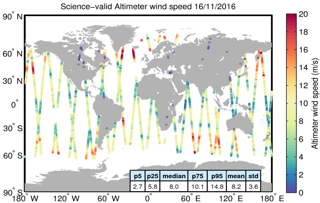
Figure 34. Geographical distribution of science-valid wind data over oceans and lakes for 16/11/2016. The statistical values shown in the table refer to the wind in m/s and are calculated over all measurements shown in the figure. Gray circles denote records that have been rejected based on the editing criteria described in Table 5.
