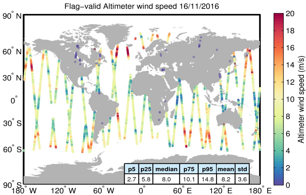
Figure 31. Geographical distribution of flag-valid wind data over oceans and lakes for 16/11/2016. The statistical values shown in the table refer to the wind in m/s and are calculated over all measurements shown in the figure.
