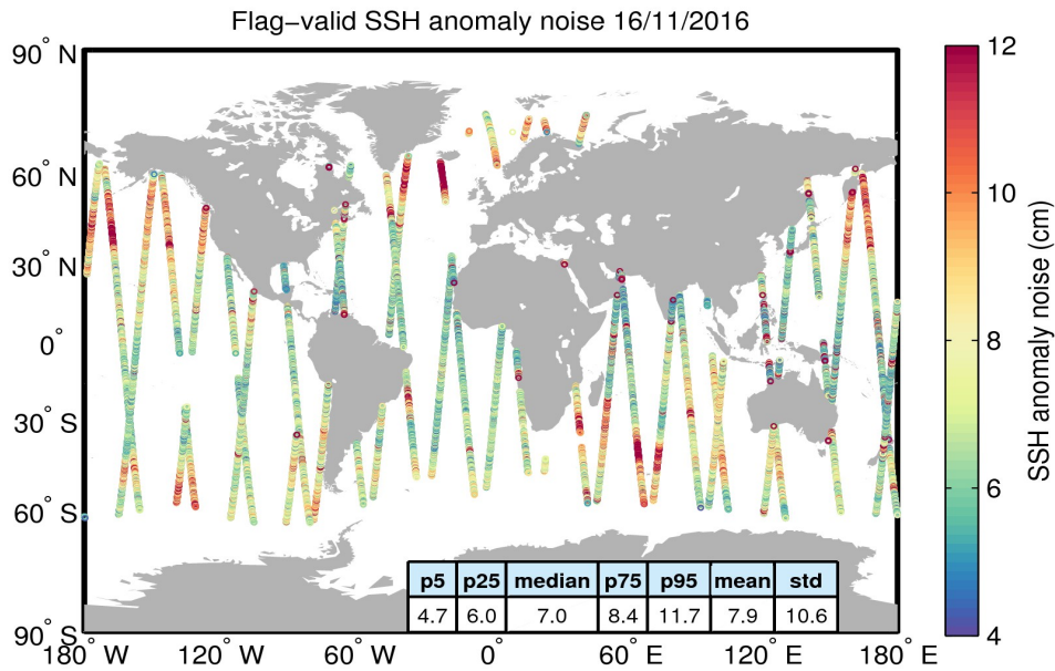
Figure 8. Geographical distribution of flag-valid 20-Hz SSH anomaly measurement noise over oceans and lakes for 16/11/2016. The statistical values shown in the table refer to the SSH anomaly noise and are calculated over all measurements shown in the figure.
