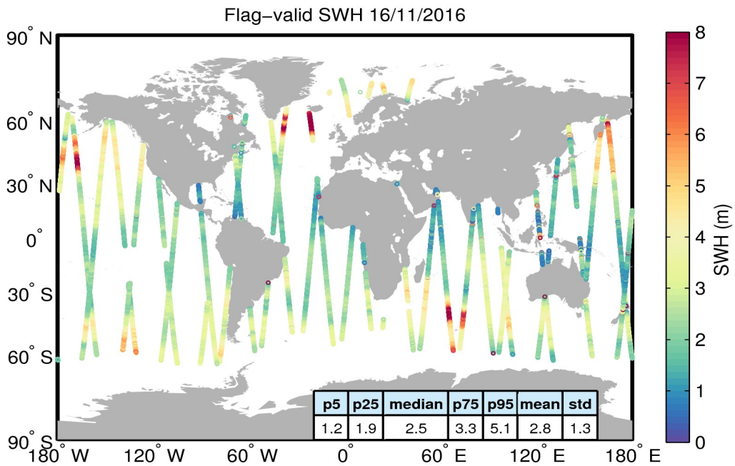
Figure 15. Geographical distribution of flag-valid SWH data over oceans and lakes for 16/11/2016. The statistical values shown in the table refer to the SWH in m and are calculated over all measurements shown in the figure.
