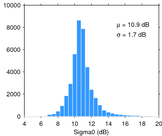
Figure 25. Histogram of flag-valid sigma0 over oceans and lakes for 16/11/2016. The mean ( \mu ) and standard deviation ( \sigma ) are also shown. Note that values outside [4 20] dB are excluded from the histogram for the sake of readability but not from the computation of \mu and \sigma .
