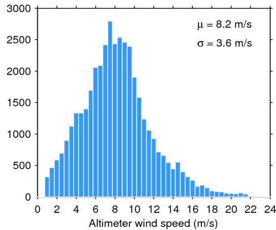
Figure 33. Histogram of flag-valid wind over oceans and lakes for 16/11/2016. The mean ( \mu ) and standard deviation ( \sigma ) are also shown. Note that values larger than 24 m/s are excluded from the histogram for the sake of readability but not from the computation of \mu and \sigma .
