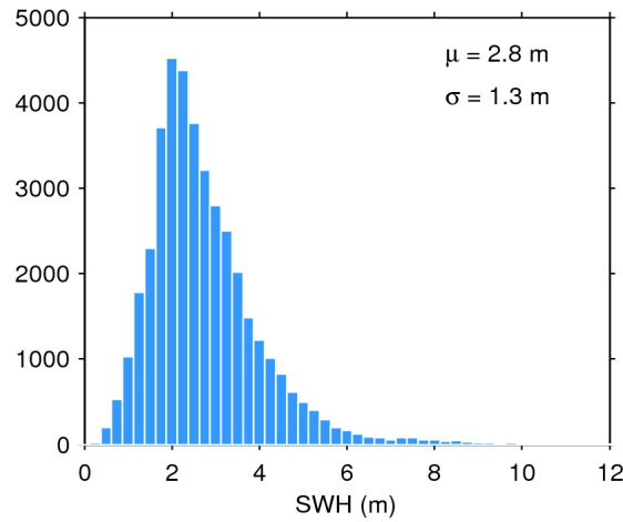
Figure 17. Histogram of flag-valid SWH over oceans and lakes for 16/11/2016. The mean ( \mu ) and standard deviation ( \sigma ) are also shown. Note that values larger than 12 m are excluded from the histogram for the sake of readability but not from the computation of \mu and \sigma .
