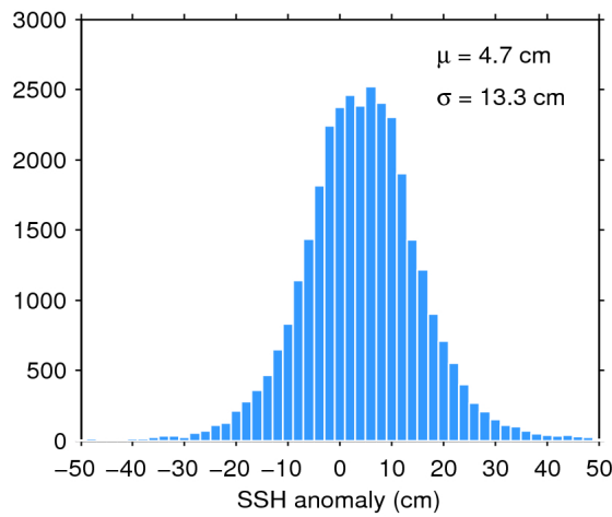
Figure 11. Histogram of science-valid SSH anomaly over oceans and lakes for 14/11/2016. The mean ( \mu ) and standard deviation ( \sigma ) are also shown. Note that values outside [-50 50] cm are excluded from the histogram for the sake of readability but not from the computation of \mu and \sigma .
