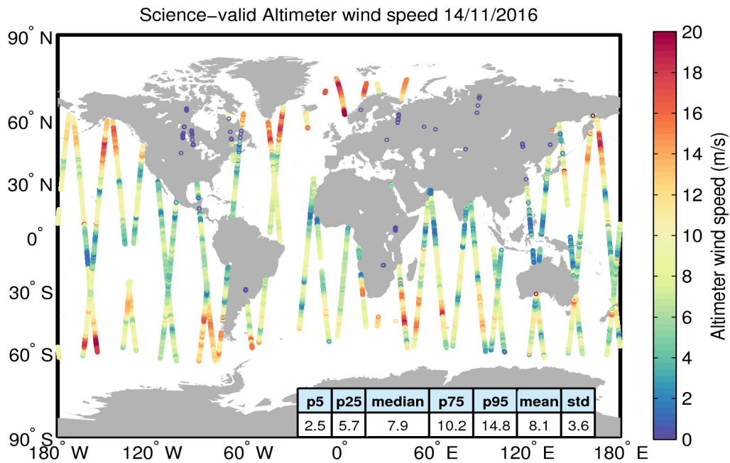
Figure 34. Geographical distribution of science-valid wind data over oceans and lakes for 14/11/2016. The statistical values shown in the table refer to the wind in m/s and are calculated over all measurements shown in the figure. Gray circles denote records that have been rejected based on the editing criteria described in Table 5.
