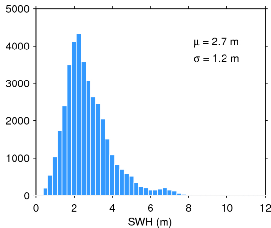
Figure 20. Histogram of science-valid SWH over oceans and lakes for 14/11/2016. The mean ( \mu ) and standard deviation ( \sigma ) are also shown. Note that values larger than 12 m are excluded from the histogram for the sake of readability but not from the computation of \mu and \sigma .
