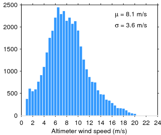
Figure 33. Histogram of flag-valid wind over oceans and lakes for 14/11/2016. The mean ( \mu ) and standard deviation ( \sigma ) are also shown. Note that values larger than 24 m/s are excluded from the histogram for the sake of readability but not from the computation of \mu and \sigma .
