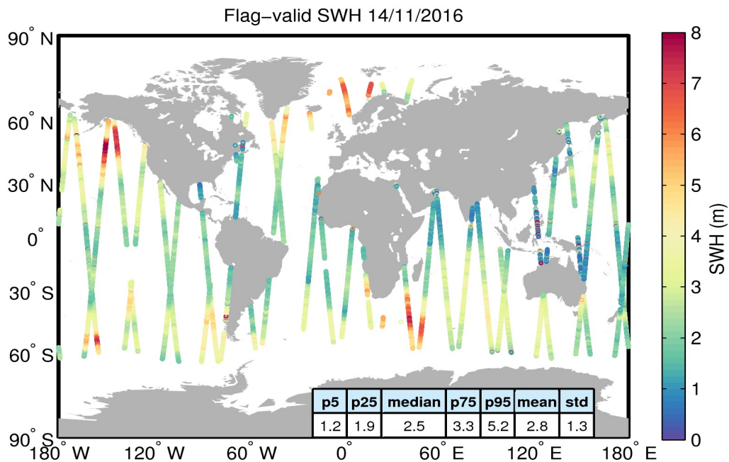
Figure 15. Geographical distribution of flag-valid SWH data over oceans and lakes for 14/11/2016. The statistical values shown in the table refer to the SWH in m and are calculated over all measurements shown in the figure.
