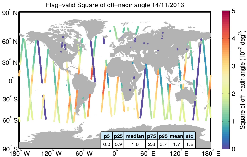
Figure 37. Geographical distribution of flag-valid mispointing data over oceans and lakes for 14/11/2016. The statistical values shown in the table refer to the mispointing in 10^{-2} deg 2 and are calculated over all measurements shown in the figure.
