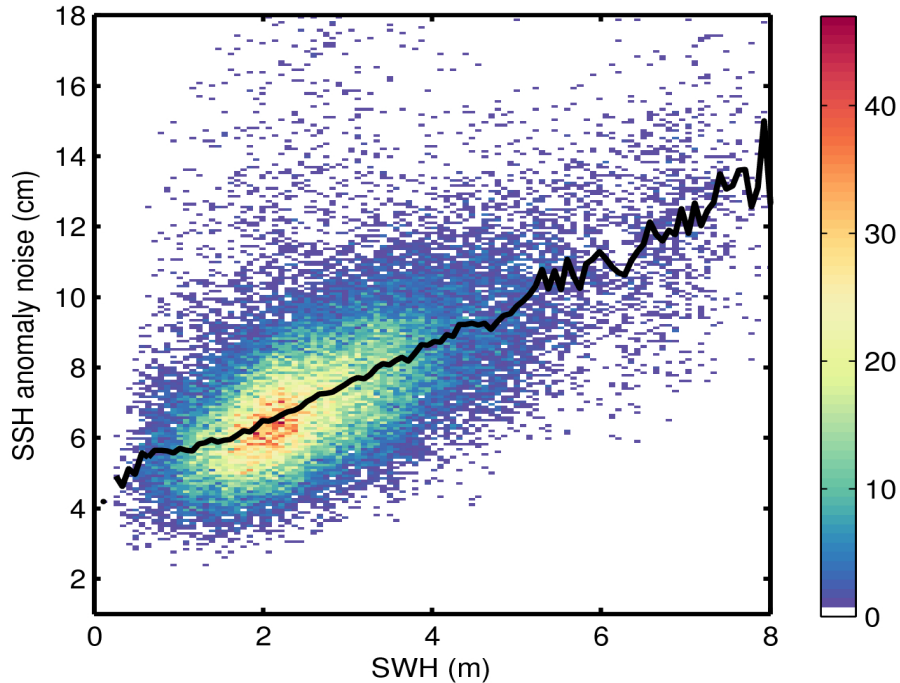
Figure 9. 2D histogram showing flag-valid SSH anomaly noise as a function of SWH for 14/11/2016. The black line denotes the median SSH anomaly noise as a function of SWH.
