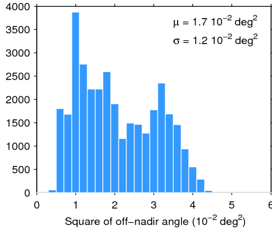
Figure 39. Histogram of flag-valid mispointing over oceans and lakes for 14/11/2016. The mean ( \mu ) and standard deviation ( \sigma ) are also shown. Note that values larger than 6 \cdot 10^{-2} \text{ deg}^2 are excluded from the histogram for the sake of readability but not from the computation of \mu and \sigma .
