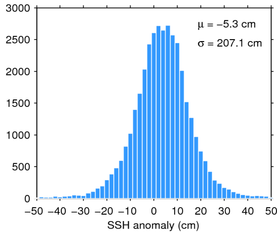
Figure 7. Histogram of flag-valid SSH anomaly over oceans and lakes for 14/11/2016. The mean ( \mu ) and standard deviation ( \sigma ) are also shown. Note that values outside [-50 50] cm are excluded from the histogram for the sake of readability but not from the computation of \mu and \sigma .
