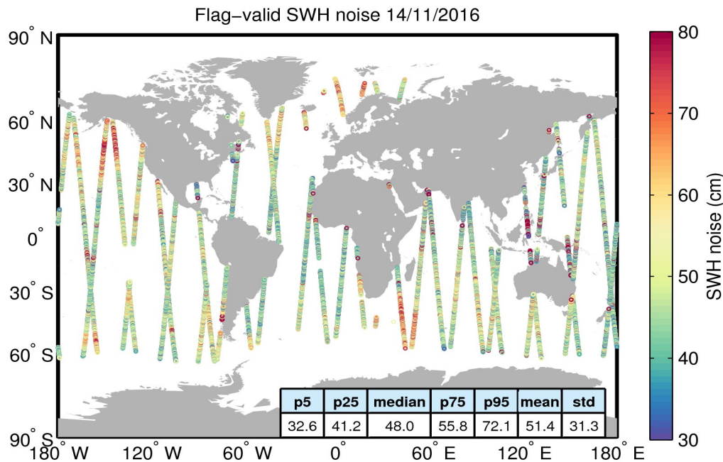
Figure 18. Geographical distribution of flag-valid 20-Hz SWH measurement noise over oceans and lakes for 14/11/2016. The statistical values shown in the table refer to the SWH noise and are calculated over all measurements shown in the figure.
