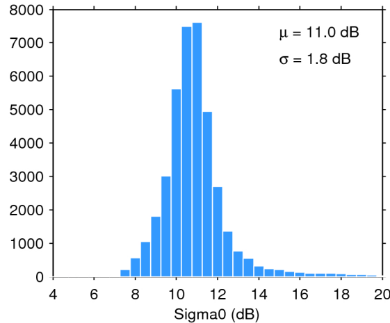
Figure 25. Histogram of flag-valid sigma0 over oceans and lakes for 14/11/2016. The mean ( \mu ) and standard deviation ( \sigma ) are also shown. Note that values outside [4 20] dB are excluded from the histogram for the sake of readability but not from the computation of \mu and \sigma .
