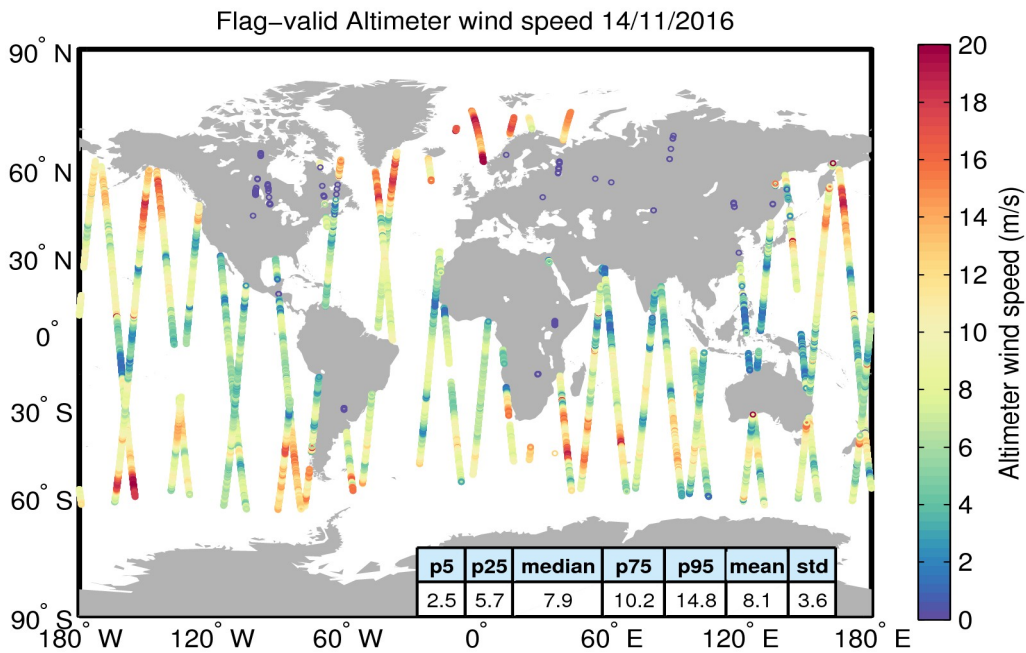
Figure 31. Geographical distribution of flag-valid wind data over oceans and lakes for 14/11/2016. The statistical values shown in the table refer to the wind in m/s and are calculated over all measurements shown in the figure.
