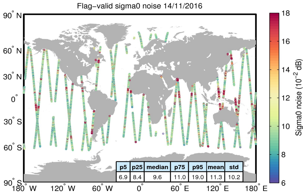
Figure 26. Geographical distribution of flag-valid 20-Hz sigma0 measurement noise over oceans and lakes for 14/11/2016. The statistical values shown in the table refer to the sigma0 noise and are calculated over all measurements shown in the figure.
