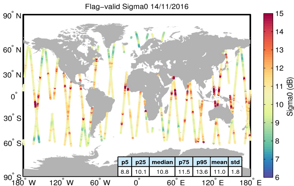
Figure 23. Geographical distribution of flag-valid sigma0 data over oceans and lakes for 14/11/2016. The statistical values shown in the table refer to the sigma0 in dB and are calculated over all measurements shown in the figure.
