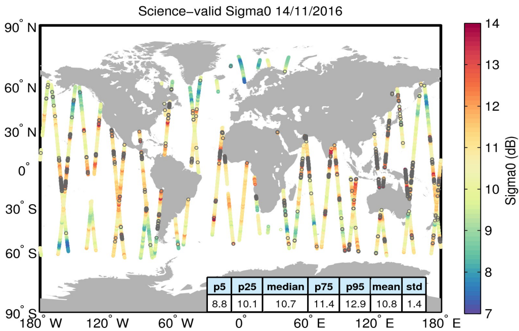
Figure 27. Geographical distribution of science-valid sigma0 data over oceans and lakes for 14/11/2016. The statistical values shown in the table refer to the sigma0 in dB and are calculated over all measurements shown in the figure. Gray circles denote records that have been rejected based on the editing criteria described in Table 4.
