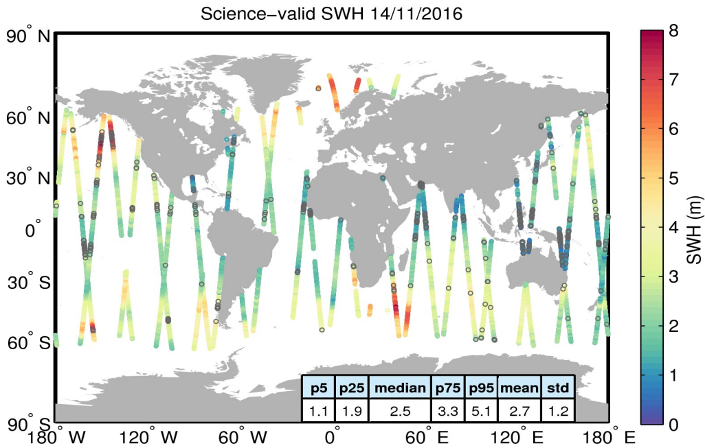
Figure 19. Geographical distribution of science-valid SWH data over oceans and lakes for 14/11/2016. The statistical values shown in the table refer to the SWH in m and are calculated over all measurements shown in the figure. Gray circles denote records that have been rejected based on the editing criteria described in Table 3.
