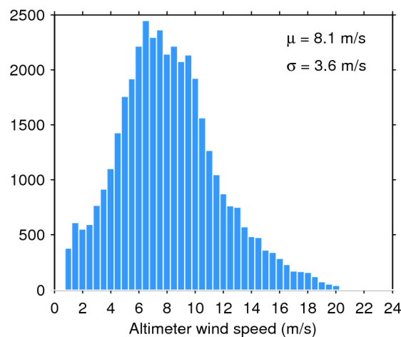
Figure 35. Histogram of science-valid wind over oceans and lakes for 14/11/2016. The mean ( \mu ) and standard deviation ( \sigma ) are also shown. Note that values larger than 24 m/s are excluded from the histogram for the sake of readability but not from the computation of \mu and \sigma .
