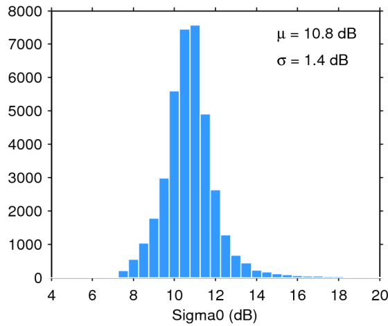
Figure 28. Histogram of science-valid sigma0 over oceans and lakes for 14/11/2016. The mean ( \mu ) and standard deviation ( \sigma ) are also shown. Note that values outside [4 20] dB are excluded from the histogram for the sake of readability but not from the computation of \mu and \sigma .
