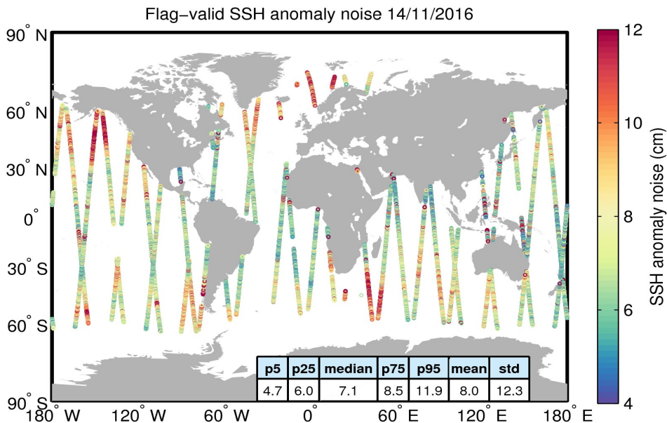
Figure 8. Geographical distribution of flag-valid 20-Hz SSH anomaly measurement noise over oceans and lakes for 14/11/2016. The statistical values shown in the table refer to the SSH anomaly noise and are calculated over all measurements shown in the figure.
