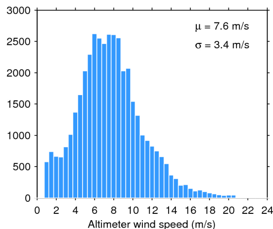
Figure 35. Histogram of science-valid wind over oceans and lakes for 13/11/2016. The mean ( \mu ) and standard deviation ( \sigma ) are also shown. Note that values larger than 24 m/s are excluded from the histogram for the sake of readability but not from the computation of \mu and \sigma .
