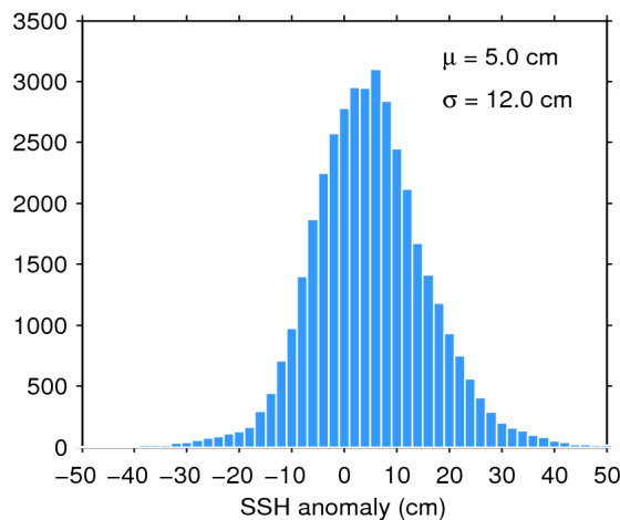
Figure 11. Histogram of science-valid SSH anomaly over oceans and lakes for 13/11/2016. The mean ( \mu ) and standard deviation ( \sigma ) are also shown. Note that values outside [-50 50] cm are excluded from the histogram for the sake of readability but not from the computation of \mu and \sigma .
