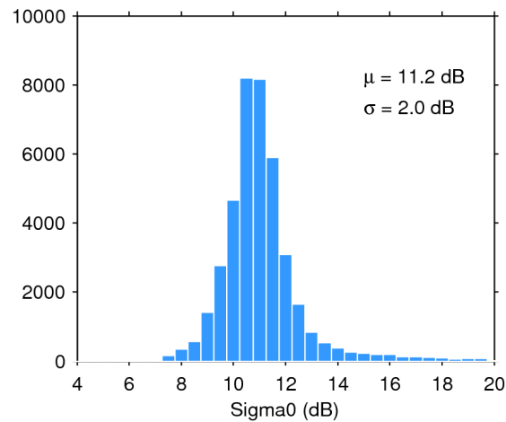
Figure 25. Histogram of flag-valid sigma0 over oceans and lakes for 13/11/2016. The mean ( \mu ) and standard deviation ( \sigma ) are also shown. Note that values outside [4 20] dB are excluded from the histogram for the sake of readability but not from the computation of \mu and \sigma .
