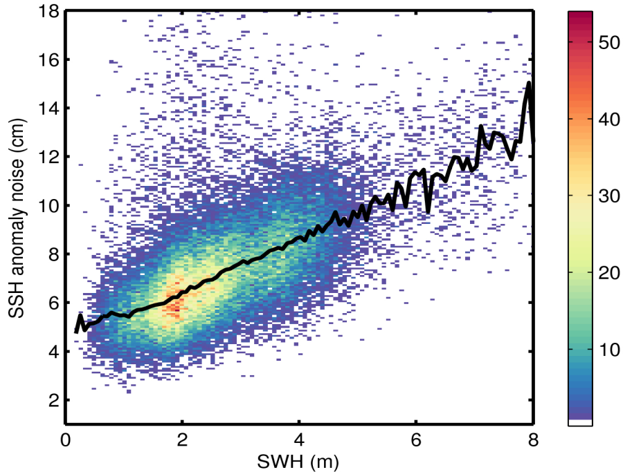
Figure 9. 2D histogram showing flag-valid SSH anomaly noise as a function of SWH for 13/11/2016. The black line denotes the median SSH anomaly noise as a function of SWH.
