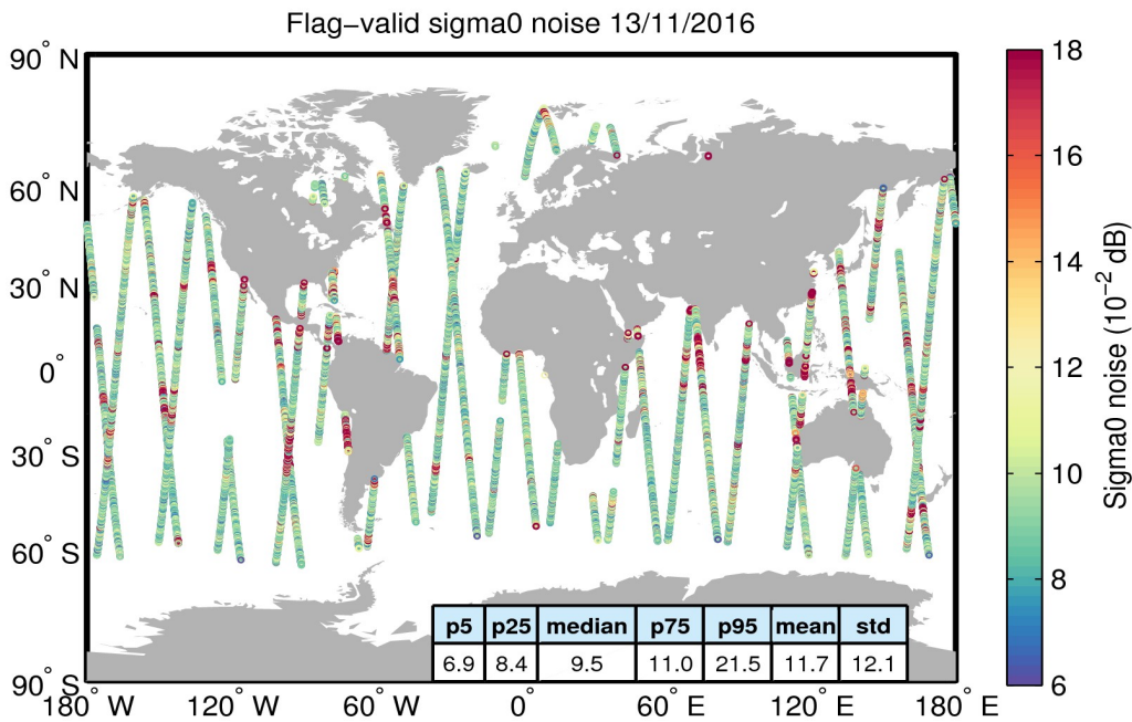
Figure 26. Geographical distribution of flag-valid 20-Hz sigma0 measurement noise over oceans and lakes for 13/11/2016. The statistical values shown in the table refer to the sigma0 noise and are calculated over all measurements shown in the figure.
