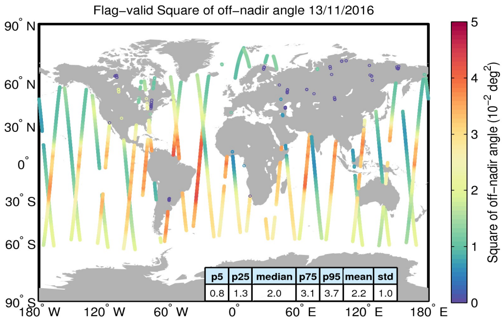
Figure 37. Geographical distribution of flag-valid mispointing data over oceans and lakes for 13/11/2016. The statistical values shown in the table refer to the mispointing in 10^{-2} deg 2 and are calculated over all measurements shown in the figure.
