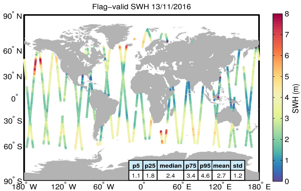
Figure 15. Geographical distribution of flag-valid SWH data over oceans and lakes for 13/11/2016. The statistical values shown in the table refer to the SWH in m and are calculated over all measurements shown in the figure.
