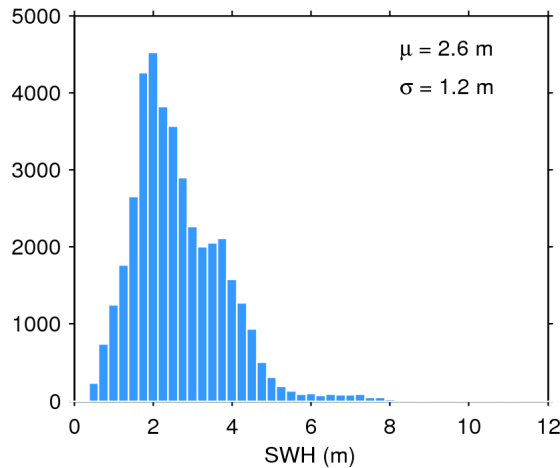
Figure 20. Histogram of science-valid SWH over oceans and lakes for 13/11/2016. The mean ( \mu ) and standard deviation ( \sigma ) are also shown. Note that values larger than 12 m are excluded from the histogram for the sake of readability but not from the computation of \mu and \sigma .
