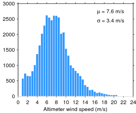
Figure 33. Histogram of flag-valid wind over oceans and lakes for 13/11/2016. The mean ( \mu ) and standard deviation ( \sigma ) are also shown. Note that values larger than 24 m/s are excluded from the histogram for the sake of readability but not from the computation of \mu and \sigma .
