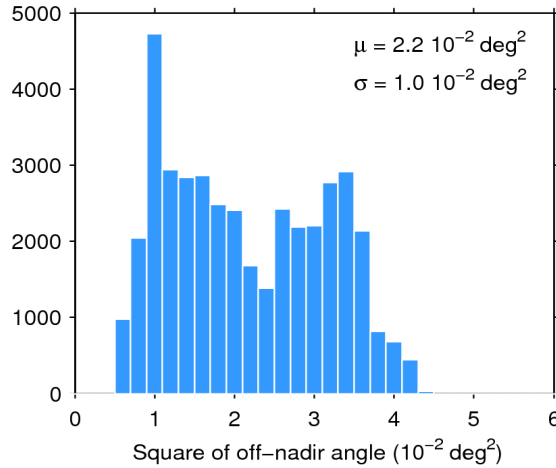
Figure 39. Histogram of flag-valid mispointing over oceans and lakes for 13/11/2016. The mean ( \mu ) and standard deviation ( \sigma ) are also shown. Note that values larger than 6 \cdot 10^{-2} \text{ deg}^2 are excluded from the histogram for the sake of readability but not from the computation of \mu and \sigma .
