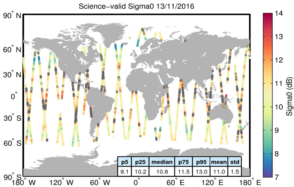
Figure 27. Geographical distribution of science-valid sigma0 data over oceans and lakes for 13/11/2016. The statistical values shown in the table refer to the sigma0 in dB and are calculated over all measurements shown in the figure. Gray circles denote records that have been rejected based on the editing criteria described in Table 4.
