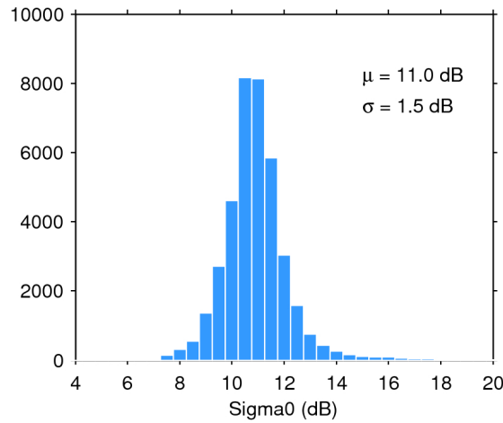
Figure 28. Histogram of science-valid sigma0 over oceans and lakes for 13/11/2016. The mean ( \mu ) and standard deviation ( \sigma ) are also shown. Note that values outside [4 20] dB are excluded from the histogram for the sake of readability but not from the computation of \mu and \sigma .
