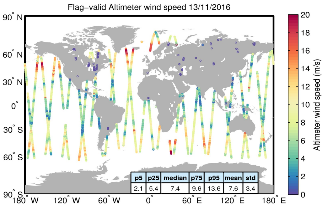
Figure 31. Geographical distribution of flag-valid wind data over oceans and lakes for 13/11/2016. The statistical values shown in the table refer to the wind in m/s and are calculated over all measurements shown in the figure.
