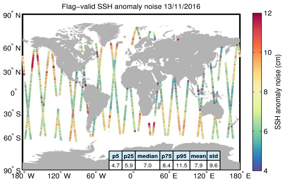
Figure 8. Geographical distribution of flag-valid 20-Hz SSH anomaly measurement noise over oceans and lakes for 13/11/2016. The statistical values shown in the table refer to the SSH anomaly noise and are calculated over all measurements shown in the figure.
