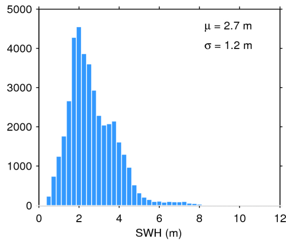
Figure 17. Histogram of flag-valid SWH over oceans and lakes for 13/11/2016. The mean ( \mu ) and standard deviation ( \sigma ) are also shown. Note that values larger than 12 m are excluded from the histogram for the sake of readability but not from the computation of \mu and \sigma .
