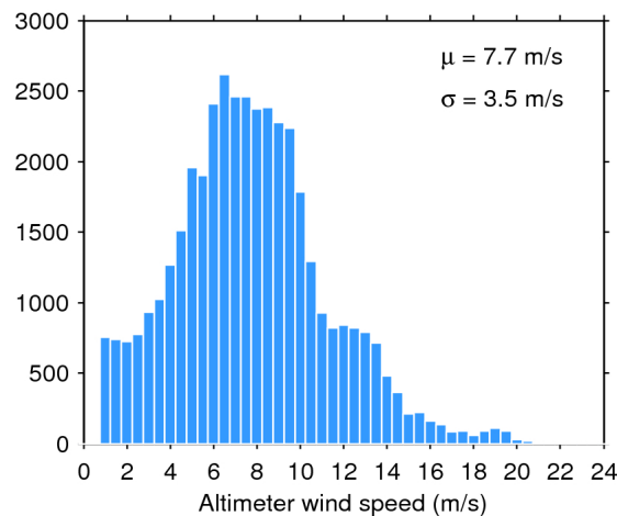
Figure 35. Histogram of science-valid wind over oceans and lakes for 12/11/2016. The mean ( \mu ) and standard deviation ( \sigma ) are also shown. Note that values larger than 24 m/s are excluded from the histogram for the sake of readability but not from the computation of \mu and \sigma .
