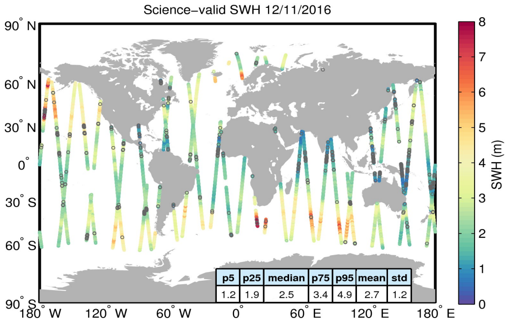
Figure 19. Geographical distribution of science-valid SWH data over oceans and lakes for 12/11/2016. The statistical values shown in the table refer to the SWH in m and are calculated over all measurements shown in the figure. Gray circles denote records that have been rejected based on the editing criteria described in Table 3.
