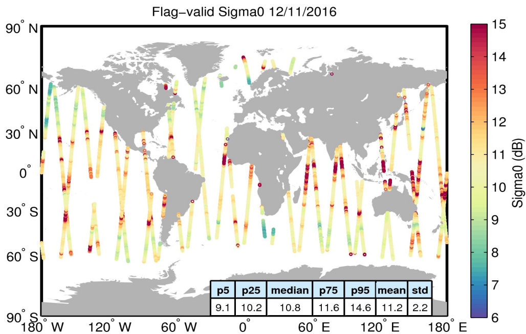
Figure 23. Geographical distribution of flag-valid sigma0 data over oceans and lakes for 12/11/2016. The statistical values shown in the table refer to the sigma0 in dB and are calculated over all measurements shown in the figure.
