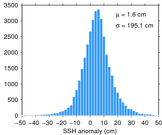
Figure 7. Histogram of flag-valid SSH anomaly over oceans and lakes for 12/11/2016. The mean ( \mu ) and standard deviation ( \sigma ) are also shown. Note that values outside [-50\ 50] cm are excluded from the histogram for the sake of readability but not from the computation of \mu and \sigma .
