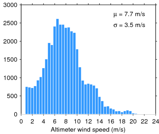
Figure 33. Histogram of flag-valid wind over oceans and lakes for 12/11/2016. The mean ( \mu ) and standard deviation ( \sigma ) are also shown. Note that values larger than 24 m/s are excluded from the histogram for the sake of readability but not from the computation of \mu and \sigma .
