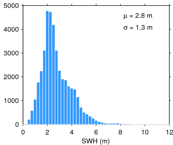
Figure 17. Histogram of flag-valid SWH over oceans and lakes for 12/11/2016. The mean ( \mu ) and standard deviation ( \sigma ) are also shown. Note that values larger than 12 m are excluded from the histogram for the sake of readability but not from the computation of \mu and \sigma .
