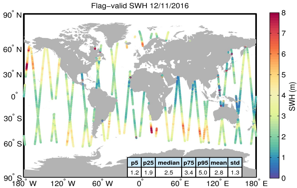
Figure 15. Geographical distribution of flag-valid SWH data over oceans and lakes for 12/11/2016. The statistical values shown in the table refer to the SWH in m and are calculated over all measurements shown in the figure.
