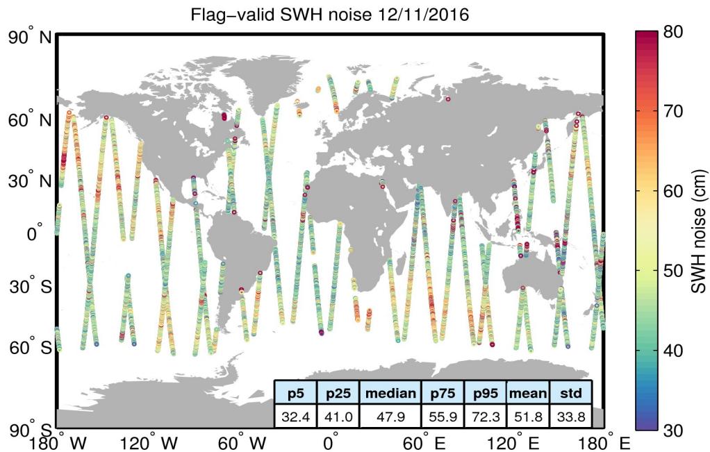
Figure 18. Geographical distribution of flag-valid 20-Hz SWH measurement noise over oceans and lakes for 12/11/2016. The statistical values shown in the table refer to the SWH noise and are calculated over all measurements shown in the figure.
