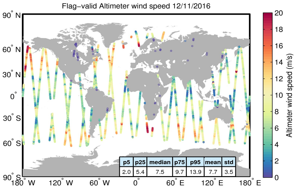
Figure 31. Geographical distribution of flag-valid wind data over oceans and lakes for 12/11/2016. The statistical values shown in the table refer to the wind in m/s and are calculated over all measurements shown in the figure.
