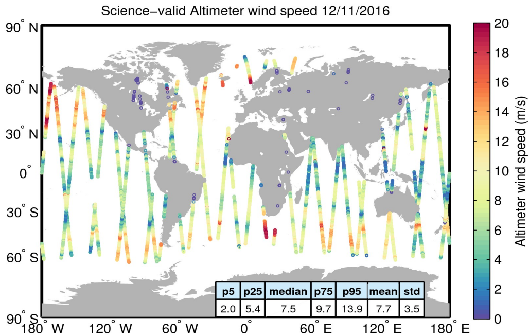
Figure 34. Geographical distribution of science-valid wind data over oceans and lakes for 12/11/2016. The statistical values shown in the table refer to the wind in m/s and are calculated over all measurements shown in the figure. Gray circles denote records that have been rejected based on the editing criteria described in Table 5.
