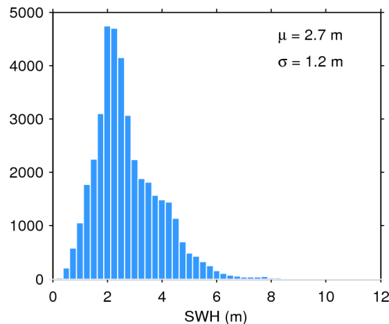
Figure 20. Histogram of science-valid SWH over oceans and lakes for 12/11/2016. The mean ( \mu ) and standard deviation ( \sigma ) are also shown. Note that values larger than 12 m are excluded from the histogram for the sake of readability but not from the computation of \mu and \sigma .
