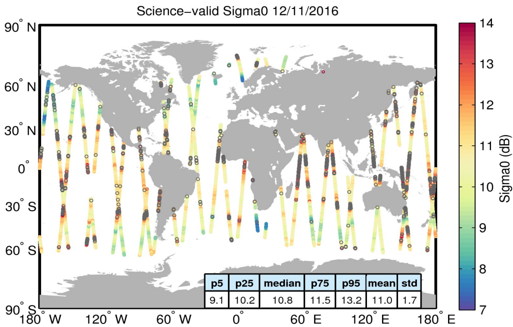
Figure 27. Geographical distribution of science-valid sigma0 data over oceans and lakes for 12/11/2016. The statistical values shown in the table refer to the sigma0 in dB and are calculated over all measurements shown in the figure. Gray circles denote records that have been rejected based on the editing criteria described in Table 4.
