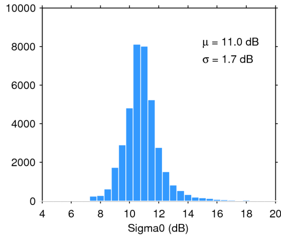
Figure 28. Histogram of science-valid sigma0 over oceans and lakes for 12/11/2016. The mean ( \mu ) and standard deviation ( \sigma ) are also shown. Note that values outside [4 20] dB are excluded from the histogram for the sake of readability but not from the computation of \mu and \sigma .
