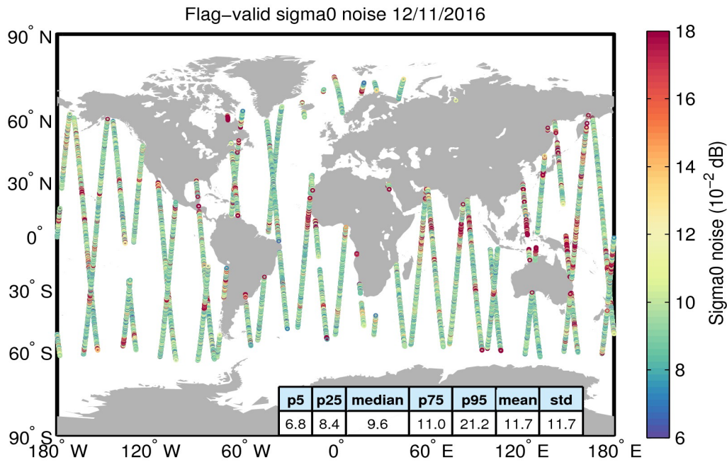
Figure 26. Geographical distribution of flag-valid 20-Hz sigma0 measurement noise over oceans and lakes for 12/11/2016. The statistical values shown in the table refer to the sigma0 noise and are calculated over all measurements shown in the figure.
