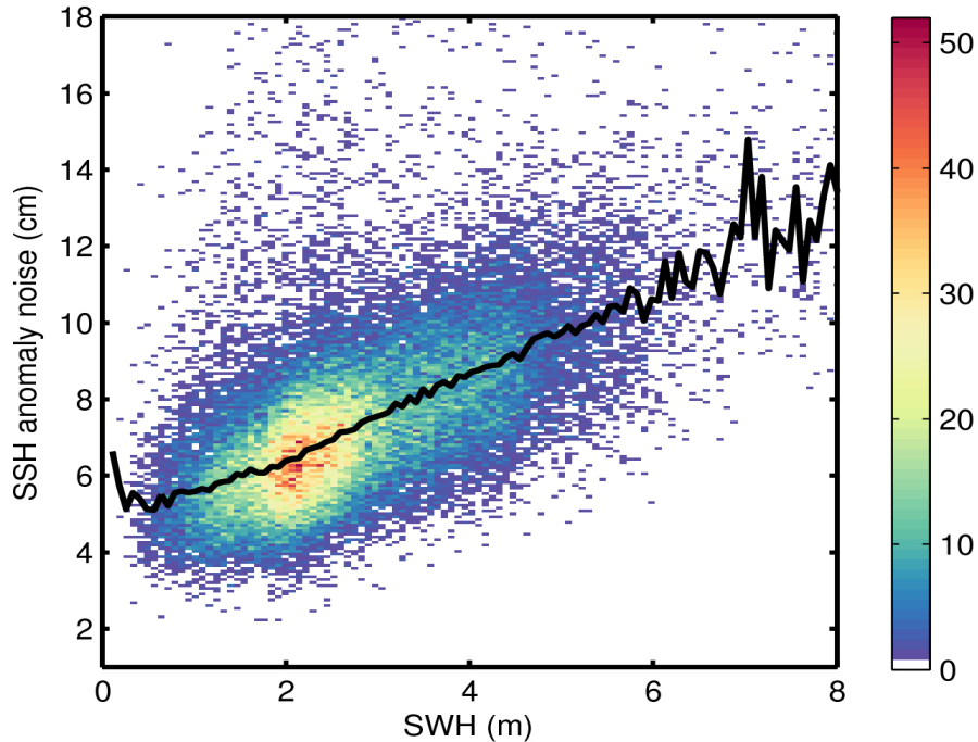
Figure 9. 2D histogram showing flag-valid SSH anomaly noise as a function of SWH for 12/11/2016. The black line denotes the median SSH anomaly noise as a function of SWH.
