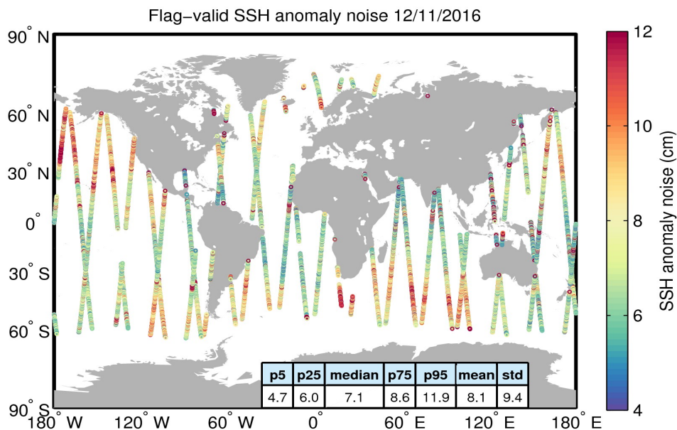
Figure 8. Geographical distribution of flag-valid 20-Hz SSH anomaly measurement noise over oceans and lakes for 12/11/2016. The statistical values shown in the table refer to the SSH anomaly noise and are calculated over all measurements shown in the figure.
