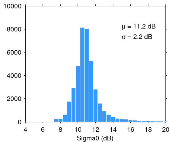
Figure 25. Histogram of flag-valid sigma0 over oceans and lakes for 12/11/2016. The mean ( \mu ) and standard deviation ( \sigma ) are also shown. Note that values outside [4 20] dB are excluded from the histogram for the sake of readability but not from the computation of \mu and \sigma .
