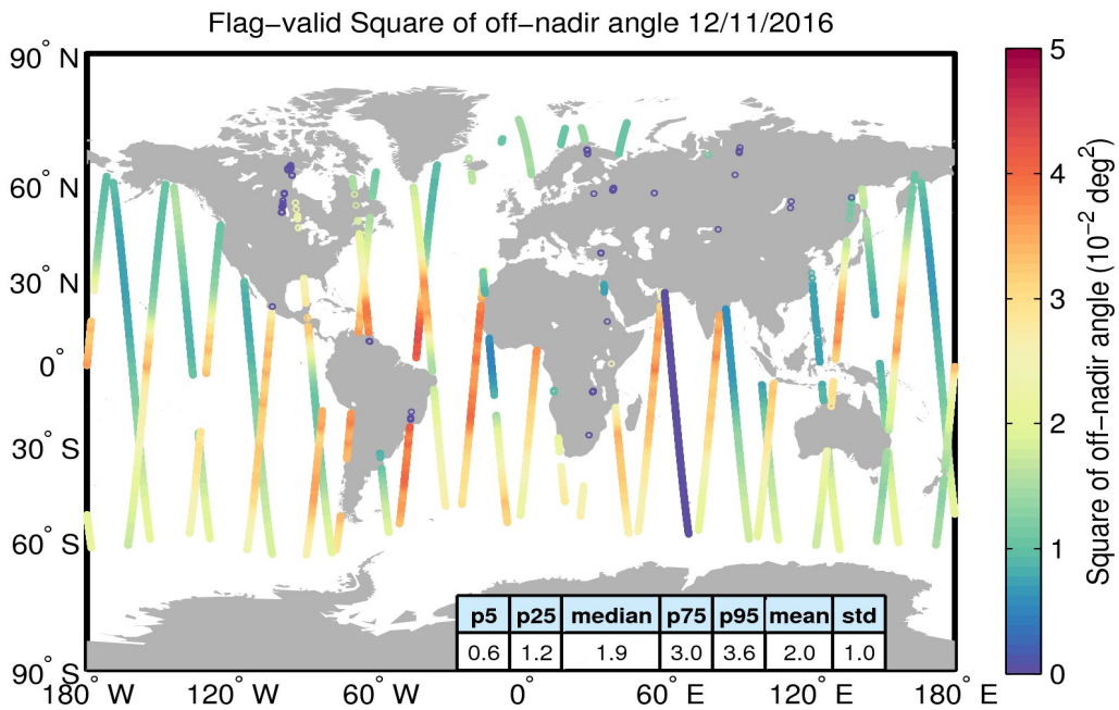
Figure 37. Geographical distribution of flag-valid mispointing data over oceans and lakes for 12/11/2016. The statistical values shown in the table refer to the mispointing in 10^{-2} deg 2 and are calculated over all measurements shown in the figure.
