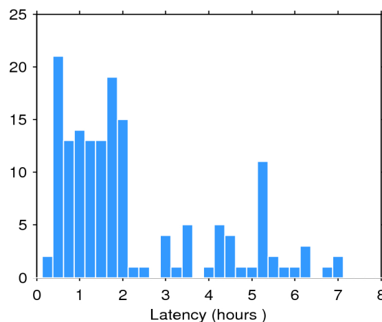
Figure 2. Histogram of the data latency for 12/11/2016. The y-axis denotes the number of files that are made available with a delay of x-hours with respect to the mean time of the records stored in the file.
