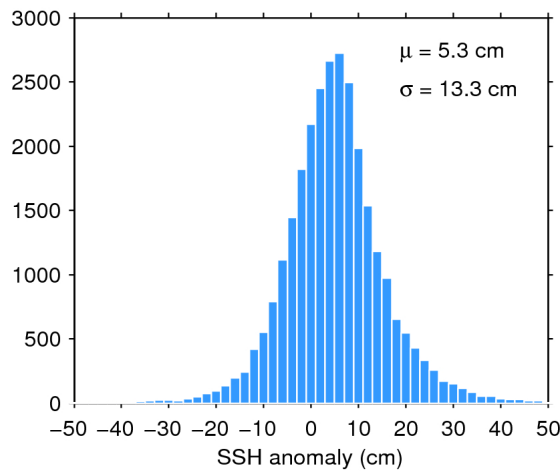
Figure 11. Histogram of science-valid SSH anomaly over oceans and lakes for 12/11/2016. The mean ( \mu ) and standard deviation ( \sigma ) are also shown. Note that values outside [-50 50] cm are excluded from the histogram for the sake of readability but not from the computation of \mu and \sigma .
