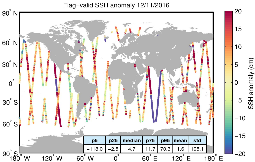
Figure 5. Geographical distribution of flag-valid 1-Hz SSH anomaly data over oceans and lakes for 12/11/2016. The statistical values shown in the table refer to the SSH anomaly in cm and are calculated over all measurements shown in the figure.
