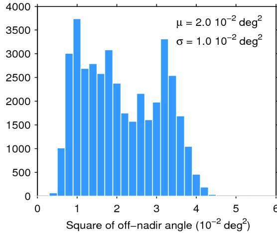
Figure 39. Histogram of flag-valid mispointing over oceans and lakes for 12/11/2016. The mean ( \mu ) and standard deviation ( \sigma ) are also shown. Note that values larger than 6 \cdot 10^{-2} \text{ deg}^2 are excluded from the histogram for the sake of readability but not from the computation of \mu and \sigma .
