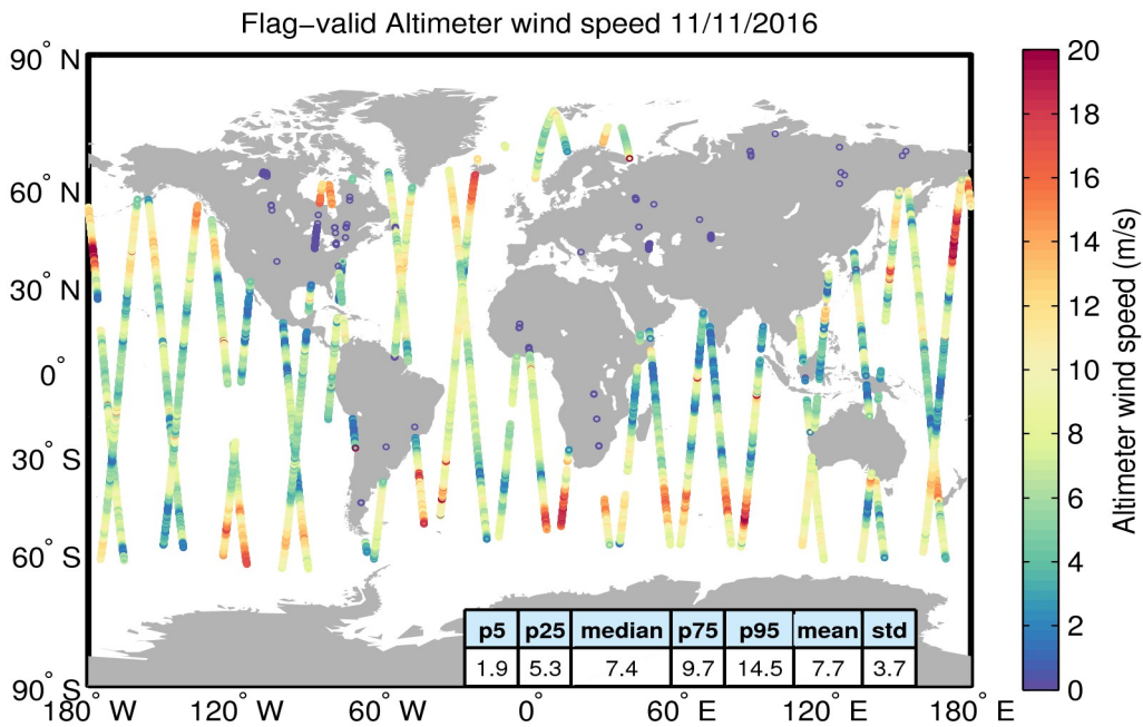
Figure 31. Geographical distribution of flag-valid wind data over oceans and lakes for 11/11/2016. The statistical values shown in the table refer to the wind in m/s and are calculated over all measurements shown in the figure.
