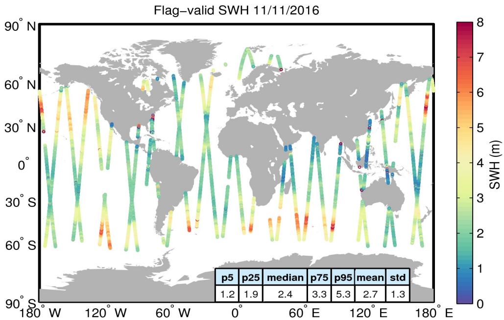
Figure 15. Geographical distribution of flag-valid SWH data over oceans and lakes for 11/11/2016. The statistical values shown in the table refer to the SWH in m and are calculated over all measurements shown in the figure.
