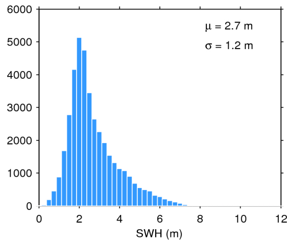
Figure 20. Histogram of science-valid SWH over oceans and lakes for 11/11/2016. The mean ( \mu ) and standard deviation ( \sigma ) are also shown. Note that values larger than 12 m are excluded from the histogram for the sake of readability but not from the computation of \mu and \sigma .
