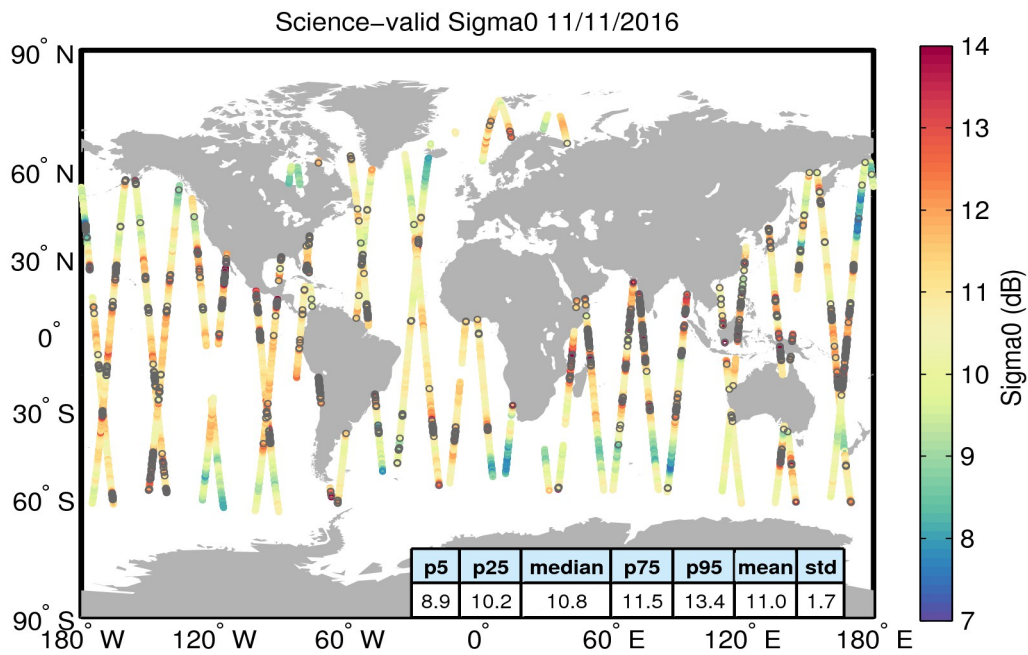
Figure 27. Geographical distribution of science-valid sigma0 data over oceans and lakes for 11/11/2016. The statistical values shown in the table refer to the sigma0 in dB and are calculated over all measurements shown in the figure. Gray circles denote records that have been rejected based on the editing criteria described in Table 4.
