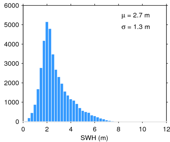
Figure 17. Histogram of flag-valid SWH over oceans and lakes for 11/11/2016. The mean ( \mu ) and standard deviation ( \sigma ) are also shown. Note that values larger than 12 m are excluded from the histogram for the sake of readability but not from the computation of \mu and \sigma .
