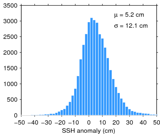
Figure 11. Histogram of science-valid SSH anomaly over oceans and lakes for 11/11/2016. The mean ( \mu ) and standard deviation ( \sigma ) are also shown. Note that values outside [-50 50] cm are excluded from the histogram for the sake of readability but not from the computation of \mu and \sigma .
