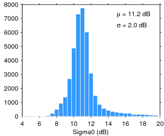
Figure 25. Histogram of flag-valid sigma0 over oceans and lakes for 11/11/2016. The mean ( \mu ) and standard deviation ( \sigma ) are also shown. Note that values outside [4 20] dB are excluded from the histogram for the sake of readability but not from the computation of \mu and \sigma .
