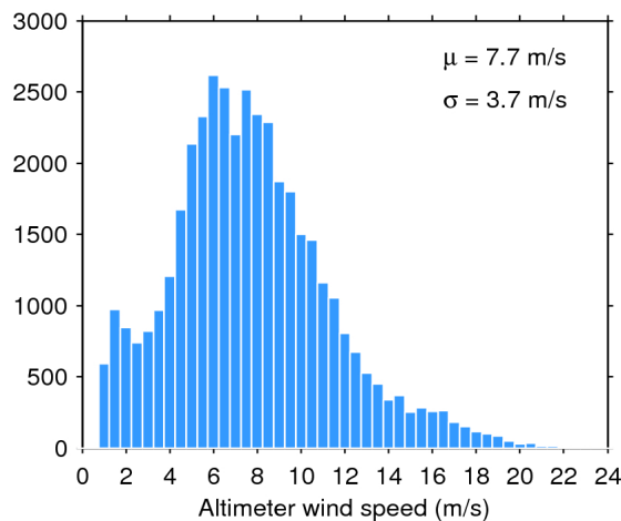
Figure 35. Histogram of science-valid wind over oceans and lakes for 11/11/2016. The mean ( \mu ) and standard deviation ( \sigma ) are also shown. Note that values larger than 24 m/s are excluded from the histogram for the sake of readability but not from the computation of \mu and \sigma .
