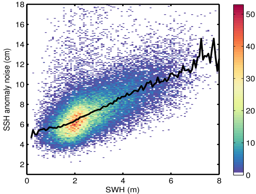
Figure 9. 2D histogram showing flag-valid SSH anomaly noise as a function of SWH for 11/11/2016. The black line denotes the median SSH anomaly noise as a function of SWH.
