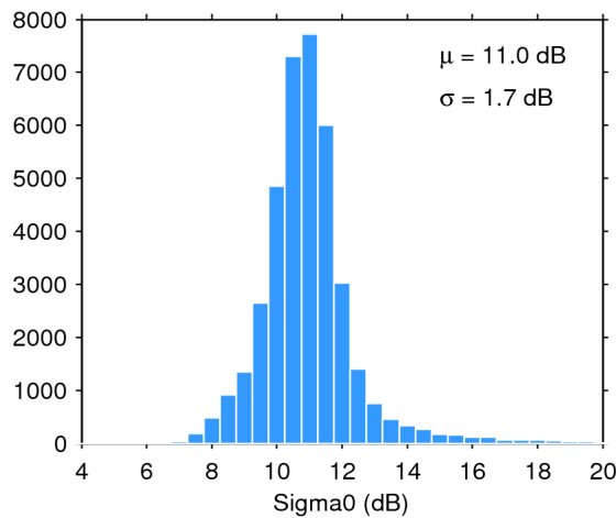
Figure 28. Histogram of science-valid sigma0 over oceans and lakes for 11/11/2016. The mean ( \mu ) and standard deviation ( \sigma ) are also shown. Note that values outside [4 20] dB are excluded from the histogram for the sake of readability but not from the computation of \mu and \sigma .
