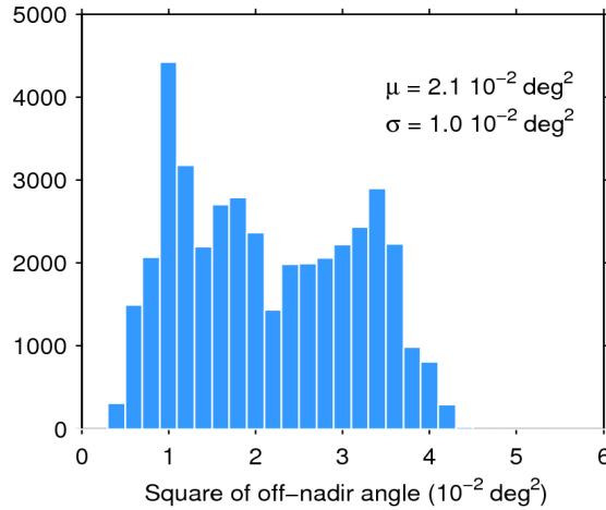
Figure 39. Histogram of flag-valid mispointing over oceans and lakes for 11/11/2016. The mean ( \mu ) and standard deviation ( \sigma ) are also shown. Note that values larger than 6 \cdot 10^{-2} \text{ deg}^2 are excluded from the histogram for the sake of readability but not from the computation of \mu and \sigma .
