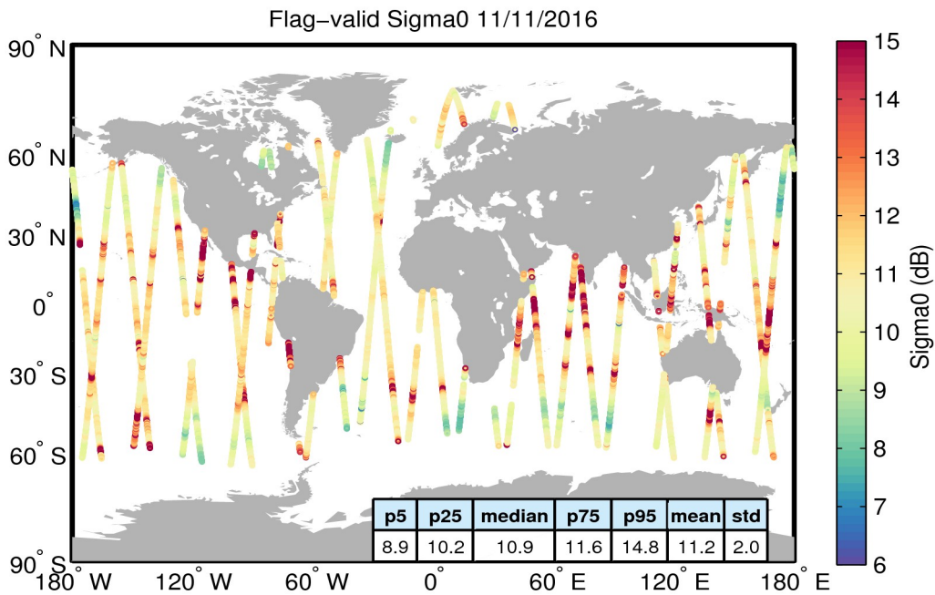
Figure 23. Geographical distribution of flag-valid sigma0 data over oceans and lakes for 11/11/2016. The statistical values shown in the table refer to the sigma0 in dB and are calculated over all measurements shown in the figure.
