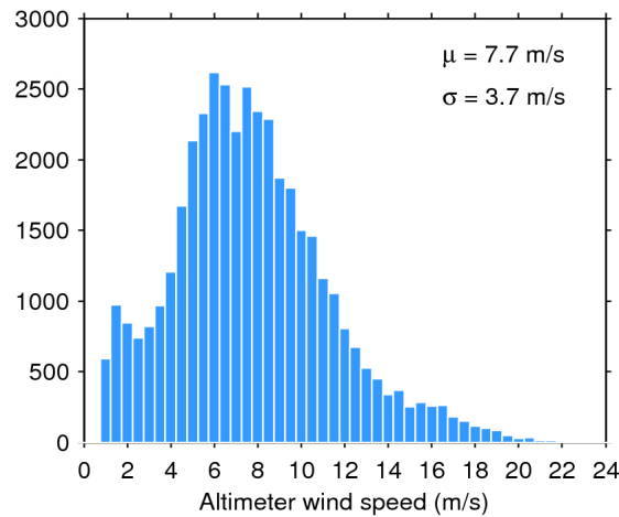
Figure 33. Histogram of flag-valid wind over oceans and lakes for 11/11/2016. The mean ( \mu ) and standard deviation ( \sigma ) are also shown. Note that values larger than 24 m/s are excluded from the histogram for the sake of readability but not from the computation of \mu and \sigma .
