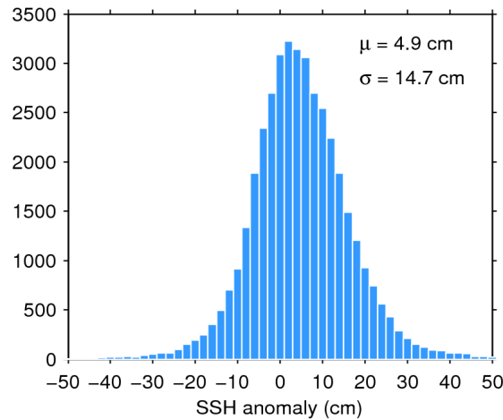
Figure 7. Histogram of flag-valid SSH anomaly over oceans and lakes for 11/11/2016. The mean ( \mu ) and standard deviation ( \sigma ) are also shown. Note that values outside [-50\ 50] cm are excluded from the histogram for the sake of readability but not from the computation of \mu and \sigma .
