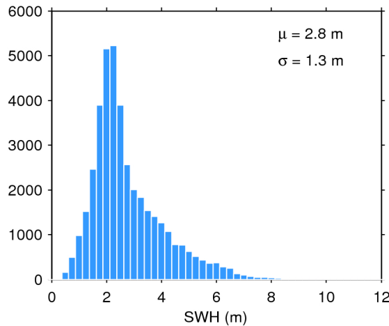
Figure 20. Histogram of science-valid SWH over oceans and lakes for 10/11/2016. The mean ( \mu ) and standard deviation ( \sigma ) are also shown. Note that values larger than 12 m are excluded from the histogram for the sake of readability but not from the computation of \mu and \sigma .
