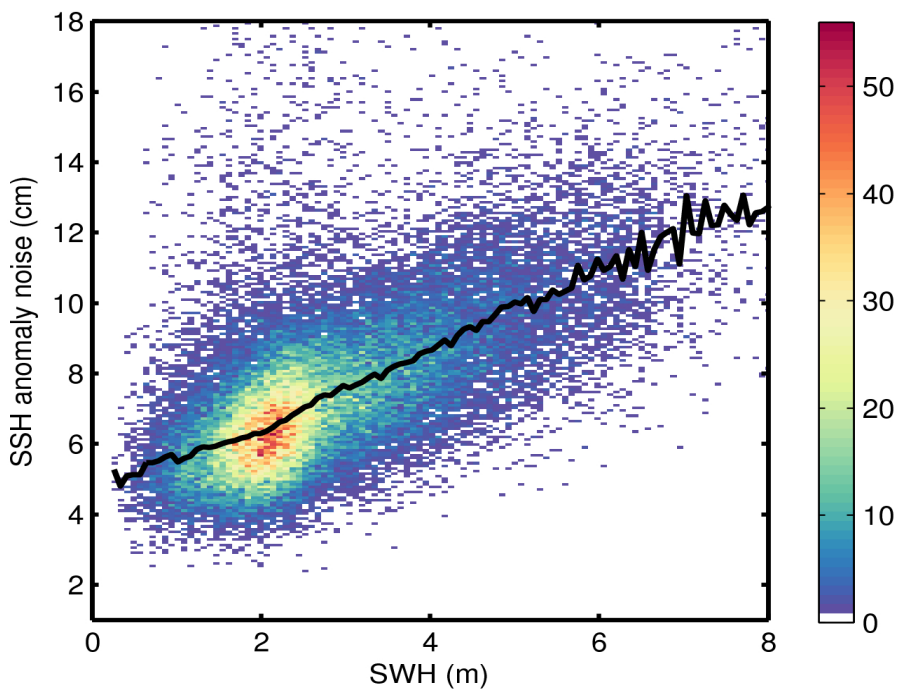
Figure 9. 2D histogram showing flag-valid SSH anomaly noise as a function of SWH for 10/11/2016. The black line denotes the median SSH anomaly noise as a function of SWH.
