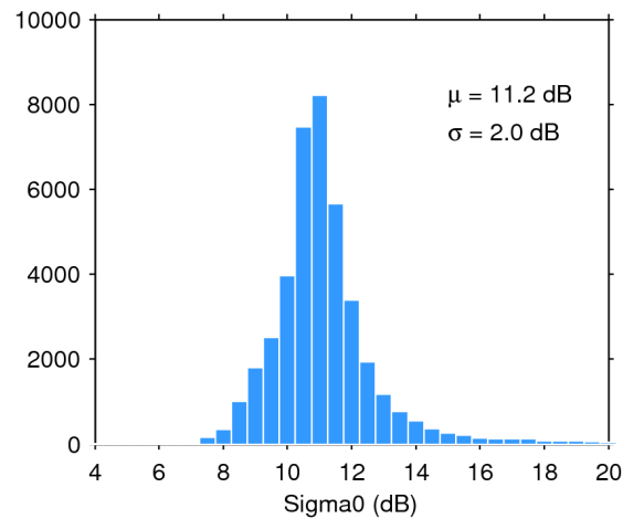
Figure 25. Histogram of flag-valid sigma0 over oceans and lakes for 10/11/2016. The mean ( \mu ) and standard deviation ( \sigma ) are also shown. Note that values outside [4 20] dB are excluded from the histogram for the sake of readability but not from the computation of \mu and \sigma .
