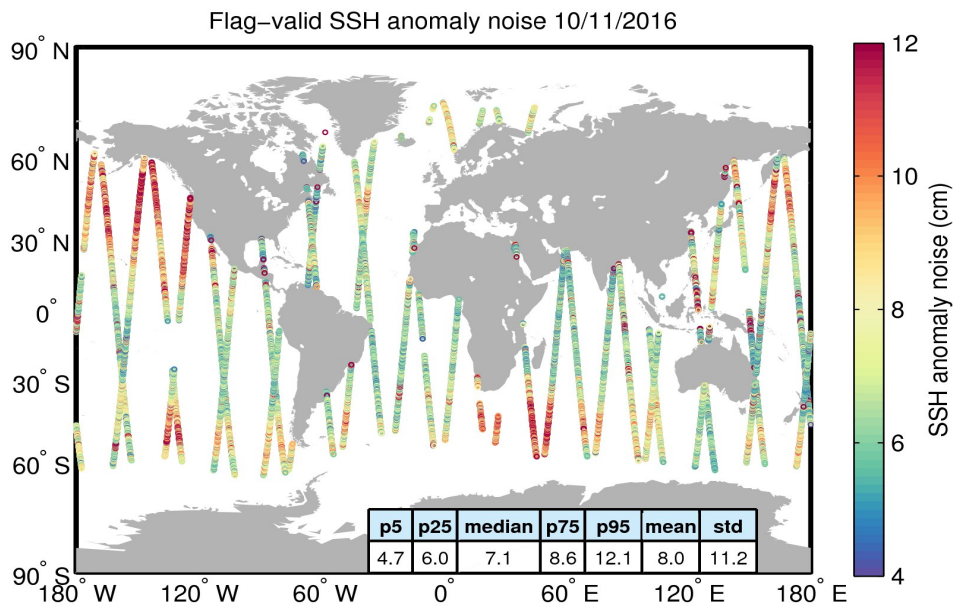
Figure 8. Geographical distribution of flag-valid 20-Hz SSH anomaly measurement noise over oceans and lakes for 10/11/2016. The statistical values shown in the table refer to the SSH anomaly noise and are calculated over all measurements shown in the figure.
