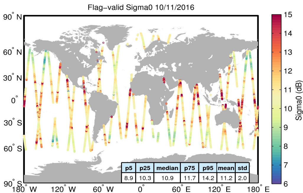
Figure 23. Geographical distribution of flag-valid sigma0 data over oceans and lakes for 10/11/2016. The statistical values shown in the table refer to the sigma0 in dB and are calculated over all measurements shown in the figure.
