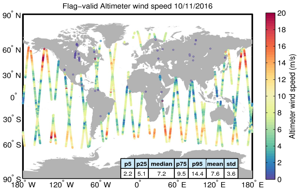
Figure 31. Geographical distribution of flag-valid wind data over oceans and lakes for 10/11/2016. The statistical values shown in the table refer to the wind in m/s and are calculated over all measurements shown in the figure.
