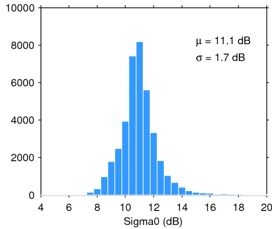
Figure 28. Histogram of science-valid sigma0 over oceans and lakes for 10/11/2016. The mean ( \mu ) and standard deviation ( \sigma ) are also shown. Note that values outside [4 20] dB are excluded from the histogram for the sake of readability but not from the computation of \mu and \sigma .
