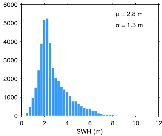
Figure 17. Histogram of flag-valid SWH over oceans and lakes for 10/11/2016. The mean ( \mu ) and standard deviation ( \sigma ) are also shown. Note that values larger than 12 m are excluded from the histogram for the sake of readability but not from the computation of \mu and \sigma .
