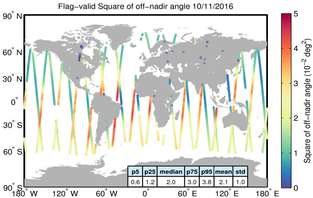
Figure 37. Geographical distribution of flag-valid mispointing data over oceans and lakes for 10/11/2016. The statistical values shown in the table refer to the mispointing in 10^{-2} deg 2 and are calculated over all measurements shown in the figure.
