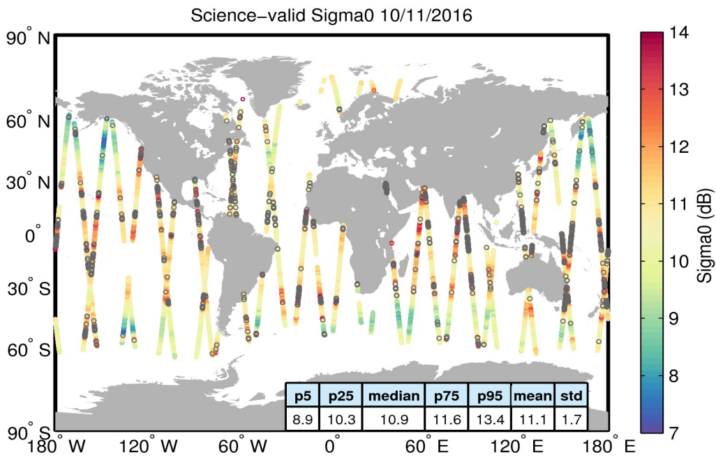
Figure 27. Geographical distribution of science-valid sigma0 data over oceans and lakes for 10/11/2016. The statistical values shown in the table refer to the sigma0 in dB and are calculated over all measurements shown in the figure. Gray circles denote records that have been rejected based on the editing criteria described in Table 4.
