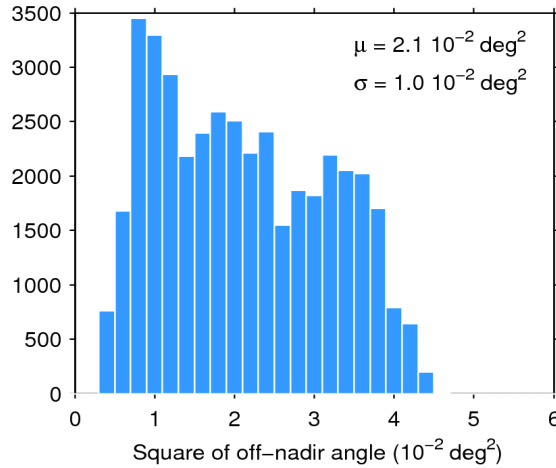
Figure 39. Histogram of flag-valid mispointing over oceans and lakes for 10/11/2016. The mean ( \mu ) and standard deviation ( \sigma ) are also shown. Note that values larger than 6 \cdot 10^{-2} \text{ deg}^2 are excluded from the histogram for the sake of readability but not from the computation of \mu and \sigma .
