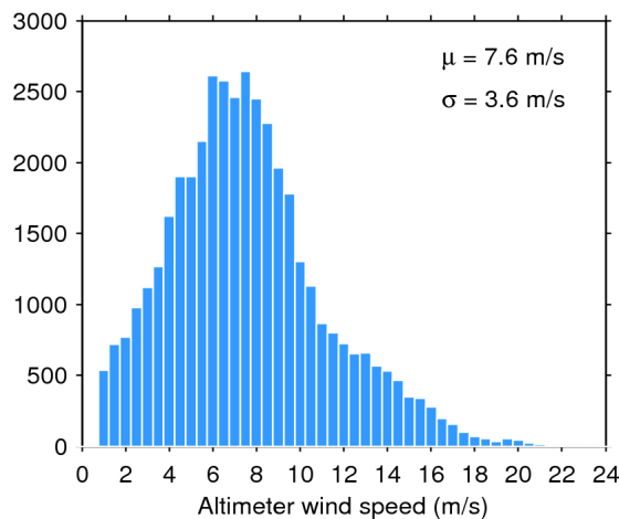
Figure 35. Histogram of science-valid wind over oceans and lakes for 10/11/2016. The mean ( \mu ) and standard deviation ( \sigma ) are also shown. Note that values larger than 24 m/s are excluded from the histogram for the sake of readability but not from the computation of \mu and \sigma .
