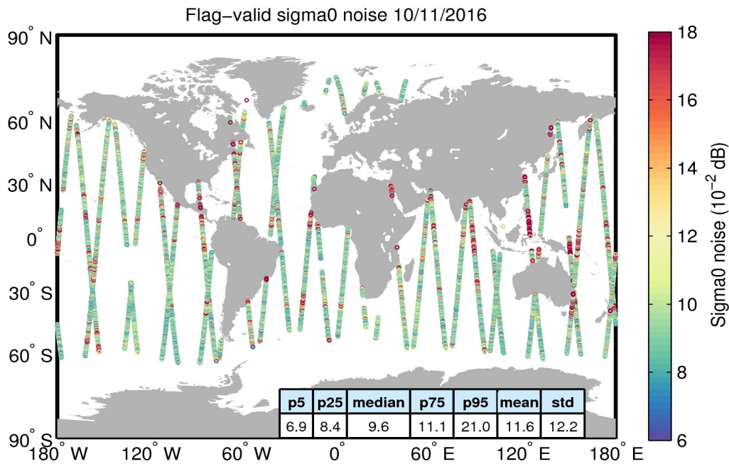
Figure 26. Geographical distribution of flag-valid 20-Hz sigma0 measurement noise over oceans and lakes for 10/11/2016. The statistical values shown in the table refer to the sigma0 noise and are calculated over all measurements shown in the figure.
