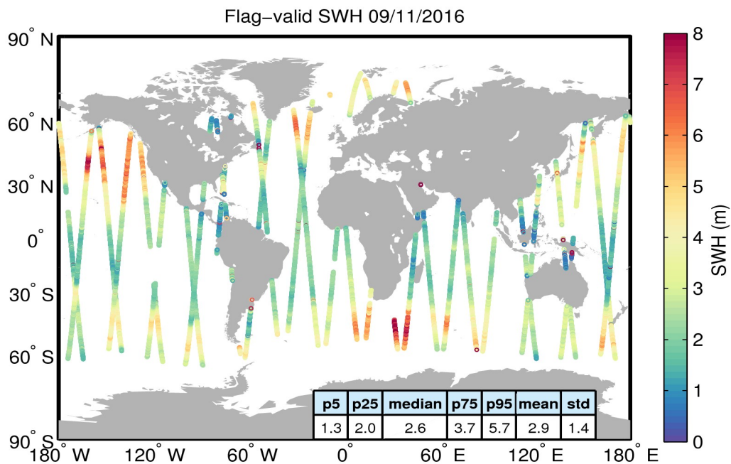
Figure 15. Geographical distribution of flag-valid SWH data over oceans and lakes for 09/11/2016. The statistical values shown in the table refer to the SWH in m and are calculated over all measurements shown in the figure.
