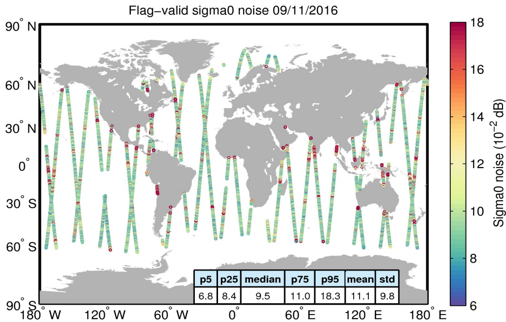
Figure 26. Geographical distribution of flag-valid 20-Hz sigma0 measurement noise over oceans and lakes for 09/11/2016. The statistical values shown in the table refer to the sigma0 noise and are calculated over all measurements shown in the figure.
