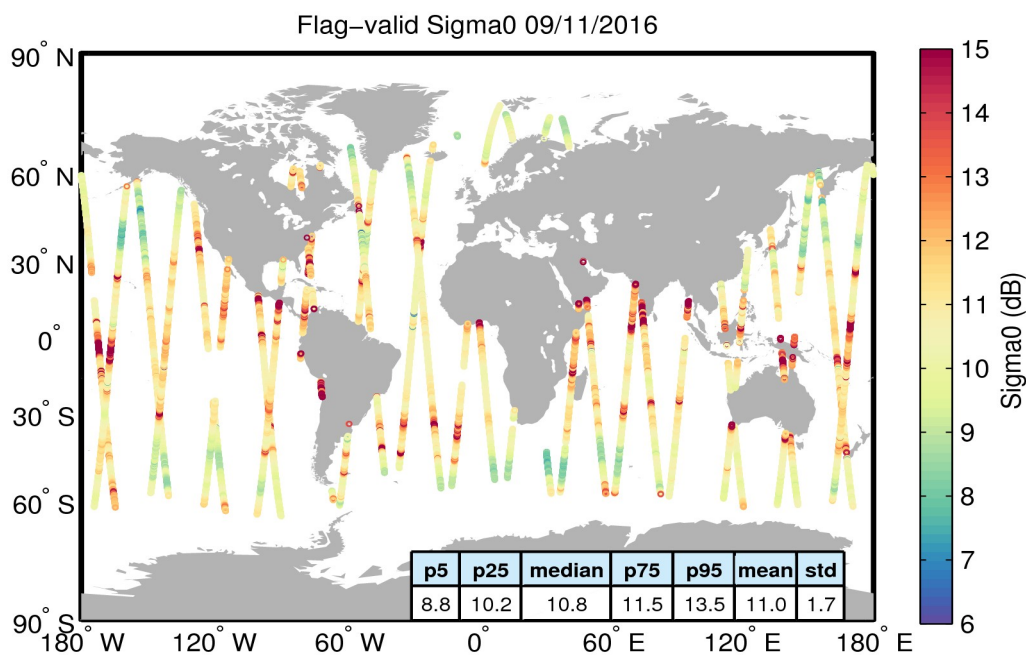
Figure 23. Geographical distribution of flag-valid sigma0 data over oceans and lakes for 09/11/2016. The statistical values shown in the table refer to the sigma0 in dB and are calculated over all measurements shown in the figure.
