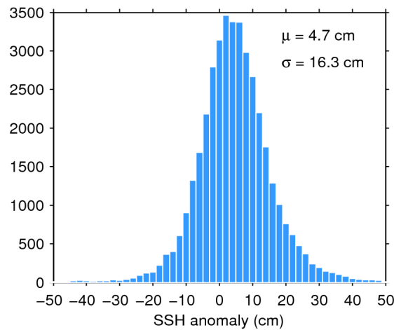
Figure 7. Histogram of flag-valid SSH anomaly over oceans and lakes for 09/11/2016. The mean ( \mu ) and standard deviation ( \sigma ) are also shown. Note that values outside [-50 50] cm are excluded from the histogram for the sake of readability but not from the computation of \mu and \sigma .
