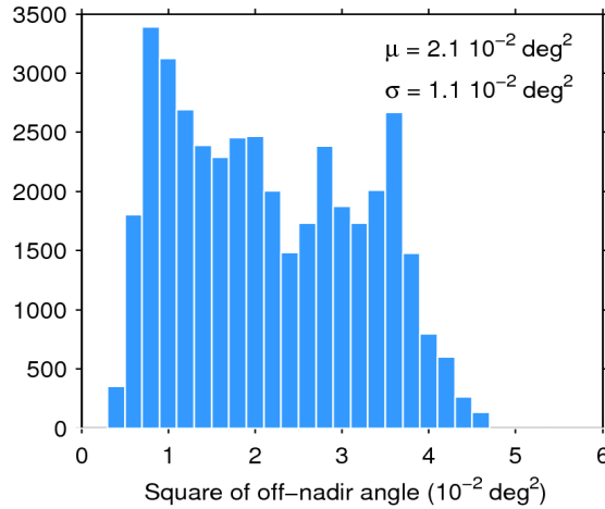
Figure 39. Histogram of flag-valid mispointing over oceans and lakes for 09/11/2016. The mean ( \mu ) and standard deviation ( \sigma ) are also shown. Note that values larger than 6 \cdot 10^{-2} \text{ deg}^2 are excluded from the histogram for the sake of readability but not from the computation of \mu and \sigma .
