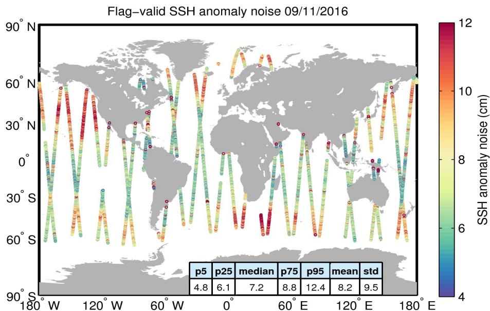
Figure 8. Geographical distribution of flag-valid 20-Hz SSH anomaly measurement noise over oceans and lakes for 09/11/2016. The statistical values shown in the table refer to the SSH anomaly noise and are calculated over all measurements shown in the figure.
