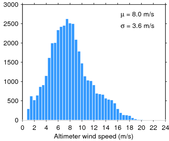
Figure 33. Histogram of flag-valid wind over oceans and lakes for 09/11/2016. The mean ( \mu ) and standard deviation ( \sigma ) are also shown. Note that values larger than 24 m/s are excluded from the histogram for the sake of readability but not from the computation of \mu and \sigma .
