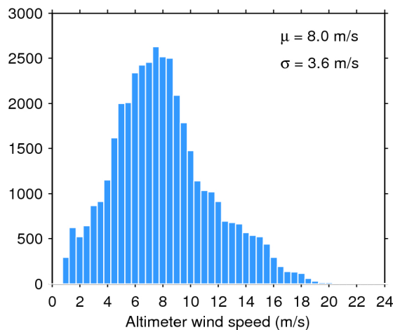
Figure 35. Histogram of science-valid wind over oceans and lakes for 09/11/2016. The mean ( \mu ) and standard deviation ( \sigma ) are also shown. Note that values larger than 24 m/s are excluded from the histogram for the sake of readability but not from the computation of \mu and \sigma .
