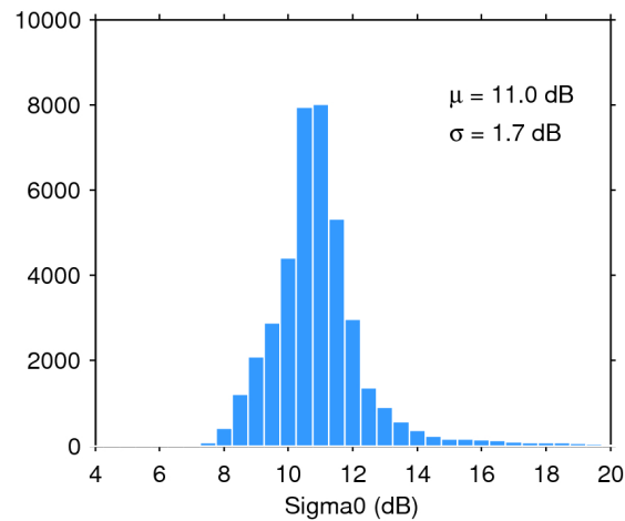
Figure 25. Histogram of flag-valid sigma0 over oceans and lakes for 09/11/2016. The mean ( \mu ) and standard deviation ( \sigma ) are also shown. Note that values outside [4 20] dB are excluded from the histogram for the sake of readability but not from the computation of \mu and \sigma .
