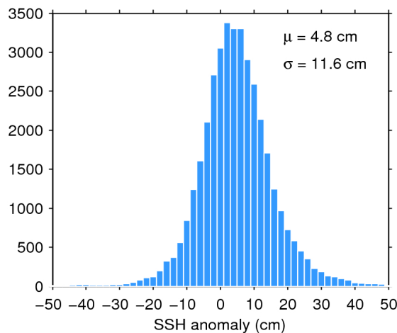
Figure 11. Histogram of science-valid SSH anomaly over oceans and lakes for 09/11/2016. The mean ( \mu ) and standard deviation ( \sigma ) are also shown. Note that values outside [-50 50] cm are excluded from the histogram for the sake of readability but not from the computation of \mu and \sigma .
