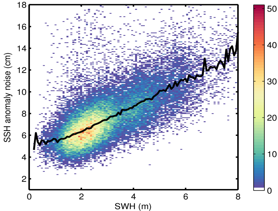
Figure 9. 2D histogram showing flag-valid SSH anomaly noise as a function of SWH for 09/11/2016. The black line denotes the median SSH anomaly noise as a function of SWH.
