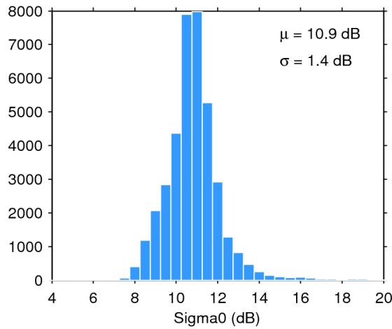
Figure 28. Histogram of science-valid sigma0 over oceans and lakes for 09/11/2016. The mean ( \mu ) and standard deviation ( \sigma ) are also shown. Note that values outside [4 20] dB are excluded from the histogram for the sake of readability but not from the computation of \mu and \sigma .
