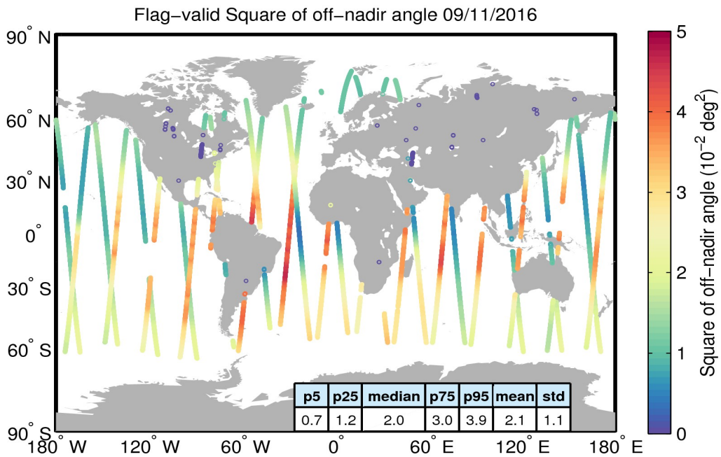
Figure 37. Geographical distribution of flag-valid mispointing data over oceans and lakes for 09/11/2016. The statistical values shown in the table refer to the mispointing in 10^{-2} deg 2 and are calculated over all measurements shown in the figure.
