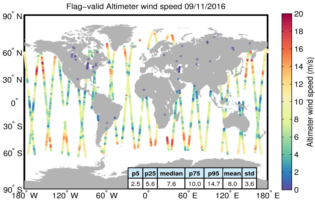
Figure 31. Geographical distribution of flag-valid wind data over oceans and lakes for 09/11/2016. The statistical values shown in the table refer to the wind in m/s and are calculated over all measurements shown in the figure.
