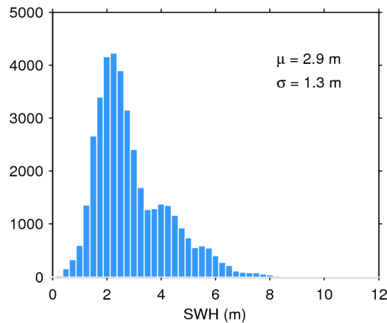
Figure 20. Histogram of science-valid SWH over oceans and lakes for 09/11/2016. The mean ( \mu ) and standard deviation ( \sigma ) are also shown. Note that values larger than 12 m are excluded from the histogram for the sake of readability but not from the computation of \mu and \sigma .
