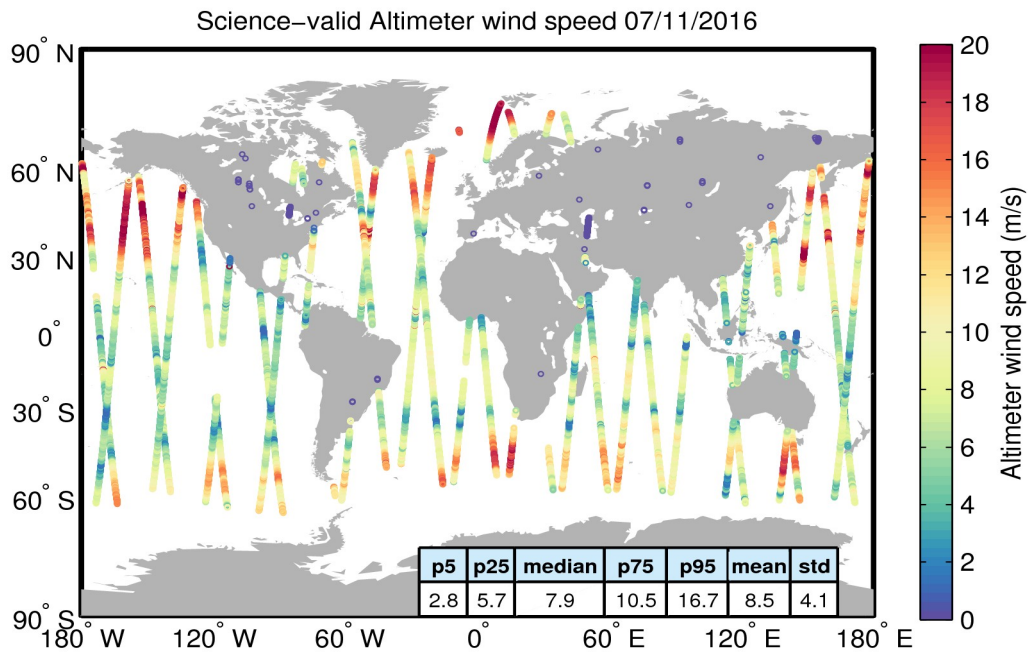
Figure 34. Geographical distribution of science-valid wind data over oceans and lakes for 07/11/2016. The statistical values shown in the table refer to the wind in m/s and are calculated over all measurements shown in the figure. Gray circles denote records that have been rejected based on the editing criteria described in Table 5.
