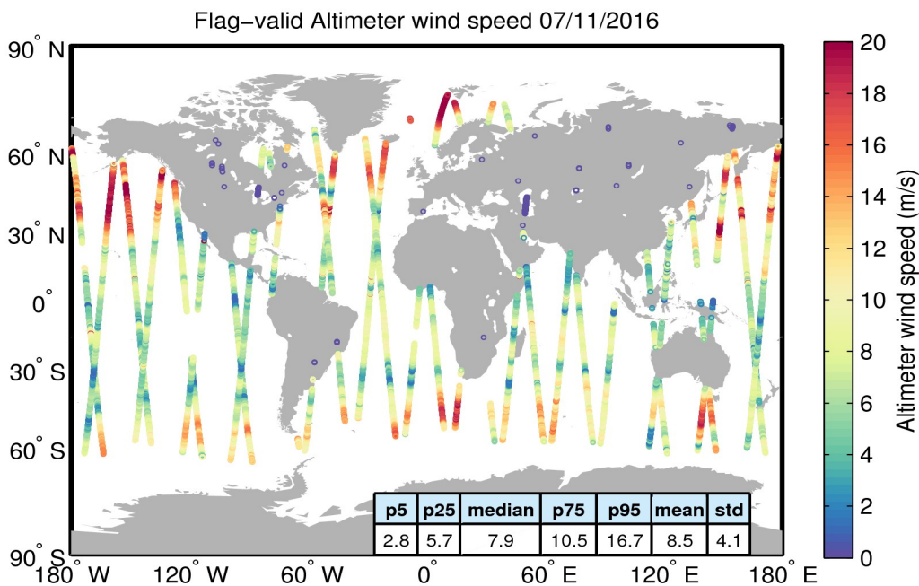
Figure 31. Geographical distribution of flag-valid wind data over oceans and lakes for 07/11/2016. The statistical values shown in the table refer to the wind in m/s and are calculated over all measurements shown in the figure.
