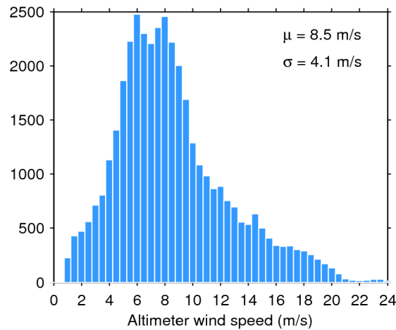
Figure 33. Histogram of flag-valid wind over oceans and lakes for 07/11/2016. The mean ( \mu ) and standard deviation ( \sigma ) are also shown. Note that values larger than 24 m/s are excluded from the histogram for the sake of readability but not from the computation of \mu and \sigma .
