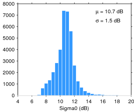
Figure 28. Histogram of science-valid sigma0 over oceans and lakes for 07/11/2016. The mean ( \mu ) and standard deviation ( \sigma ) are also shown. Note that values outside [4 20] dB are excluded from the histogram for the sake of readability but not from the computation of \mu and \sigma .
