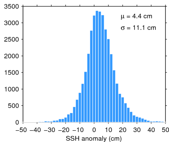
Figure 11. Histogram of science-valid SSH anomaly over oceans and lakes for 07/11/2016. The mean ( \mu ) and standard deviation ( \sigma ) are also shown. Note that values outside [-50 50] cm are excluded from the histogram for the sake of readability but not from the computation of \mu and \sigma .
