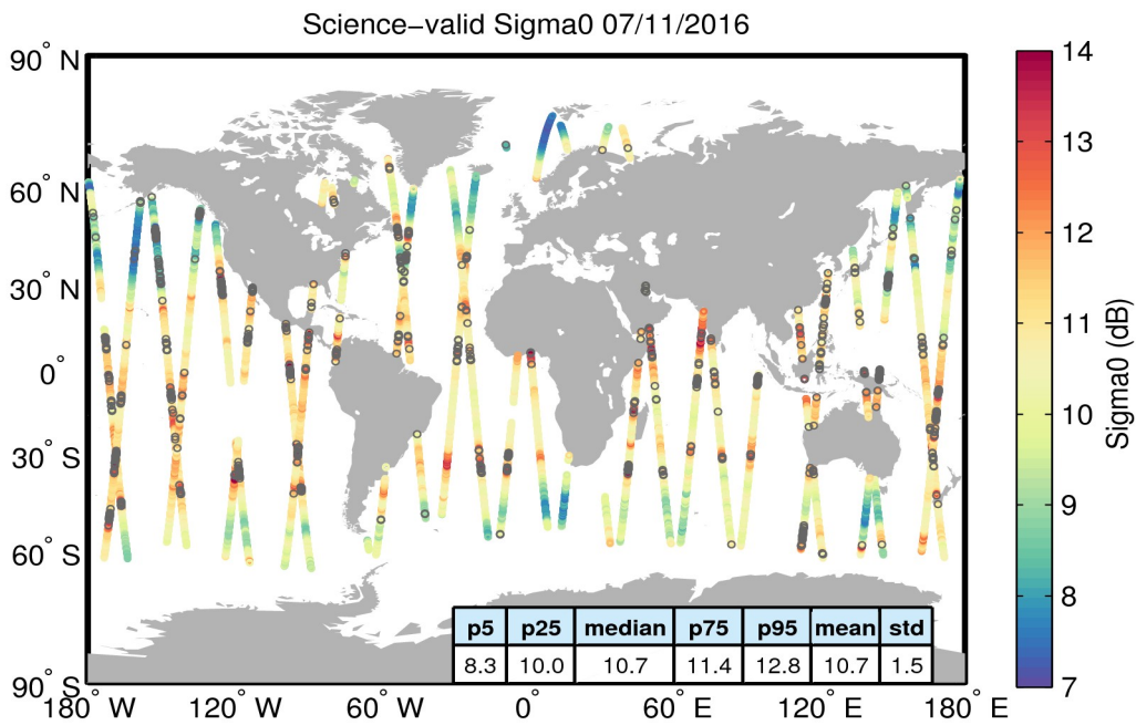
Figure 27. Geographical distribution of science-valid sigma0 data over oceans and lakes for 07/11/2016. The statistical values shown in the table refer to the sigma0 in dB and are calculated over all measurements shown in the figure. Gray circles denote records that have been rejected based on the editing criteria described in Table 4.
