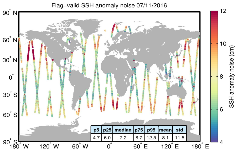
Figure 8. Geographical distribution of flag-valid 20-Hz SSH anomaly measurement noise over oceans and lakes for 07/11/2016. The statistical values shown in the table refer to the SSH anomaly noise and are calculated over all measurements shown in the figure.
