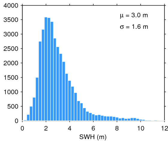
Figure 17. Histogram of flag-valid SWH over oceans and lakes for 07/11/2016. The mean ( \mu ) and standard deviation ( \sigma ) are also shown. Note that values larger than 12 m are excluded from the histogram for the sake of readability but not from the computation of \mu and \sigma .
