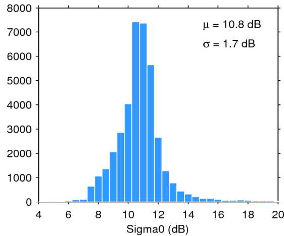
Figure 25. Histogram of flag-valid sigma0 over oceans and lakes for 07/11/2016. The mean ( \mu ) and standard deviation ( \sigma ) are also shown. Note that values outside [4 20] dB are excluded from the histogram for the sake of readability but not from the computation of \mu and \sigma .
