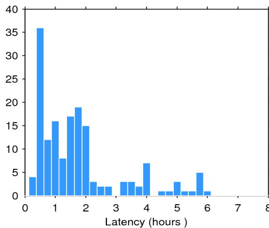
Figure 2. Histogram of the data latency for 07/11/2016. The y-axis denotes the number of files that are made available with a delay of x-hours with respect to the mean time of the records stored in the file.
