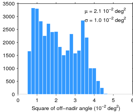
Figure 39. Histogram of flag-valid mispointing over oceans and lakes for 07/11/2016. The mean ( \mu ) and standard deviation ( \sigma ) are also shown. Note that values larger than 6 \cdot 10^{-2} \text{ deg}^2 are excluded from the histogram for the sake of readability but not from the computation of \mu and \sigma .
