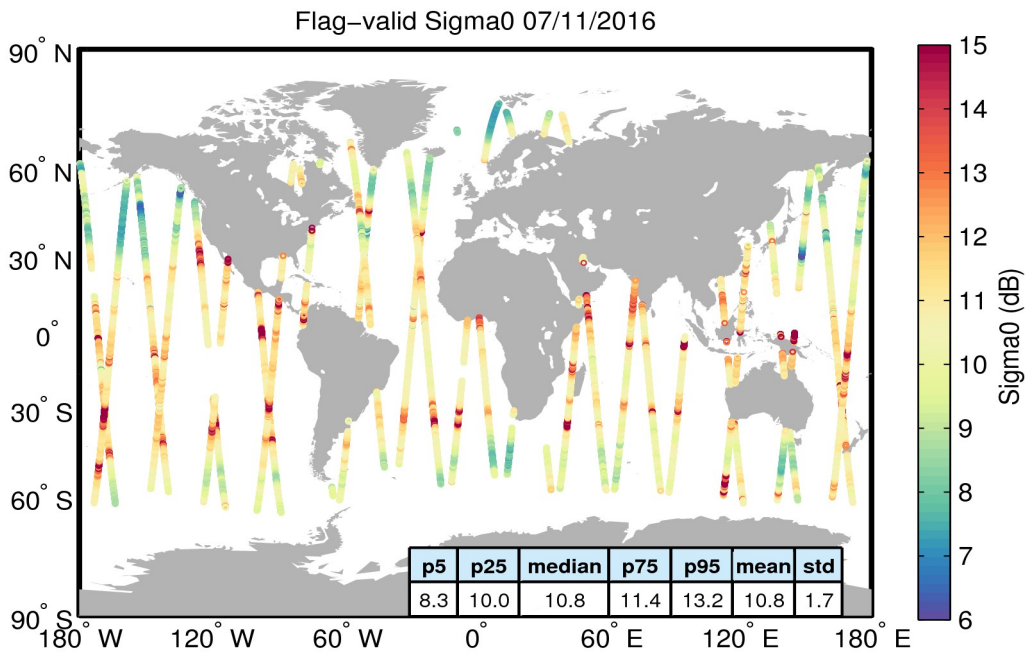
Figure 23. Geographical distribution of flag-valid sigma0 data over oceans and lakes for 07/11/2016. The statistical values shown in the table refer to the sigma0 in dB and are calculated over all measurements shown in the figure.
