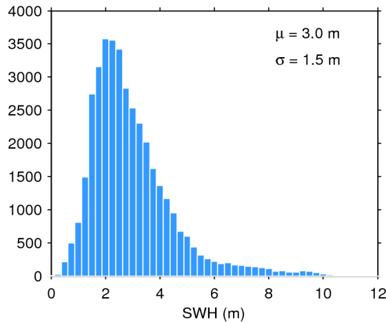
Figure 20. Histogram of science-valid SWH over oceans and lakes for 07/11/2016. The mean ( \mu ) and standard deviation ( \sigma ) are also shown. Note that values larger than 12 m are excluded from the histogram for the sake of readability but not from the computation of \mu and \sigma .
