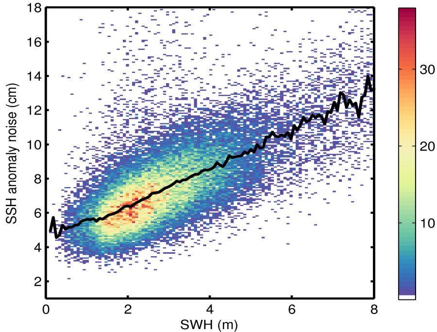
Figure 9. 2D histogram showing flag-valid SSH anomaly noise as a function of SWH for 07/11/2016. The black line denotes the median SSH anomaly noise as a function of SWH.
