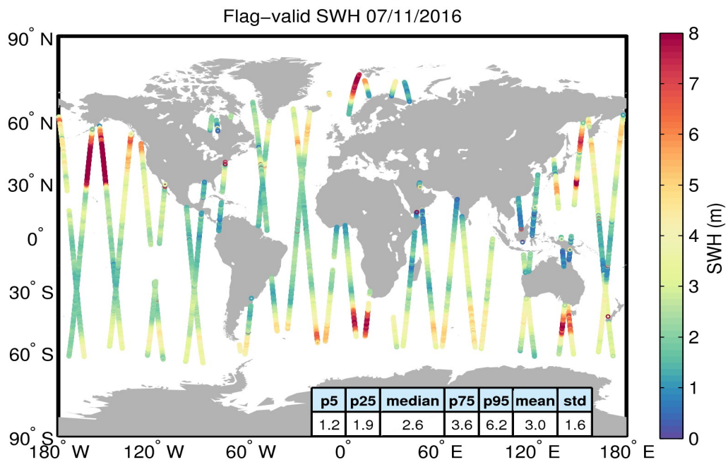
Figure 15. Geographical distribution of flag-valid SWH data over oceans and lakes for 07/11/2016. The statistical values shown in the table refer to the SWH in m and are calculated over all measurements shown in the figure.
