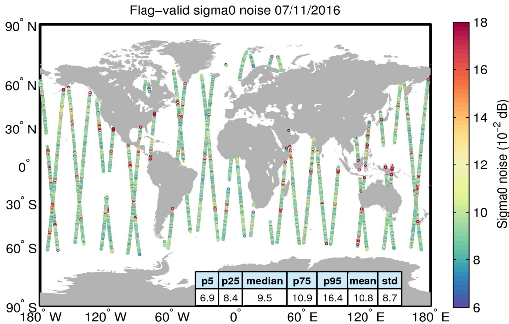
Figure 26. Geographical distribution of flag-valid 20-Hz sigma0 measurement noise over oceans and lakes for 07/11/2016. The statistical values shown in the table refer to the sigma0 noise and are calculated over all measurements shown in the figure.
