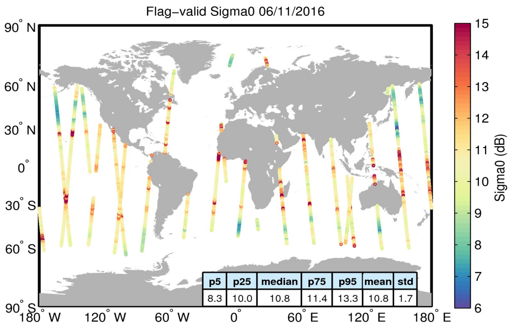
Figure 23. Geographical distribution of flag-valid sigma0 data over oceans and lakes for 06/11/2016. The statistical values shown in the table refer to the sigma0 in dB and are calculated over all measurements shown in the figure.
