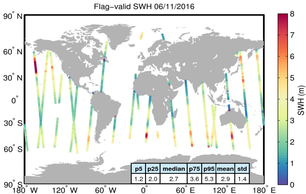
Figure 15. Geographical distribution of flag-valid SWH data over oceans and lakes for 06/11/2016. The statistical values shown in the table refer to the SWH in m and are calculated over all measurements shown in the figure.
