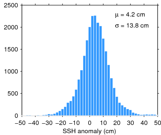
Figure 7. Histogram of flag-valid SSH anomaly over oceans and lakes for 06/11/2016. The mean ( \mu ) and standard deviation ( \sigma ) are also shown. Note that values outside [-50\ 50] cm are excluded from the histogram for the sake of readability but not from the computation of \mu and \sigma .
