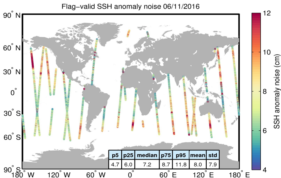
Figure 8. Geographical distribution of flag-valid 20-Hz SSH anomaly measurement noise over oceans and lakes for 06/11/2016. The statistical values shown in the table refer to the SSH anomaly noise and are calculated over all measurements shown in the figure.
