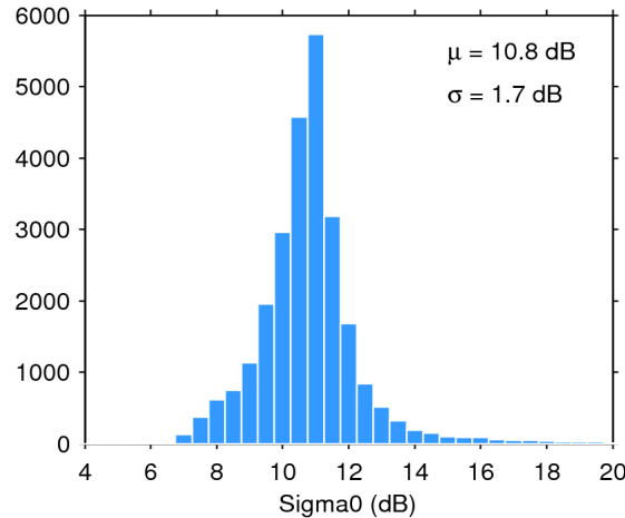
Figure 25. Histogram of flag-valid sigma0 over oceans and lakes for 06/11/2016. The mean ( \mu ) and standard deviation ( \sigma ) are also shown. Note that values outside [4 20] dB are excluded from the histogram for the sake of readability but not from the computation of \mu and \sigma .
