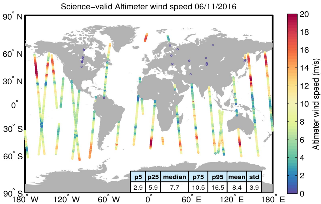
Figure 34. Geographical distribution of science-valid wind data over oceans and lakes for 06/11/2016. The statistical values shown in the table refer to the wind in m/s and are calculated over all measurements shown in the figure. Gray circles denote records that have been rejected based on the editing criteria described in Table 5.
