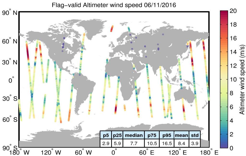
Figure 31. Geographical distribution of flag-valid wind data over oceans and lakes for 06/11/2016. The statistical values shown in the table refer to the wind in m/s and are calculated over all measurements shown in the figure.
