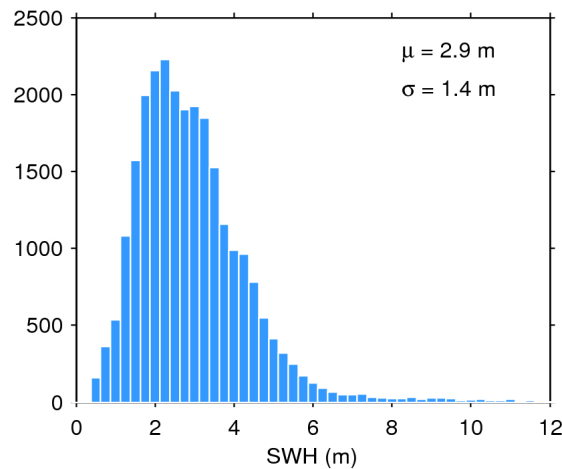
Figure 17. Histogram of flag-valid SWH over oceans and lakes for 06/11/2016. The mean ( \mu ) and standard deviation ( \sigma ) are also shown. Note that values larger than 12 m are excluded from the histogram for the sake of readability but not from the computation of \mu and \sigma .
