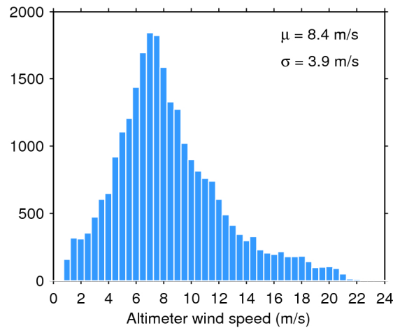
Figure 33. Histogram of flag-valid wind over oceans and lakes for 06/11/2016. The mean ( \mu ) and standard deviation ( \sigma ) are also shown. Note that values larger than 24 m/s are excluded from the histogram for the sake of readability but not from the computation of \mu and \sigma .
