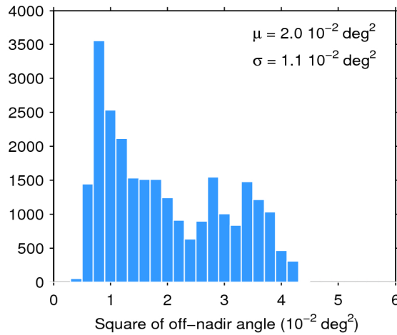
Figure 39. Histogram of flag-valid mispointing over oceans and lakes for 06/11/2016. The mean ( \mu ) and standard deviation ( \sigma ) are also shown. Note that values larger than 6 \cdot 10^{-2} \text{ deg}^2 are excluded from the histogram for the sake of readability but not from the computation of \mu and \sigma .
