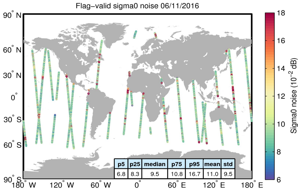
Figure 26. Geographical distribution of flag-valid 20-Hz sigma0 measurement noise over oceans and lakes for 06/11/2016. The statistical values shown in the table refer to the sigma0 noise and are calculated over all measurements shown in the figure.
