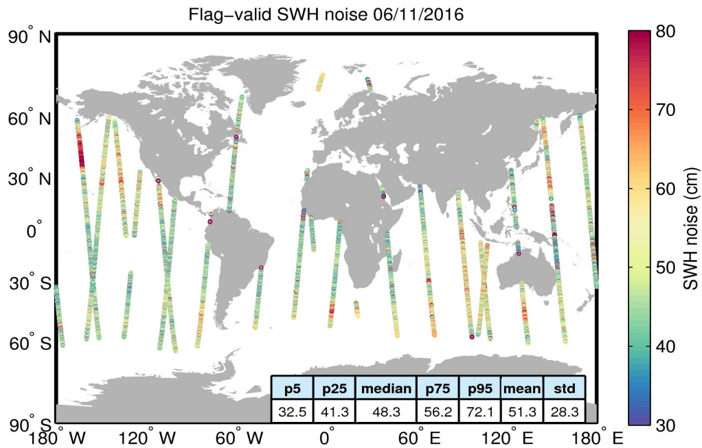
Figure 18. Geographical distribution of flag-valid 20-Hz SWH measurement noise over oceans and lakes for 06/11/2016. The statistical values shown in the table refer to the SWH noise and are calculated over all measurements shown in the figure.
