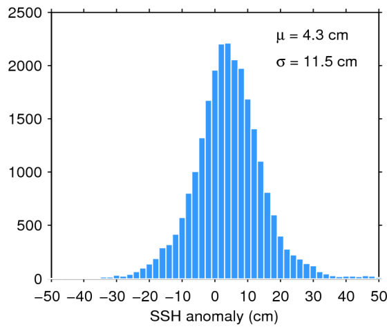
Figure 11. Histogram of science-valid SSH anomaly over oceans and lakes for 06/11/2016. The mean ( \mu ) and standard deviation ( \sigma ) are also shown. Note that values outside [-50 50] cm are excluded from the histogram for the sake of readability but not from the computation of \mu and \sigma .
