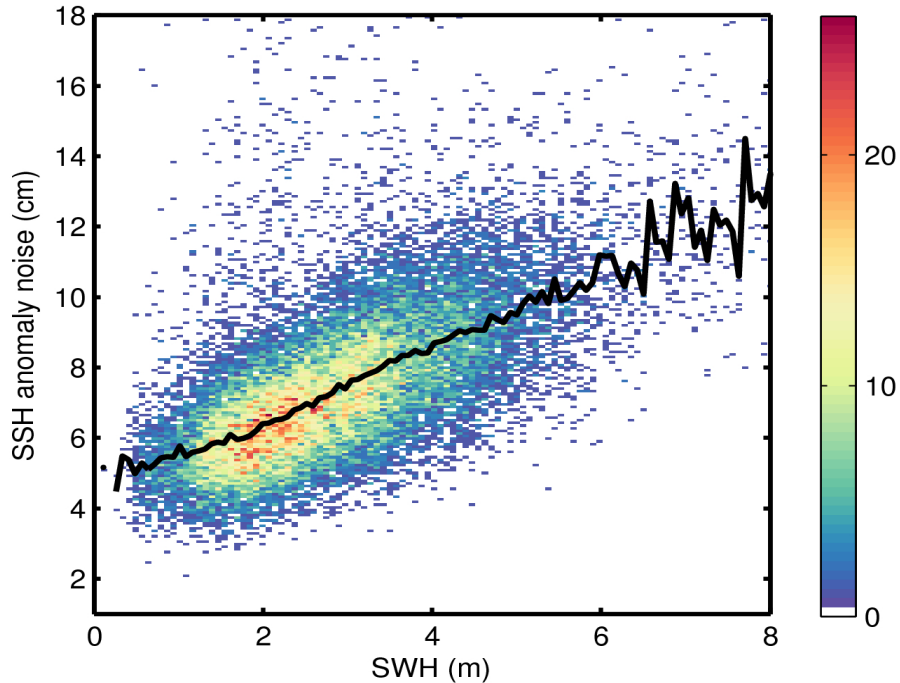
Figure 9. 2D histogram showing flag-valid SSH anomaly noise as a function of SWH for 06/11/2016. The black line denotes the median SSH anomaly noise as a function of SWH.
