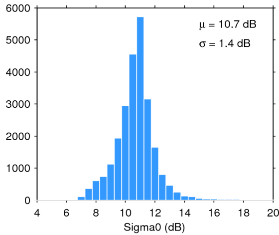
Figure 28. Histogram of science-valid sigma0 over oceans and lakes for 06/11/2016. The mean ( \mu ) and standard deviation ( \sigma ) are also shown. Note that values outside [4 20] dB are excluded from the histogram for the sake of readability but not from the computation of \mu and \sigma .
