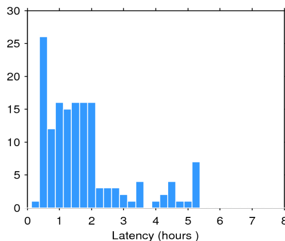
Figure 2. Histogram of the data latency for 06/11/2016. The y-axis denotes the number of files that are made available with a delay of x-hours with respect to the mean time of the records stored in the file.
