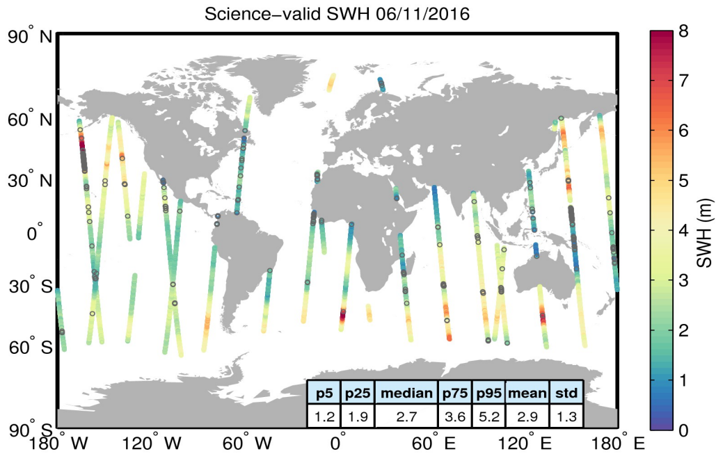
Figure 19. Geographical distribution of science-valid SWH data over oceans and lakes for 06/11/2016. The statistical values shown in the table refer to the SWH in m and are calculated over all measurements shown in the figure. Gray circles denote records that have been rejected based on the editing criteria described in Table 3.
