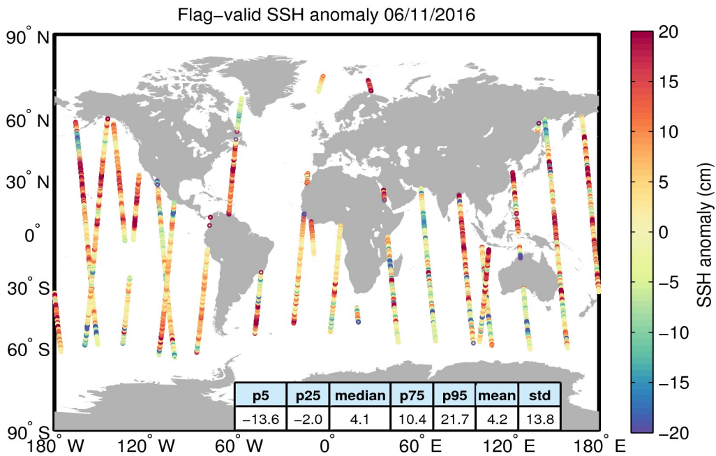
Figure 5. Geographical distribution of flag-valid 1-Hz SSH anomaly data over oceans and lakes for 06/11/2016. The statistical values shown in the table refer to the SSH anomaly in cm and are calculated over all measurements shown in the figure.
