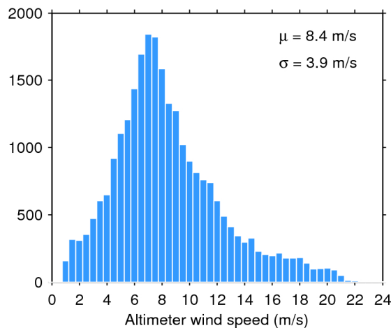
Figure 35. Histogram of science-valid wind over oceans and lakes for 06/11/2016. The mean ( \mu ) and standard deviation ( \sigma ) are also shown. Note that values larger than 24 m/s are excluded from the histogram for the sake of readability but not from the computation of \mu and \sigma .
