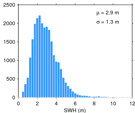
Figure 20. Histogram of science-valid SWH over oceans and lakes for 06/11/2016. The mean ( \mu ) and standard deviation ( \sigma ) are also shown. Note that values larger than 12 m are excluded from the histogram for the sake of readability but not from the computation of \mu and \sigma .
