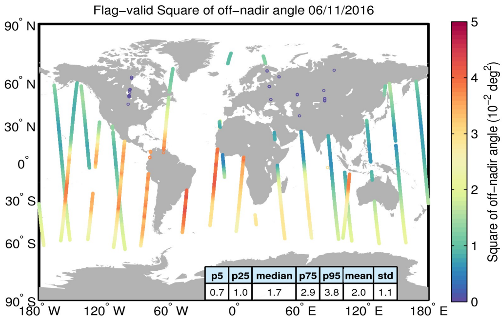
Figure 37. Geographical distribution of flag-valid mispointing data over oceans and lakes for 06/11/2016. The statistical values shown in the table refer to the mispointing in 10^{-2} deg 2 and are calculated over all measurements shown in the figure.
