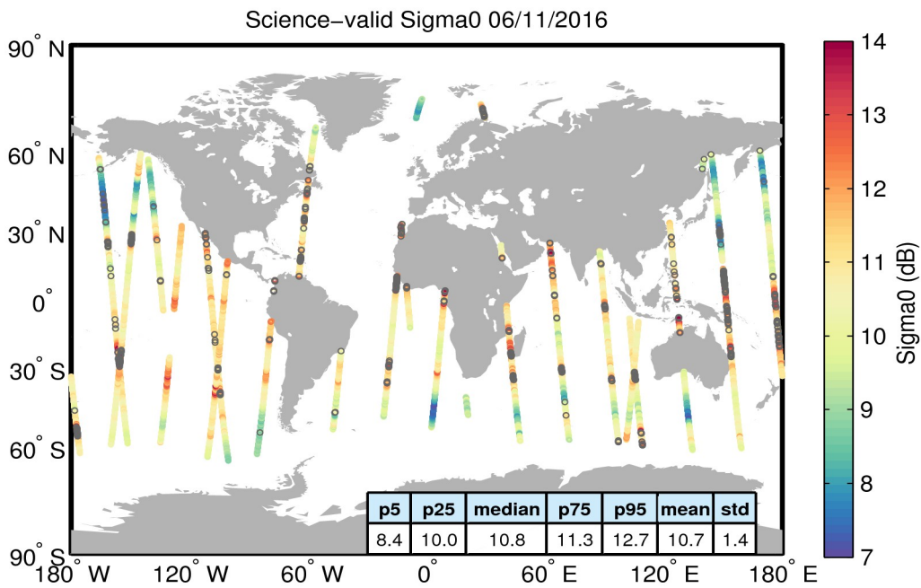
Figure 27. Geographical distribution of science-valid sigma0 data over oceans and lakes for 06/11/2016. The statistical values shown in the table refer to the sigma0 in dB and are calculated over all measurements shown in the figure. Gray circles denote records that have been rejected based on the editing criteria described in Table 4.
