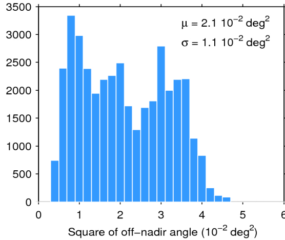
Figure 39. Histogram of flag-valid mispointing over oceans and lakes for 05/11/2016. The mean ( \mu ) and standard deviation ( \sigma ) are also shown. Note that values larger than 6 \cdot 10^{-2} \text{ deg}^2 are excluded from the histogram for the sake of readability but not from the computation of \mu and \sigma .
