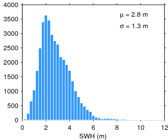
Figure 20. Histogram of science-valid SWH over oceans and lakes for 05/11/2016. The mean ( \mu ) and standard deviation ( \sigma ) are also shown. Note that values larger than 12 m are excluded from the histogram for the sake of readability but not from the computation of \mu and \sigma .
