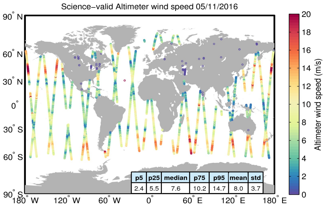
Figure 34. Geographical distribution of science-valid wind data over oceans and lakes for 05/11/2016. The statistical values shown in the table refer to the wind in m/s and are calculated over all measurements shown in the figure. Gray circles denote records that have been rejected based on the editing criteria described in Table 5.
