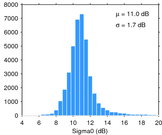
Figure 25. Histogram of flag-valid sigma0 over oceans and lakes for 05/11/2016. The mean ( \mu ) and standard deviation ( \sigma ) are also shown. Note that values outside [4 20] dB are excluded from the histogram for the sake of readability but not from the computation of \mu and \sigma .
