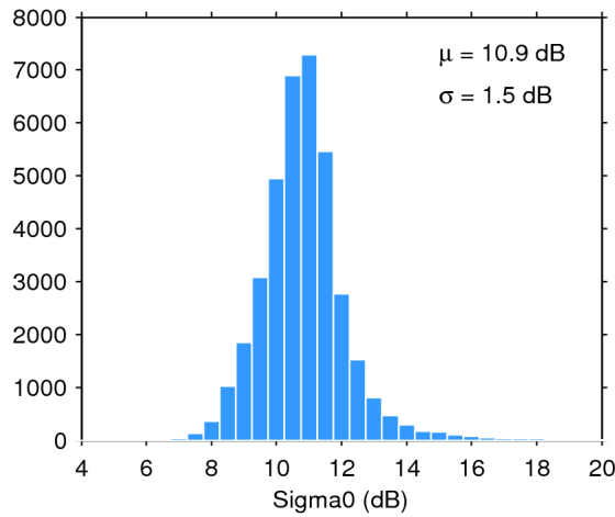
Figure 28. Histogram of science-valid sigma0 over oceans and lakes for 05/11/2016. The mean ( \mu ) and standard deviation ( \sigma ) are also shown. Note that values outside [4 20] dB are excluded from the histogram for the sake of readability but not from the computation of \mu and \sigma .
