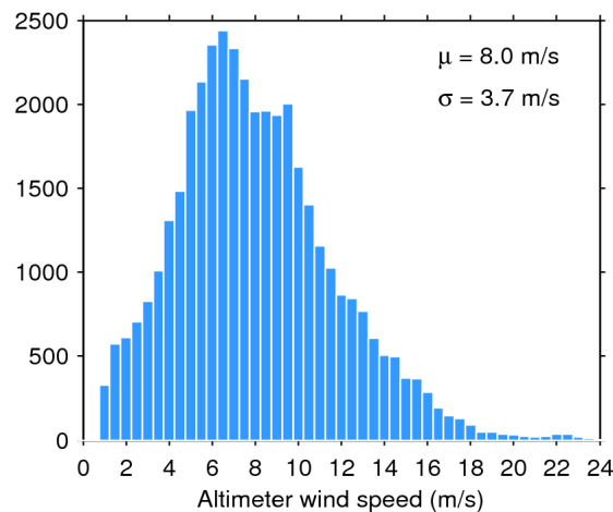
Figure 35. Histogram of science-valid wind over oceans and lakes for 05/11/2016. The mean ( \mu ) and standard deviation ( \sigma ) are also shown. Note that values larger than 24 m/s are excluded from the histogram for the sake of readability but not from the computation of \mu and \sigma .
