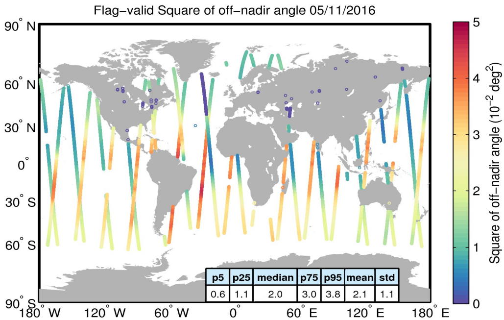
Figure 37. Geographical distribution of flag-valid mispointing data over oceans and lakes for 05/11/2016. The statistical values shown in the table refer to the mispointing in 10^{-2} deg 2 and are calculated over all measurements shown in the figure.
