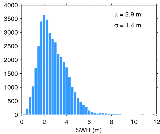
Figure 17. Histogram of flag-valid SWH over oceans and lakes for 05/11/2016. The mean ( \mu ) and standard deviation ( \sigma ) are also shown. Note that values larger than 12 m are excluded from the histogram for the sake of readability but not from the computation of \mu and \sigma .
