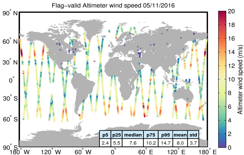
Figure 31. Geographical distribution of flag-valid wind data over oceans and lakes for 05/11/2016. The statistical values shown in the table refer to the wind in m/s and are calculated over all measurements shown in the figure.
