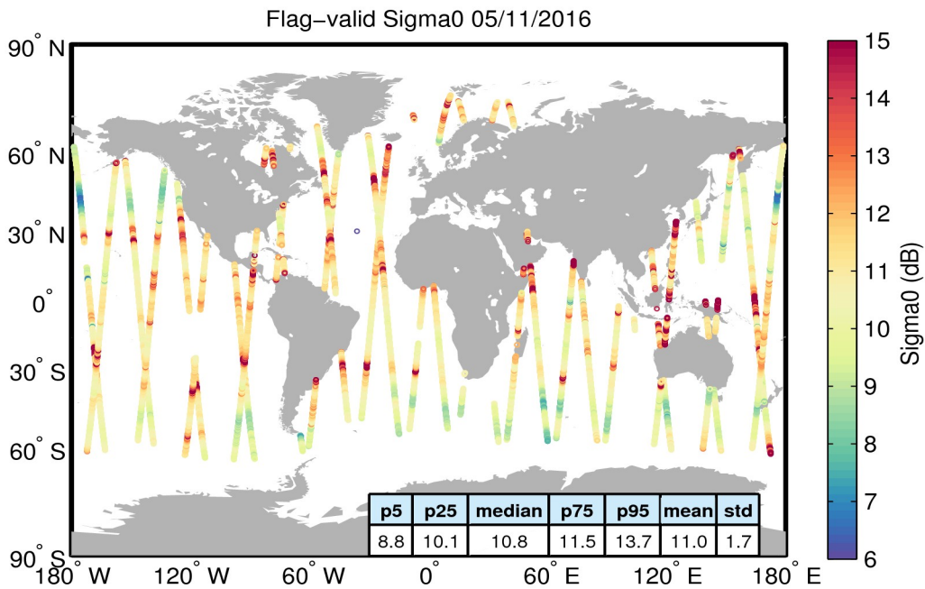
Figure 23. Geographical distribution of flag-valid sigma0 data over oceans and lakes for 05/11/2016. The statistical values shown in the table refer to the sigma0 in dB and are calculated over all measurements shown in the figure.
