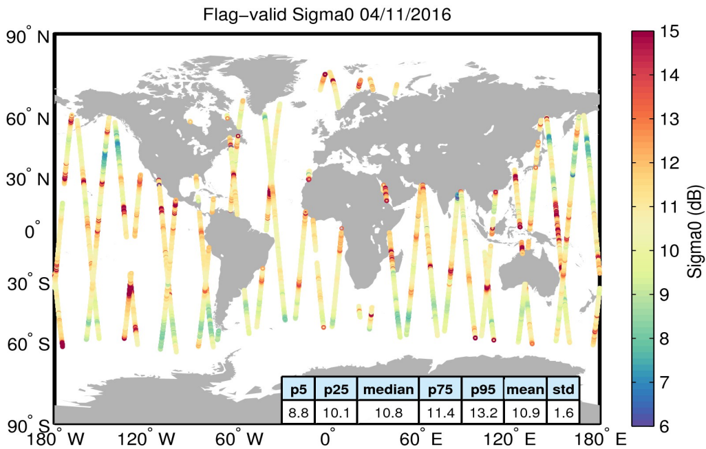
Figure 23. Geographical distribution of flag-valid sigma0 data over oceans and lakes for 04/11/2016. The statistical values shown in the table refer to the sigma0 in dB and are calculated over all measurements shown in the figure.
