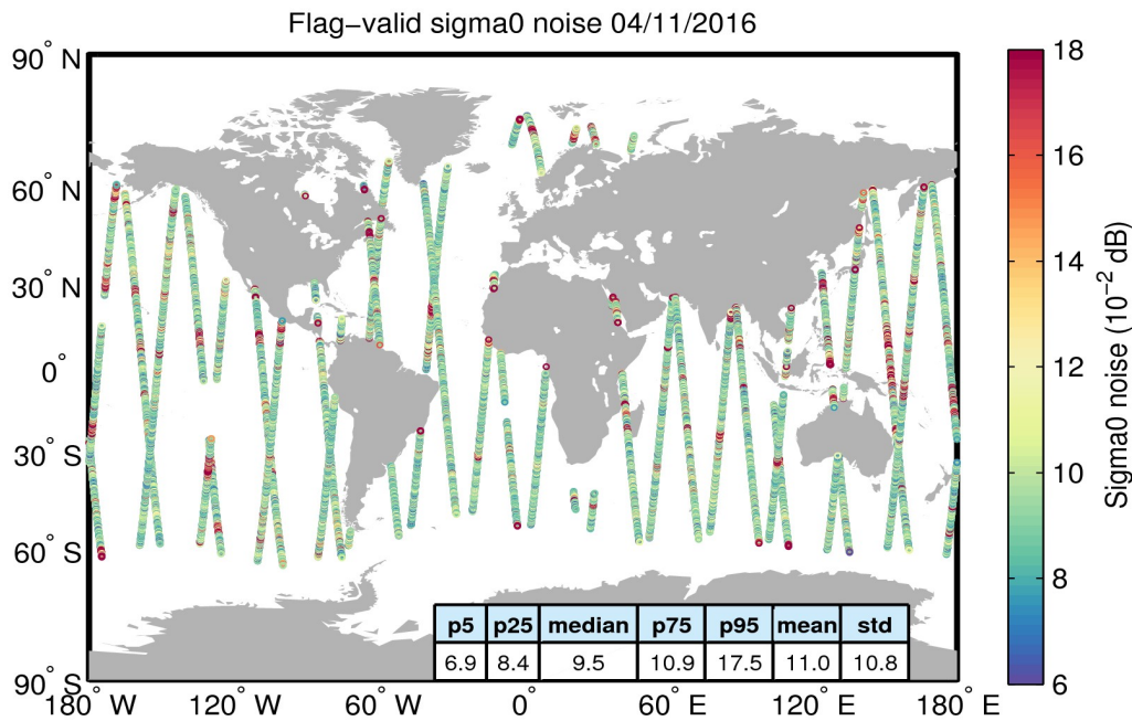
Figure 26. Geographical distribution of flag-valid 20-Hz sigma0 measurement noise over oceans and lakes for 04/11/2016. The statistical values shown in the table refer to the sigma0 noise and are calculated over all measurements shown in the figure.
