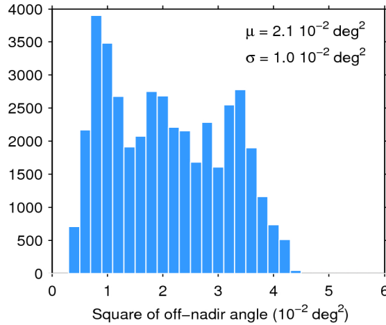
Figure 39. Histogram of flag-valid mispointing over oceans and lakes for 04/11/2016. The mean ( \mu ) and standard deviation ( \sigma ) are also shown. Note that values larger than 6 \cdot 10^{-2} \text{ deg}^2 are excluded from the histogram for the sake of readability but not from the computation of \mu and \sigma .
