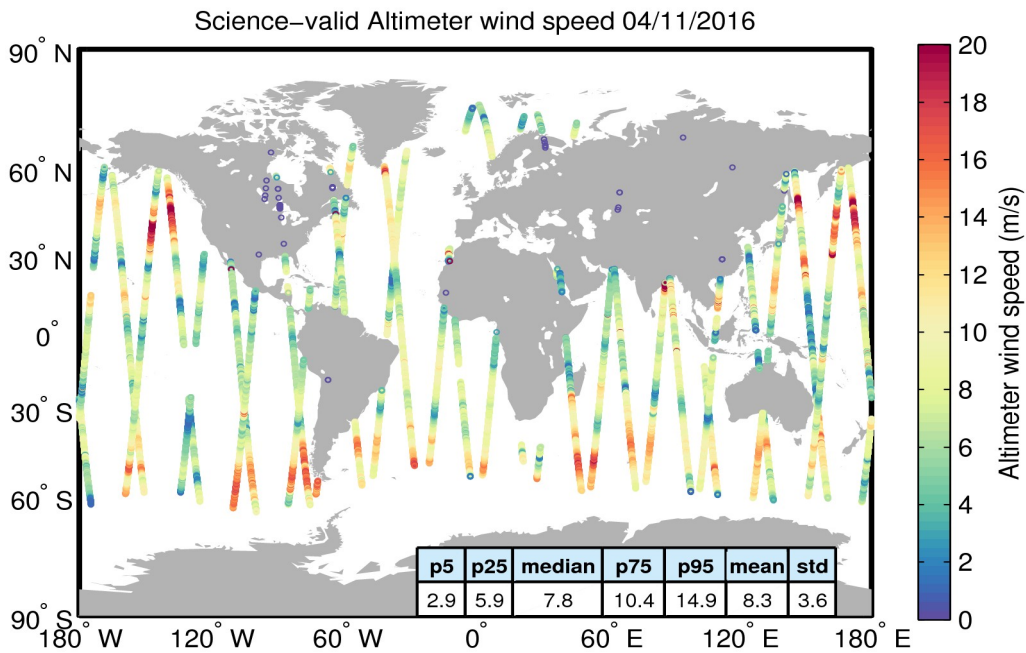
Figure 34. Geographical distribution of science-valid wind data over oceans and lakes for 04/11/2016. The statistical values shown in the table refer to the wind in m/s and are calculated over all measurements shown in the figure. Gray circles denote records that have been rejected based on the editing criteria described in Table 5.
