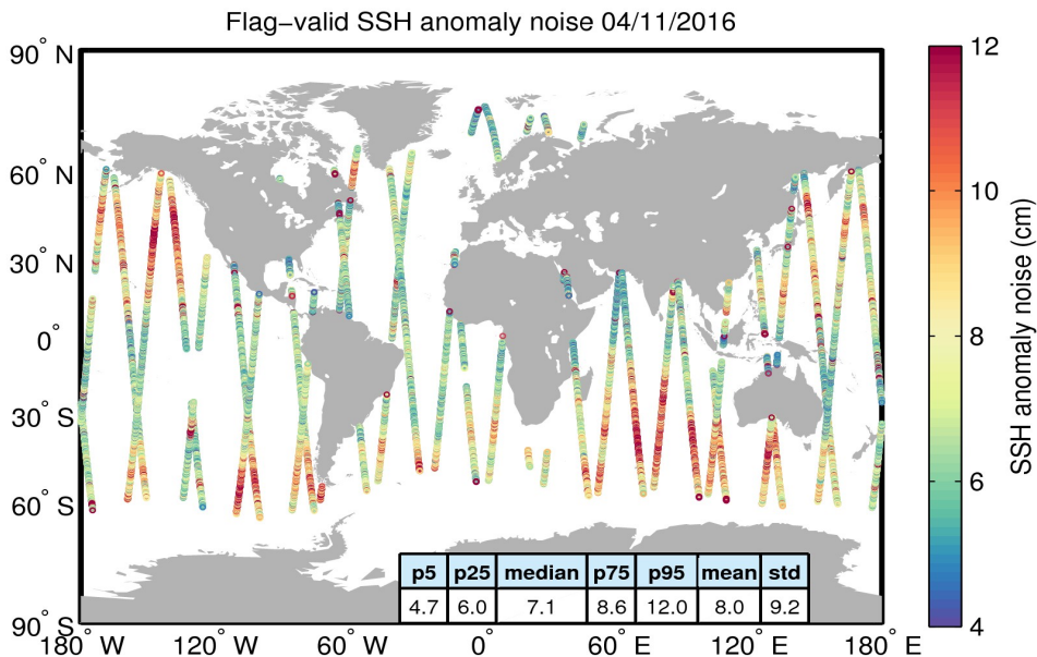
Figure 8. Geographical distribution of flag-valid 20-Hz SSH anomaly measurement noise over oceans and lakes for 04/11/2016. The statistical values shown in the table refer to the SSH anomaly noise and are calculated over all measurements shown in the figure.
