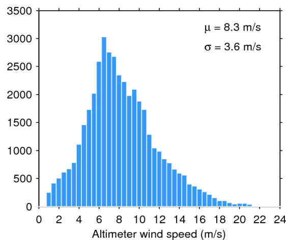
Figure 35. Histogram of science-valid wind over oceans and lakes for 04/11/2016. The mean ( \mu ) and standard deviation ( \sigma ) are also shown. Note that values larger than 24 m/s are excluded from the histogram for the sake of readability but not from the computation of \mu and \sigma .
