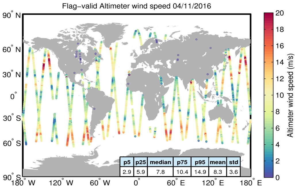
Figure 31. Geographical distribution of flag-valid wind data over oceans and lakes for 04/11/2016. The statistical values shown in the table refer to the wind in m/s and are calculated over all measurements shown in the figure.
