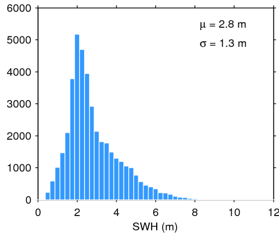
Figure 20. Histogram of science-valid SWH over oceans and lakes for 04/11/2016. The mean ( \mu ) and standard deviation ( \sigma ) are also shown. Note that values larger than 12 m are excluded from the histogram for the sake of readability but not from the computation of \mu and \sigma .
