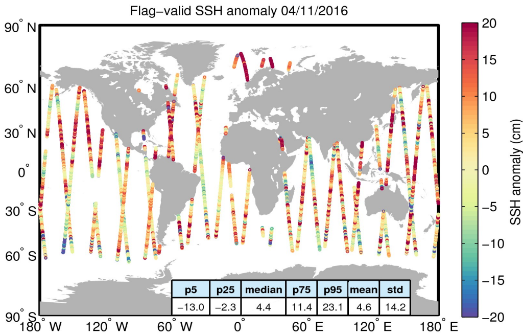
Figure 5. Geographical distribution of flag-valid 1-Hz SSH anomaly data over oceans and lakes for 04/11/2016. The statistical values shown in the table refer to the SSH anomaly in cm and are calculated over all measurements shown in the figure.
