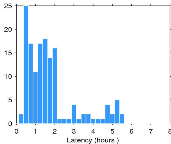
Figure 2. Histogram of the data latency for 04/11/2016. The y-axis denotes the number of files that are made available with a delay of x-hours with respect to the mean time of the records stored in the file.
