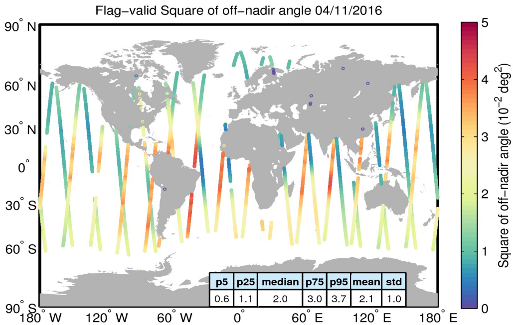
Figure 37. Geographical distribution of flag-valid mispointing data over oceans and lakes for 04/11/2016. The statistical values shown in the table refer to the mispointing in 10^{-2} deg 2 and are calculated over all measurements shown in the figure.
