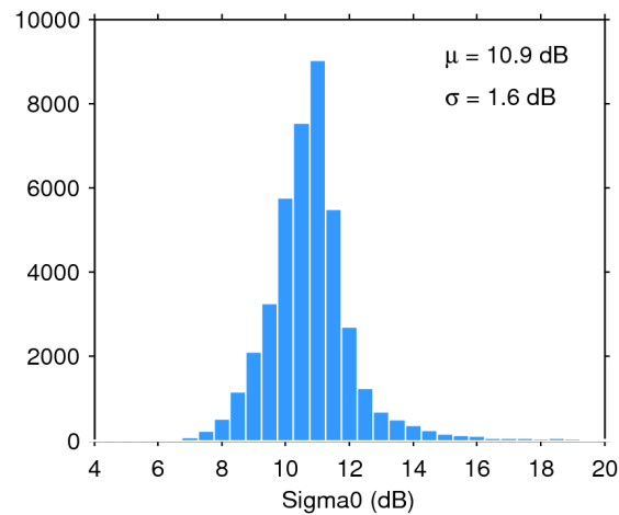
Figure 25. Histogram of flag-valid sigma0 over oceans and lakes for 04/11/2016. The mean ( \mu ) and standard deviation ( \sigma ) are also shown. Note that values outside [4 20] dB are excluded from the histogram for the sake of readability but not from the computation of \mu and \sigma .
