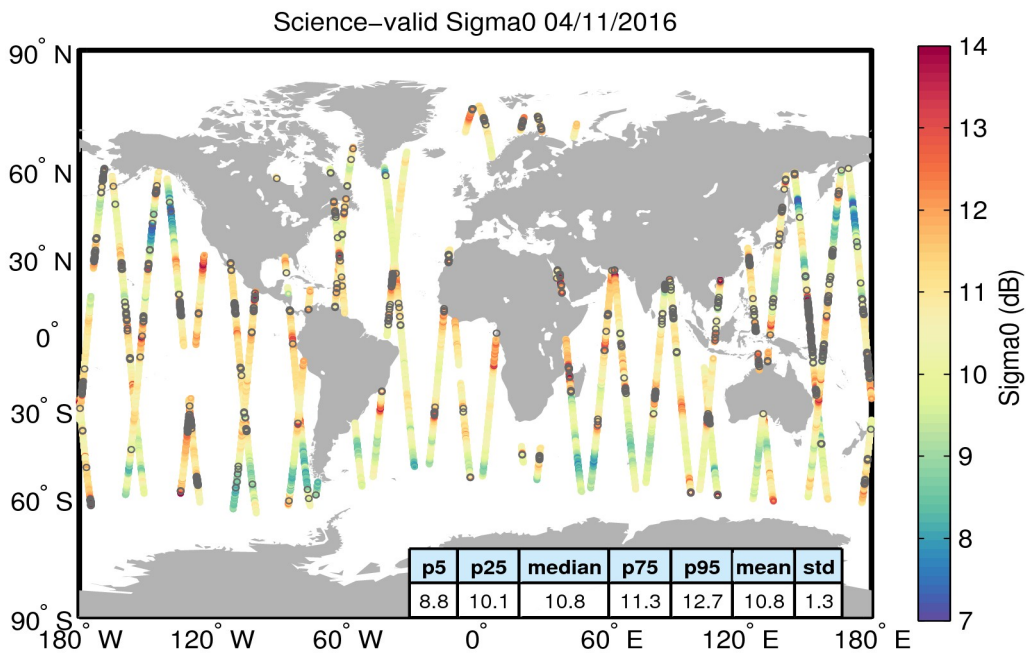
Figure 27. Geographical distribution of science-valid sigma0 data over oceans and lakes for 04/11/2016. The statistical values shown in the table refer to the sigma0 in dB and are calculated over all measurements shown in the figure. Gray circles denote records that have been rejected based on the editing criteria described in Table 4.
