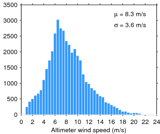
Figure 33. Histogram of flag-valid wind over oceans and lakes for 04/11/2016. The mean ( \mu ) and standard deviation ( \sigma ) are also shown. Note that values larger than 24 m/s are excluded from the histogram for the sake of readability but not from the computation of \mu and \sigma .
