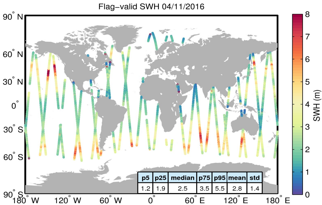
Figure 15. Geographical distribution of flag-valid SWH data over oceans and lakes for 04/11/2016. The statistical values shown in the table refer to the SWH in m and are calculated over all measurements shown in the figure.
