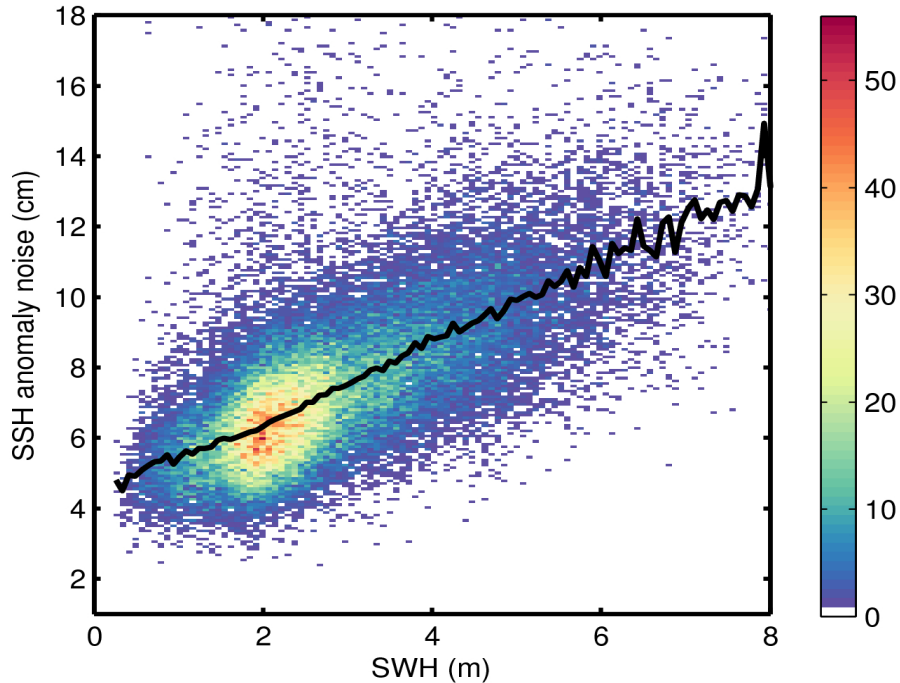
Figure 9. 2D histogram showing flag-valid SSH anomaly noise as a function of SWH for 04/11/2016. The black line denotes the median SSH anomaly noise as a function of SWH.
