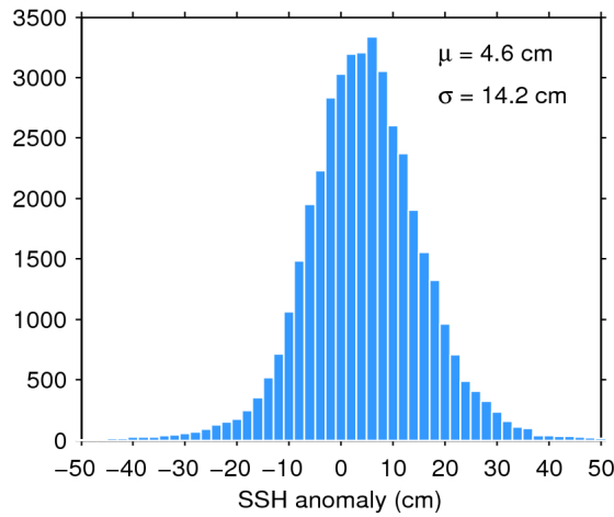
Figure 7. Histogram of flag-valid SSH anomaly over oceans and lakes for 04/11/2016. The mean ( \mu ) and standard deviation ( \sigma ) are also shown. Note that values outside [-50\ 50] cm are excluded from the histogram for the sake of readability but not from the computation of \mu and \sigma .
