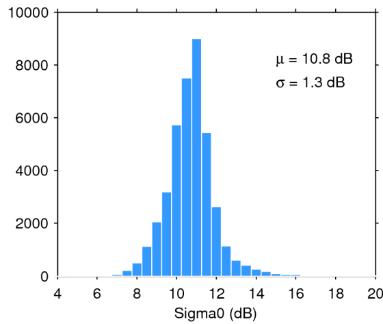
Figure 28. Histogram of science-valid sigma0 over oceans and lakes for 04/11/2016. The mean ( \mu ) and standard deviation ( \sigma ) are also shown. Note that values outside [4 20] dB are excluded from the histogram for the sake of readability but not from the computation of \mu and \sigma .
