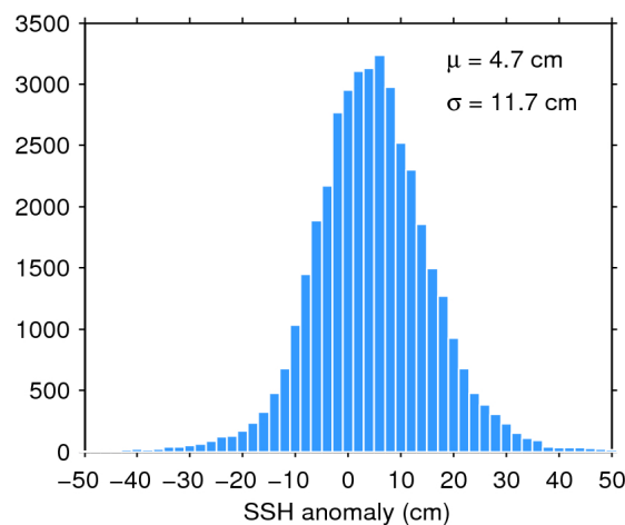
Figure 11. Histogram of science-valid SSH anomaly over oceans and lakes for 04/11/2016. The mean ( \mu ) and standard deviation ( \sigma ) are also shown. Note that values outside [-50 50] cm are excluded from the histogram for the sake of readability but not from the computation of \mu and \sigma .
