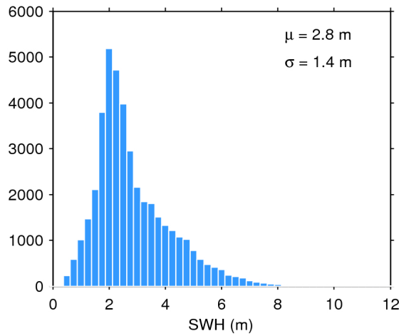
Figure 17. Histogram of flag-valid SWH over oceans and lakes for 04/11/2016. The mean ( \mu ) and standard deviation ( \sigma ) are also shown. Note that values larger than 12 m are excluded from the histogram for the sake of readability but not from the computation of \mu and \sigma .
