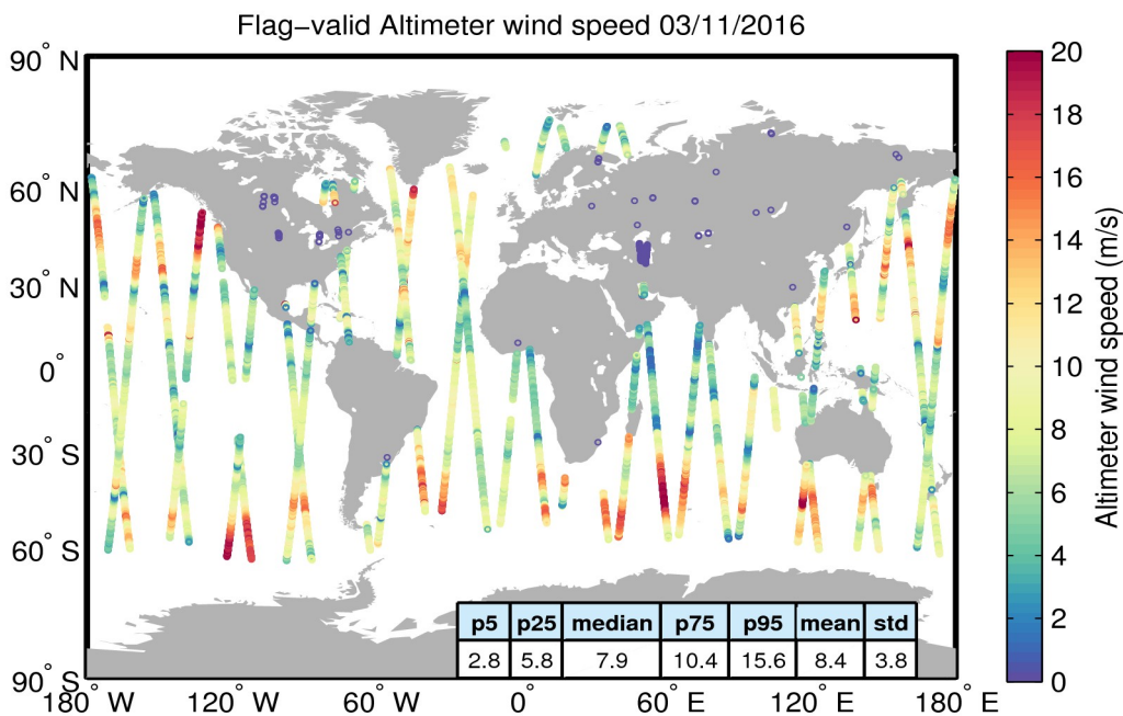
Figure 31. Geographical distribution of flag-valid wind data over oceans and lakes for 03/11/2016. The statistical values shown in the table refer to the wind in m/s and are calculated over all measurements shown in the figure.
