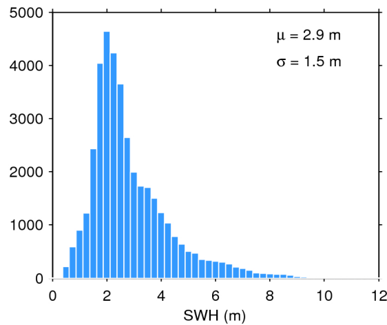
Figure 17. Histogram of flag-valid SWH over oceans and lakes for 03/11/2016. The mean ( \mu ) and standard deviation ( \sigma ) are also shown. Note that values larger than 12 m are excluded from the histogram for the sake of readability but not from the computation of \mu and \sigma .
