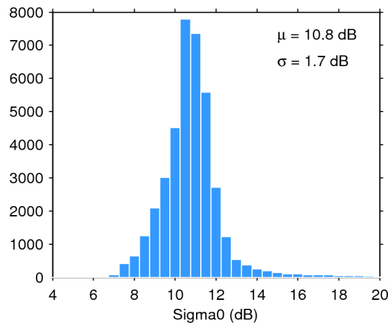
Figure 25. Histogram of flag-valid sigma0 over oceans and lakes for 03/11/2016. The mean ( \mu ) and standard deviation ( \sigma ) are also shown. Note that values outside [4 20] dB are excluded from the histogram for the sake of readability but not from the computation of \mu and \sigma .
