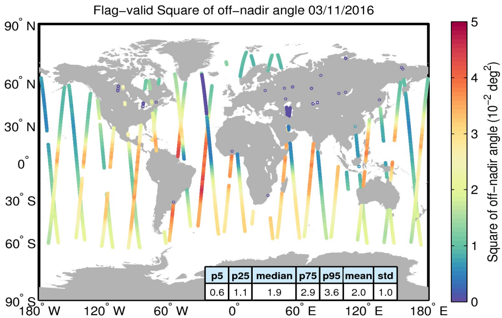
Figure 37. Geographical distribution of flag-valid mispointing data over oceans and lakes for 03/11/2016. The statistical values shown in the table refer to the mispointing in 10^{-2} \text{ deg}^2 and are calculated over all measurements shown in the figure.
