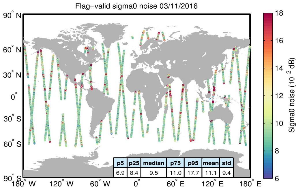
Figure 26. Geographical distribution of flag-valid 20-Hz sigma0 measurement noise over oceans and lakes for 03/11/2016. The statistical values shown in the table refer to the sigma0 noise and are calculated over all measurements shown in the figure.
