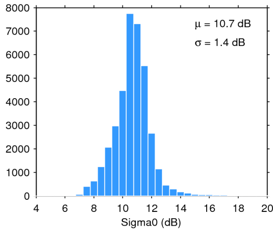
Figure 28. Histogram of science-valid sigma0 over oceans and lakes for 03/11/2016. The mean ( \mu ) and standard deviation ( \sigma ) are also shown. Note that values outside [4 20] dB are excluded from the histogram for the sake of readability but not from the computation of \mu and \sigma .
