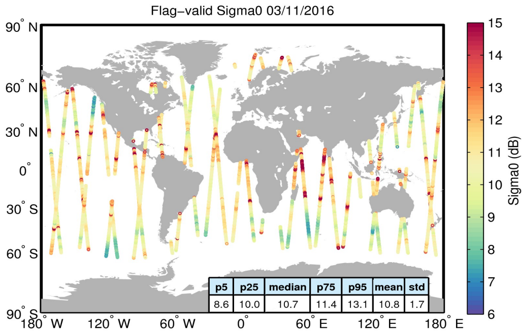
Figure 23. Geographical distribution of flag-valid sigma0 data over oceans and lakes for 03/11/2016. The statistical values shown in the table refer to the sigma0 in dB and are calculated over all measurements shown in the figure.
