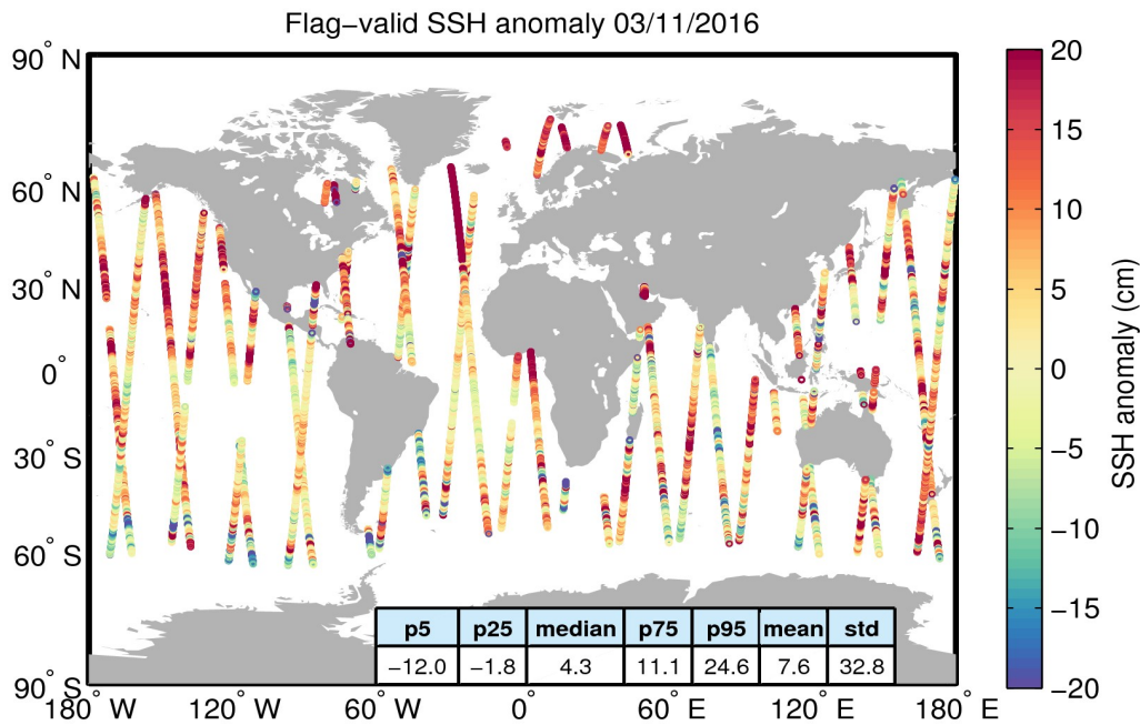
Figure 5. Geographical distribution of flag-valid 1-Hz SSH anomaly data over oceans and lakes for 03/11/2016. The statistical values shown in the table refer to the SSH anomaly in cm and are calculated over all measurements shown in the figure.
