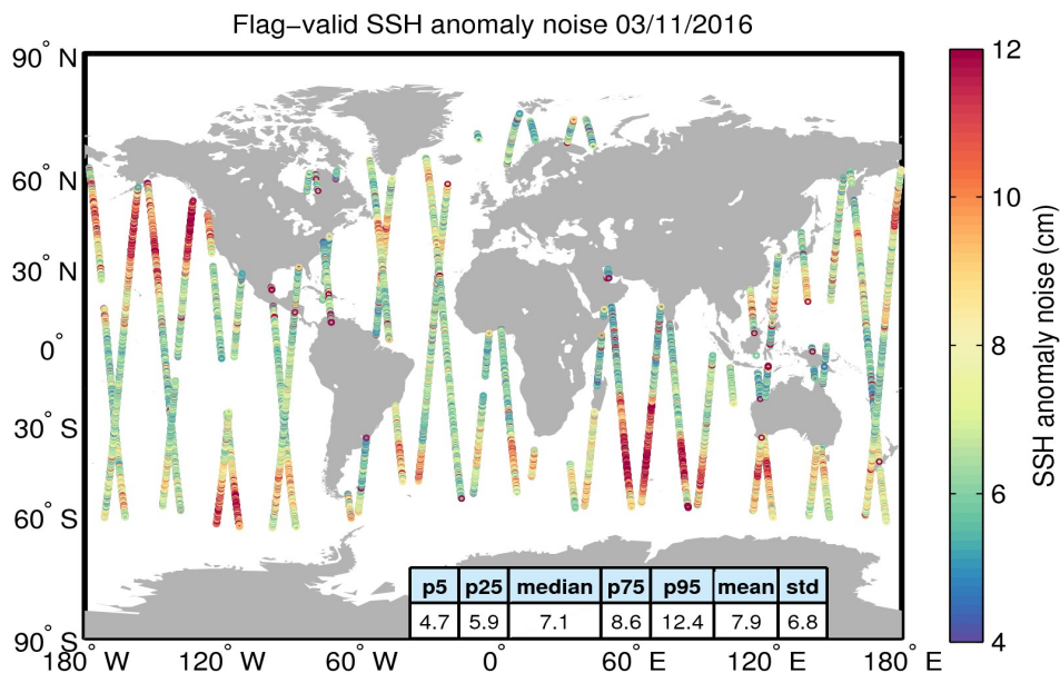
Figure 8. Geographical distribution of flag-valid 20-Hz SSH anomaly measurement noise over oceans and lakes for 03/11/2016. The statistical values shown in the table refer to the SSH anomaly noise and are calculated over all measurements shown in the figure.
