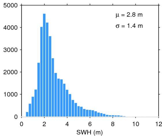
Figure 20. Histogram of science-valid SWH over oceans and lakes for 03/11/2016. The mean ( \mu ) and standard deviation ( \sigma ) are also shown. Note that values larger than 12 m are excluded from the histogram for the sake of readability but not from the computation of \mu and \sigma .
