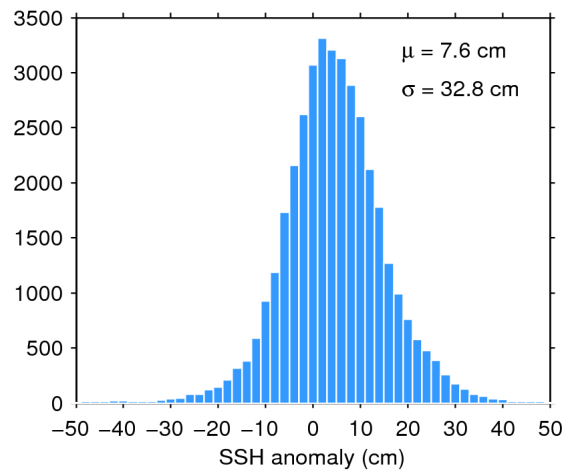
Figure 7. Histogram of flag-valid SSH anomaly over oceans and lakes for 03/11/2016. The mean ( \mu ) and standard deviation ( \sigma ) are also shown. Note that values outside [-50\ 50] cm are excluded from the histogram for the sake of readability but not from the computation of \mu and \sigma .
