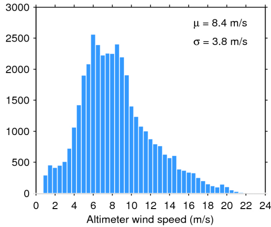
Figure 33. Histogram of flag-valid wind over oceans and lakes for 03/11/2016. The mean ( \mu ) and standard deviation ( \sigma ) are also shown. Note that values larger than 24 m/s are excluded from the histogram for the sake of readability but not from the computation of \mu and \sigma .
