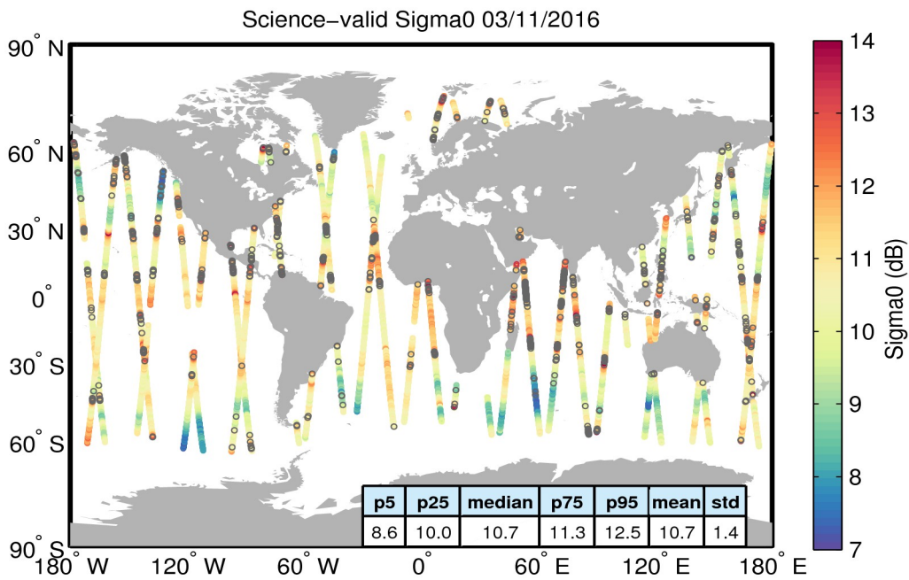
Figure 27. Geographical distribution of science-valid sigma0 data over oceans and lakes for 03/11/2016. The statistical values shown in the table refer to the sigma0 in dB and are calculated over all measurements shown in the figure. Gray circles denote records that have been rejected based on the editing criteria described in Table 4.
