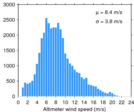
Figure 35. Histogram of science-valid wind over oceans and lakes for 03/11/2016. The mean ( \mu ) and standard deviation ( \sigma ) are also shown. Note that values larger than 24 m/s are excluded from the histogram for the sake of readability but not from the computation of \mu and \sigma .
