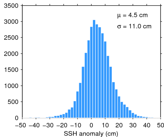
Figure 11. Histogram of science-valid SSH anomaly over oceans and lakes for 03/11/2016. The mean ( \mu ) and standard deviation ( \sigma ) are also shown. Note that values outside [-50 50] cm are excluded from the histogram for the sake of readability but not from the computation of \mu and \sigma .
