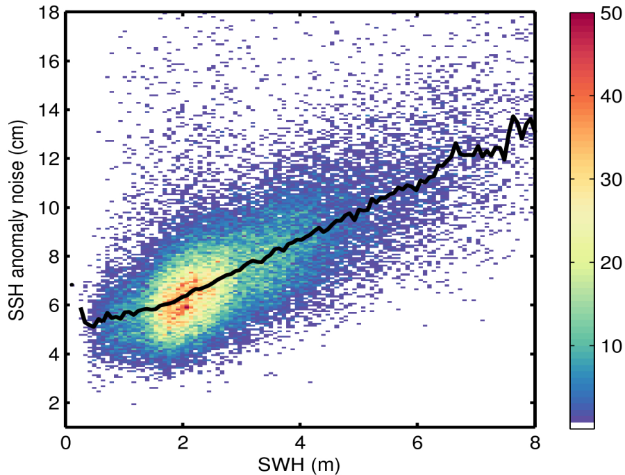
Figure 9. 2D histogram showing flag-valid SSH anomaly noise as a function of SWH for 03/11/2016. The black line denotes the median SSH anomaly noise as a function of SWH.
