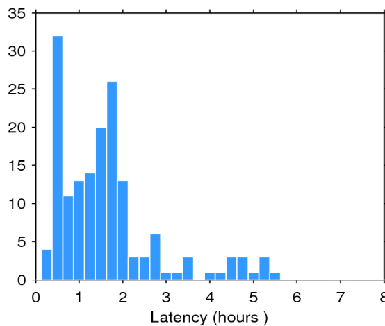
Figure 2. Histogram of the data latency for 03/11/2016. The y-axis denotes the number of files that are made available with a delay of x-hours with respect to the mean time of the records stored in the file.
