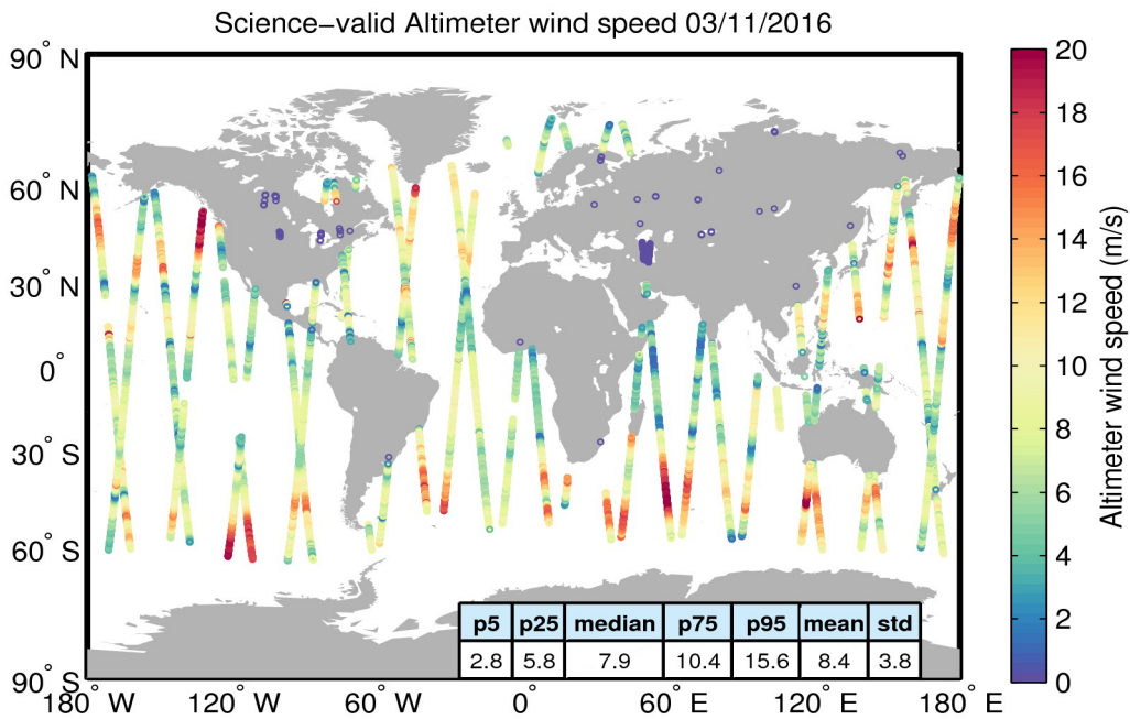
Figure 34. Geographical distribution of science-valid wind data over oceans and lakes for 03/11/2016. The statistical values shown in the table refer to the wind in m/s and are calculated over all measurements shown in the figure. Gray circles denote records that have been rejected based on the editing criteria described in Table 5.
