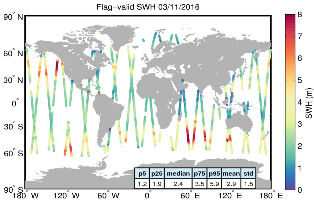
Figure 15. Geographical distribution of flag-valid SWH data over oceans and lakes for 03/11/2016. The statistical values shown in the table refer to the SWH in m and are calculated over all measurements shown in the figure.
