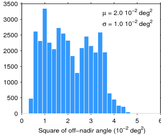
Figure 39. Histogram of flag-valid mispointing over oceans and lakes for 03/11/2016. The mean ( \mu ) and standard deviation ( \sigma ) are also shown. Note that values larger than 6 \cdot 10^{-2} \text{ deg}^2 are excluded from the histogram for the sake of readability but not from the computation of \mu and \sigma .
