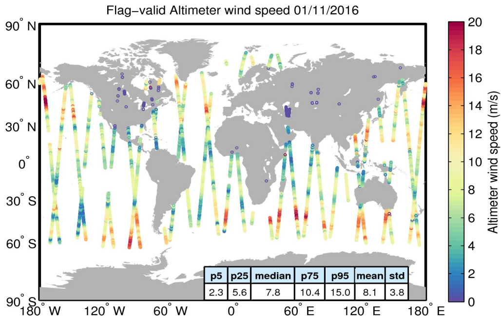
Figure 31. Geographical distribution of flag-valid wind data over oceans and lakes for 01/11/2016. The statistical values shown in the table refer to the wind in m/s and are calculated over all measurements shown in the figure.
