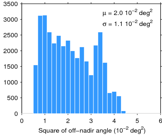
Figure 39. Histogram of flag-valid mispointing over oceans and lakes for 01/11/2016. The mean ( \mu ) and standard deviation ( \sigma ) are also shown. Note that values larger than 6 \cdot 10^{-2} \text{ deg}^2 are excluded from the histogram for the sake of readability but not from the computation of \mu and \sigma .
