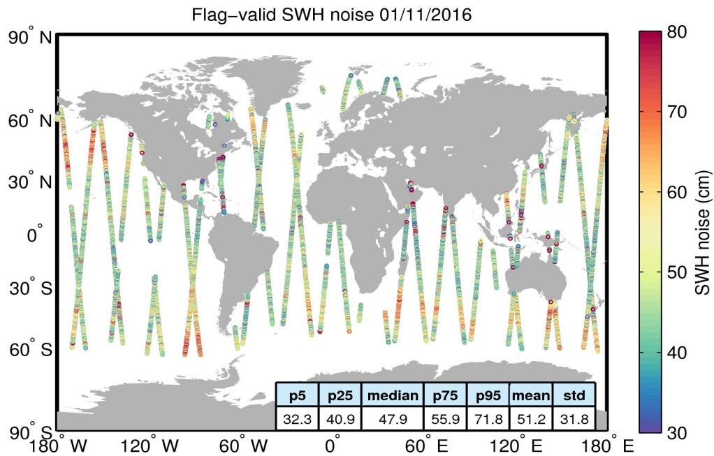
Figure 18. Geographical distribution of flag-valid 20-Hz SWH measurement noise over oceans and lakes for 01/11/2016. The statistical values shown in the table refer to the SWH noise and are calculated over all measurements shown in the figure.
