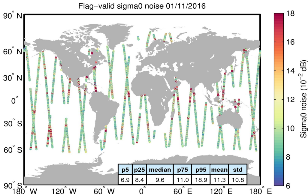
Figure 26. Geographical distribution of flag-valid 20-Hz sigma0 measurement noise over oceans and lakes for 01/11/2016. The statistical values shown in the table refer to the sigma0 noise and are calculated over all measurements shown in the figure.
