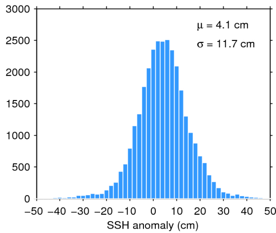
Figure 11. Histogram of science-valid SSH anomaly over oceans and lakes for 01/11/2016. The mean ( \mu ) and standard deviation ( \sigma ) are also shown. Note that values outside [-50 50] cm are excluded from the histogram for the sake of readability but not from the computation of \mu and \sigma .
