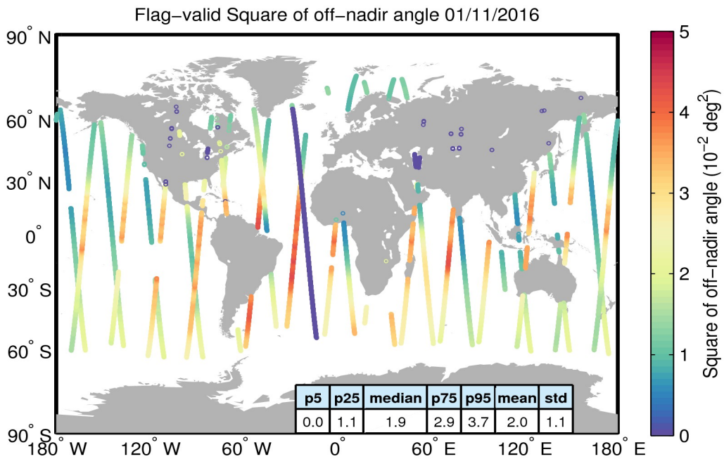
Figure 37. Geographical distribution of flag-valid mispointing data over oceans and lakes for 01/11/2016. The statistical values shown in the table refer to the mispointing in 10^{-2} deg 2 and are calculated over all measurements shown in the figure.
