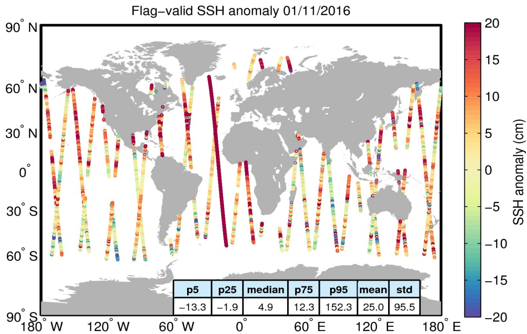
Figure 5. Geographical distribution of flag-valid 1-Hz SSH anomaly data over oceans and lakes for 01/11/2016. The statistical values shown in the table refer to the SSH anomaly in cm and are calculated over all measurements shown in the figure.
