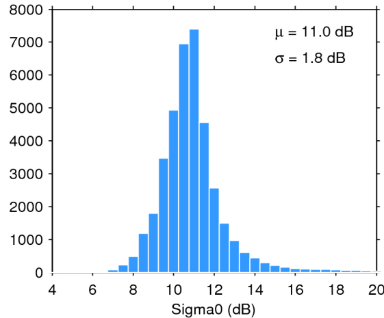
Figure 25. Histogram of flag-valid sigma0 over oceans and lakes for 01/11/2016. The mean ( \mu ) and standard deviation ( \sigma ) are also shown. Note that values outside [4 20] dB are excluded from the histogram for the sake of readability but not from the computation of \mu and \sigma .
