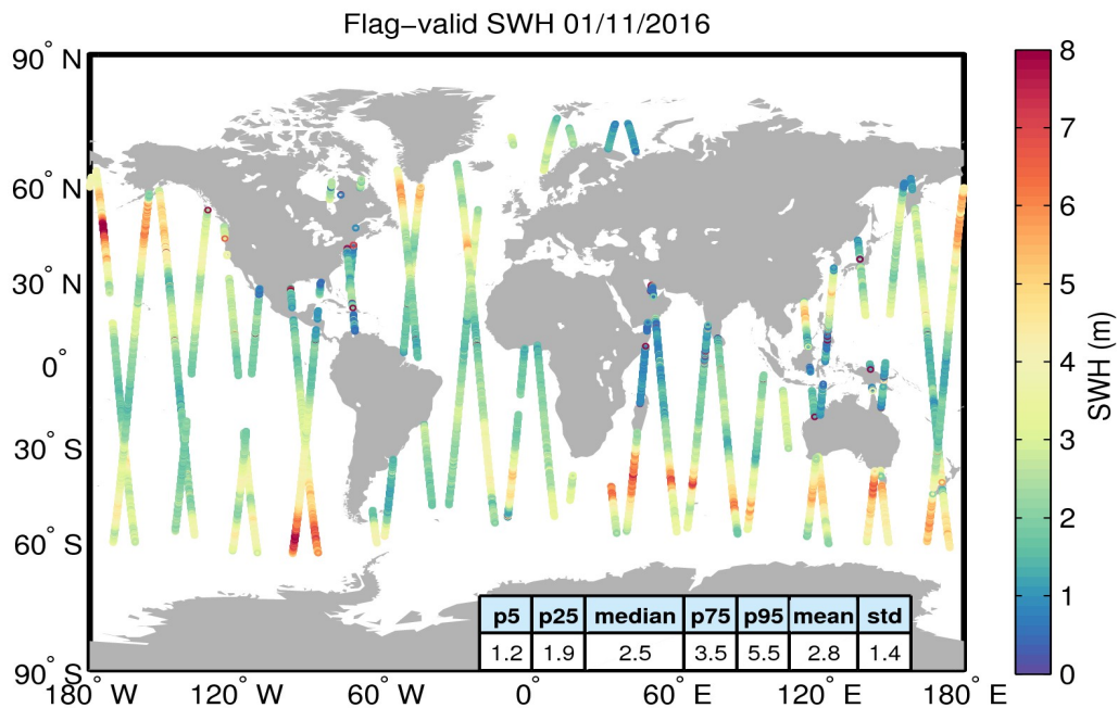
Figure 15. Geographical distribution of flag-valid SWH data over oceans and lakes for 01/11/2016. The statistical values shown in the table refer to the SWH in m and are calculated over all measurements shown in the figure.
