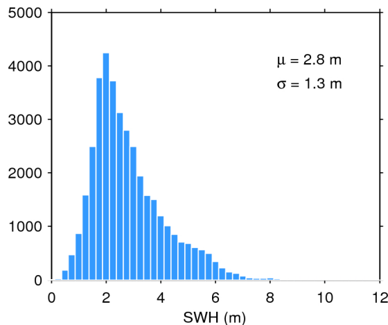
Figure 20. Histogram of science-valid SWH over oceans and lakes for 01/11/2016. The mean ( \mu ) and standard deviation ( \sigma ) are also shown. Note that values larger than 12 m are excluded from the histogram for the sake of readability but not from the computation of \mu and \sigma .
