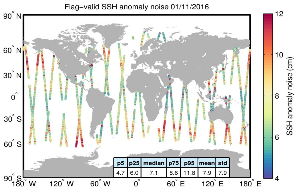
Figure 8. Geographical distribution of flag-valid 20-Hz SSH anomaly measurement noise over oceans and lakes for 01/11/2016. The statistical values shown in the table refer to the SSH anomaly noise and are calculated over all measurements shown in the figure.
