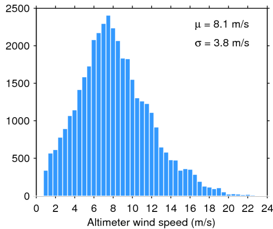
Figure 33. Histogram of flag-valid wind over oceans and lakes for 01/11/2016. The mean ( \mu ) and standard deviation ( \sigma ) are also shown. Note that values larger than 24 m/s are excluded from the histogram for the sake of readability but not from the computation of \mu and \sigma .
