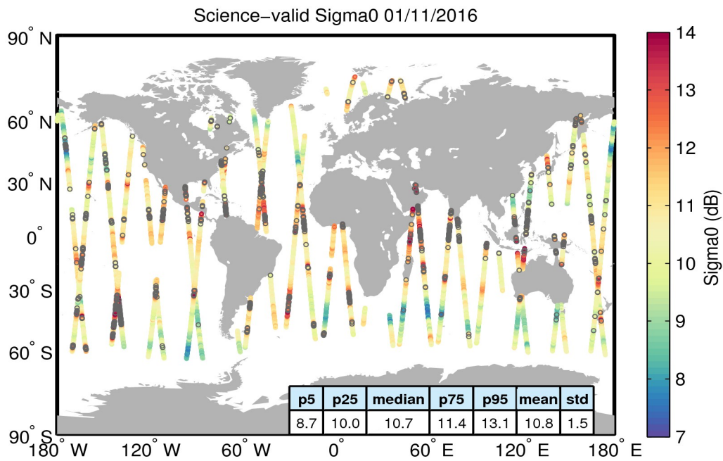
Figure 27. Geographical distribution of science-valid sigma0 data over oceans and lakes for 01/11/2016. The statistical values shown in the table refer to the sigma0 in dB and are calculated over all measurements shown in the figure. Gray circles denote records that have been rejected based on the editing criteria described in Table 4.
