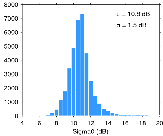
Figure 28. Histogram of science-valid sigma0 over oceans and lakes for 01/11/2016. The mean ( \mu ) and standard deviation ( \sigma ) are also shown. Note that values outside [4 20] dB are excluded from the histogram for the sake of readability but not from the computation of \mu and \sigma .
