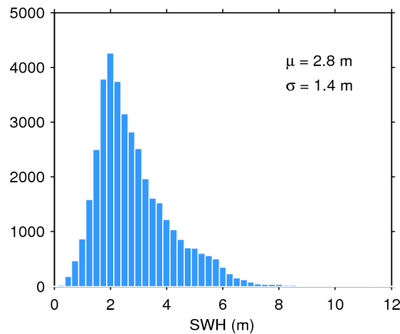
Figure 17. Histogram of flag-valid SWH over oceans and lakes for 01/11/2016. The mean ( \mu ) and standard deviation ( \sigma ) are also shown. Note that values larger than 12 m are excluded from the histogram for the sake of readability but not from the computation of \mu and \sigma .
