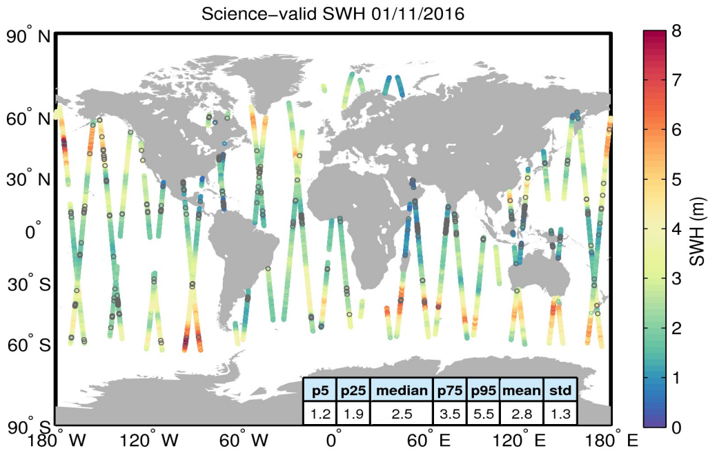
Figure 19. Geographical distribution of science-valid SWH data over oceans and lakes for 01/11/2016. The statistical values shown in the table refer to the SWH in m and are calculated over all measurements shown in the figure. Gray circles denote records that have been rejected based on the editing criteria described in Table 3.
