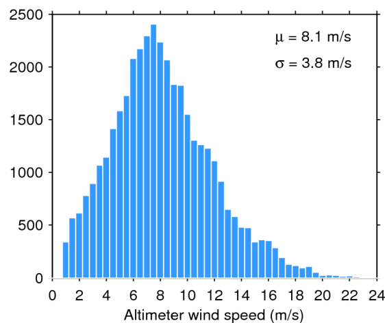
Figure 35. Histogram of science-valid wind over oceans and lakes for 01/11/2016. The mean ( \mu ) and standard deviation ( \sigma ) are also shown. Note that values larger than 24 m/s are excluded from the histogram for the sake of readability but not from the computation of \mu and \sigma .
