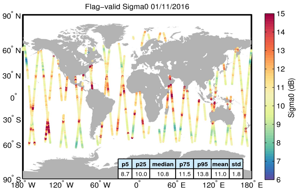
Figure 23. Geographical distribution of flag-valid sigma0 data over oceans and lakes for 01/11/2016. The statistical values shown in the table refer to the sigma0 in dB and are calculated over all measurements shown in the figure.
