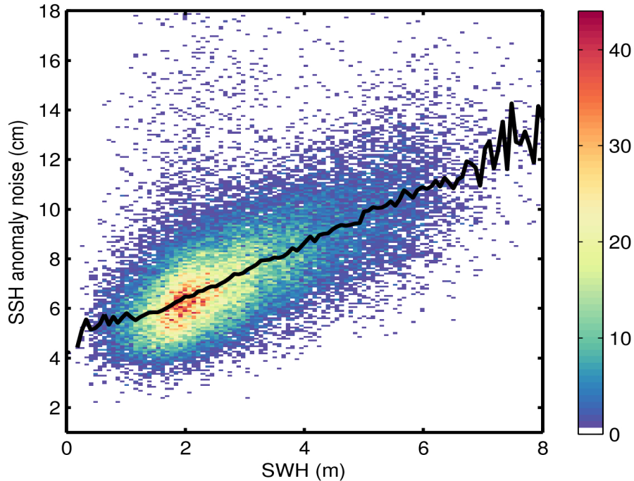
Figure 9. 2D histogram showing flag-valid SSH anomaly noise as a function of SWH for 01/11/2016. The black line denotes the median SSH anomaly noise as a function of SWH.
