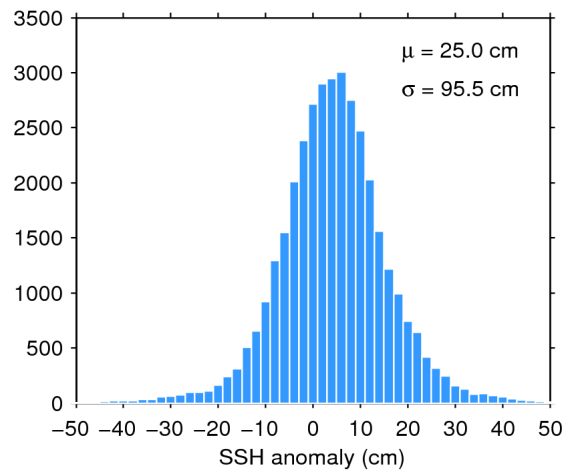
Figure 7. Histogram of flag-valid SSH anomaly over oceans and lakes for 01/11/2016. The mean ( \mu ) and standard deviation ( \sigma ) are also shown. Note that values outside [-50 50] cm are excluded from the histogram for the sake of readability but not from the computation of \mu and \sigma .
